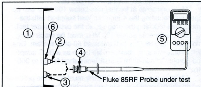
Figure 1. Schematic Diagram
