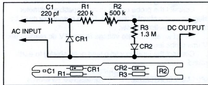
Figure 1. Schematic Diagram
