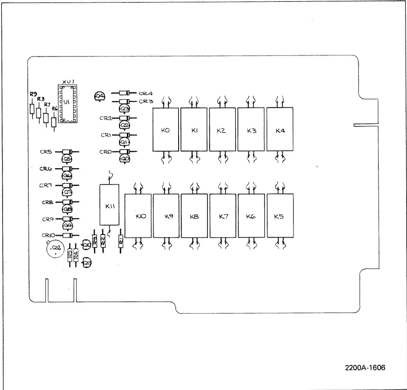
Figure 605-5. General Purpose Scanner PCB Assembly
