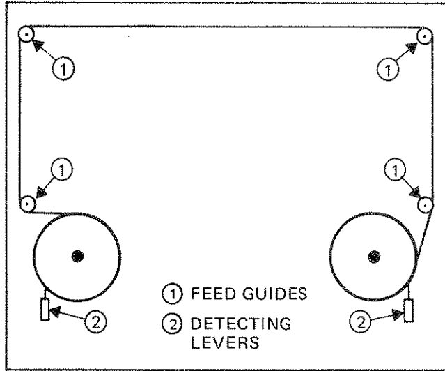
Figure 2-2. Properly Installed Ribbon
