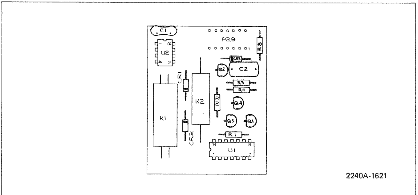
Figure 643-3. Temperature Option PCB Assembly
