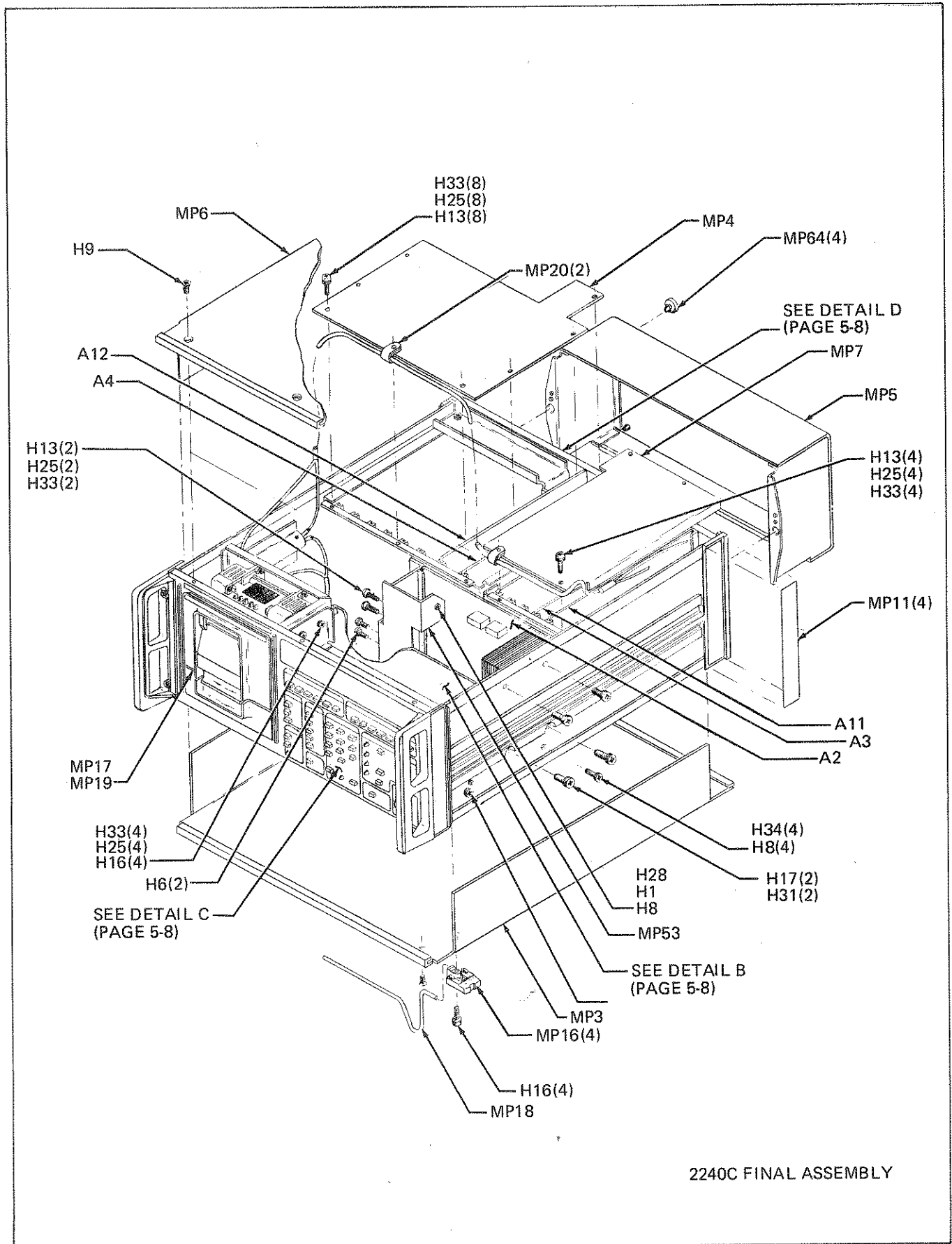
Figure 5-1. 2240C Final Assembly
