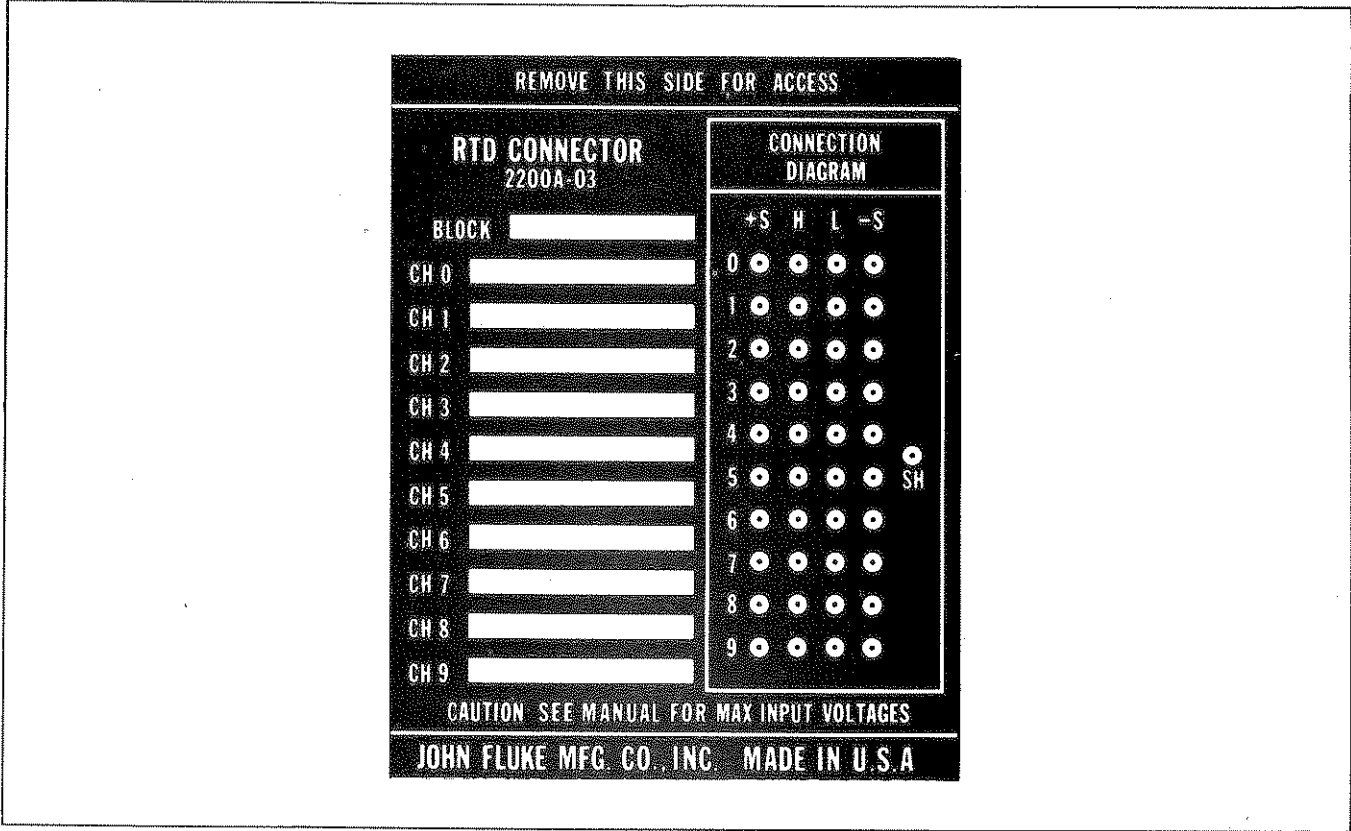
Figure 603-2. RTD Connector Terminal Assignments
