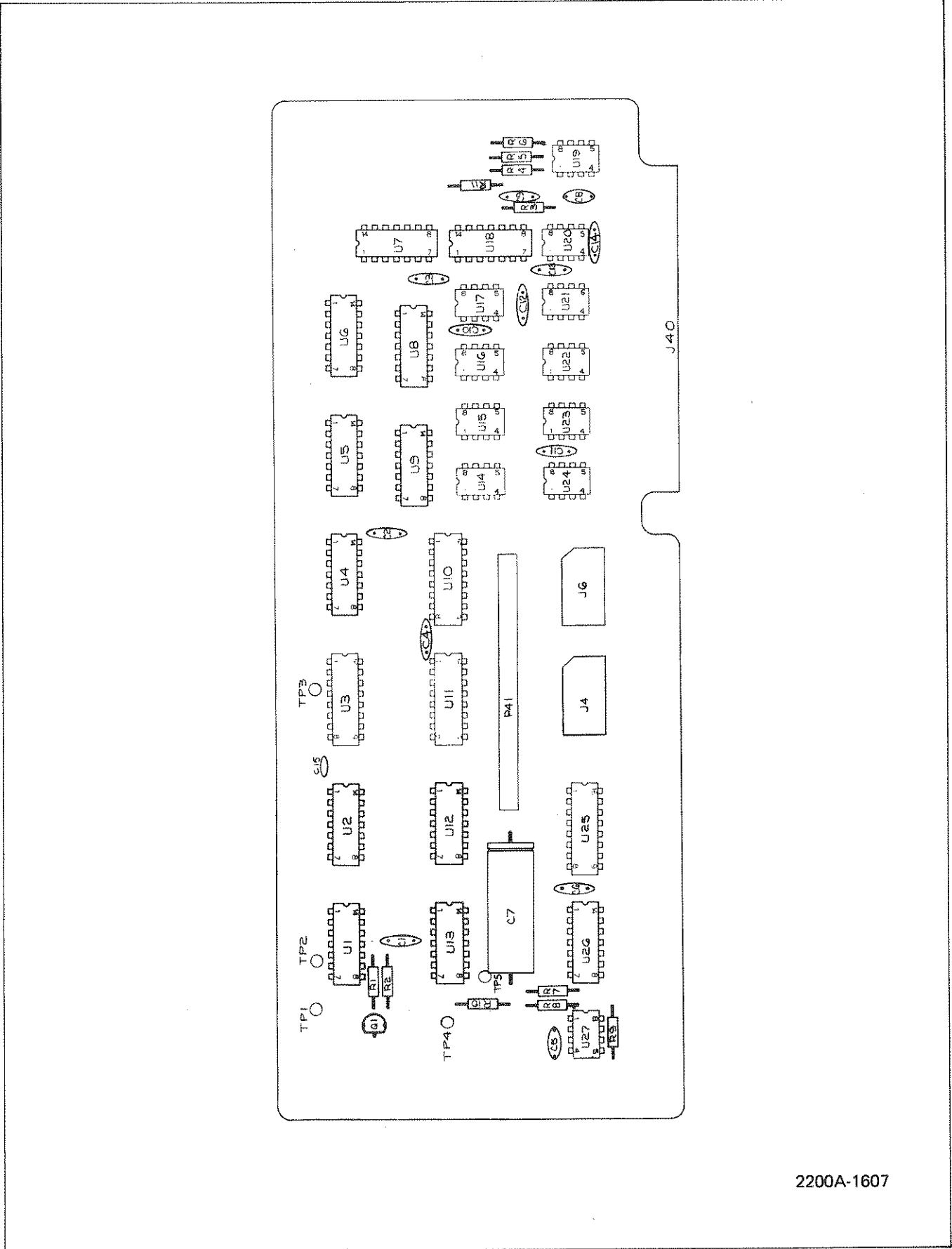
Figure 5-6. A5 Printer Drive PCB Assembly
