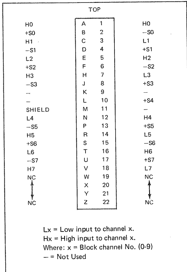
Figure 633-1. RTD Scanner Rear Panel Connector Pin Assignments
