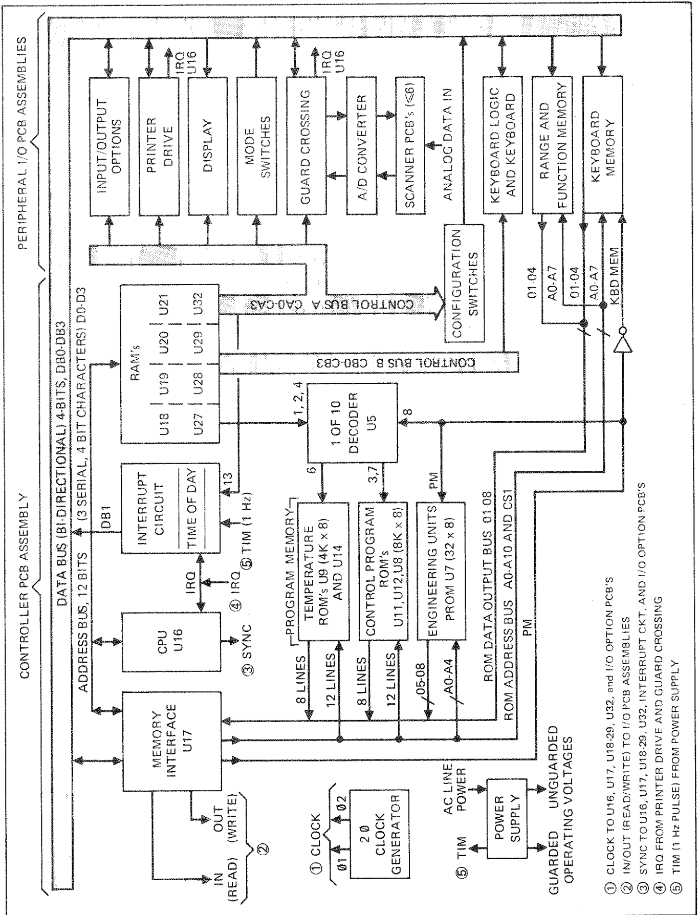
Figure 3-2. 2240C Data Logger, Detailed Block Diagram
