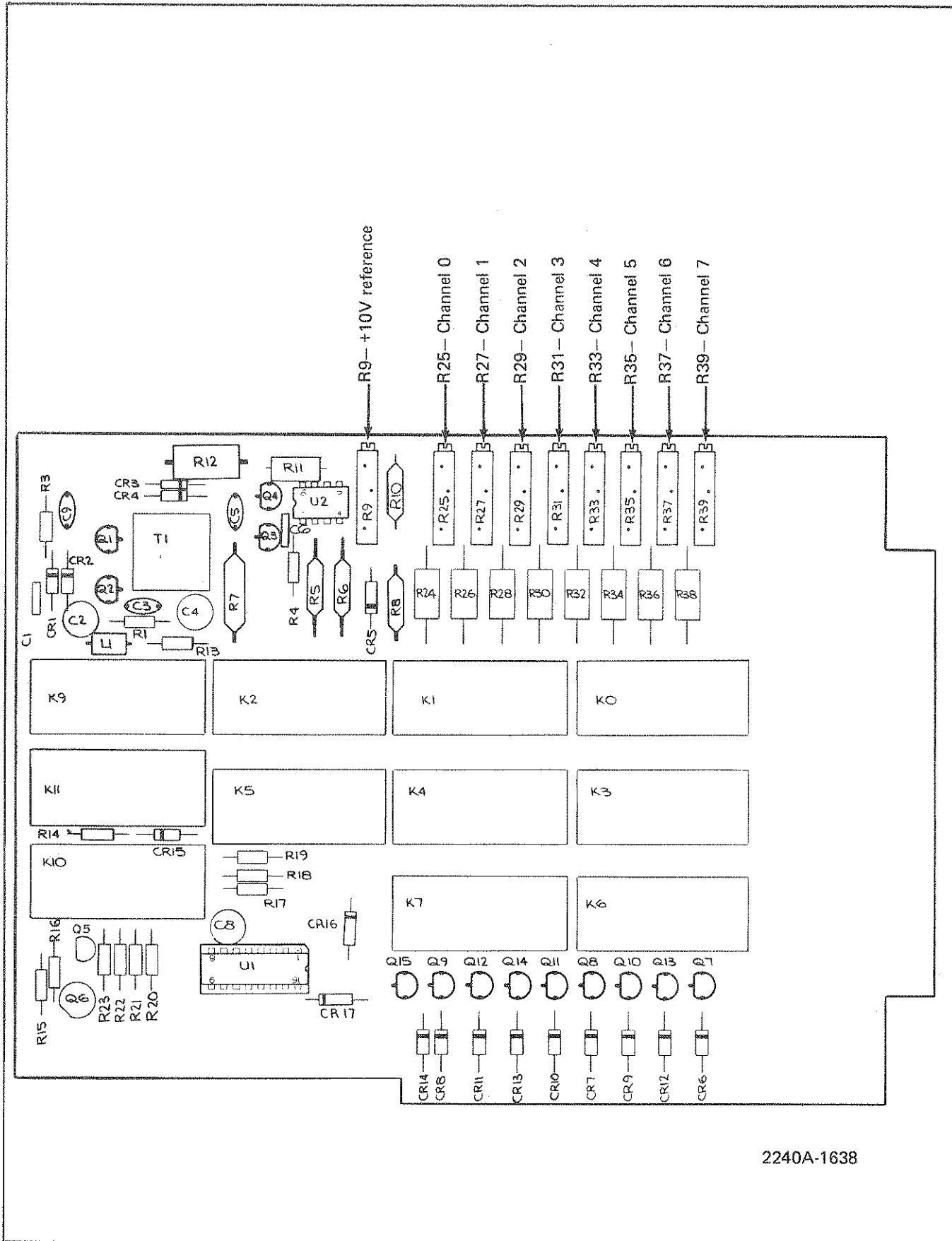
Figure 633-4. Eight Channel RTD Scanner PCB Assembly
