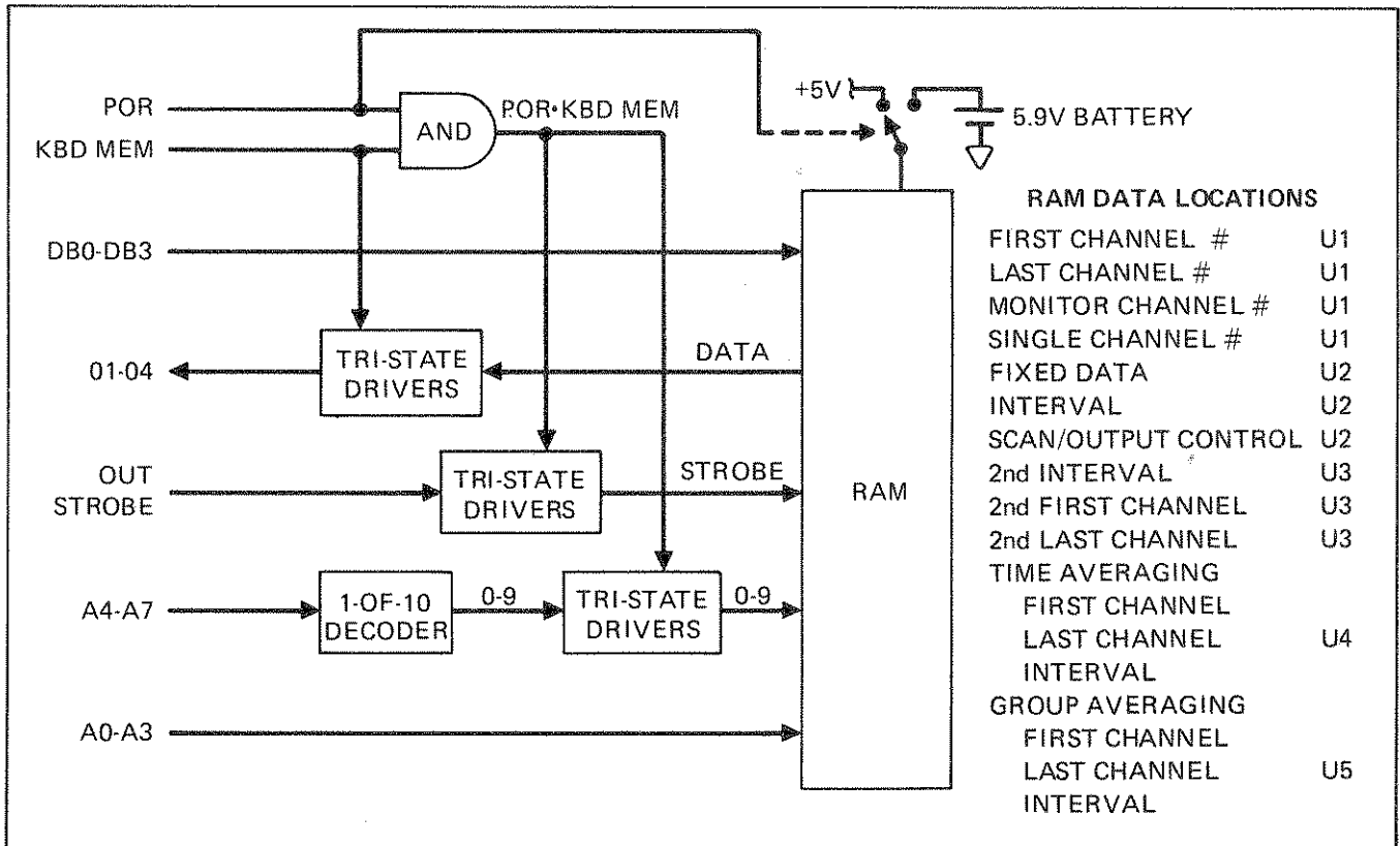
Figure 3-5. Keyboard Memory, Simplified Block Diagram
