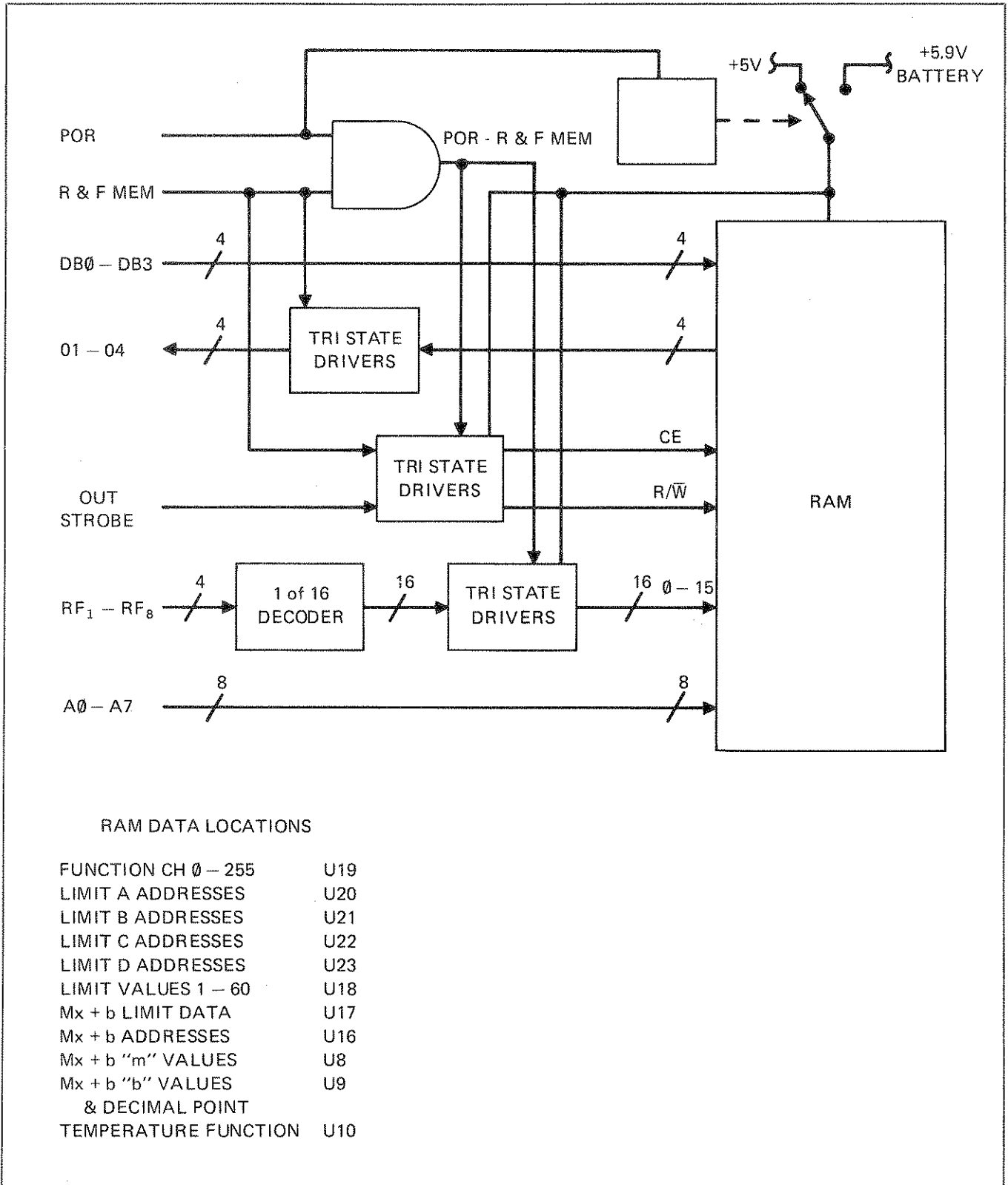
Figure 3-10. Range and Function Memory PCB Block Diagram
