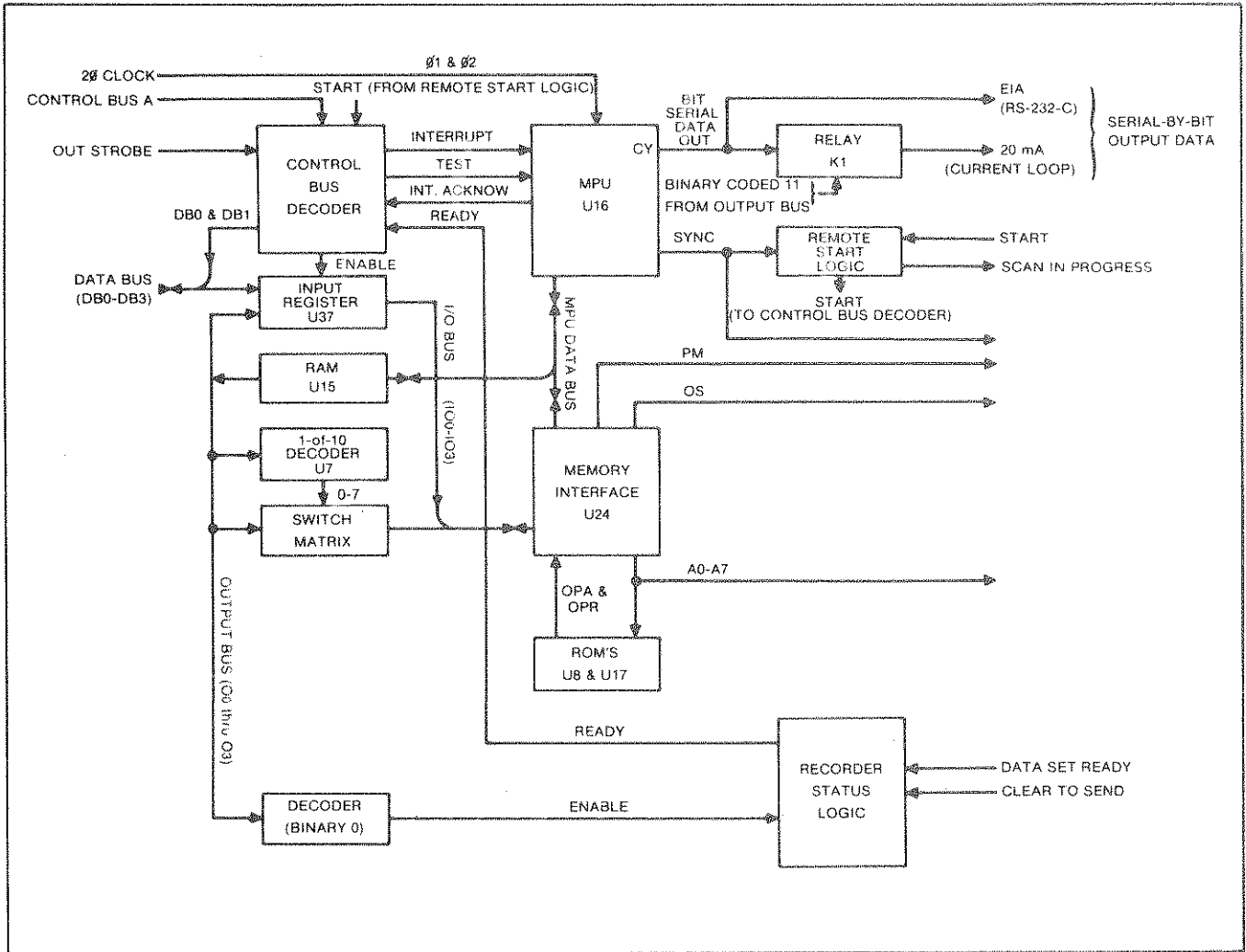
Figure 612-3. Digital Output PCB Simplified Block Diagram
