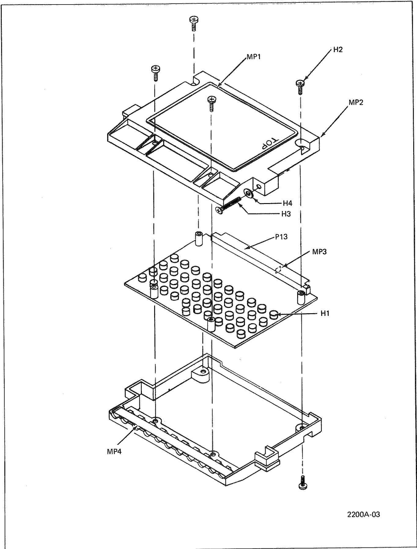
Figure 603-2. RTD Connector Assembly
