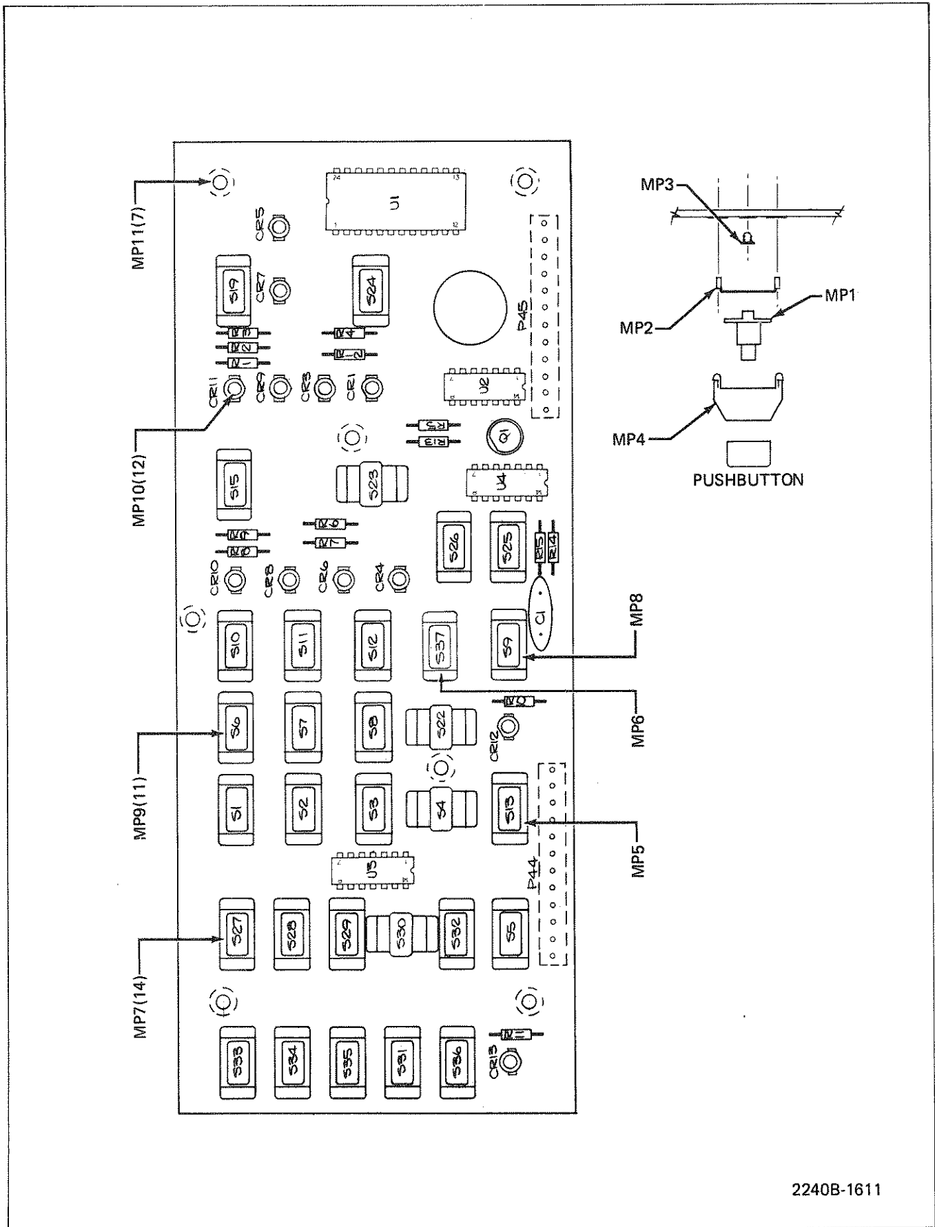
Figure 5-9. A8 Keyboard Switch PCB Assembly
