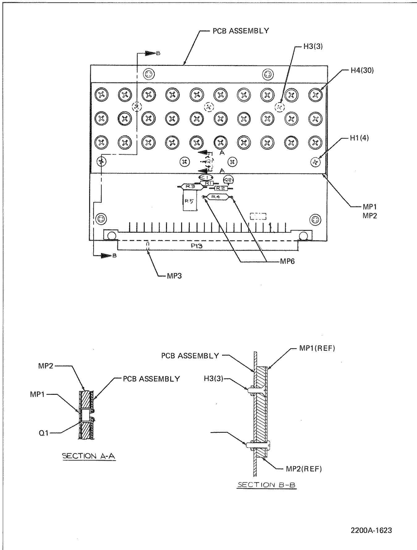
Figure 608-3. Isothermal Block Connector
