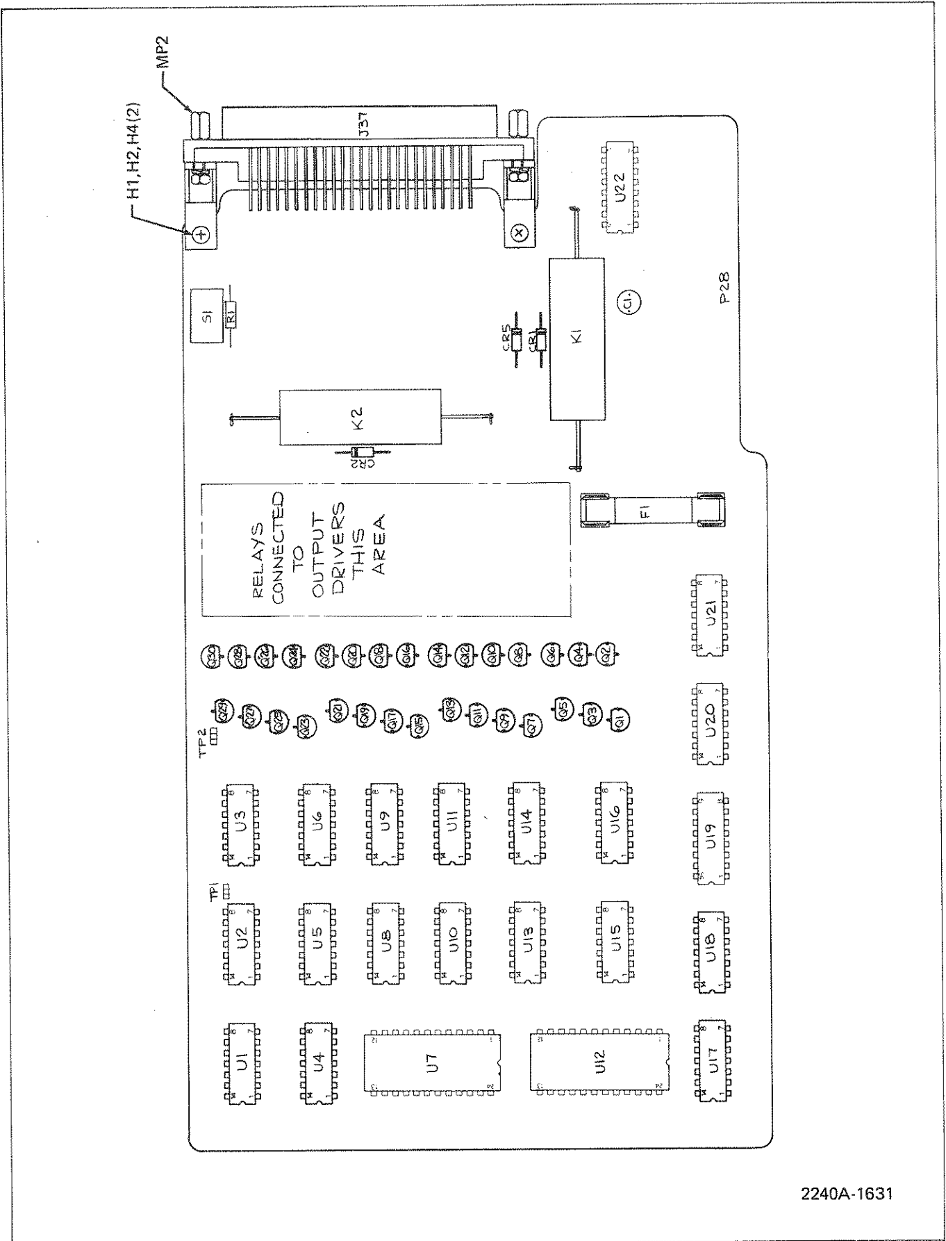
Figure 623-7. Alarm Set Point Output PCB Assembly
