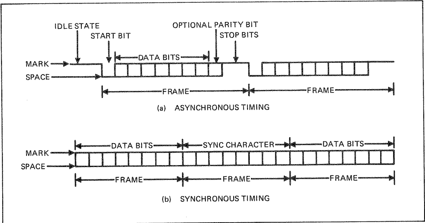
Figure 617-1. RS-232-C Timing Formats
