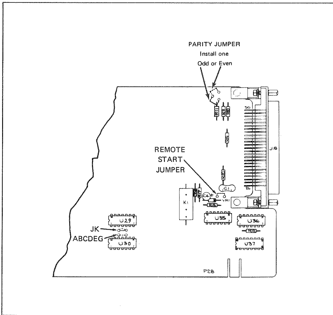
Figure 614-3. Jumper Location, -14 Series Options
