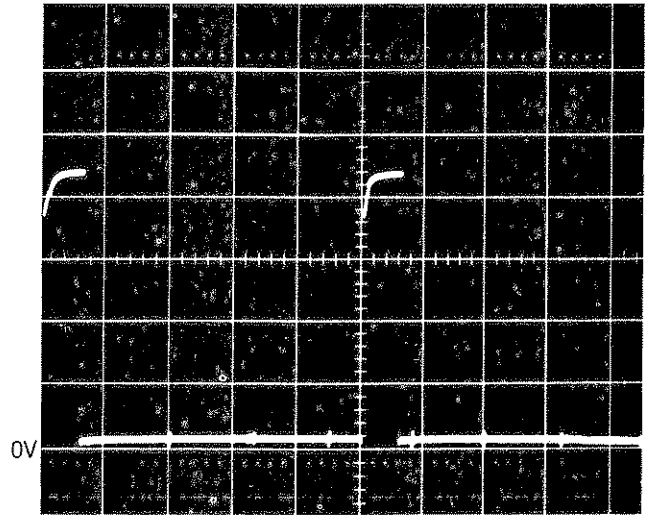
TEST POINT: TP RD+WR 2.0 \mu s/div. 0.1V/div. UNDER CONTROL OF FLUKE 1720A (PULSES BECOME RANDOM WITHOUT CONTROLLER CONNECTED)
