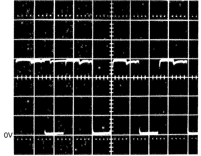
TEST POINT: U4-9 ( \overline{PSEN} ) 1.0 \mu s/div. 0.1V/div.
