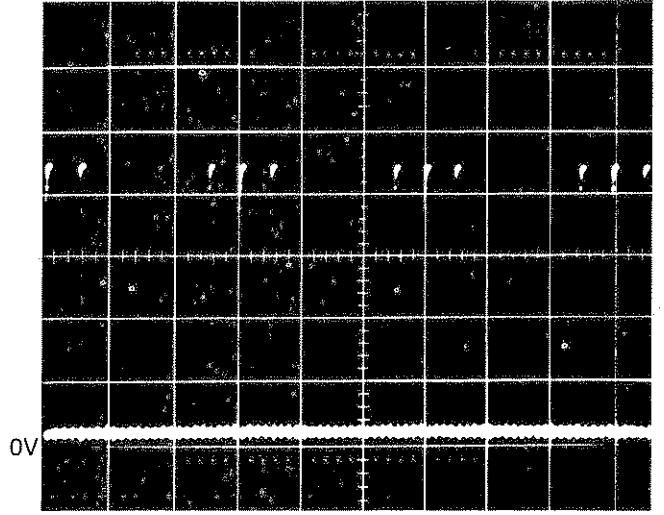
TEST POINT: TP RD+WR 20 \mu s/div. 0.1V/div. UNDER CONTROL OF FLUKE 1720A
