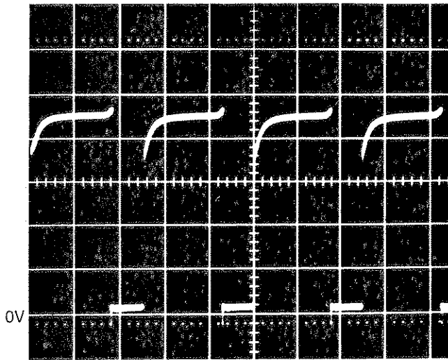
TEST POINT: U9-8 1.0 \mu s/div. 1.0V/div.
