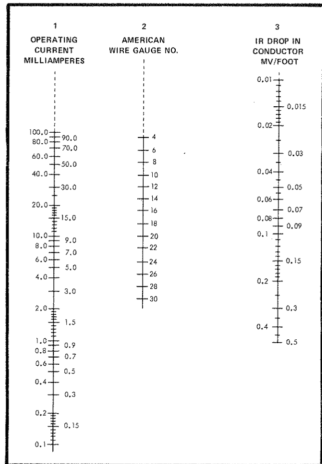
Figure 2-4. NOMOGRAPH OF VOLTAGE DROP ACROSS LOAD WIRES
