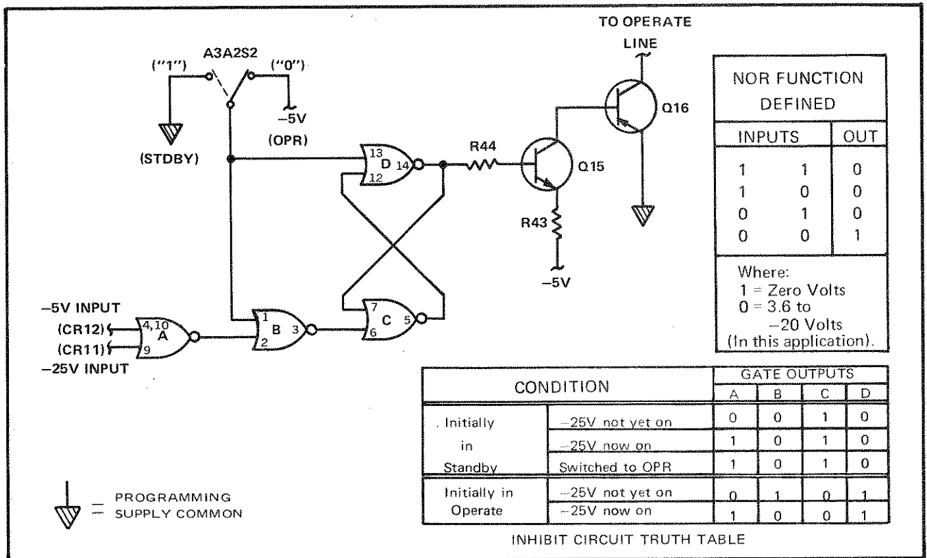
Figure 3-8. INHIBIT CIRCUIT
