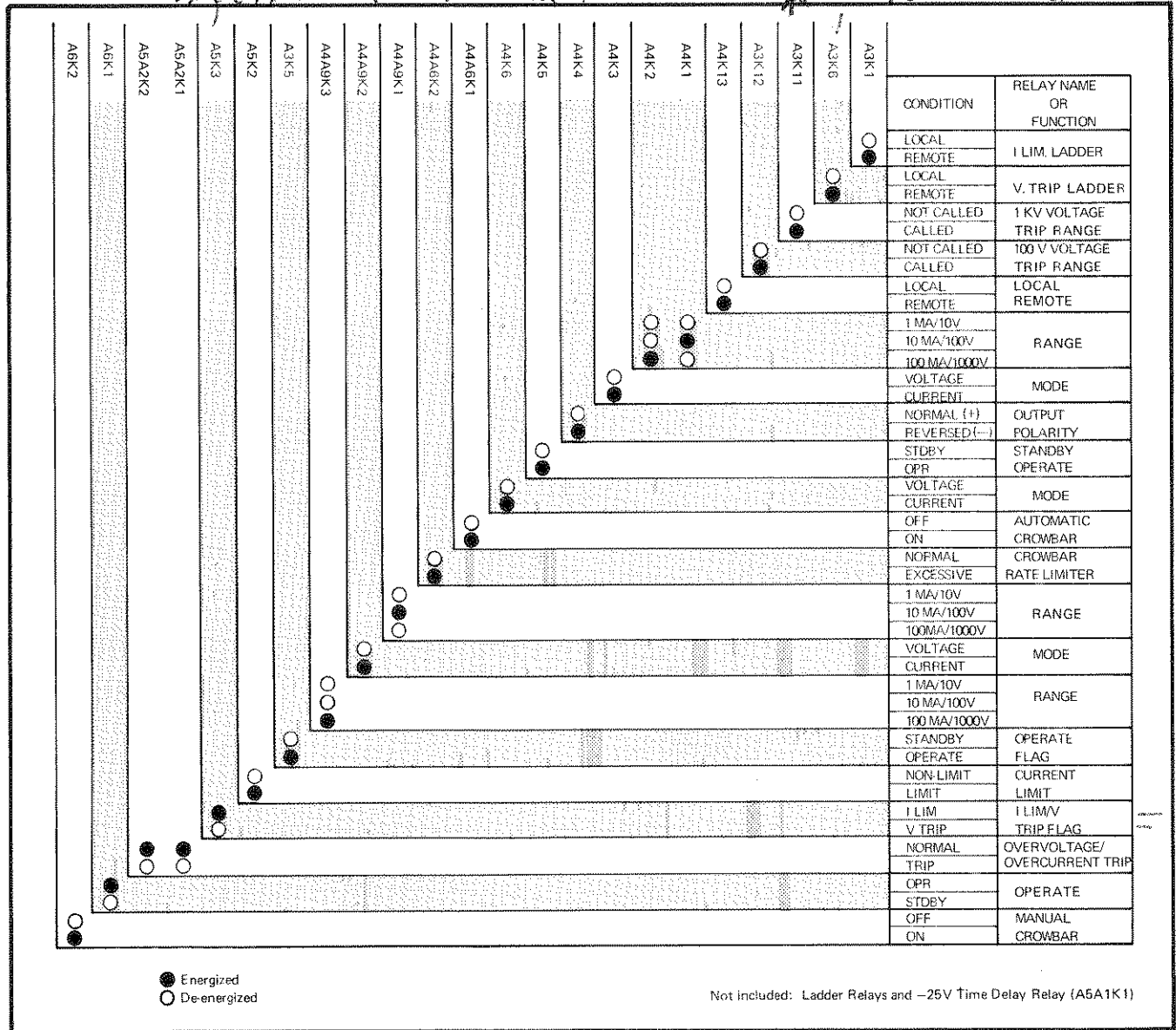
Figure 3-9. RELAY SUMMARY
