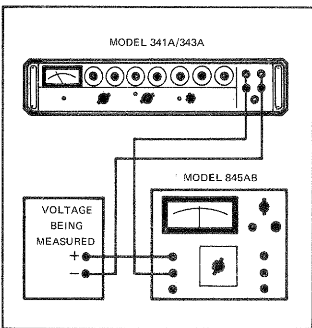
Figure 2-3. DIFFERENTIAL VOLTMETER
