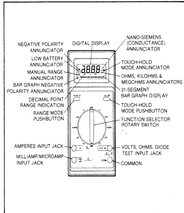
Figure 2-3. 8025A Features
