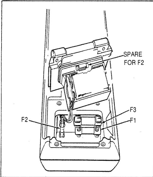
Figure 2-2. Fuse Replacement
