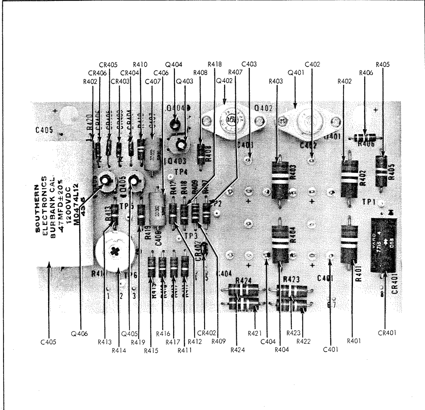
Figure 5-9. HIGH VOLTAGE BOARD ASSEMBLY
