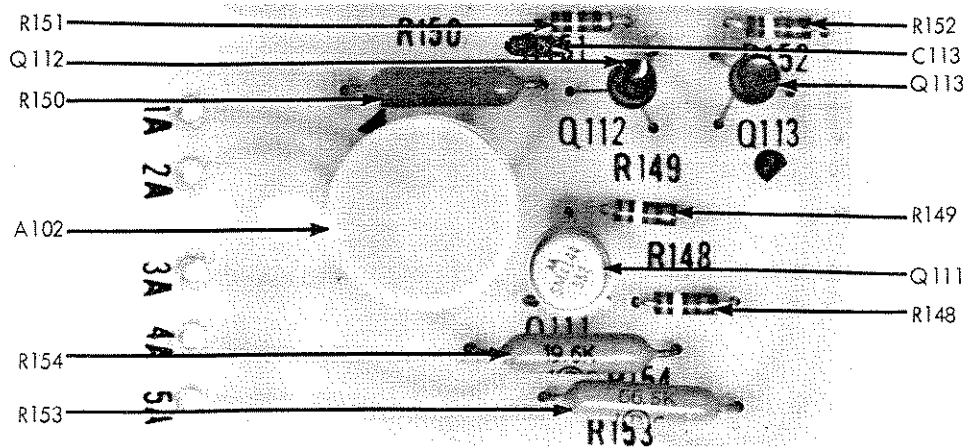
Figure 5-6. ZENER DIODE OVEN ASSEMBLY
