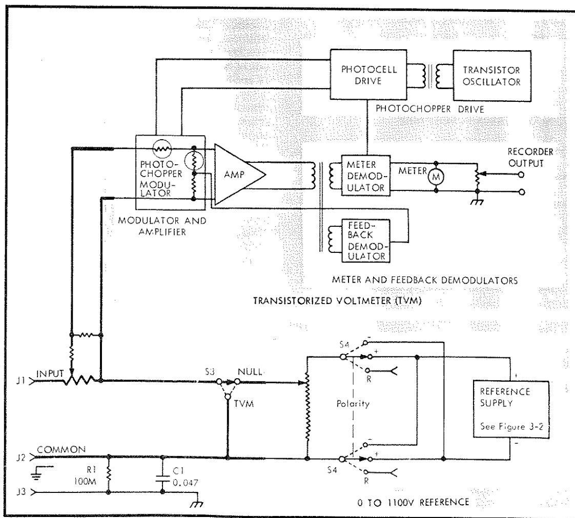
Figure 3-1. MODEL 895A BLOCK DIAGRAM
