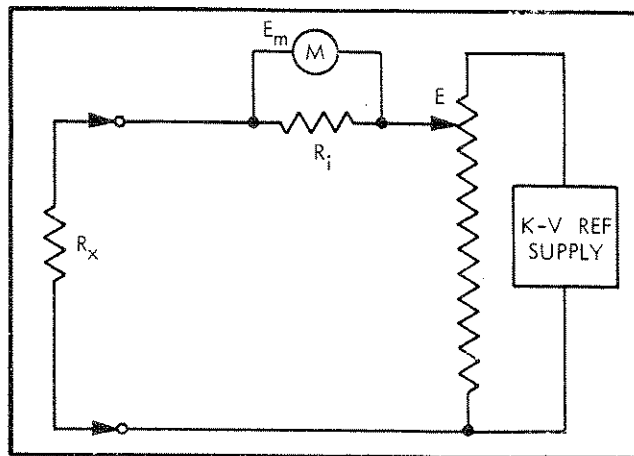
Figure 2-4. MEASUREMENT OF RESISTANCE
