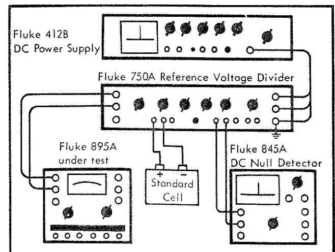
Figure 4-3. SOURCE FOR TEST VOLTAGES
