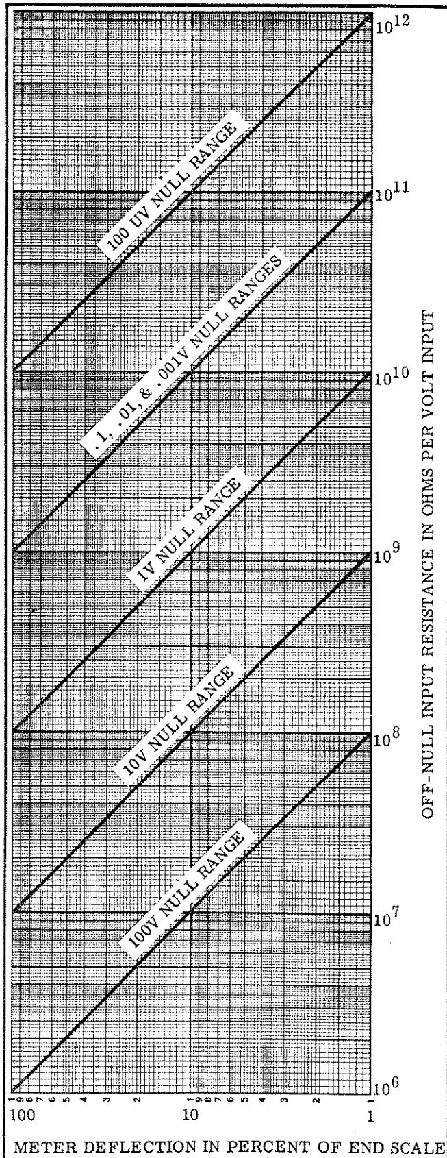
Figure 2-7. OFF-NULL INPUT RESISTANCE
