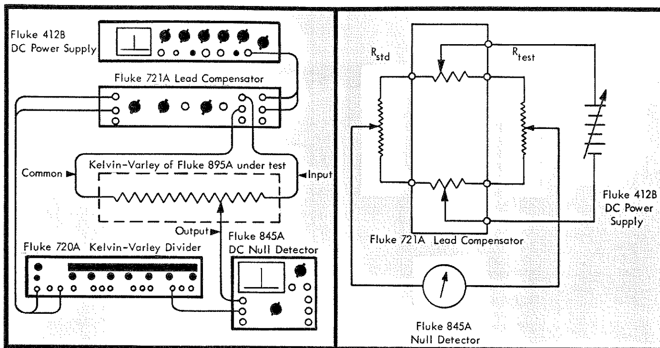
Figure 4-6. KELVIN-VARLEY DIVIDER TEST
