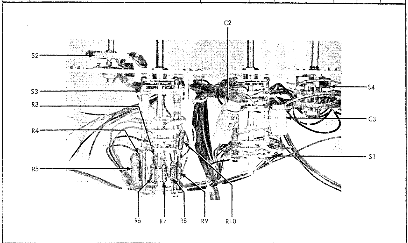
Figure 5-4. SWITCH ASSEMBLY
