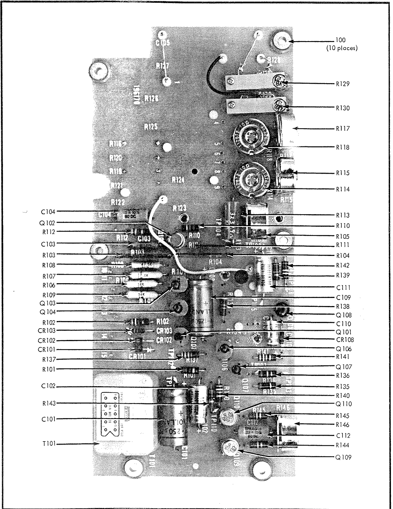
Figure 5-5. REFERENCE SUPPLY BOARD ASSEMBLY (Sheet 2 of 2)
