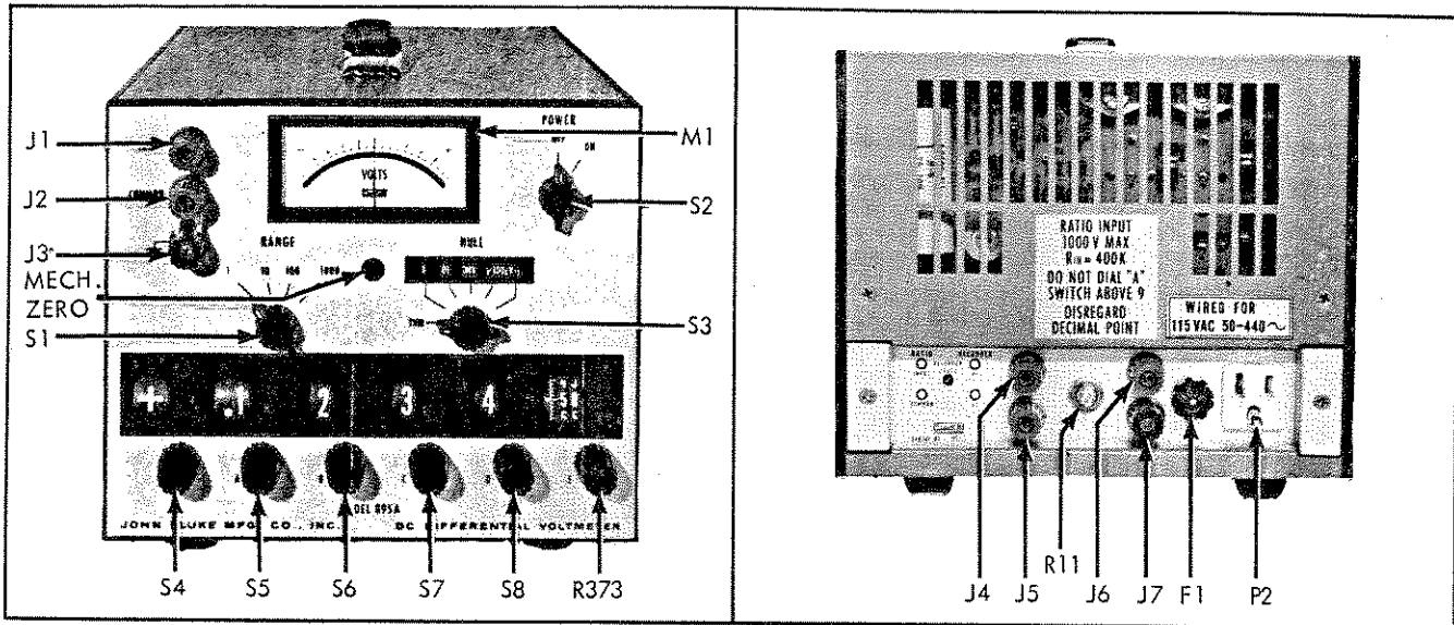
Figure 2-1. LOCATION OF CONTROLS, TERMINALS, AND INDICATORS
