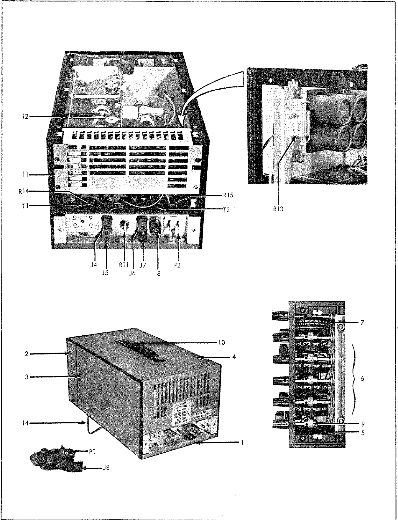
Figure 5-2. CHASSIS ASSEMBLY
