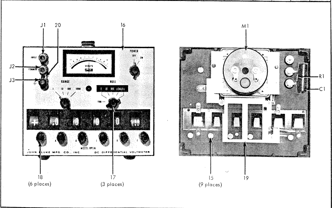
Figure 5-3. FRONT PANEL ASSEMBLY
