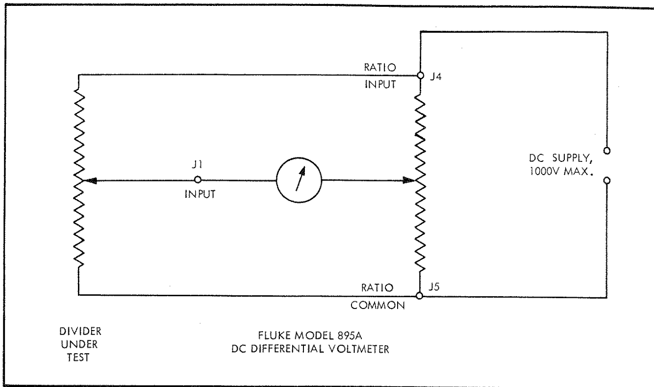
Figure 2-6. MEASUREMENT OF RESISTANCE RATIOS
