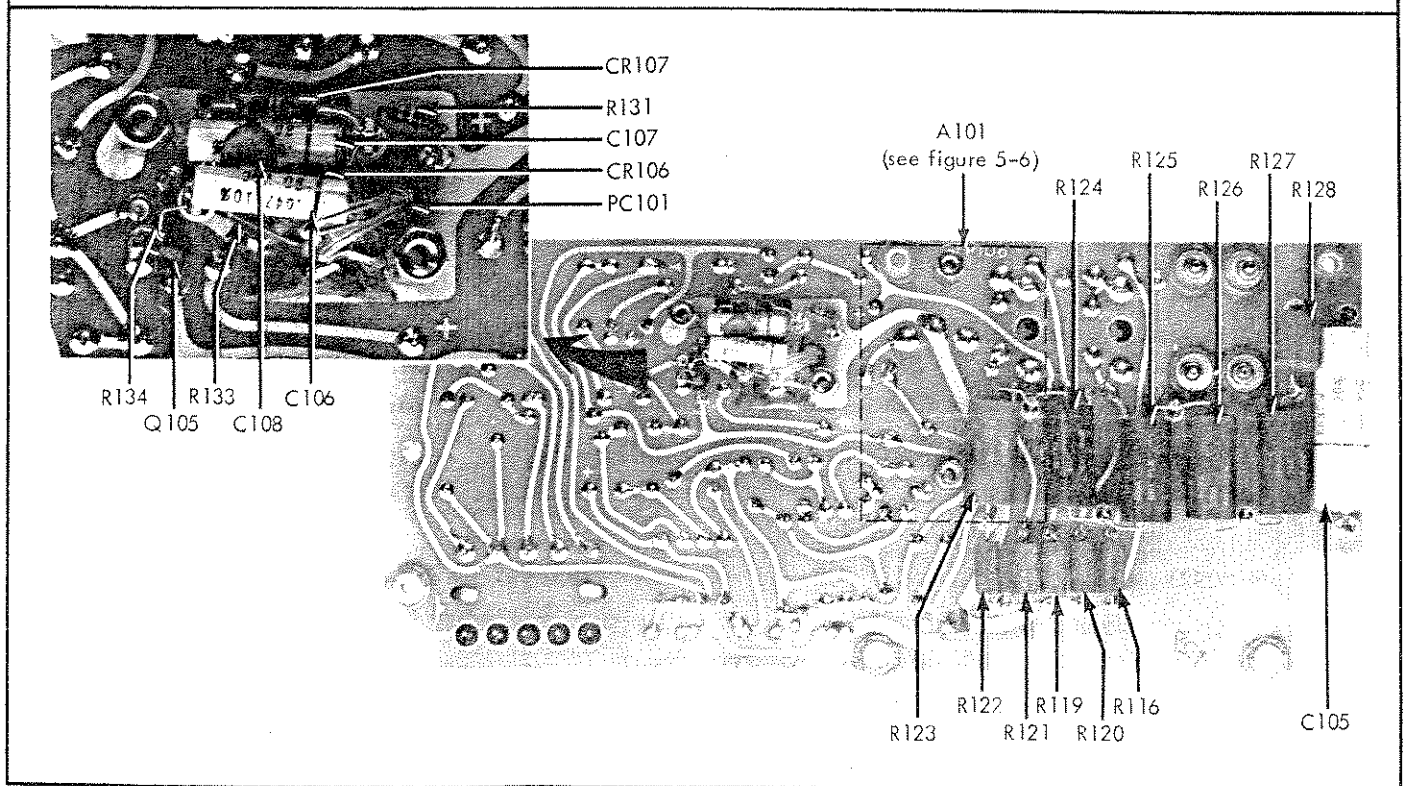
Figure 5-5. REFERENCE SUPPLY BOARD ASSEMBLY (Sheet 1 of 2)
