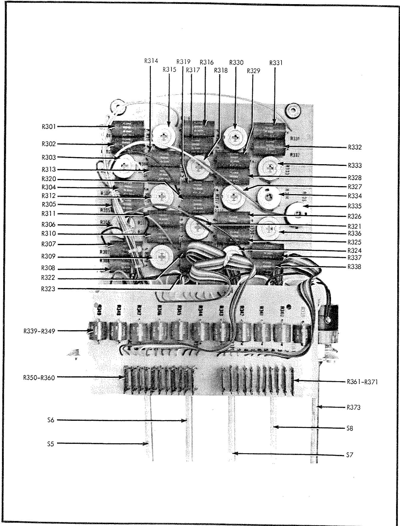
Figure 5-8. KELVIN-VARLEY BOARD ASSEMBLY
