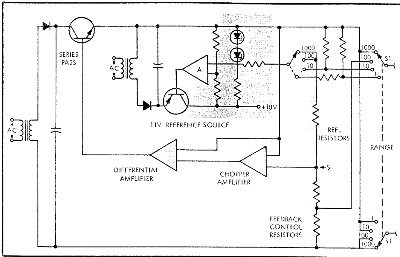
Figure 3-2. +1100 VOLT REFERENCE SUPPLY
