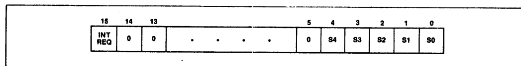
Figure H-23. Poll Register Format
