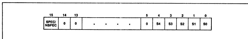
Figure H-22. EOI Register Format
