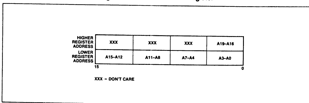
Figure H-10a. DMA Memory Pointer Register Format
