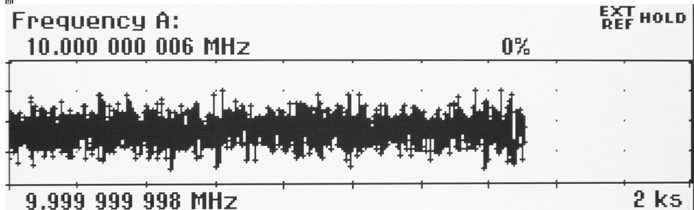
HP Z 3805A as extRef and DUT smart Freq off_1 Sec GateTime Plot.JPG (140.64 kB, 1538x465 - viewed 136 times.)
