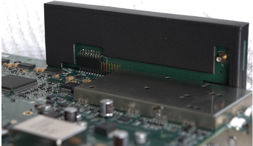
Tektronix FCA 3000 Fluke PM 9624 Shield 1 .jpg (304.02 kB, 1254x740 - viewed 277 times.)
