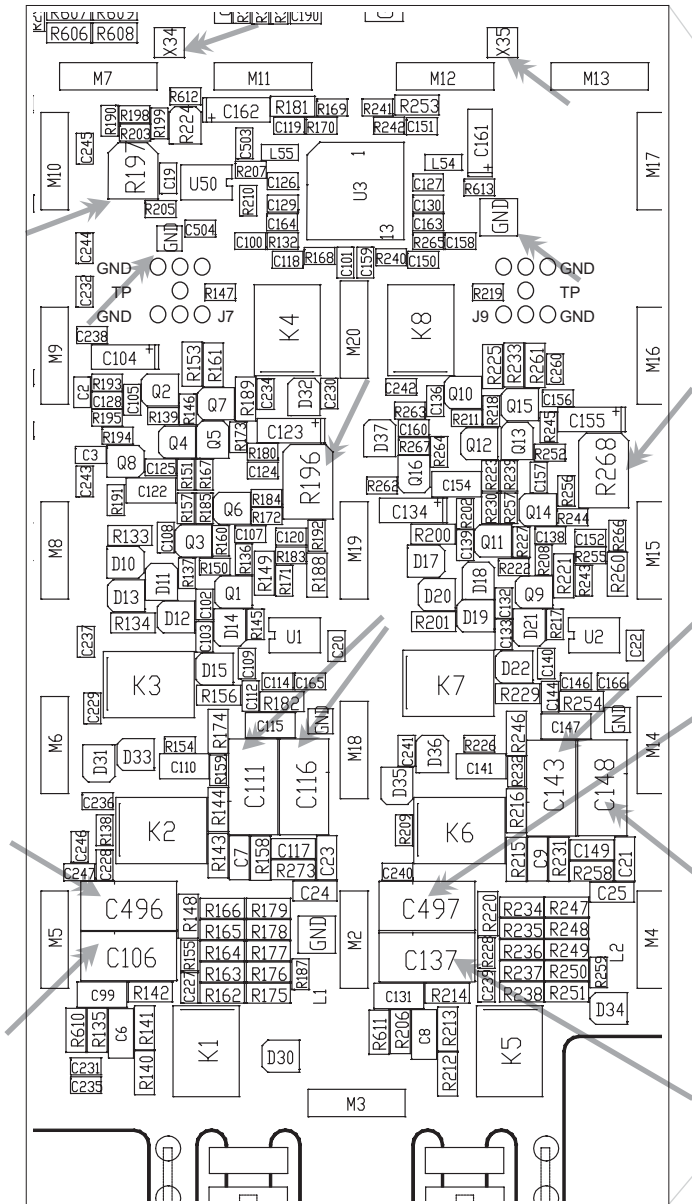
Figure 7-2 Test points and trimmers for the input amplifiers.
