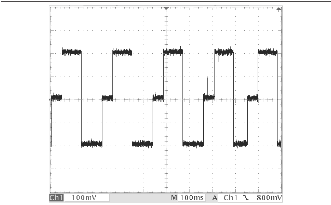
Figure 6-13 Oscilloscope showing the signal at XT, Period Single B.
