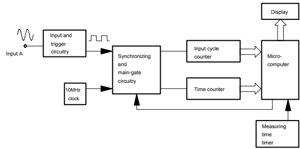
Figure 3. Block diagram for a reciprocal frequency counter
