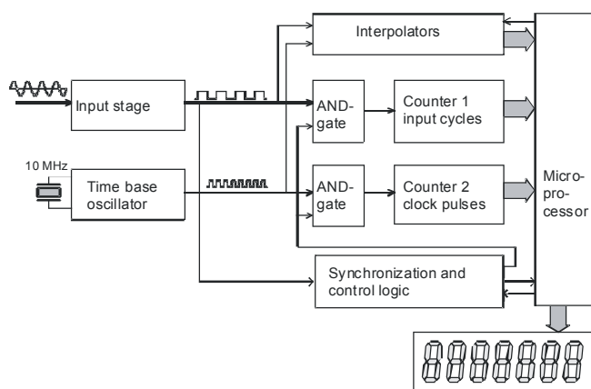
Figure 5. Block diagram for an interpolating reciprocal frequency counter
