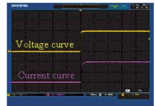
Under C.C Priority Mode, Inrush and Surge Voltage are Effectively Restrained
