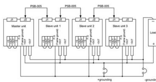
Parallel Connection
