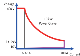
PEL-5010C-600-700
