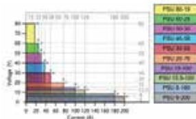
PSU-Series Operating Area (6-80V models)
