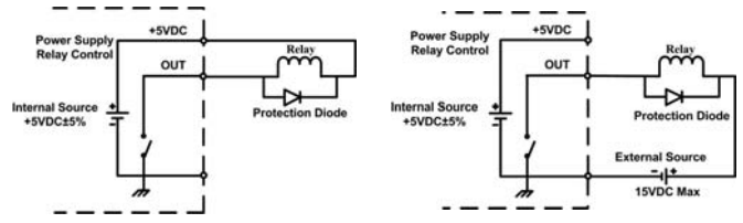
+5VDC Relay Output
