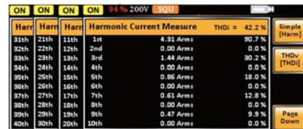
Current Harmonic
