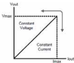
CV/CC Operation Mode
