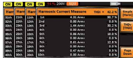
Current Harmonic
