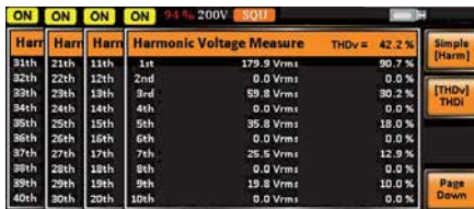
Voltage Harmonic
