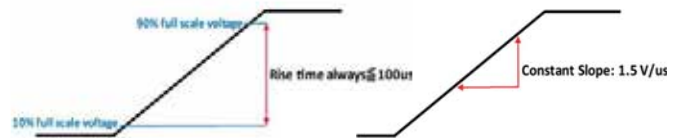
Time Mode
