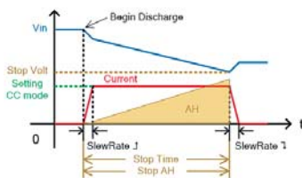
CC Mode
