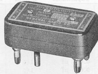
TYPE 493 Thermocouples are mounted in a bakelite case with plugs to fit a TYPE 274-RJ Mounting Base
