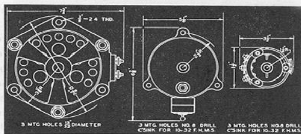
100-K, -L 200-CM, -CU 200-B VARIAC TYPES
