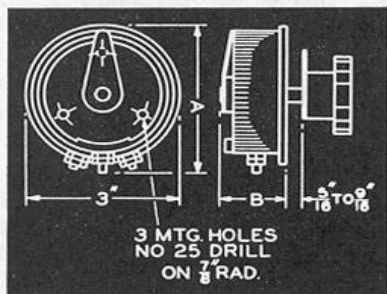
Standard 3-hole mounting method for rheostat-potentiometers
