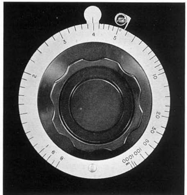
The MEGOHMS dial of TYPE 544-B Megohm Bridge. The scale is approximately logarithmic over the main decade from 1 to 10.
