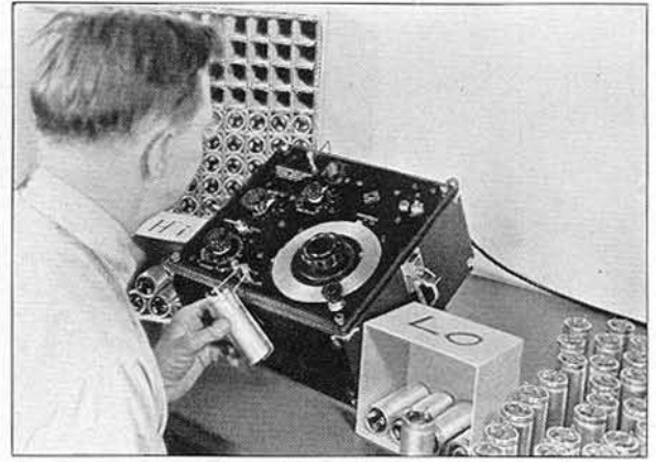
Production testing of electrolytic condensers with the capacitance test bridge.
