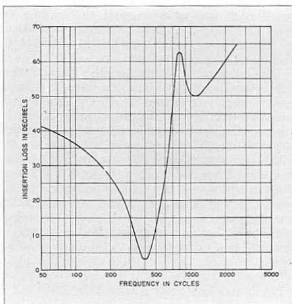
Transmission characteristic of TYPE 530 Band-Pass Filter.
