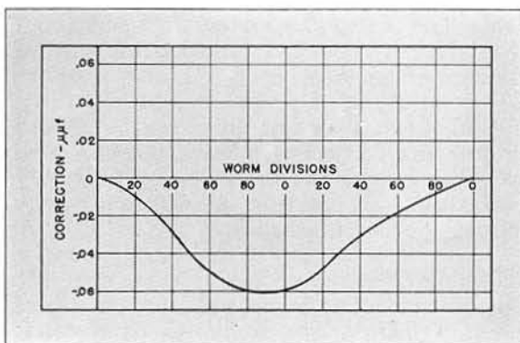
Plot of a typical worm correction for a TYPE 722-F Precision Condenser.
