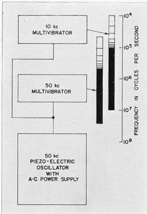
FIGURE 4. Functional diagram of CLASS C-10-H Secondary Frequency Standard.
