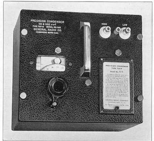
Panel view of the TYPE 722-D Precision Condenser.
