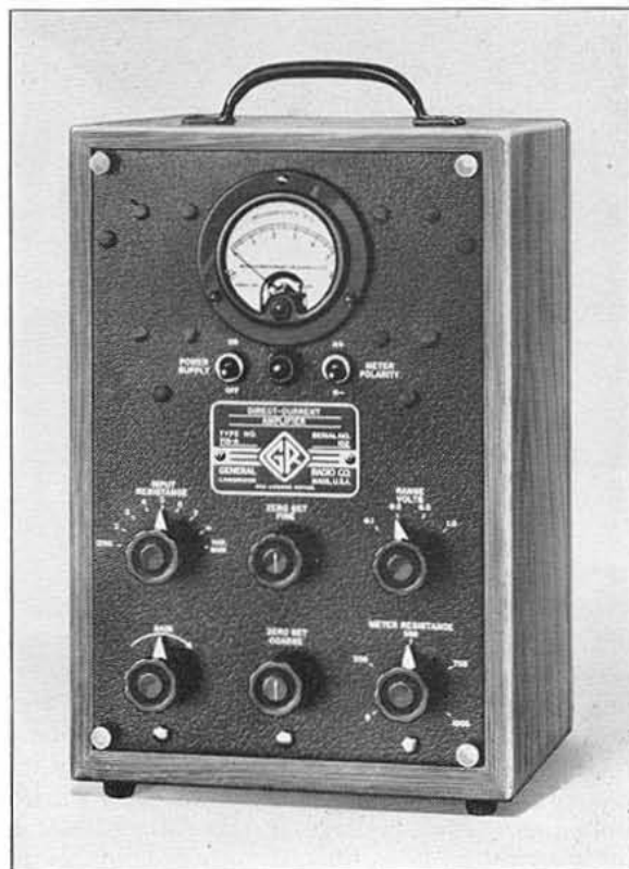
The TYPE 715-AM Direct-Current Amplifier.
