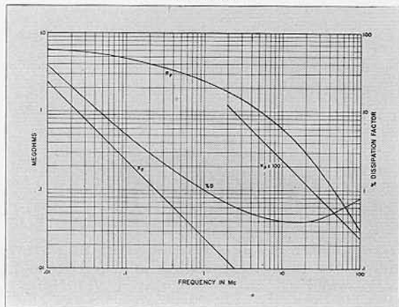
Plots of the resistive and reactive components of the input impedance, and of the dissipation factor of the input circuit, of TYPE 726-A Vacuum-Tube Voltmeter.
