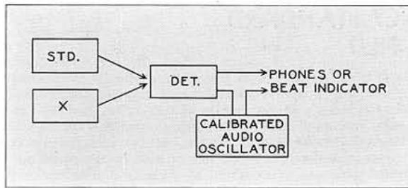
FIGURE 6. Functional diagram showing the operation of the direct-beating method of frequency measurement.
