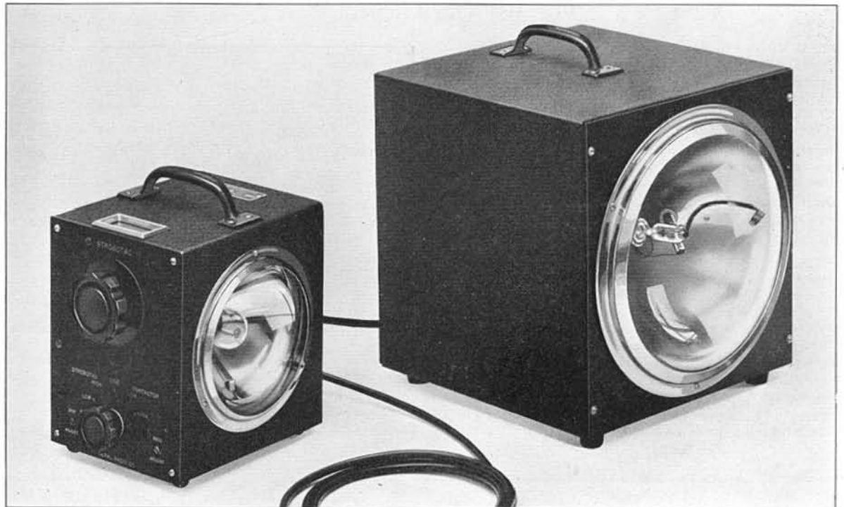
TYPE 631-B Strobotac with TYPE 648-A Strobolux.
