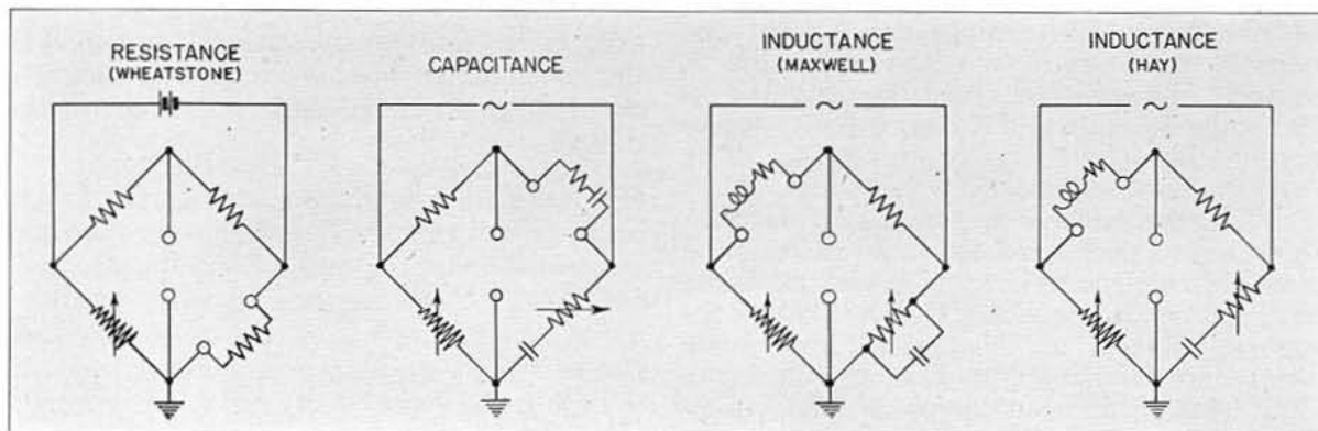
Schematic diagrams of the circuits used in TYPE 650-A Impedance Bridge.
