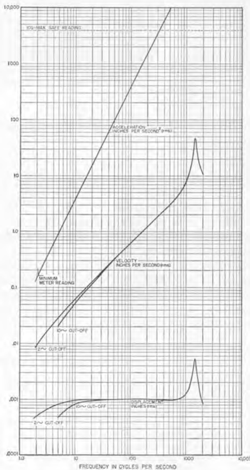
Readings of the Vibration Meter as a function of frequency for a constant displacement of 0.001 inch (rms).
