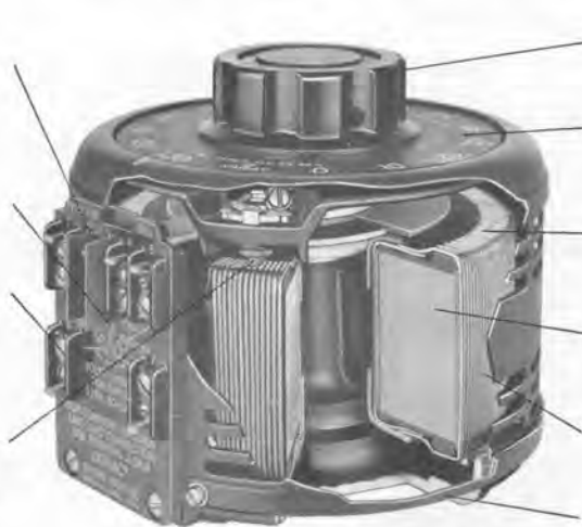
Cutaway view of V-model Variac
