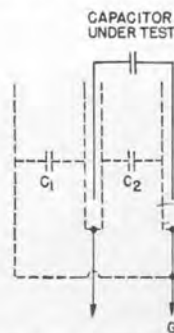
Sketch showing the nature and magnitude of the zero capacitance. This capacitance does not enter the measurement when a substitution method is used.
