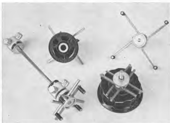
View of the coupling attachments furnished with the Sweep Drive. At left is the coupling shaft, to which has been attached the universal clutch. The other views show the clutch and the clutch attached to a knob.
