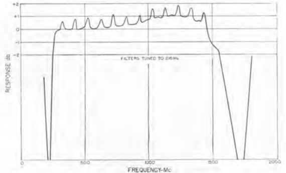
Response curve of a pair of TYPE 874-FR3 Rejection Filters with the TYPE 874-Mixer Rectifier.
