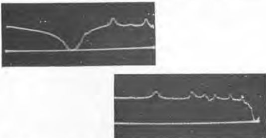
Oscillograms of the frequency characteristic of a TYPE 874-FR Rejection Filter tuned to 76 Mc. Sweep range is 43 to 250 Mc (upper) and 250 to 900 Mc (lower). Oscillator is driven by the TYPE 1750-A Sweep Drive; input amplitude is held constant by the TYPE 1263-A Amplitude-Regulating Power Supply. Vertical scale is square-law.
