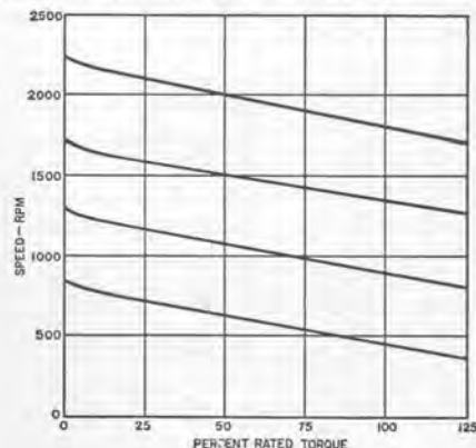
FIGURE 2. Speed-Torque Characteristics of a typical motor and speed control installation.
