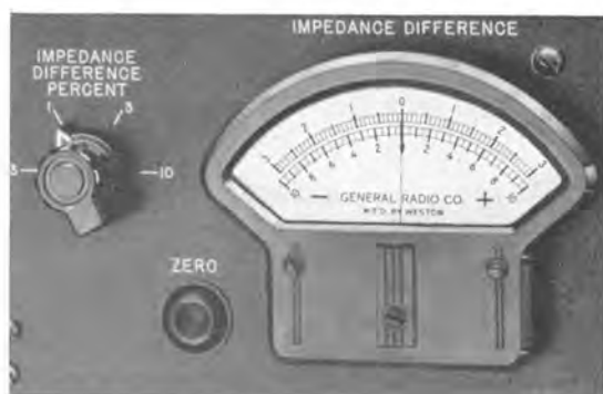
Close-up views of the meter scales and range switches.
