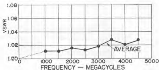
TYPE 874 Connector standing-wave ratio as a function of frequency.
