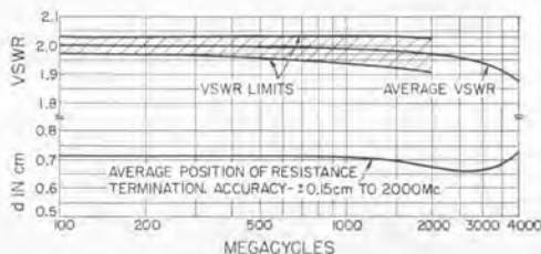
Plot of the VSWR and position of the pure resistance termination, for a Type 874-W100 100-Ohm Coaxial Standard. The distance, d , (see cross section above) is the distance from the position of the short or open circuit produced by a TYPE WN3 or WO3 Termination Unit to the position of the pure resistance termination. The cross-lined area indicates the tolerances on the characteristics.
