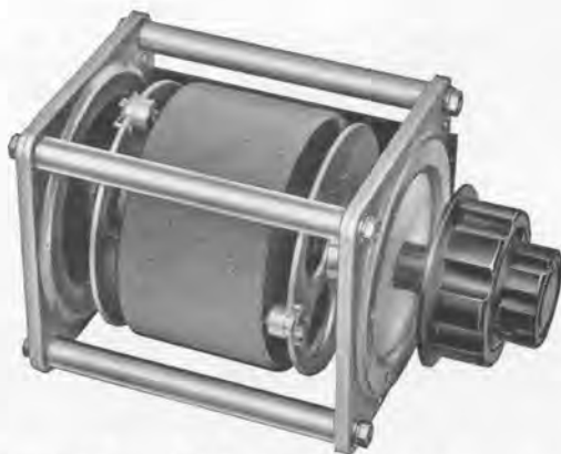
A special TYPE W5 Variac with two brushes, one at each face of winding.
