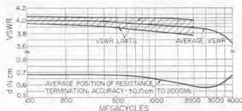
Plot of the characteristics of a Type 874-W200 200-Ohm Coaxial Standard.
