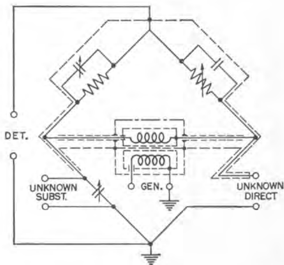
FIGURE 9. Showing how series inductance in the generator and detector leads can cause errors in measurement at radio frequencies.
