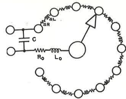
Equivalent circuit of a resistance decade, showing location and nature of residual impedances.
