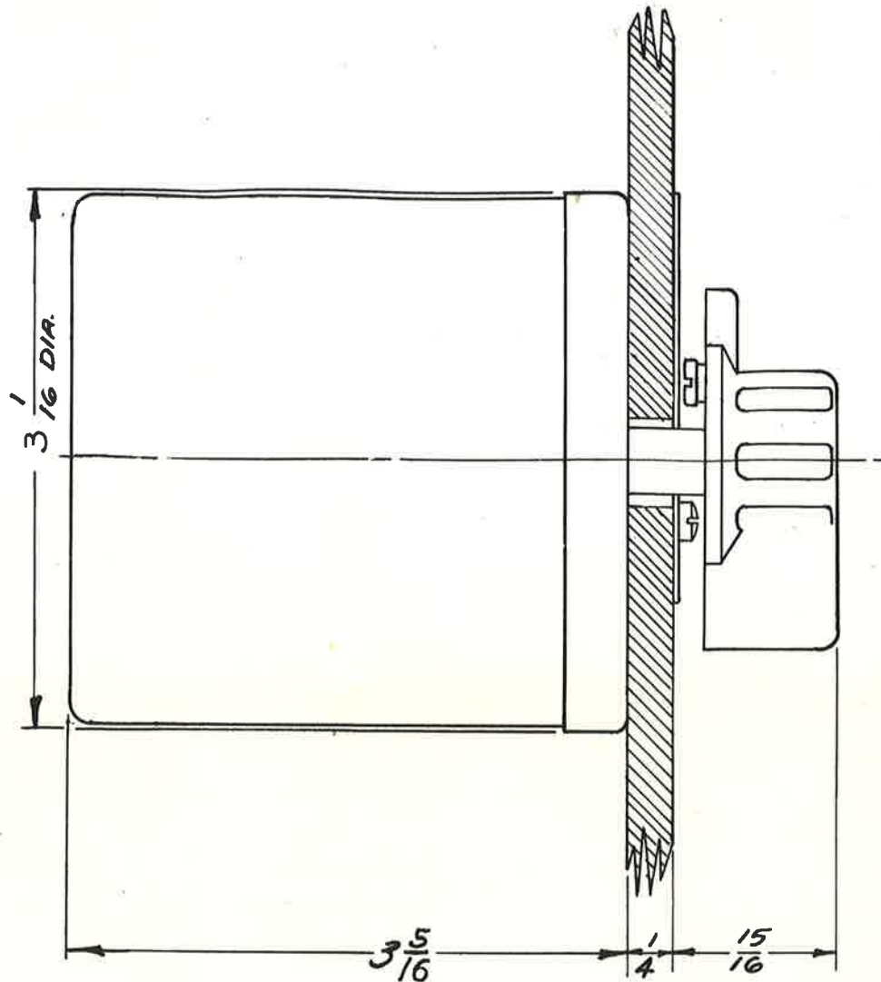
OVER-ALL DIMENSIONS
