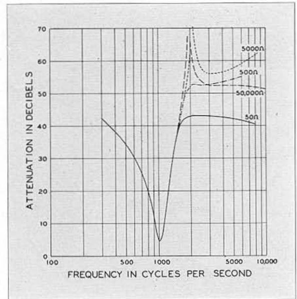
Attenuation characteristics of TYPE 830-R Band-Pass Filter for the various terminating impedances.
