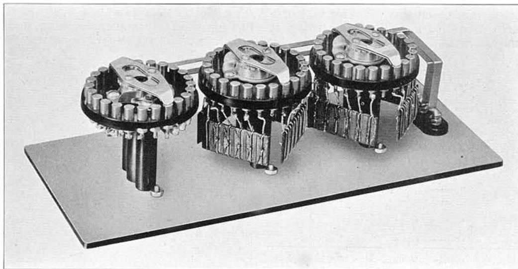
Interior of TYPE 670-F Compensated Decade Resistor.
