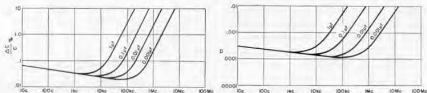
Figure 5. (Left) Fractional change in capacitance as a function of frequency. (Right) Dissipation factor as a function of frequency.
