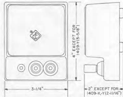
Figure 3. Dimensions of the Type 1409 Standard Capacitors.
