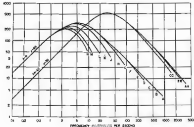
Figure 1. Q versus frequency for typical units.
