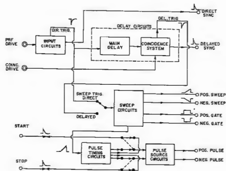
System block diagram showing major circuit groups and their interconnections.
