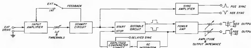
Block diagram of the circuit system.
