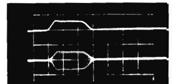
(Left) Amplitude-modulation characteristic at 900 Mc. Peak rf output is 10 millivolts; rf input, 50 millivolts. (Right) Oscilloscope showing modulation pulse and rf output pulse. Pulse duration is 0.25 \mu sec with 0.05- \mu sec rise time. Carrier frequency is 60 Mc. Scale is 0.1 \mu sec per horizontal division.
