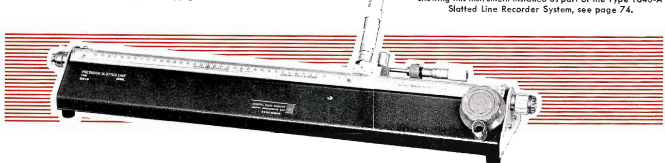
Type 900-LB Precision Slotted Line. For a photograph showing this instrument installed as part of the Type 1640-A Slotted Line Recorder System, see page 74.
