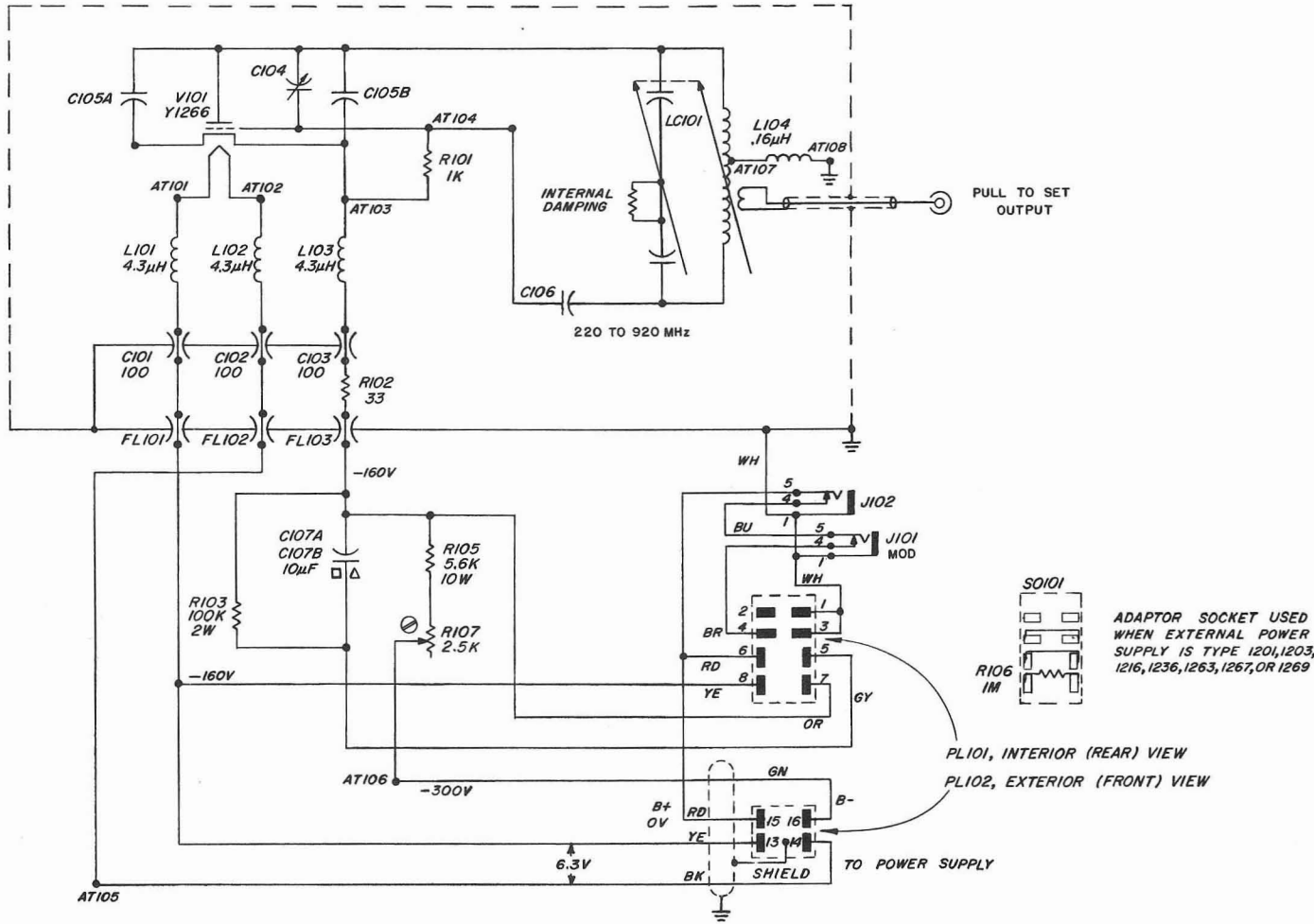
Figure 6-8. Schematic diagram of the Type 1362 UHF Oscillator.
