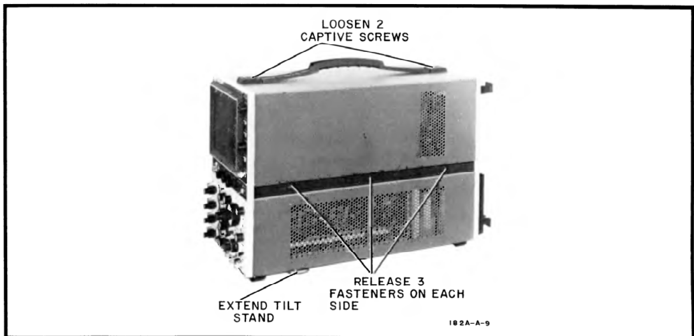
Figure 5-1. Cover Removal
