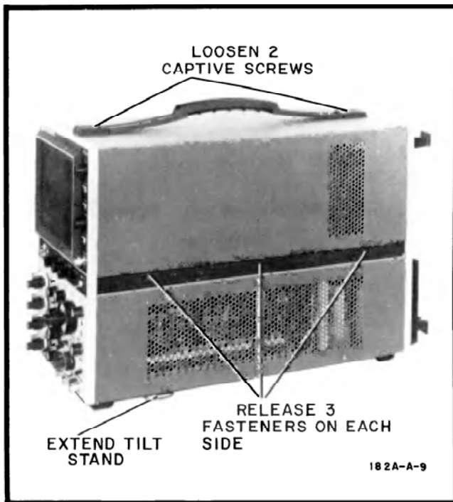
Figure 8-2. Cover Removal
