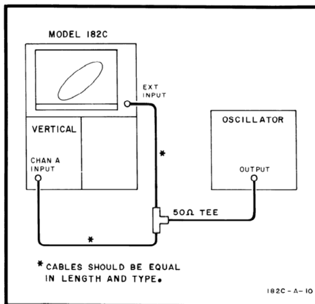
Figure 5-4. Phase Adjustment Test Setup
