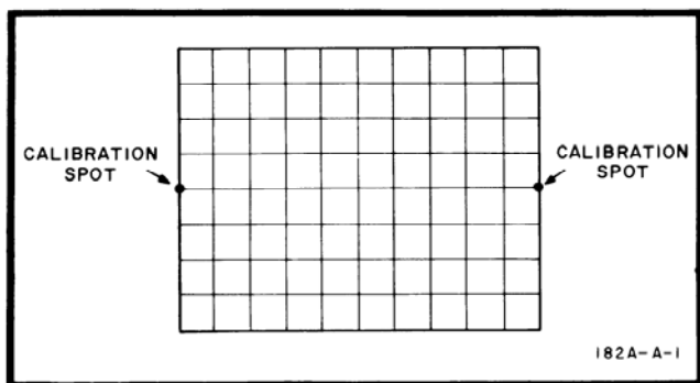
Figure 5-3. Calibration Display
