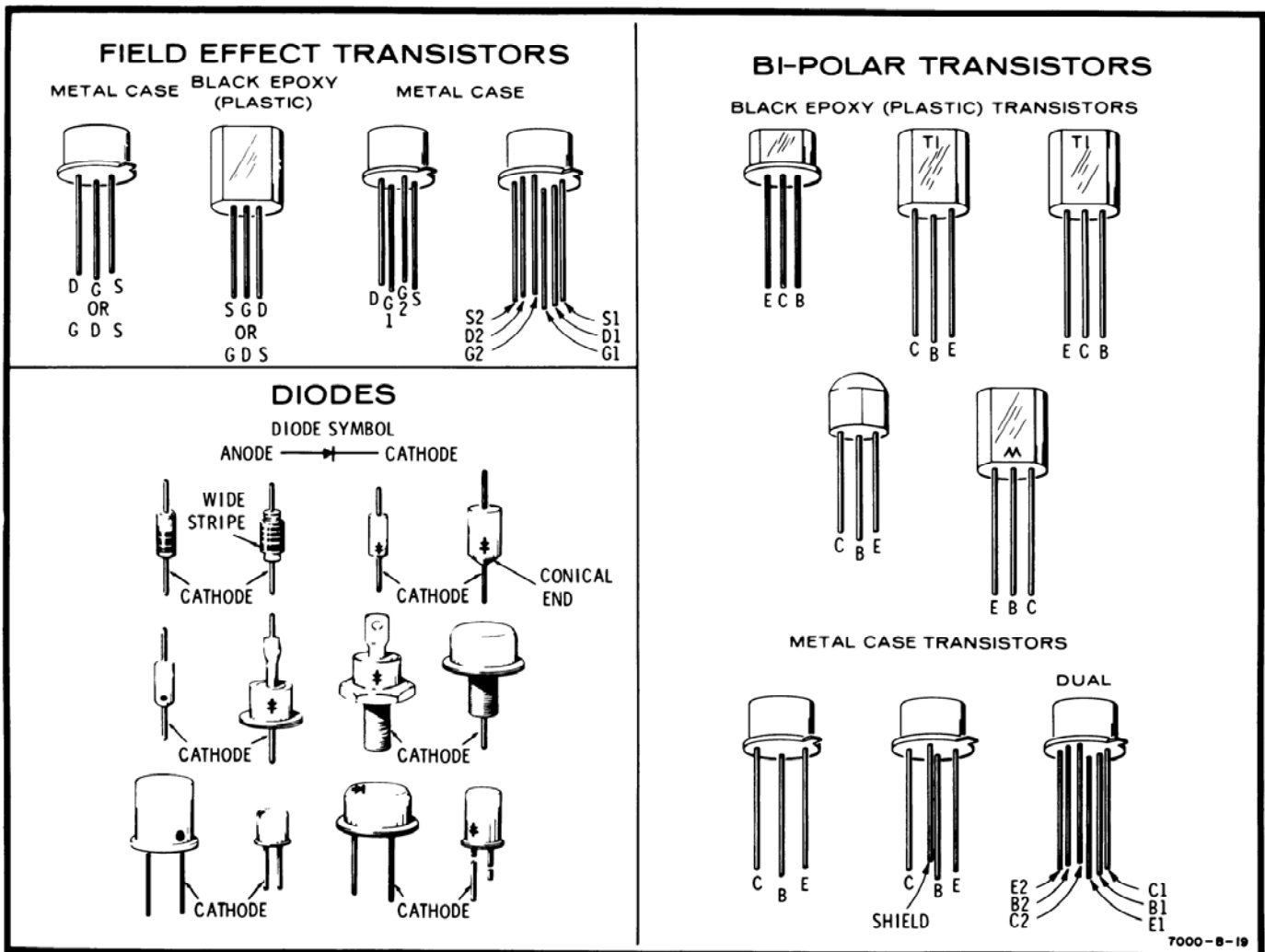
Figure 8-1. Semiconductor Identification
