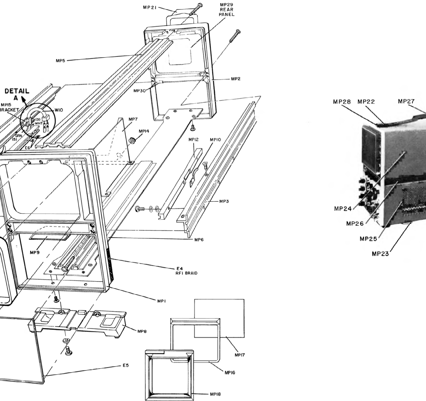
Figure 6-1. Model 182C Mechanical Parts
