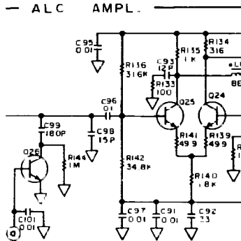
Figure 8-46. A2 Schematic Diagram.
