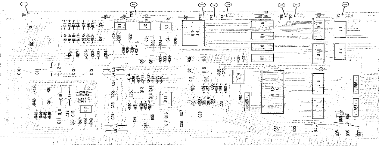
Figure 8-73. A23 DC Bias Supply Board Assembly Component Locations.
