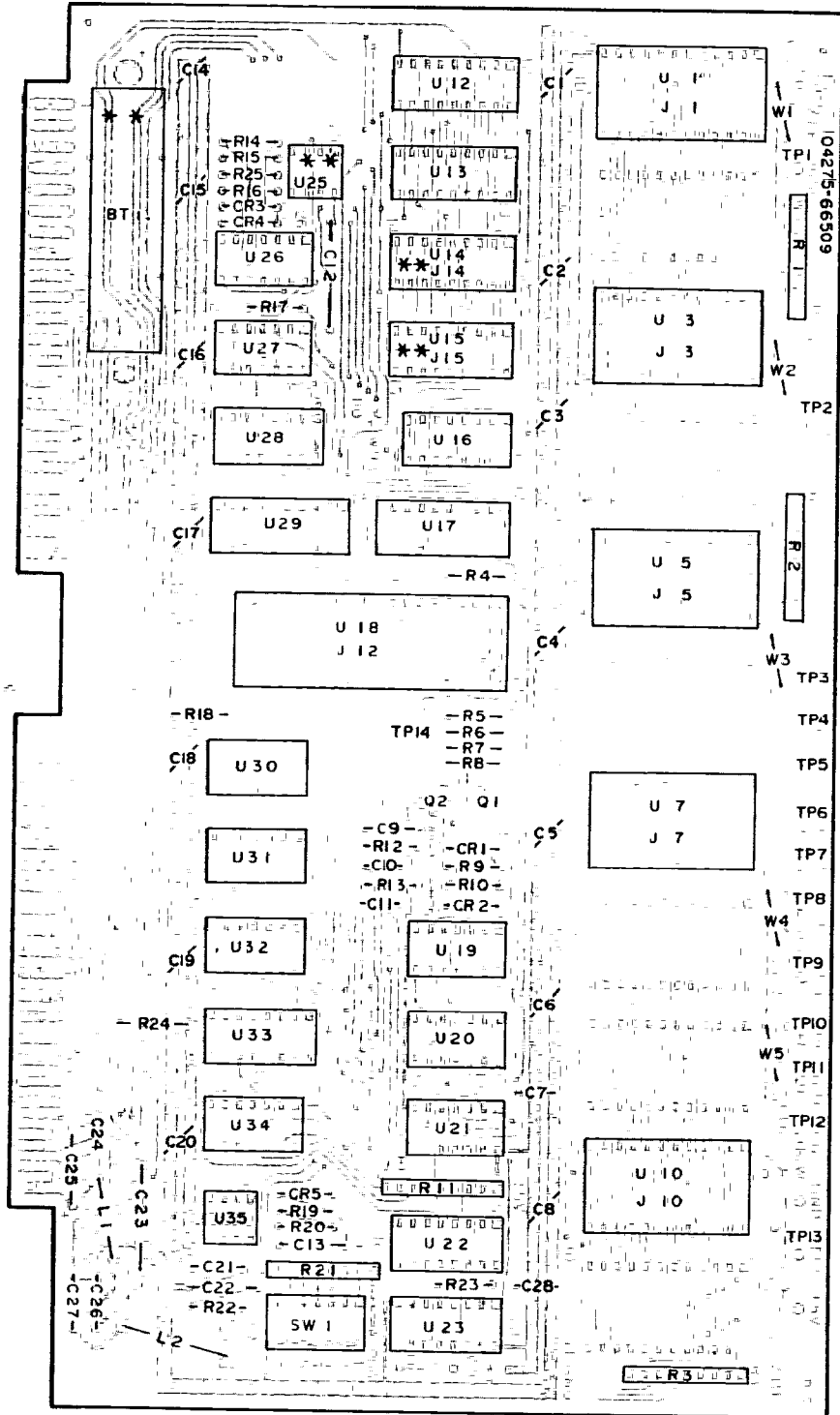
Figure 8-63. A9 MPU Component Locations.
