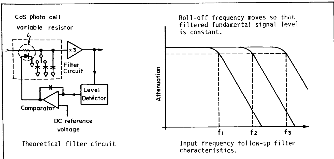
Figure 8-9. Frequency Follow-up Filter Operating Theory.
