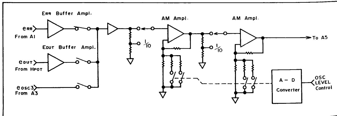
Figure 8-11. A4 Process Amplifier Block Diagram.
