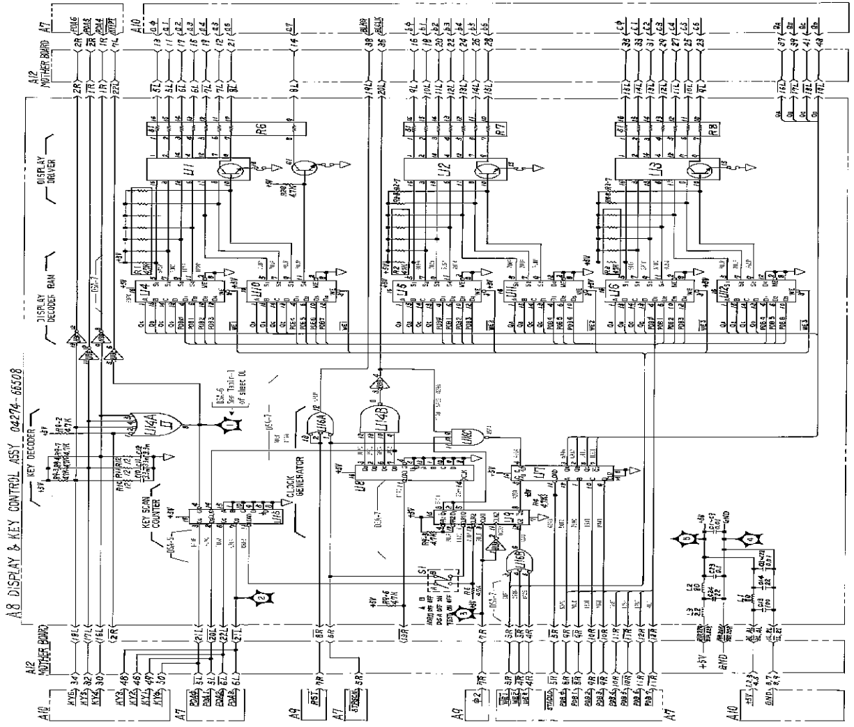
Figure 8-62. A8 Display Control Board Assembly Schematic Diagram.
