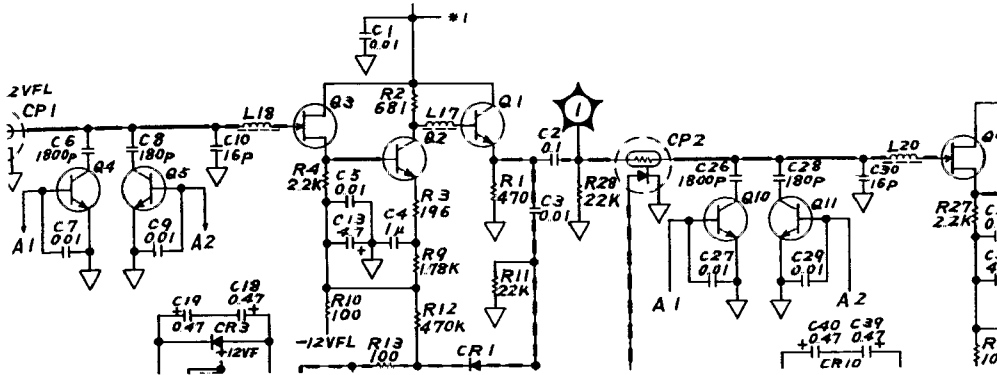
Figure 8-58 (B). A6 Schematic Diagram.
