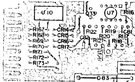
Figure 8-45. A2 Component Locations.
