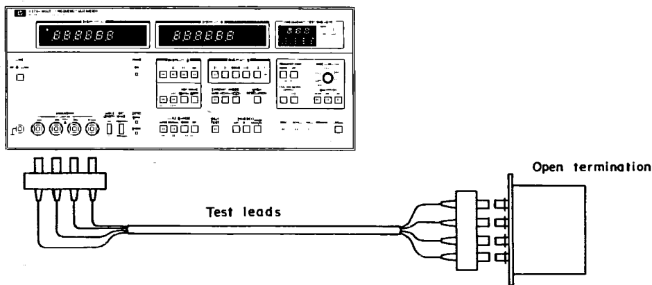
Figure 5-11. 10MHz CMR Amplifier and Range Resistor phase Adjustment Setup.
