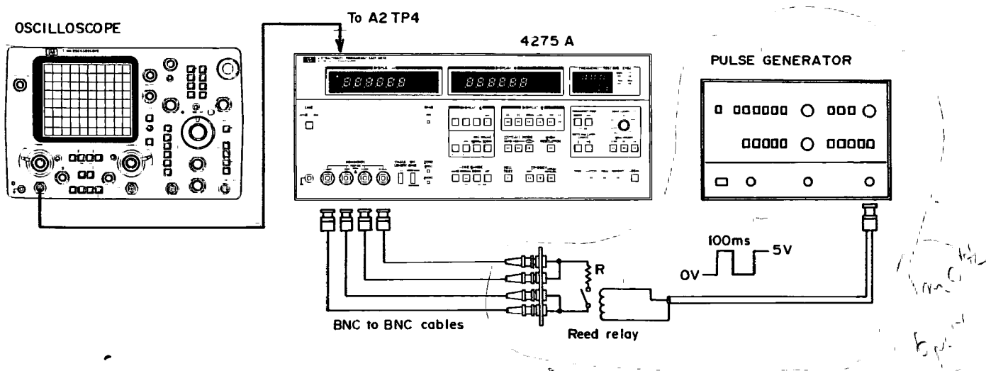
Figure 5-6. Balance Control Phase Tracking Adjustment Setup.
