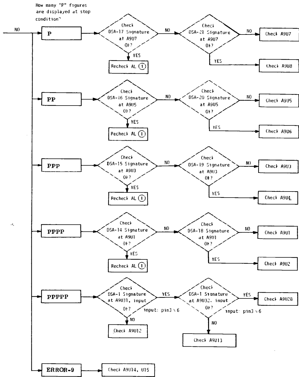
Page 8-51, Figure 8-33. Digital Section Troubleshooting Flow Diagram BL: Partially change the flow diagram as follows:
