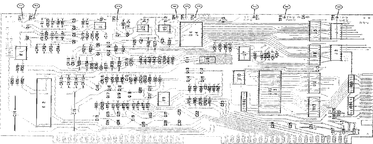
Figure 8-69. A21 DC Bias Supply Board Assembly Component Locations.
