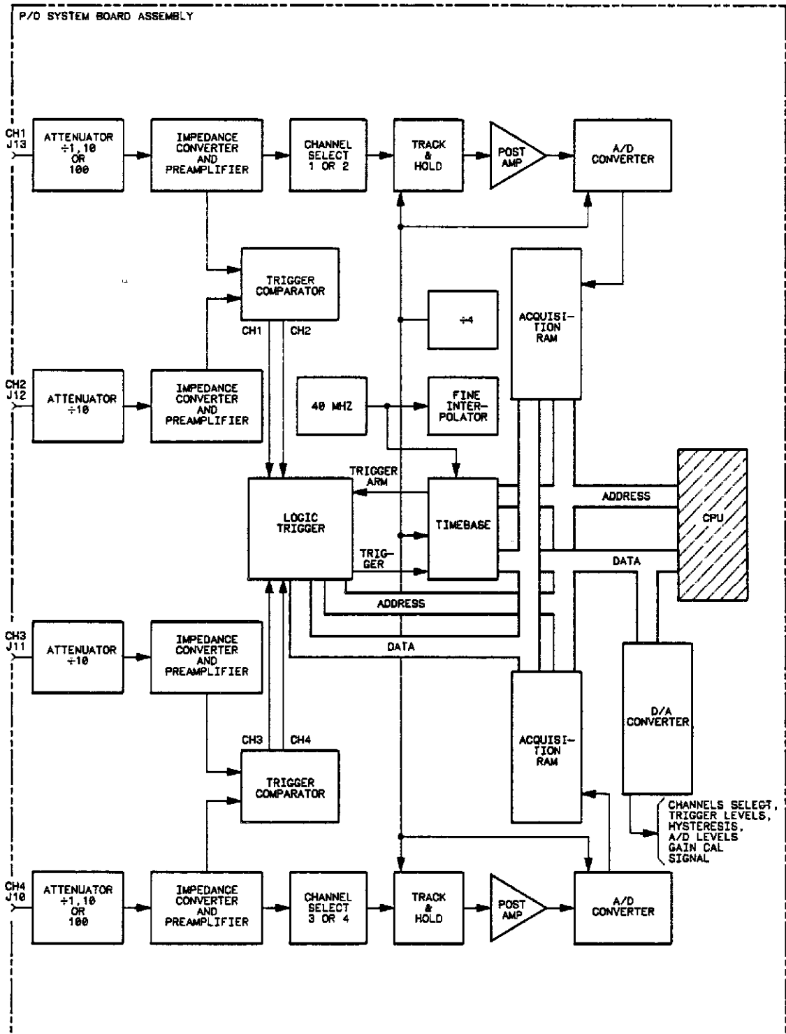
Figure 6-2. HP 54501A Acquisition Block Diagram
