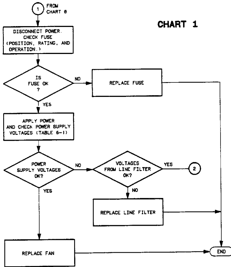
Figure 6-5. Trouble Isolation Chart for HP 54501A Fan/Fuse
