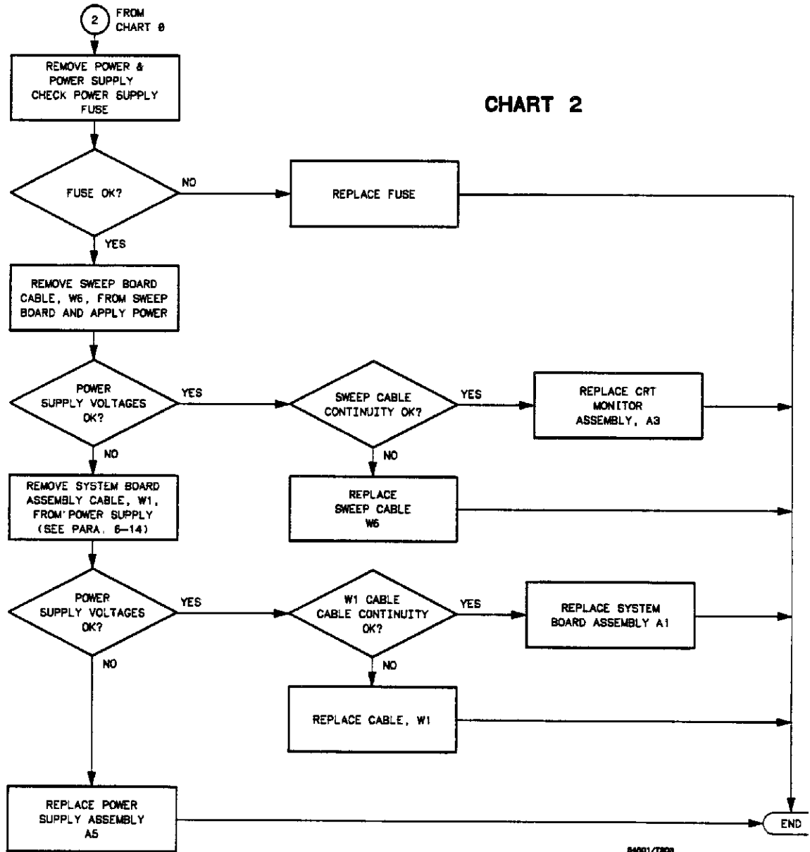
Figure 6-6. Trouble Isolation Flowchart for HP 54501A Power Supply
