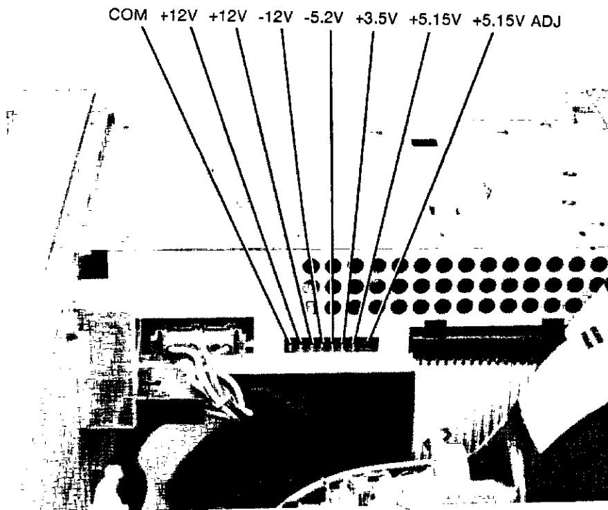
Figure 4-1. HP 54501A Power Supply Assembly Testpoints and Adjustment Location
