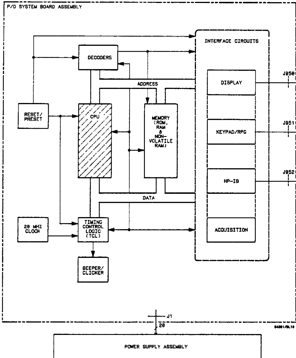
Figure 6-3. HP 54501A System Control Block Diagram
