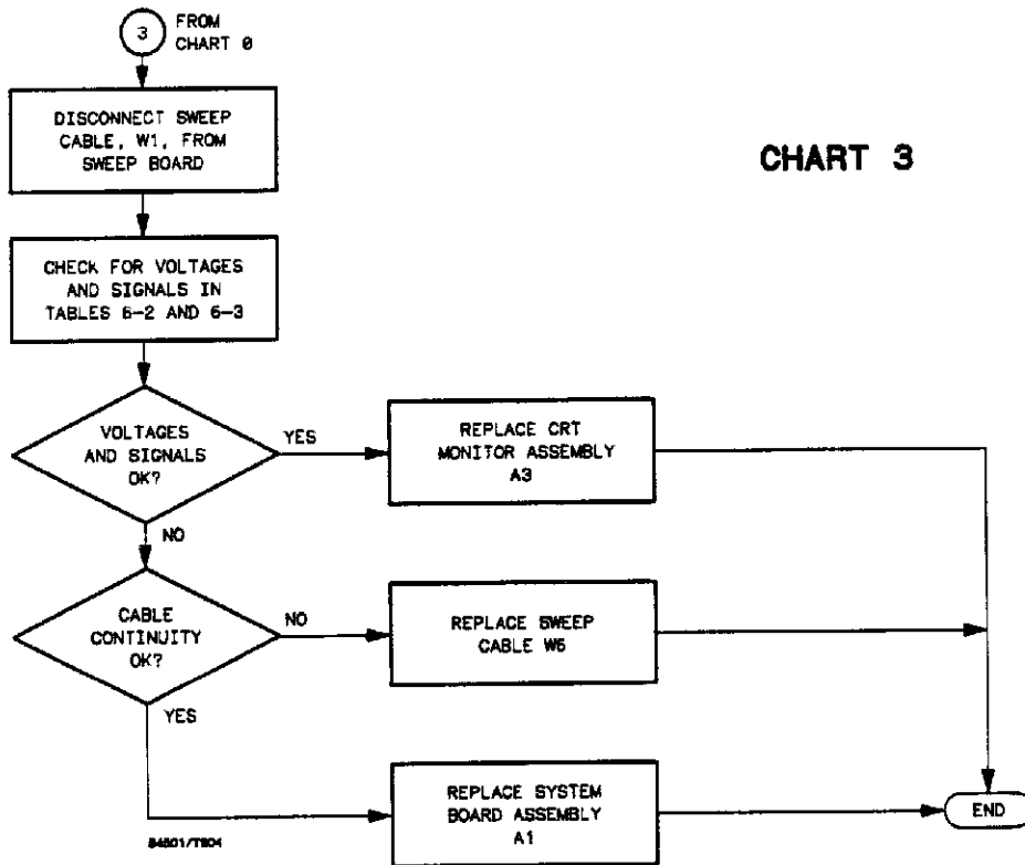
Figure 6-7. Trouble Isolation Flowchart for HP 54501A CRT Monitor
