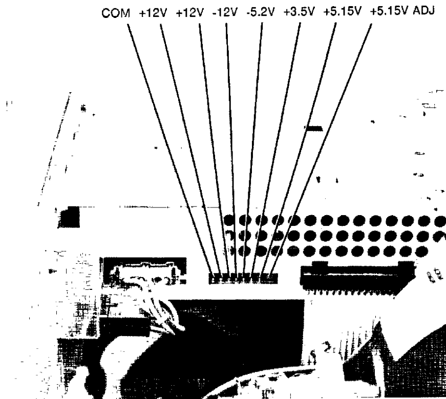
Figure 6-10. HP 54501A Power Supply Test Points
