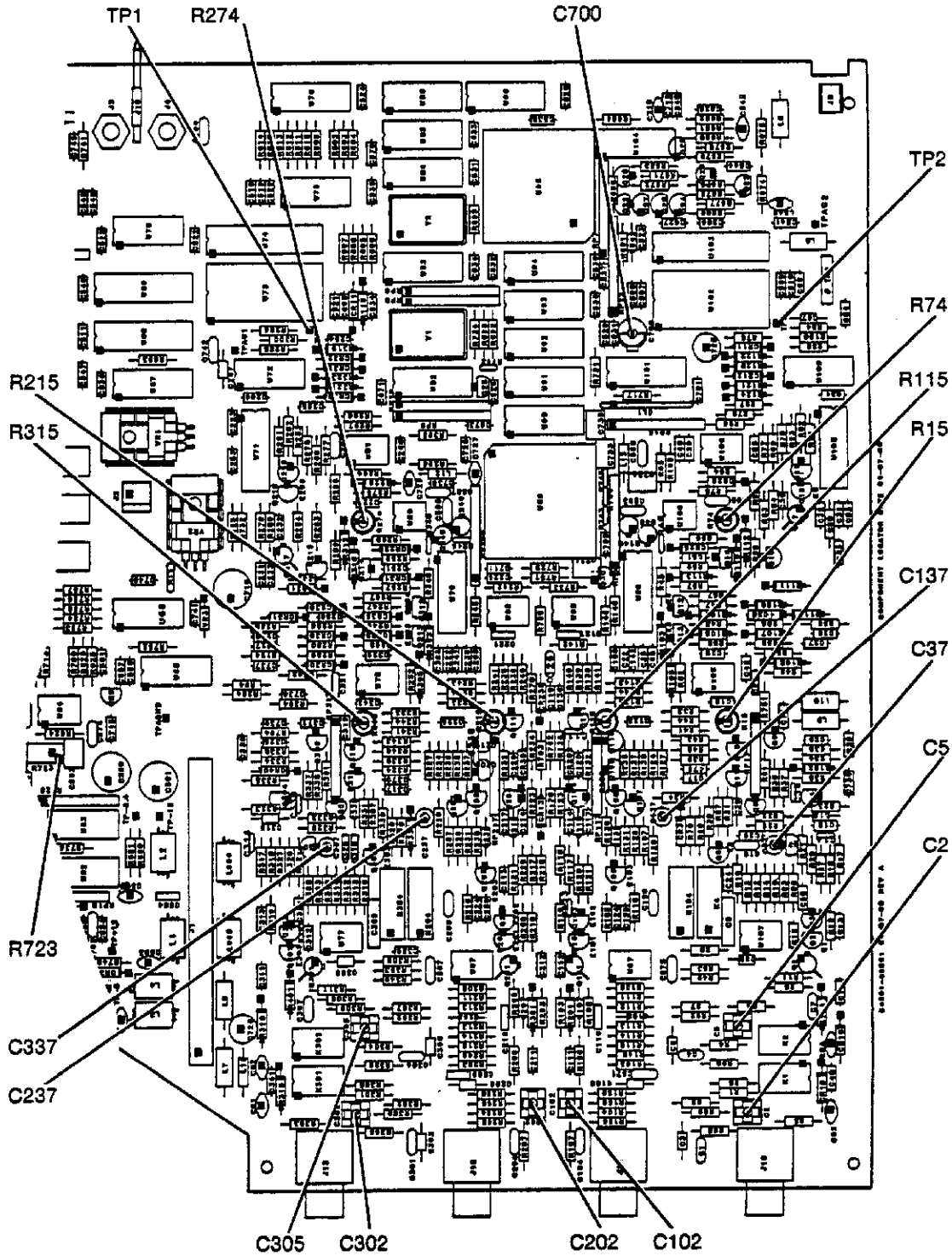
Figure 4-3. HP 54501A System Board Component Locator
