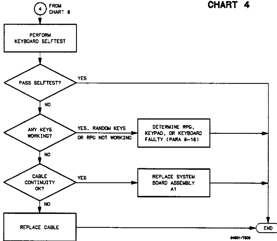
Figure 6-8. Trouble Isolation Flowchart for HP 54501A Keyboard
