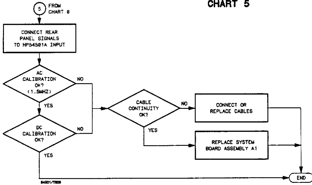
Figure 6-9. Trouble Isolation Flowchart for HP 54501A Calibration Signals
