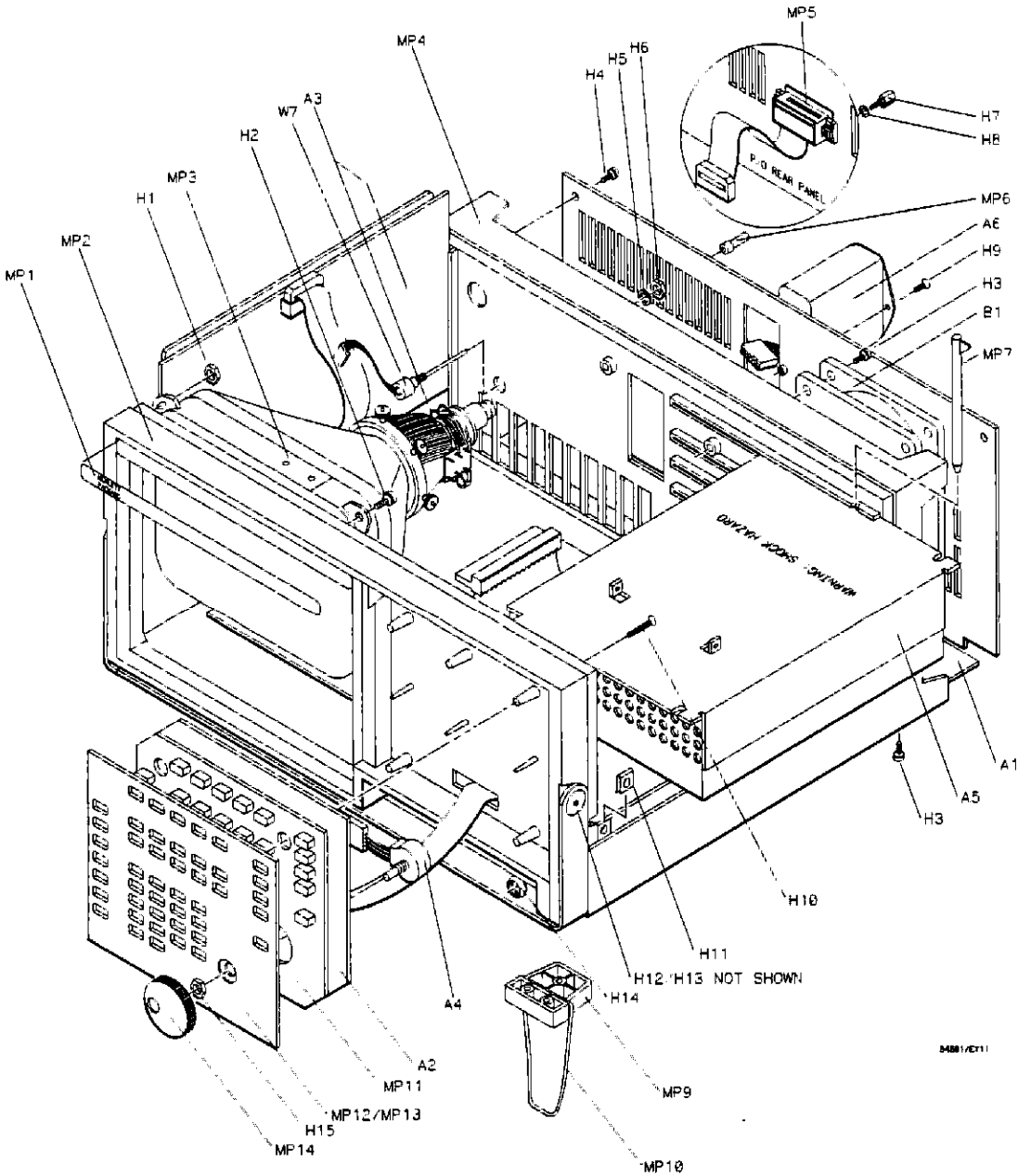
Figure 5-1. HP 54501A Exploded View
