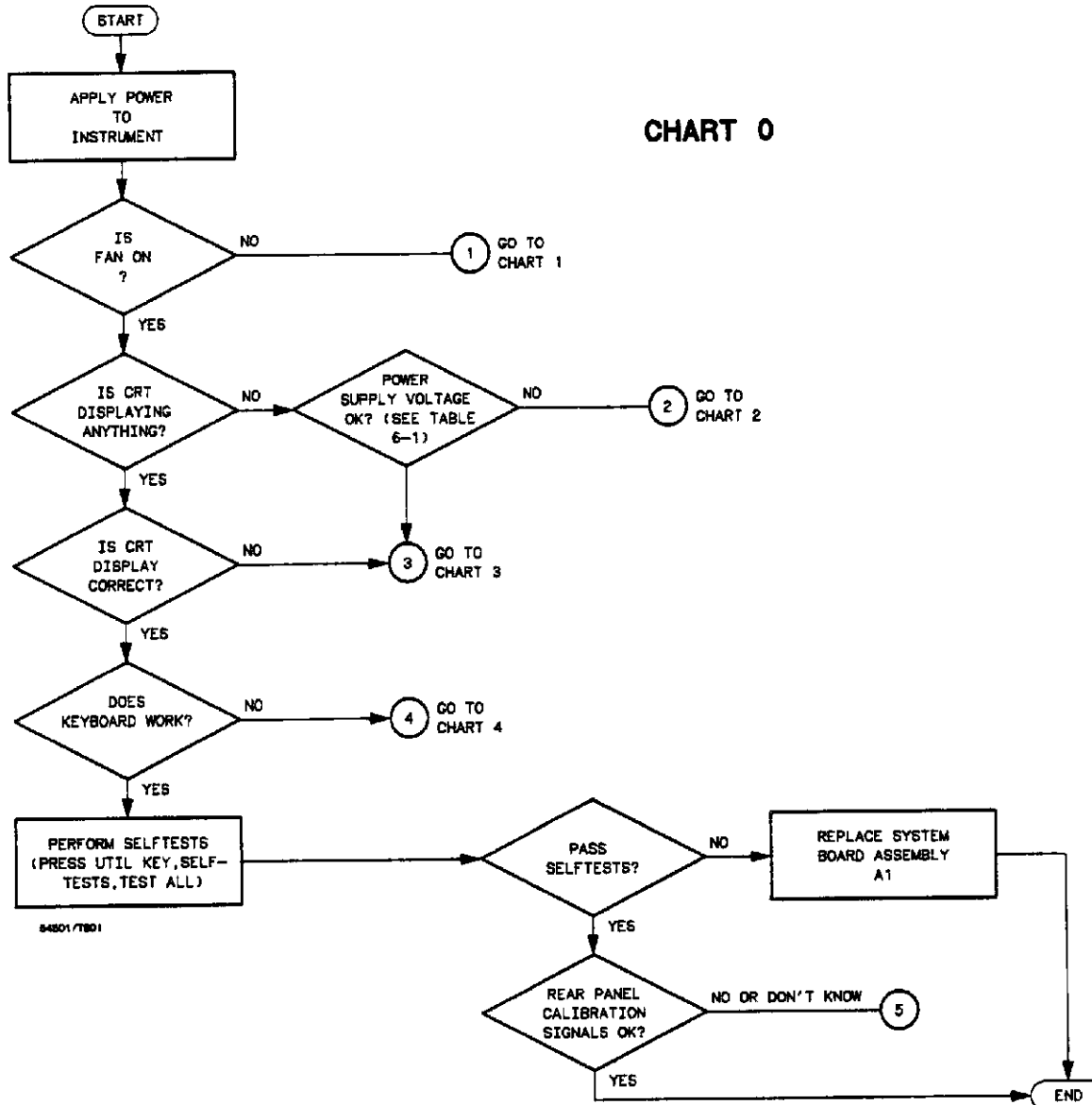
Figure 6-4. General Trouble Isolation Flowchart for HP 54501A
