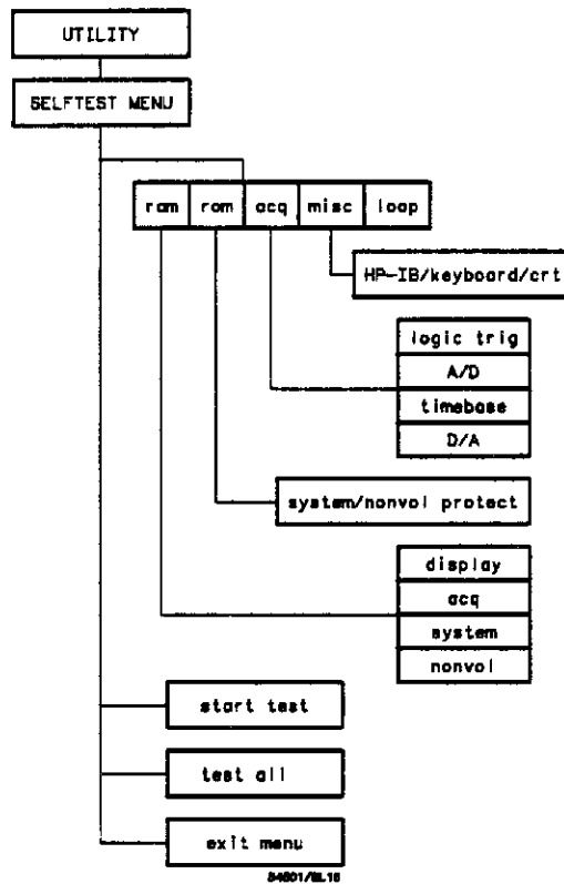
Figure 6-12. HP 54501A Selftest Menu Selections
