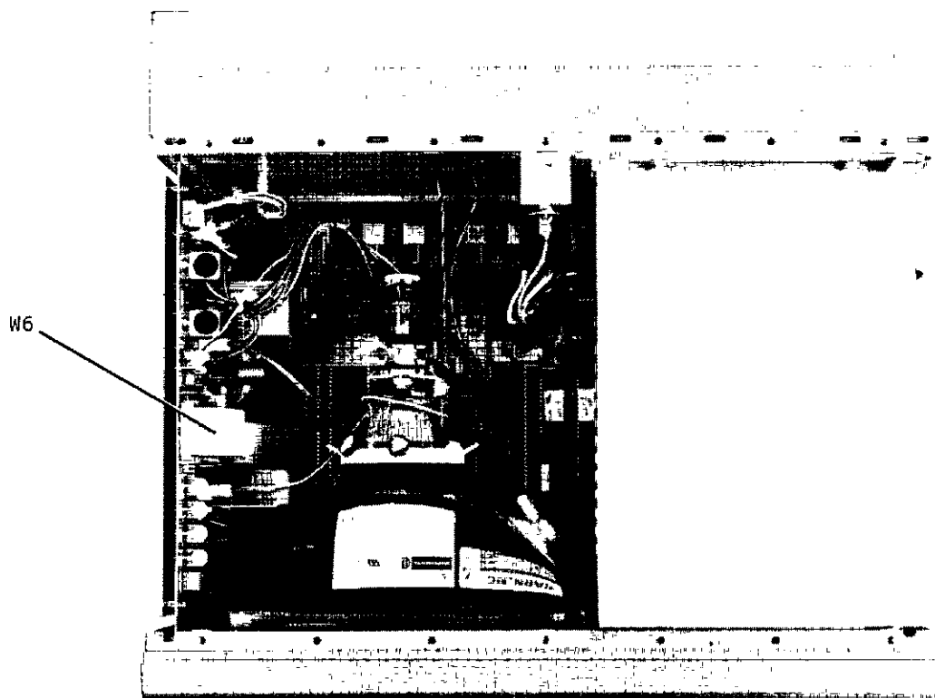
Figure 6-13. HP 54501A CRT Monitor Assembly Cable, W6, Location
