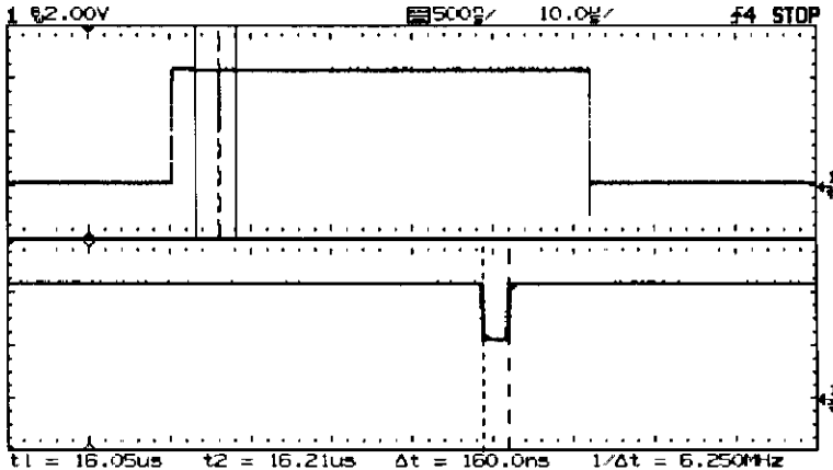
The cursors track delayed sweep. Expand the display with delayed sweep, then characterize the event of interest with the cursors.
