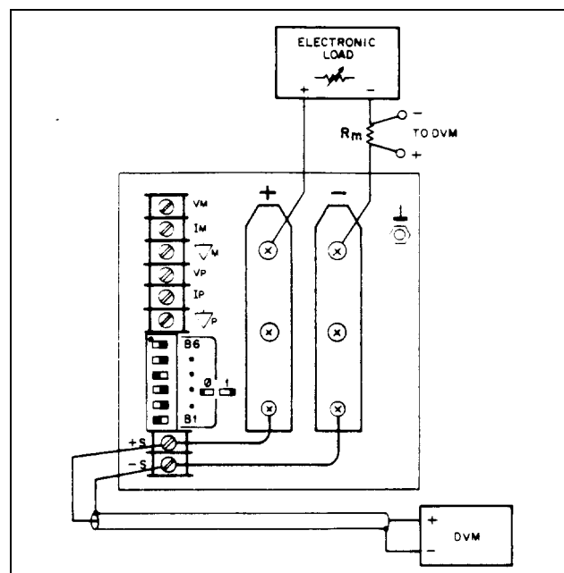
Figure 2-3. Basic Test Setup
