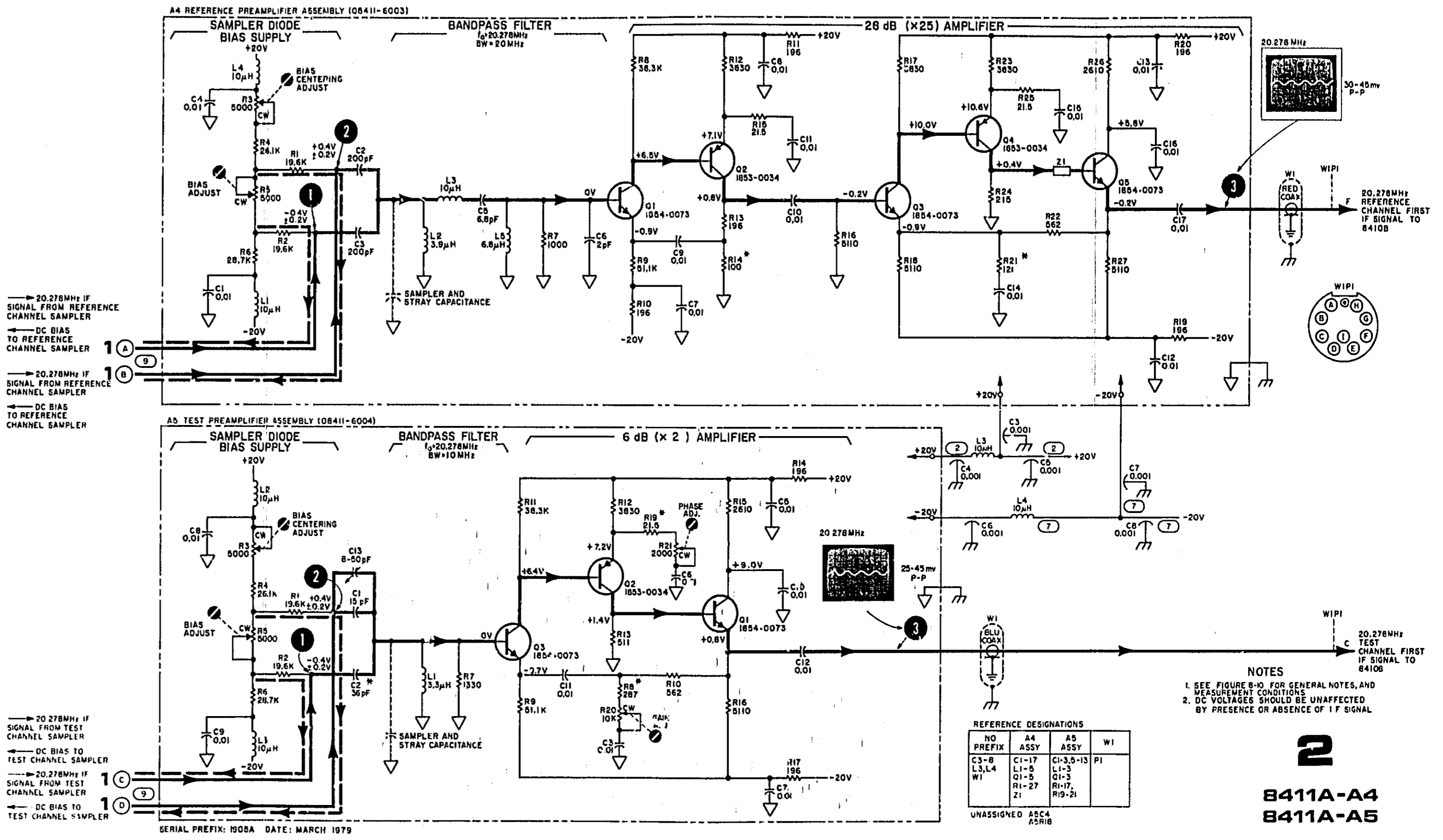
Figure 8-30. 8411A-A4 and A5 Schematic Diagram
