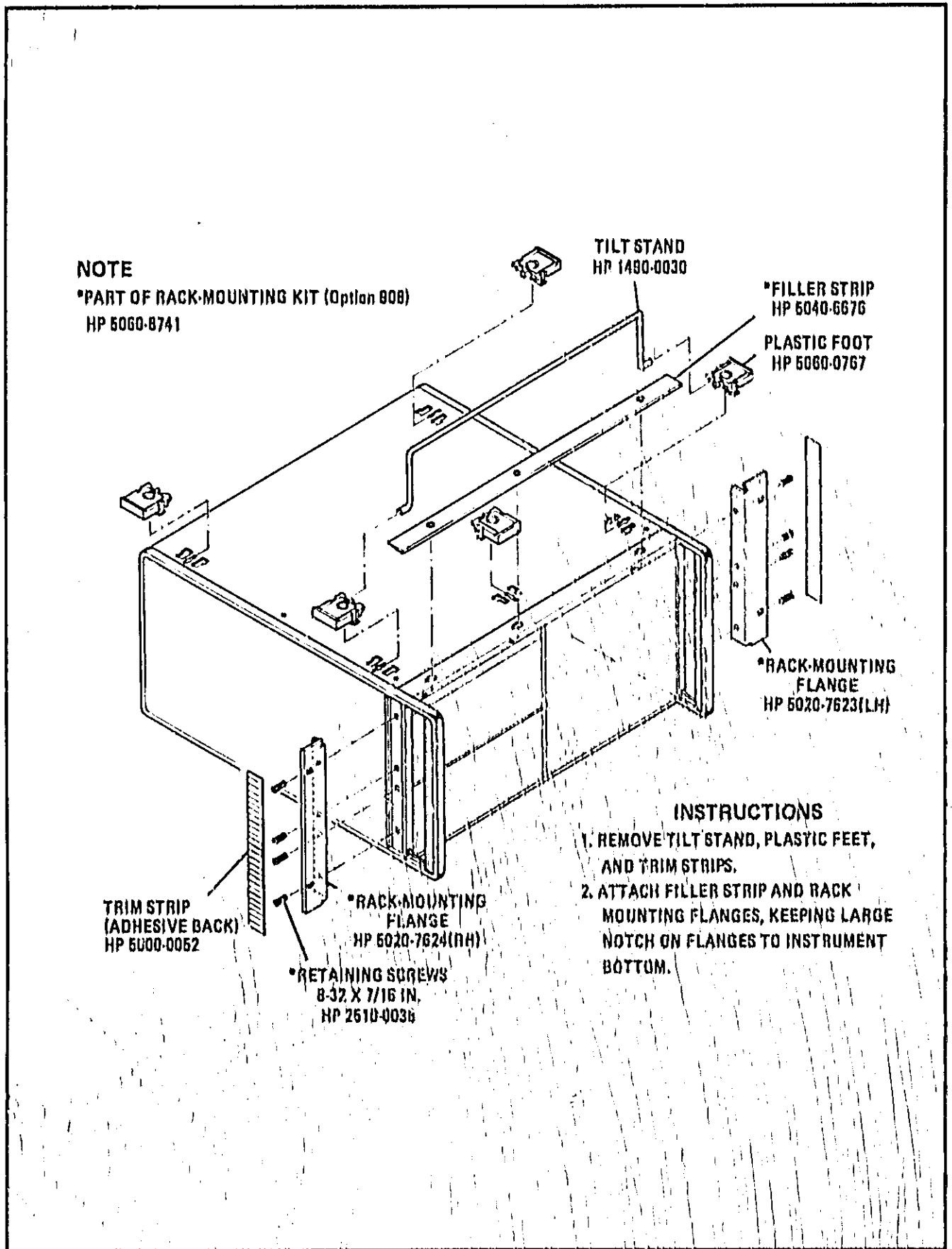
Figure 2-2. Rack-Mounting Kit Installation
