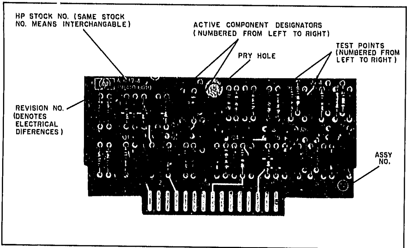
Figure 8-1. Servicing Aids on Circuit Boards
