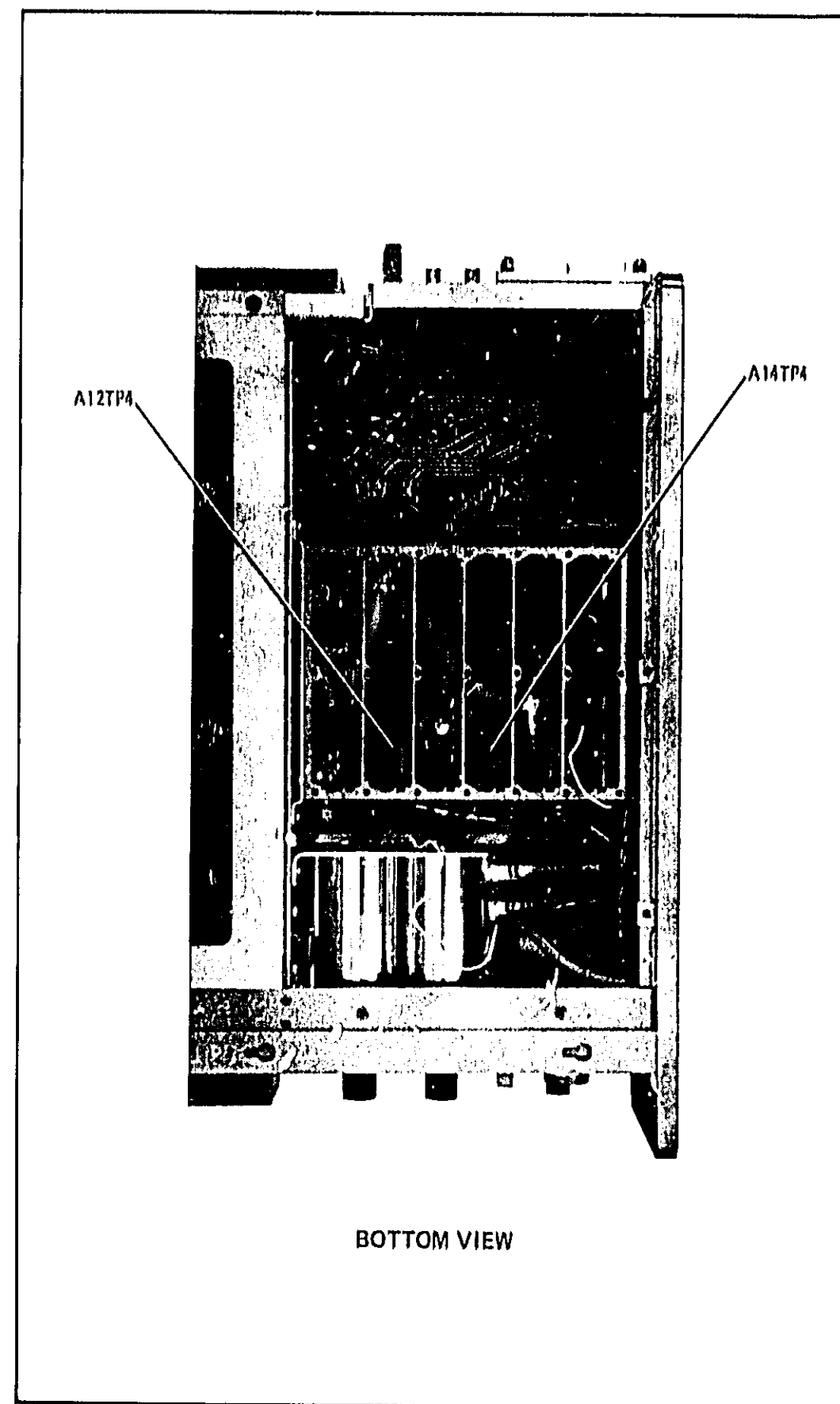
Figure 8-22. Test Points for 8411A Troubleshooting (2 of 2) (Shows 8410B TP's)
