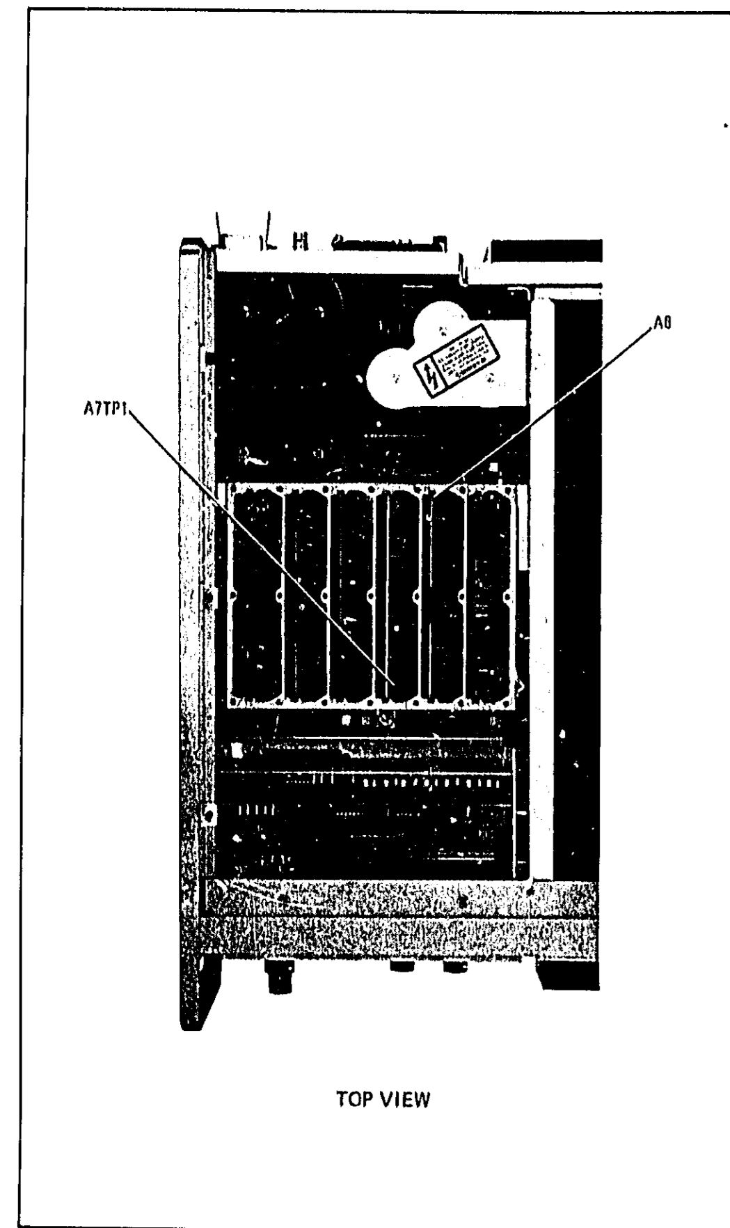
Figure 8-18. Models 8410B/8411A Interface Test Points ( 1 of 2 )
