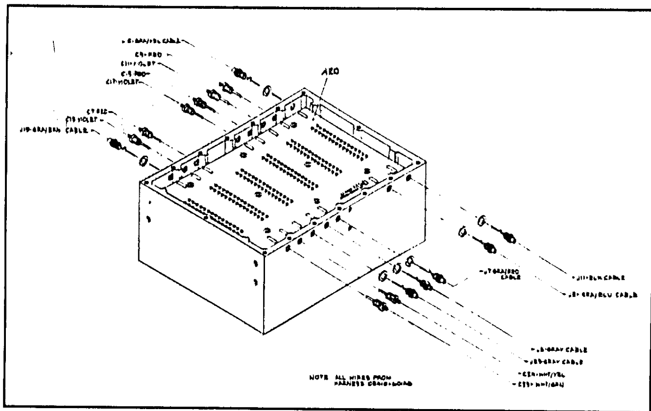
Figure 8-71. Wiring Connections to Fixed Housing (CHANGE 6)
