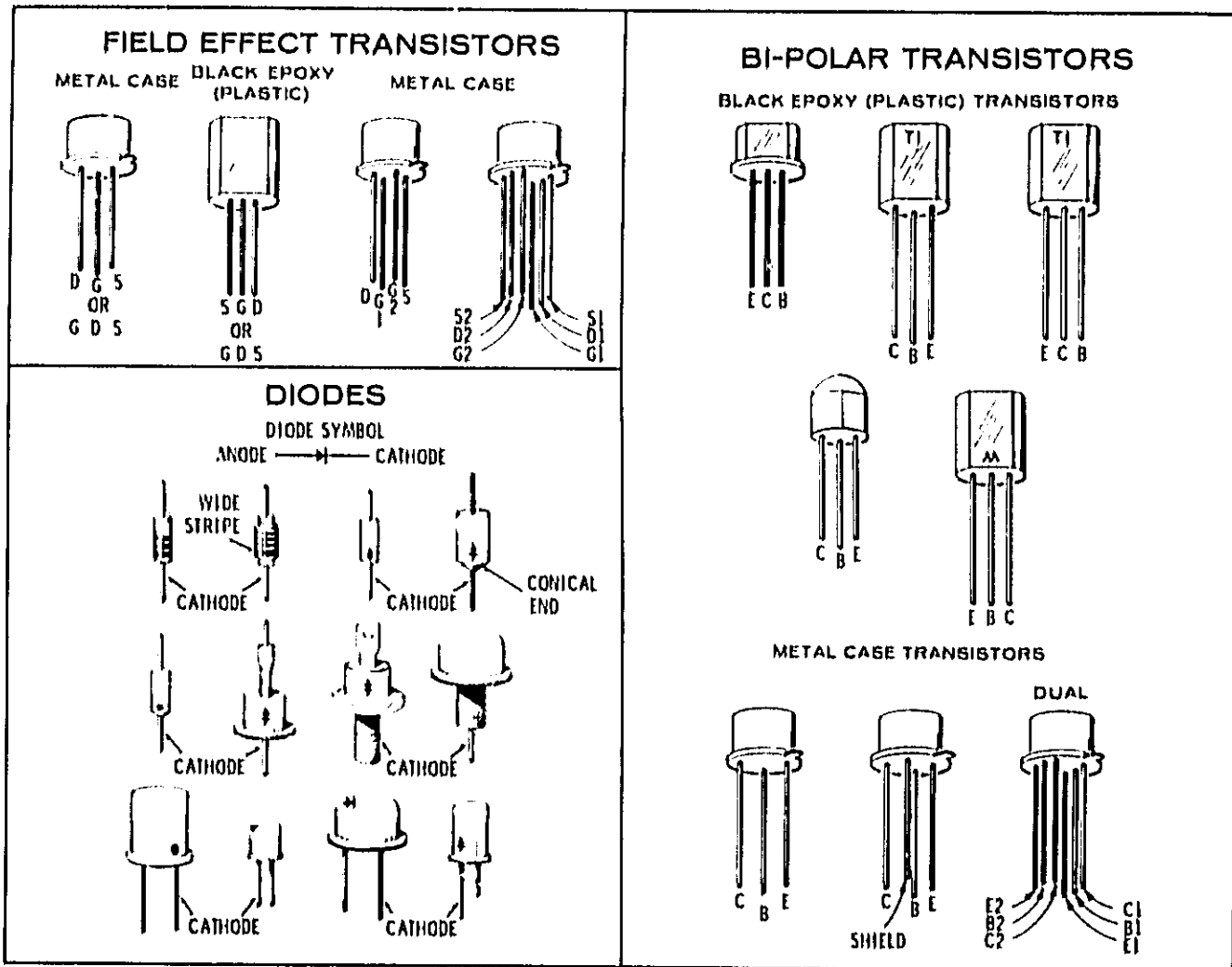
Figure 8-4. Examples of Diode and Transistor Marking Methods
