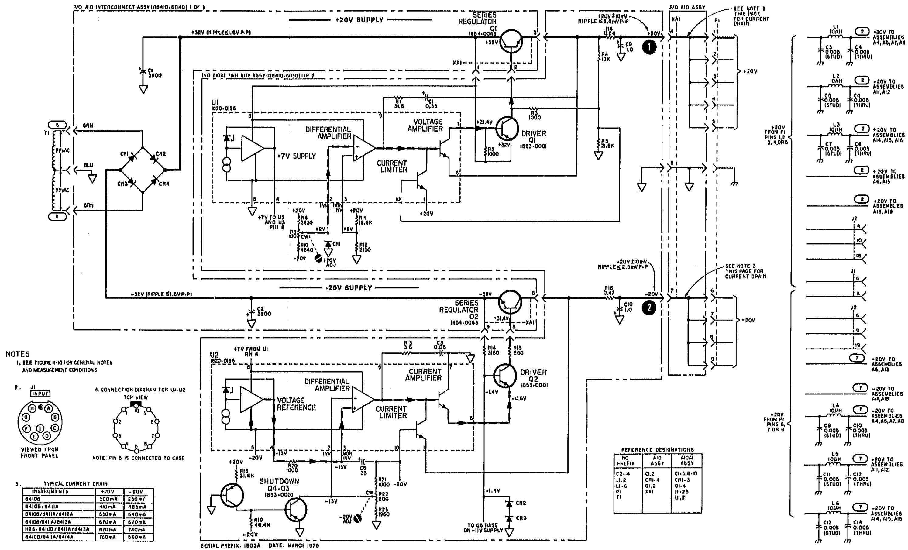
Figure 8-60. 8410B +20V and -20V Power Supply Schematic
