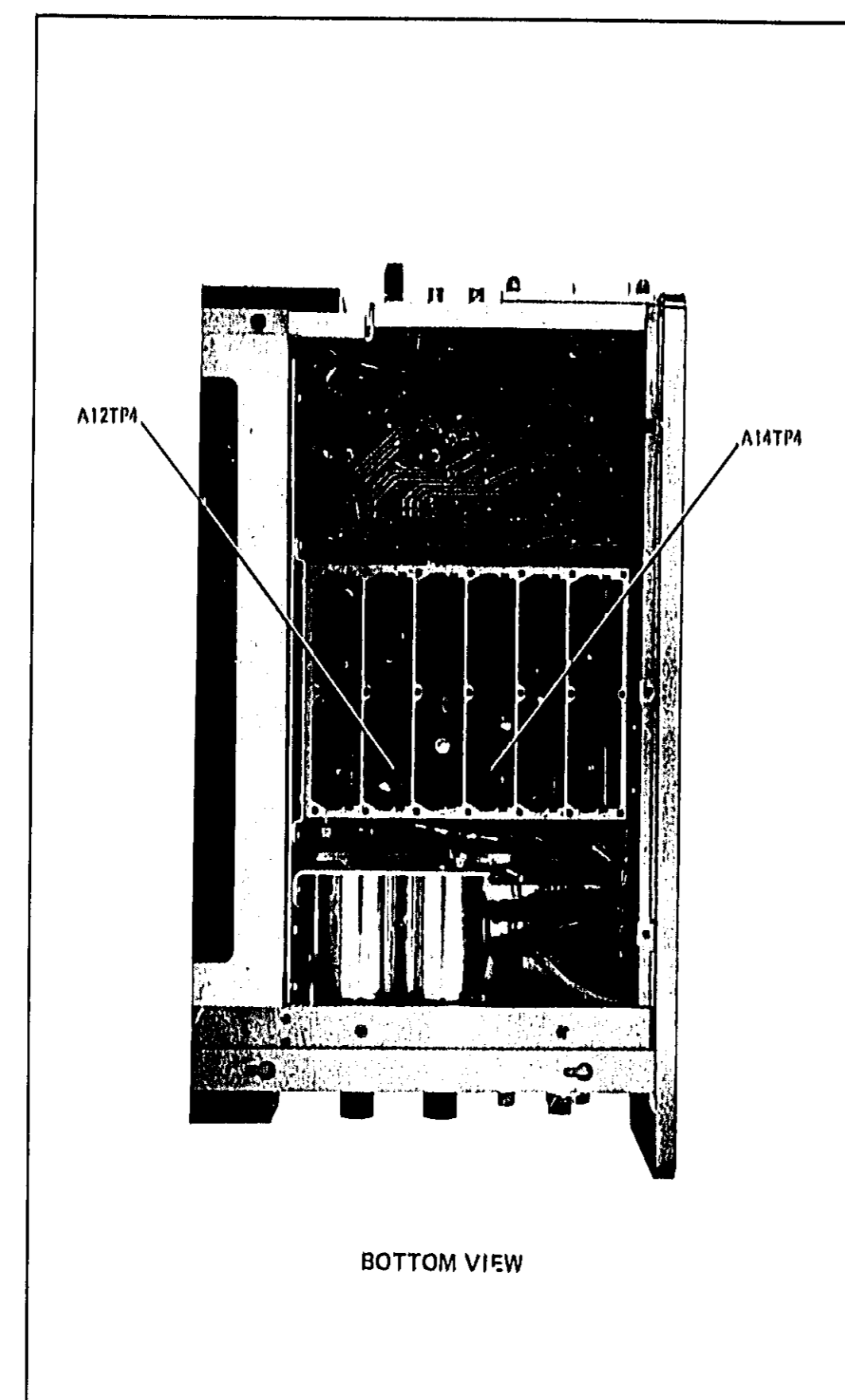
Figure 8-18. Models 8410B/8411A Interface Test Points ( 2 of 2 )
