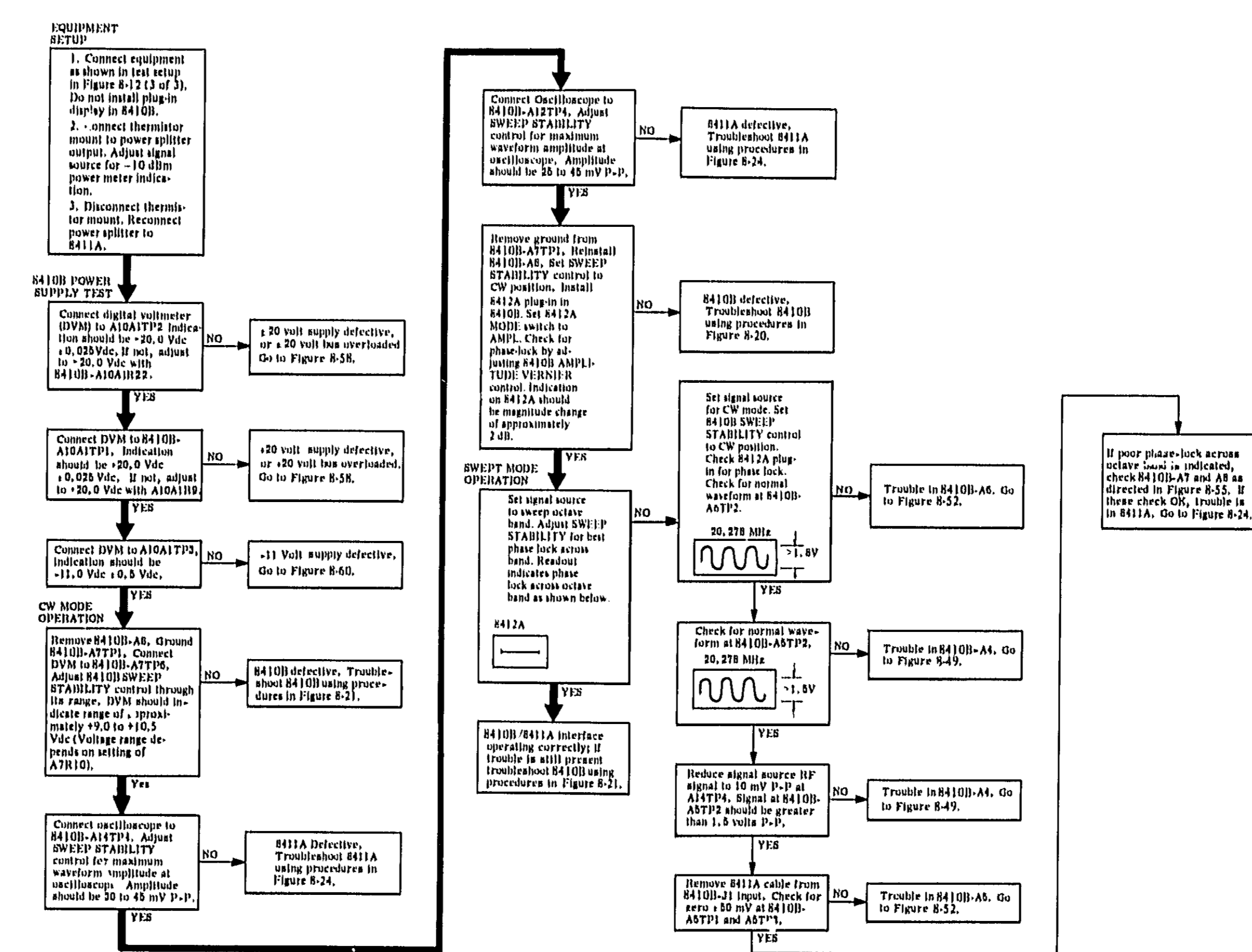
Figure 8-19. Model 8410B/8411A Interface Troubleshooting
