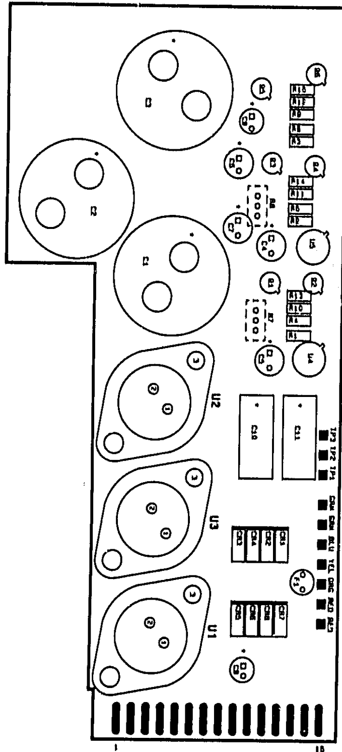
Figure 8-59. HP 8410B - A10 Parts Locations (CHANGE 14)
