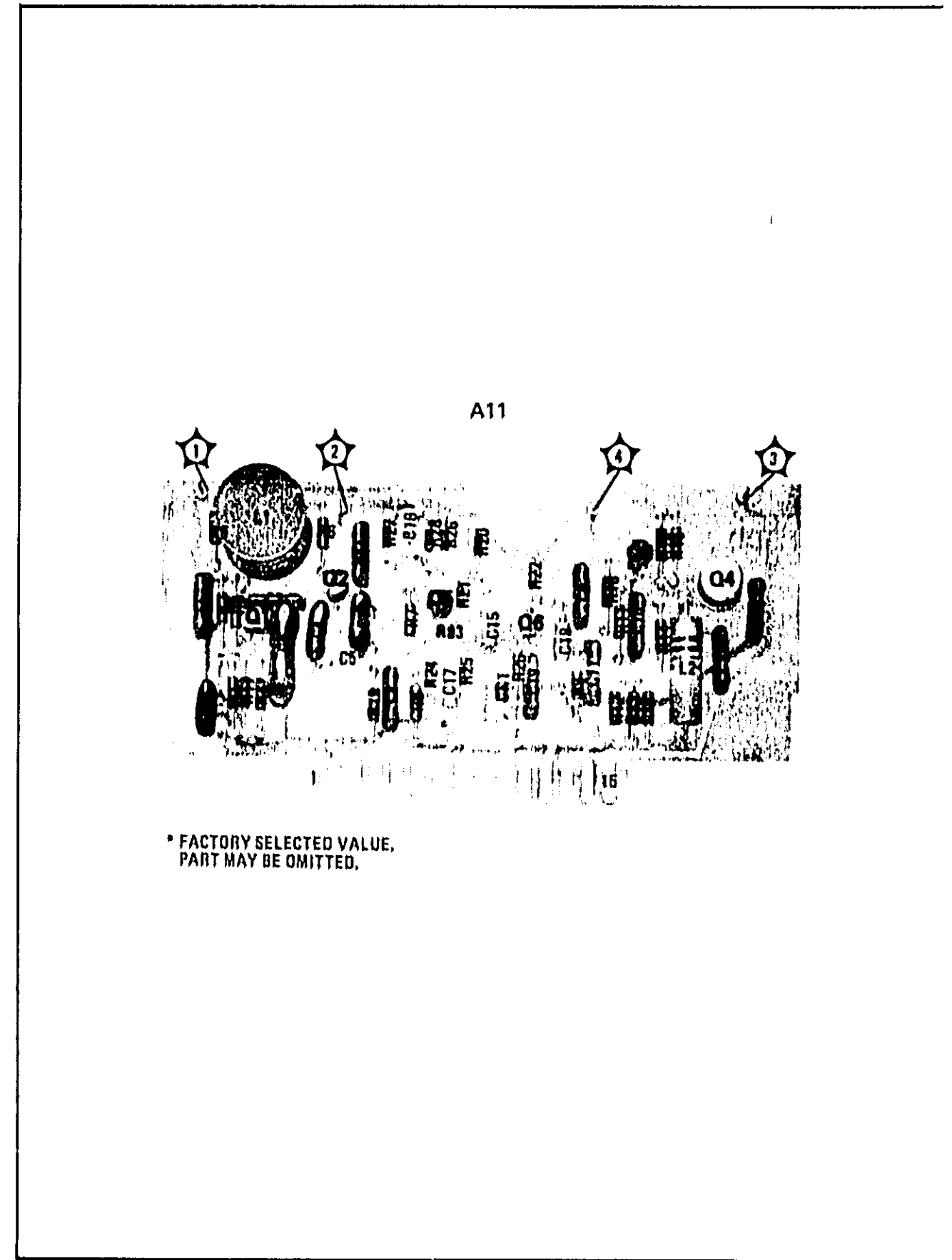
Figure S-17. 8410B-A11 Parts Location
