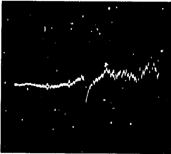
Figure 5-10. Power Hole 10 to 18 GHz Caused By Discontinuity in Sampler
