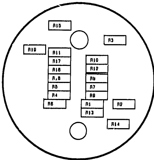
Figure 8-75. A3A1 0-60 dB Attenuator, Parts Location (CHANGE 11)
