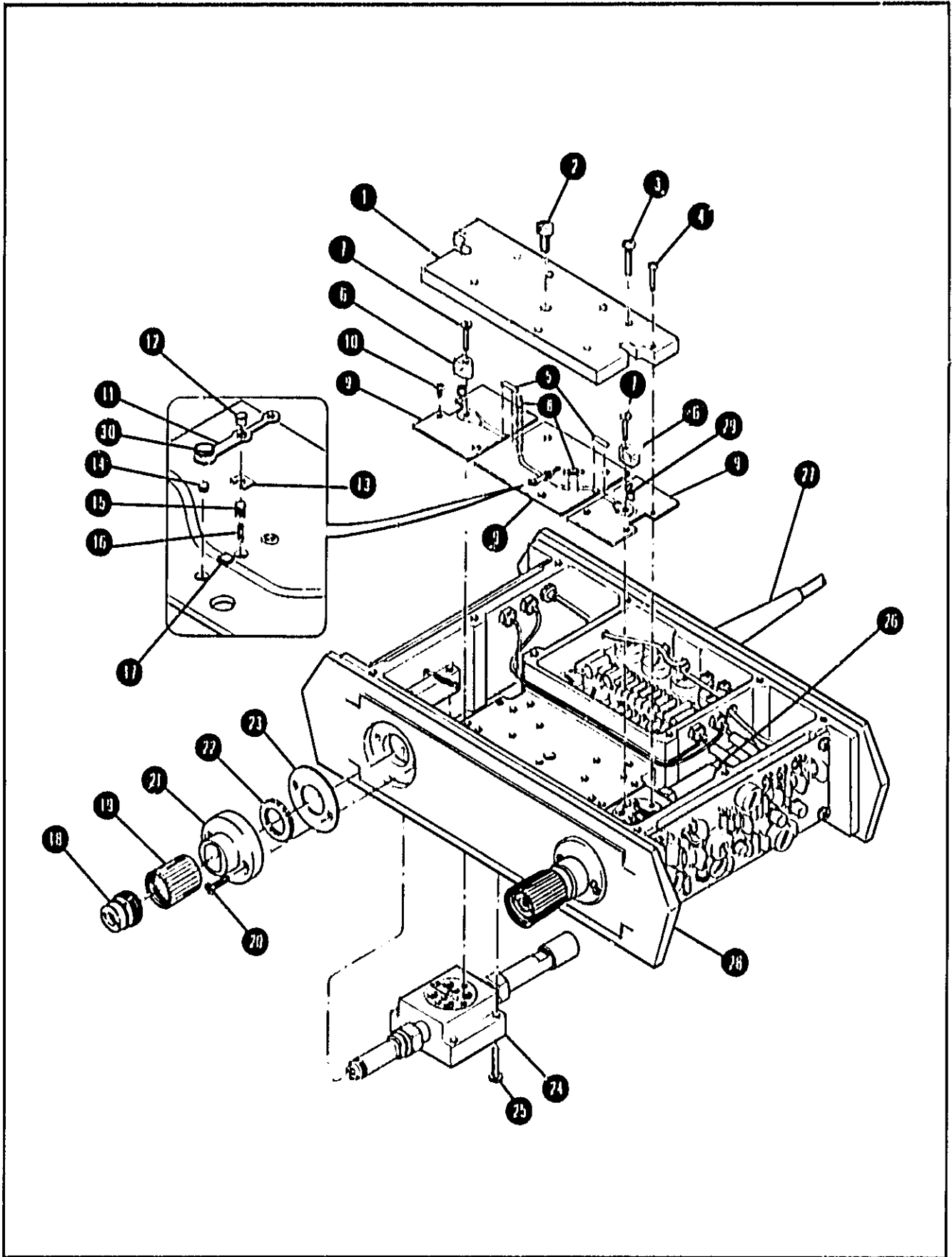
Figure 6-5. Model 8411A Exploded View (1 of 2)
