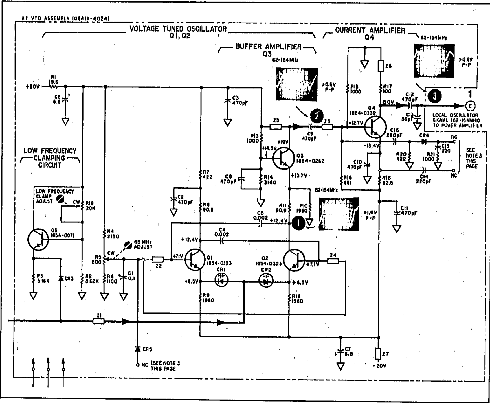
Figure 7-3. (P/O Figure 8-33.) 8411A-A7 Schematic Diagram (Change J)
