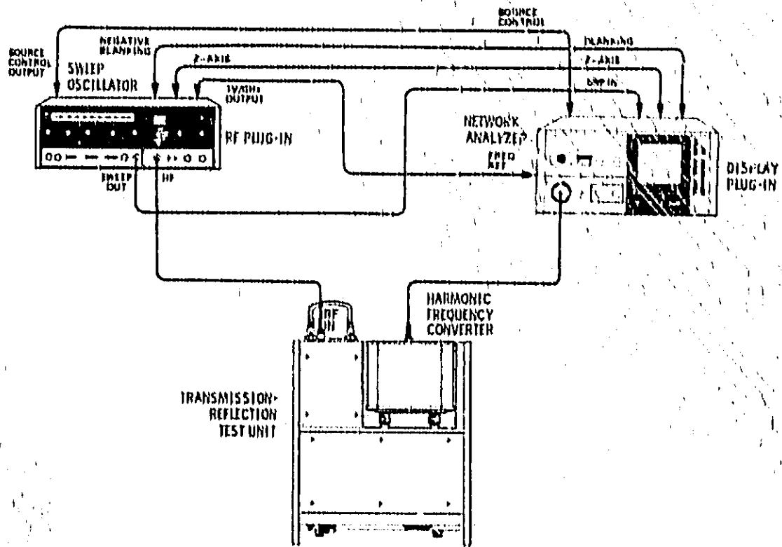
Figure 3-3. Typical Test Setup for Multioctave Measurements
