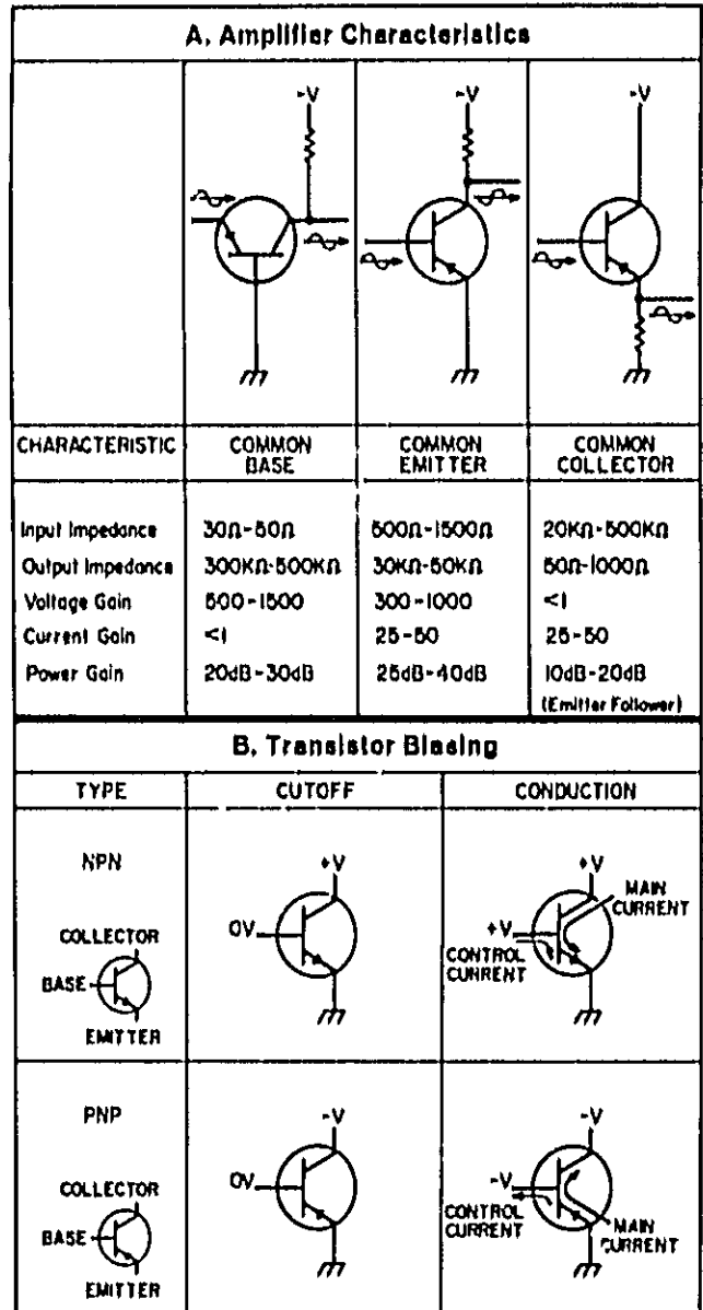
Figure 8-3. Transistor Operation
