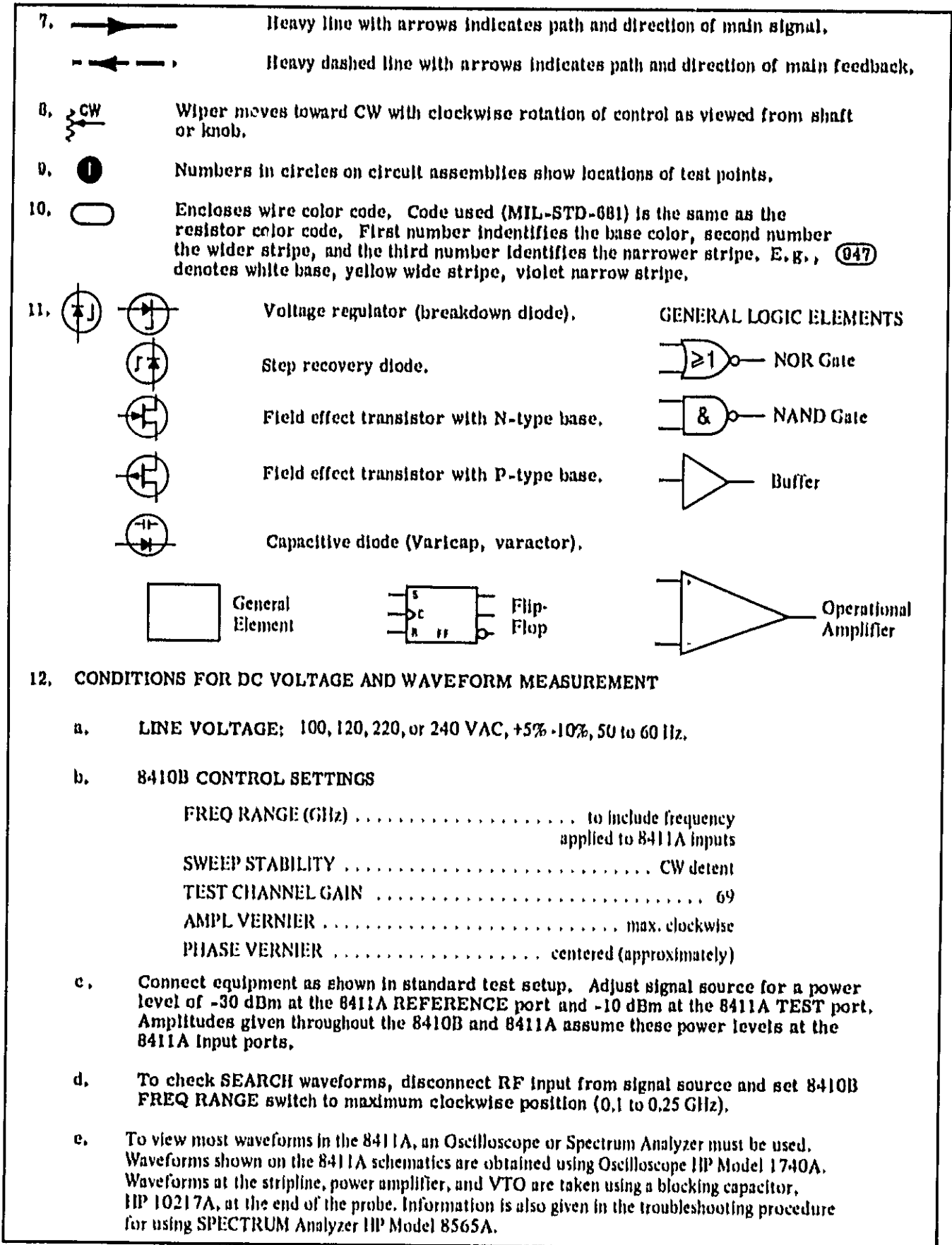
Figure 8-12. Schematic Diagram Notes (Sheet 2 of 3)
