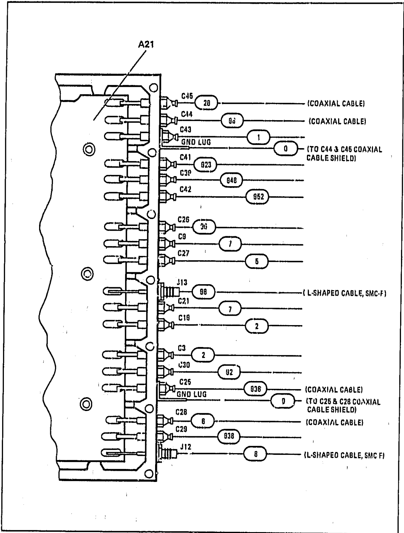
Figure 8-73. Wiring Connections to Movable Housing (CHANGE 6)
