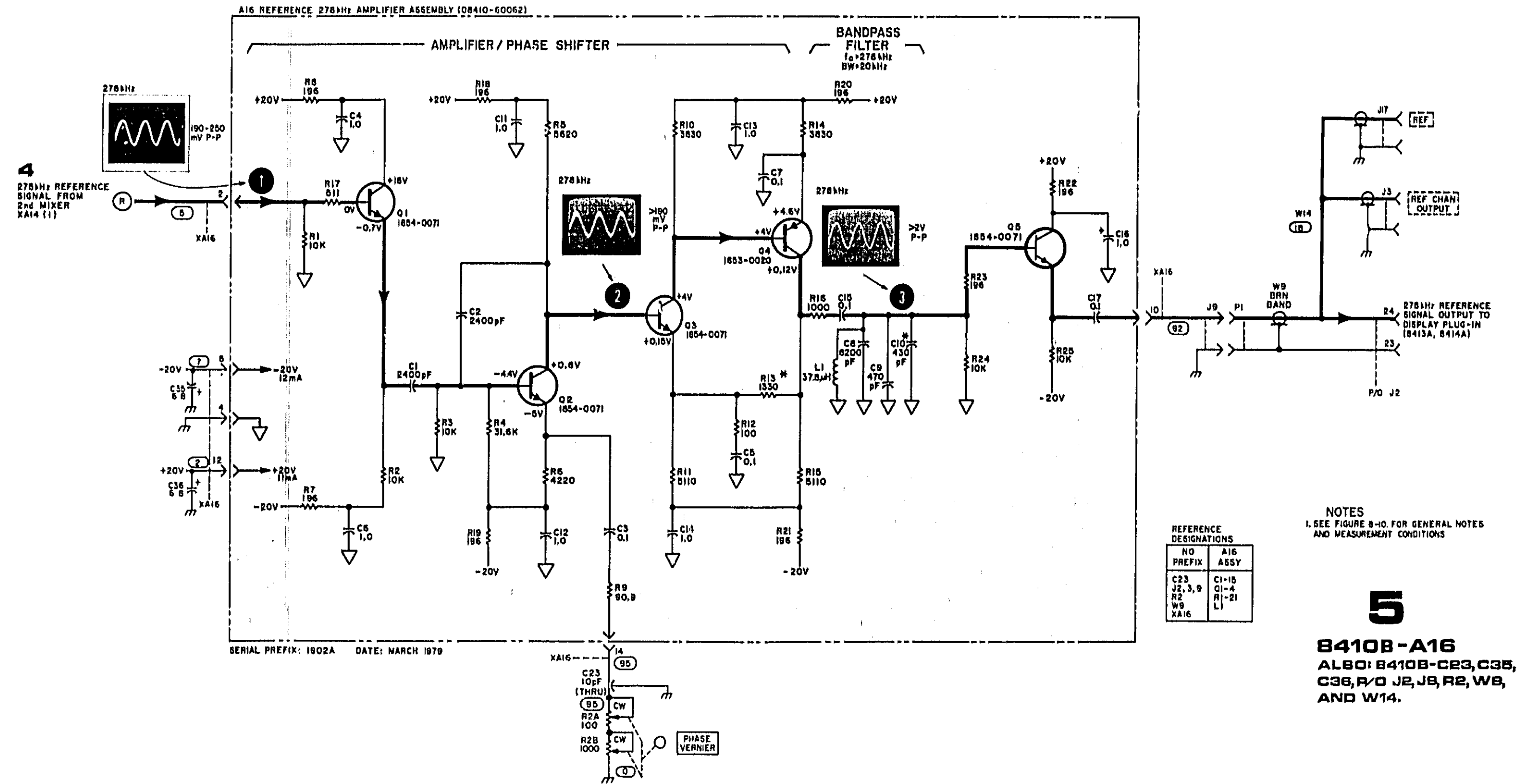
Figure 8-39. 8410B-A16 Schematic Diagram
