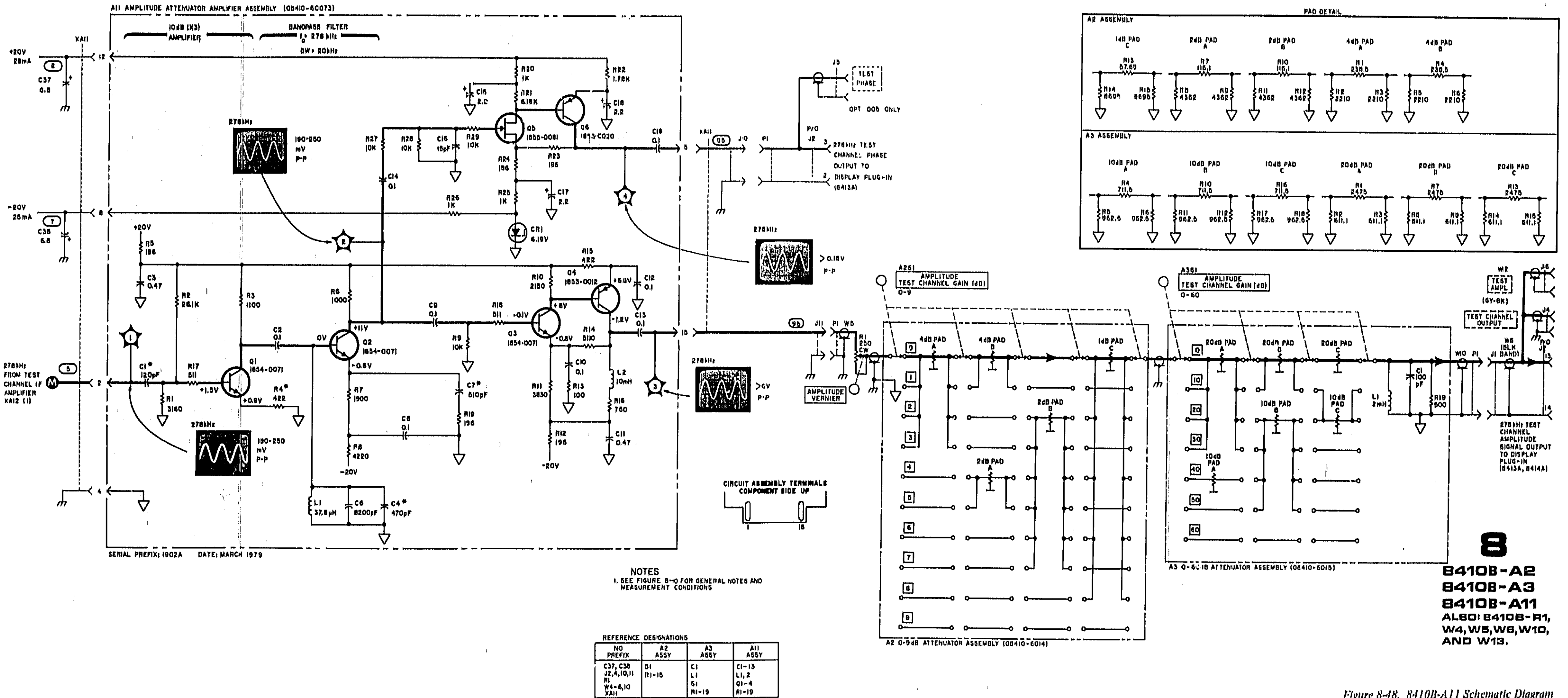
Figure 8-18. 8410B-A11 Schematic Diagram
