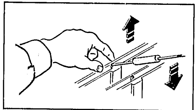
Figure 8-2. Printed Circuit Board Removal
