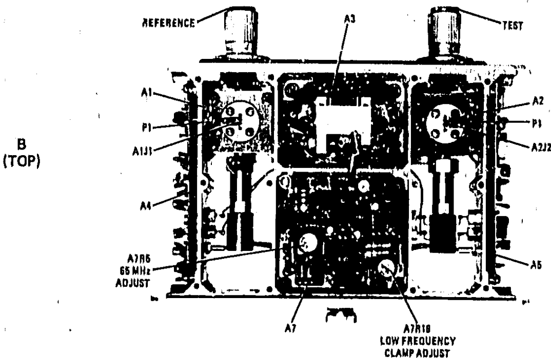
Figure 5-1. 8411A Adjustments Location and Preset Position
