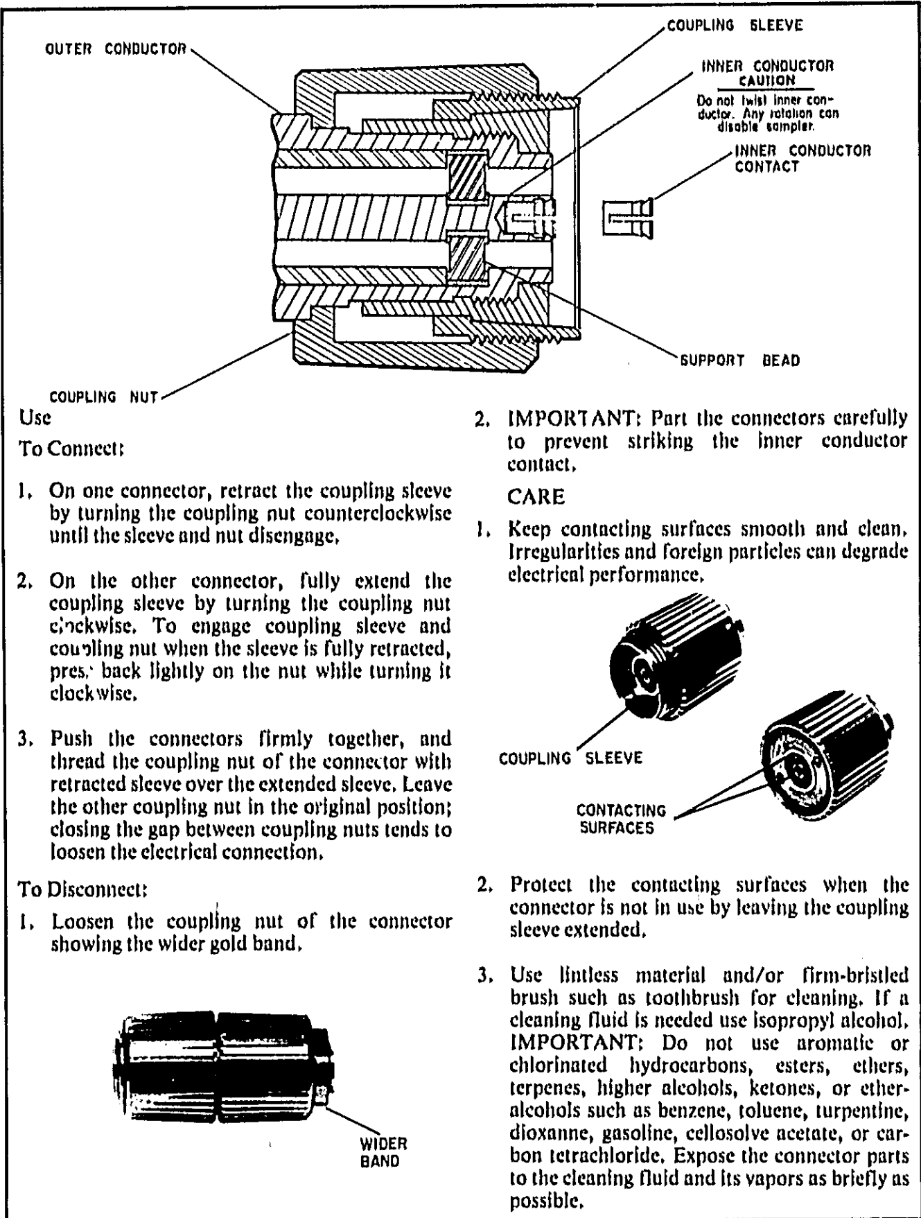
Figure 2-3. APC-7 Connectors
