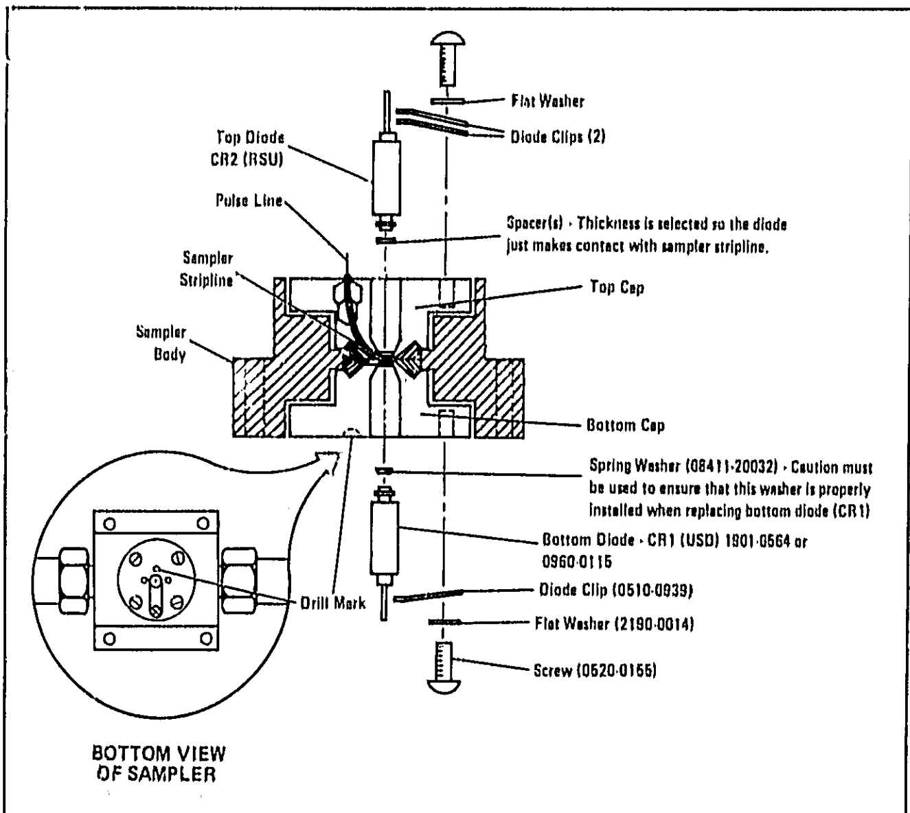
Figure 8-10. Sampler Diode Replacement
