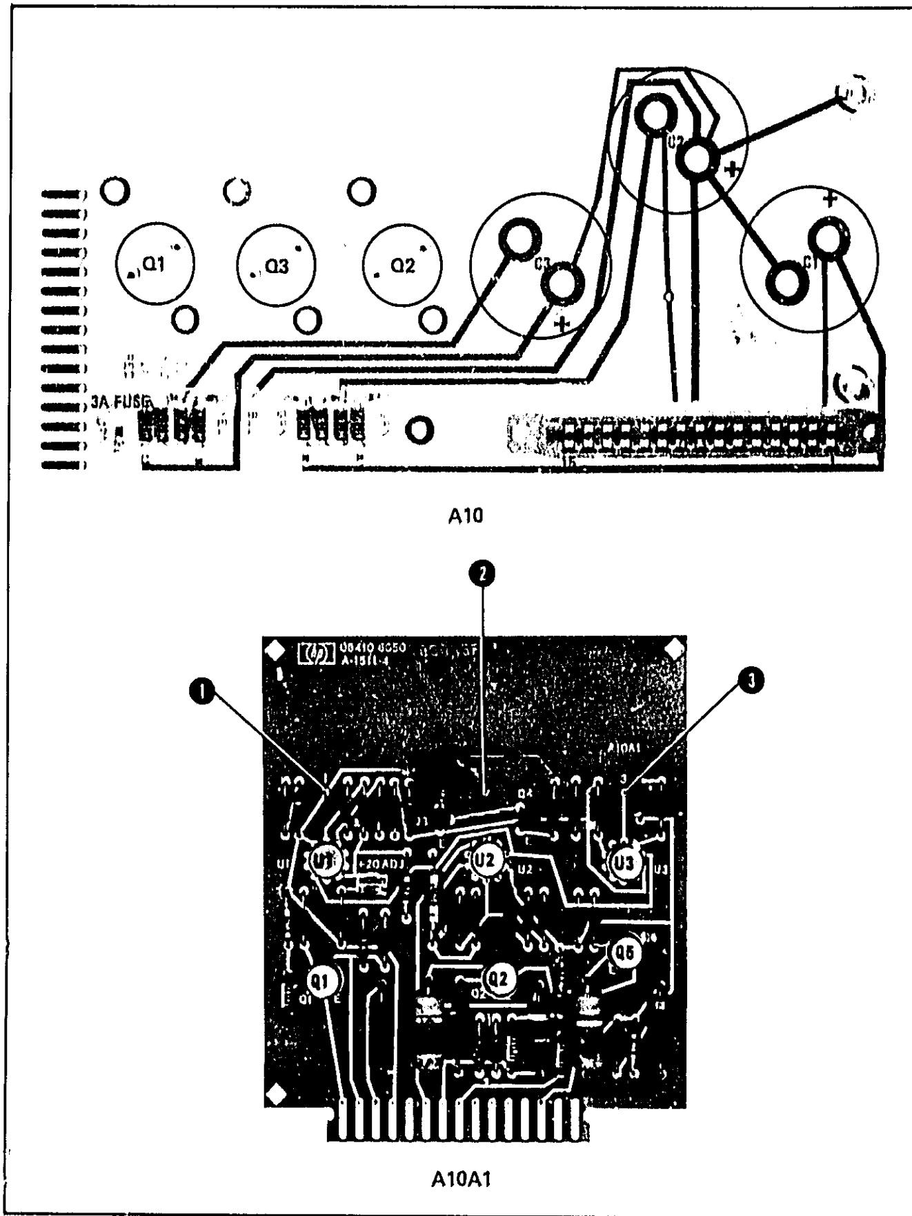
Figure 8-59. S410B-A10A1 Parts Location
