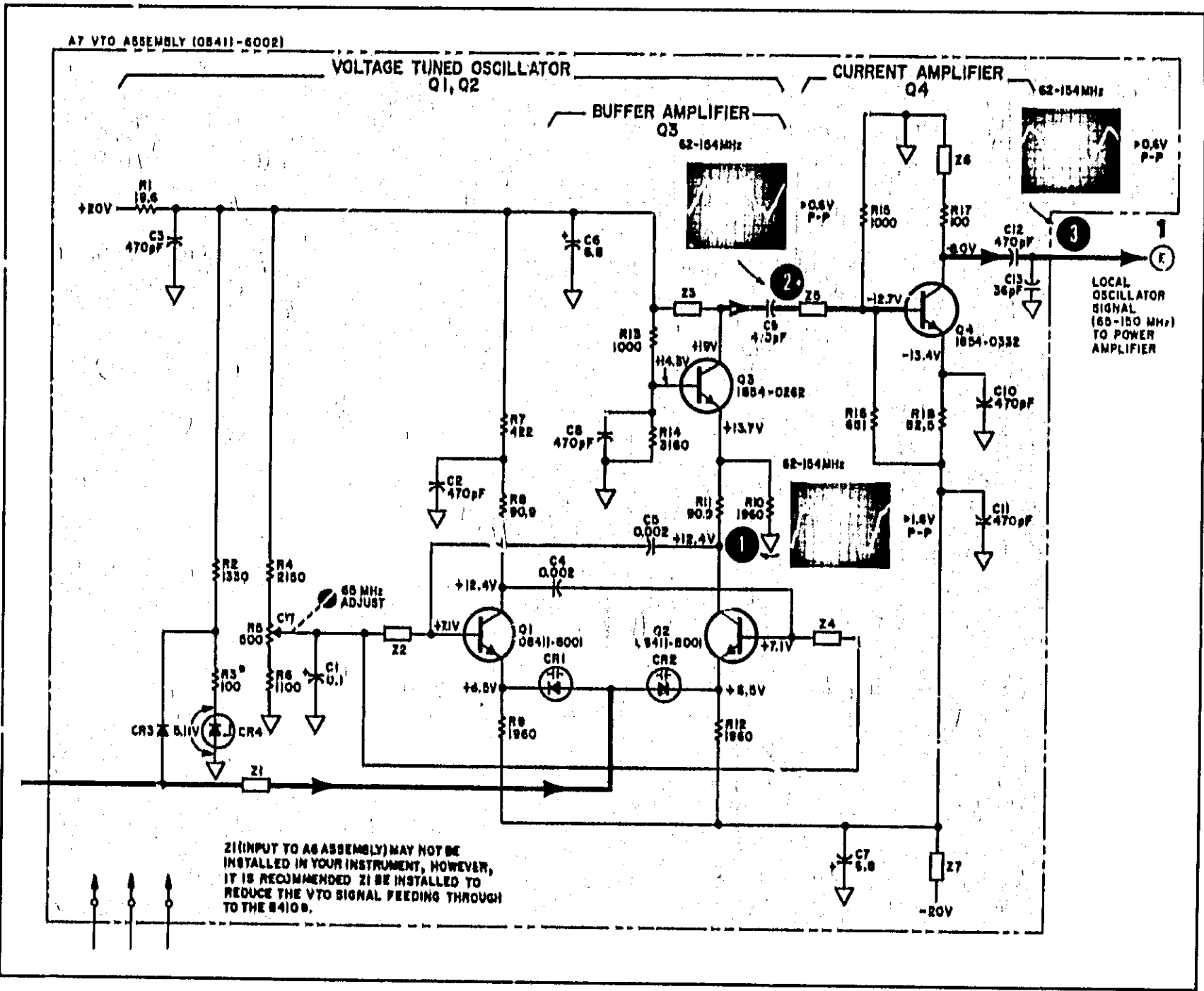
Figure 7-5. (P/O Figure 8-33.) 8411A-A7 Schematic Diagram (Change L)
