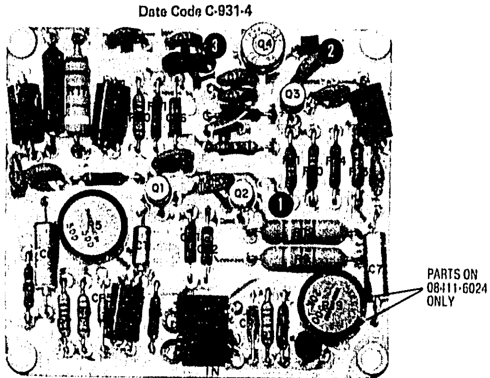
Figure 5-4. A7 VTO Assembly 08411-6024, Date Code C-931-4
