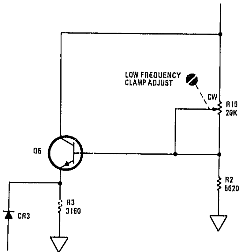
Figure 7-2. (P/O Figure 8-33) 8411A-A6 and A7, Schematic Diagram (CHANGE F)
