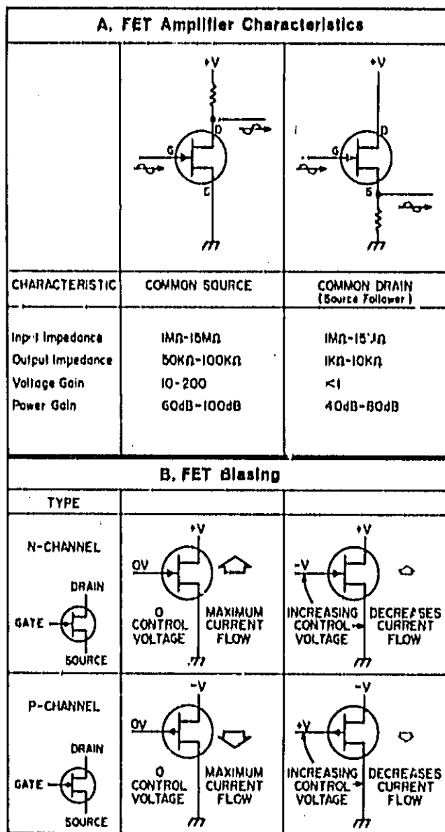
Figure 8-7. Field Effect Transistor Operation
