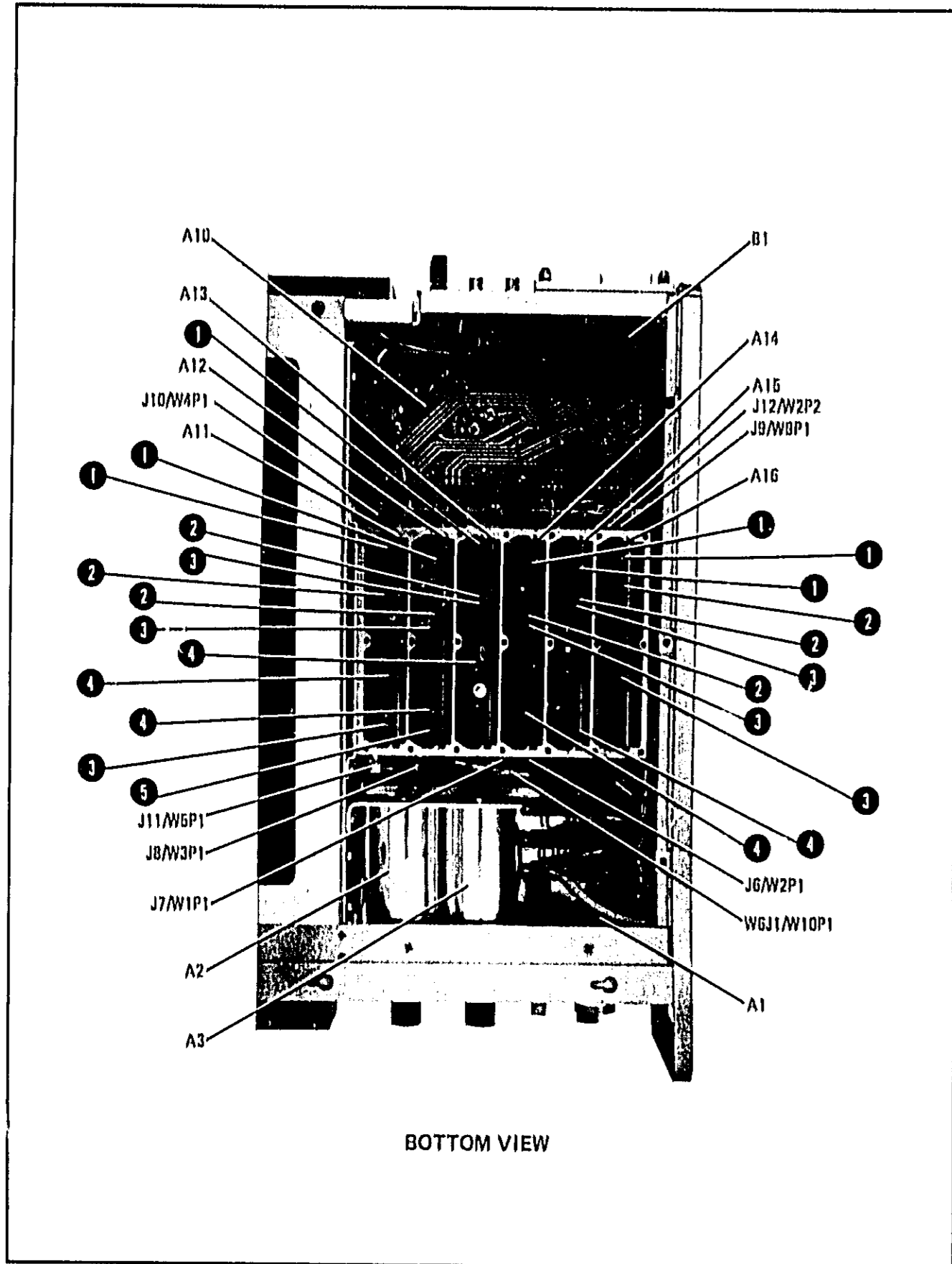
Figure 8-20. Model 8410B Test Points ( 2 of 2 )
