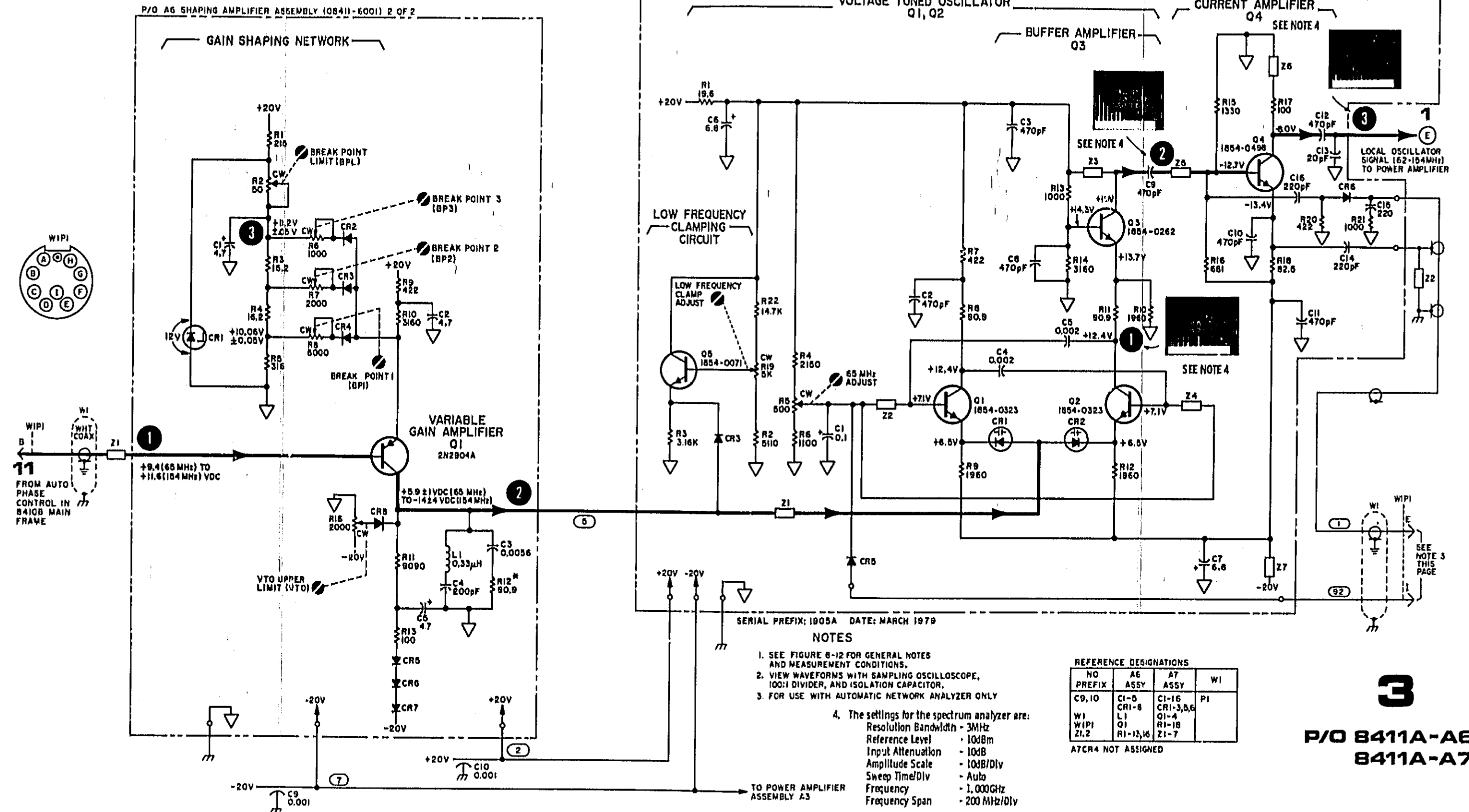
Figure 8-33. 8411A-A6 and A7 Schematic Diagram
