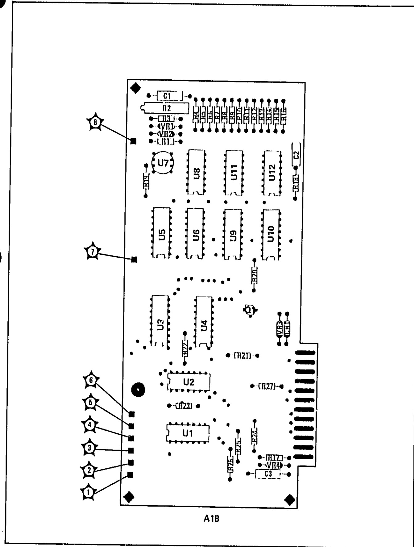
Figure 8-65. 8410B-A18 Parts Location
