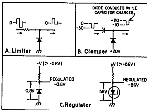
Figure 8-5. Basic Diode Circuits
