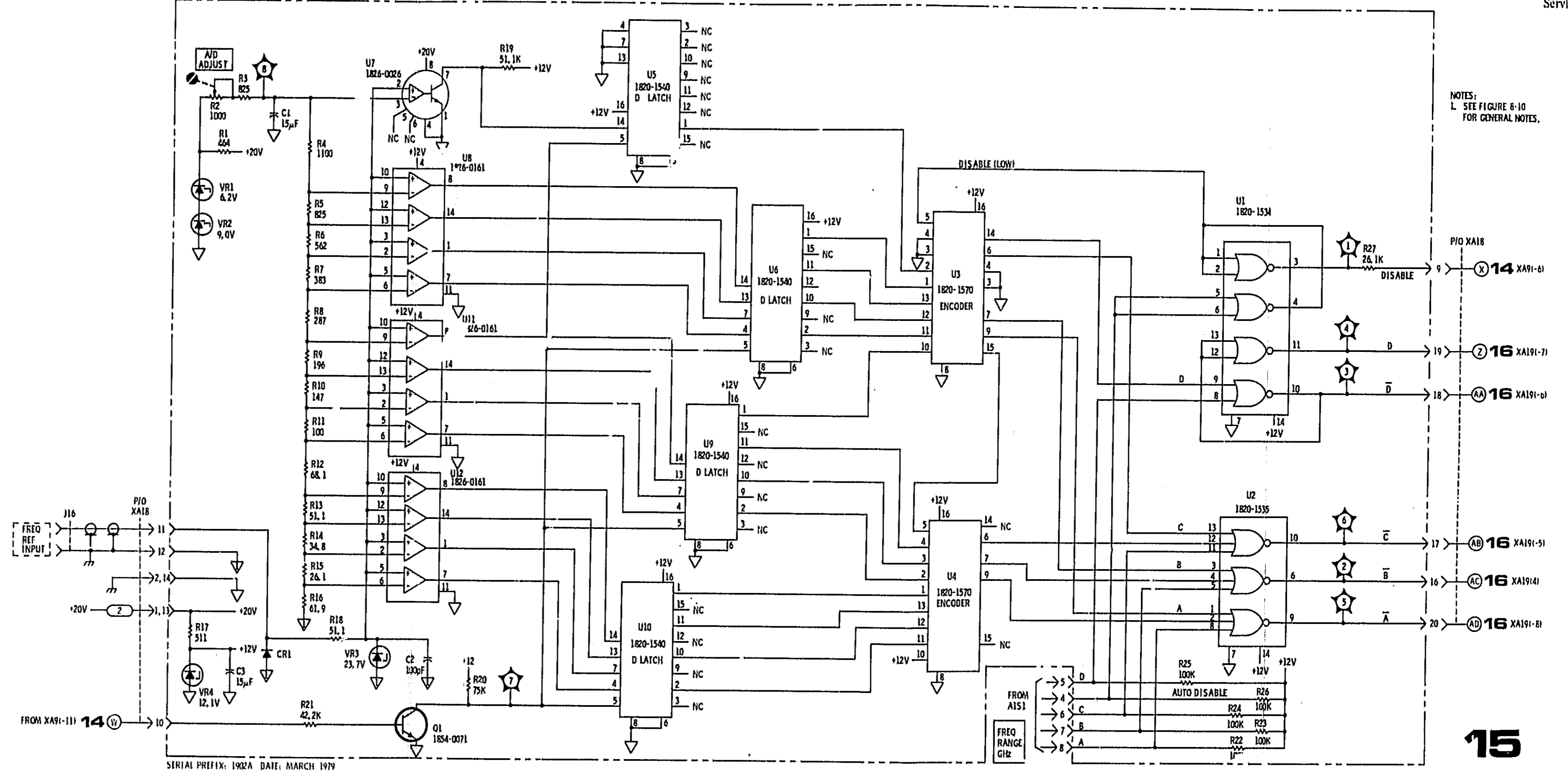
Figure 8-66. 8410B-A18 Schematic Diagram
