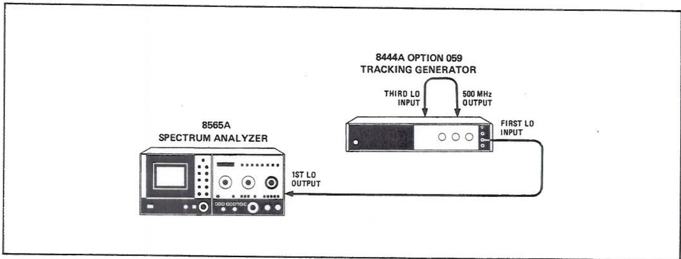
Figure E-5. Equipment Connections for 8444A Option 059/8565A
