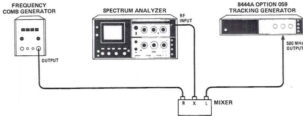
Figure E-3. 500 MHz L.O. Residual FM Check Equipment Setup
