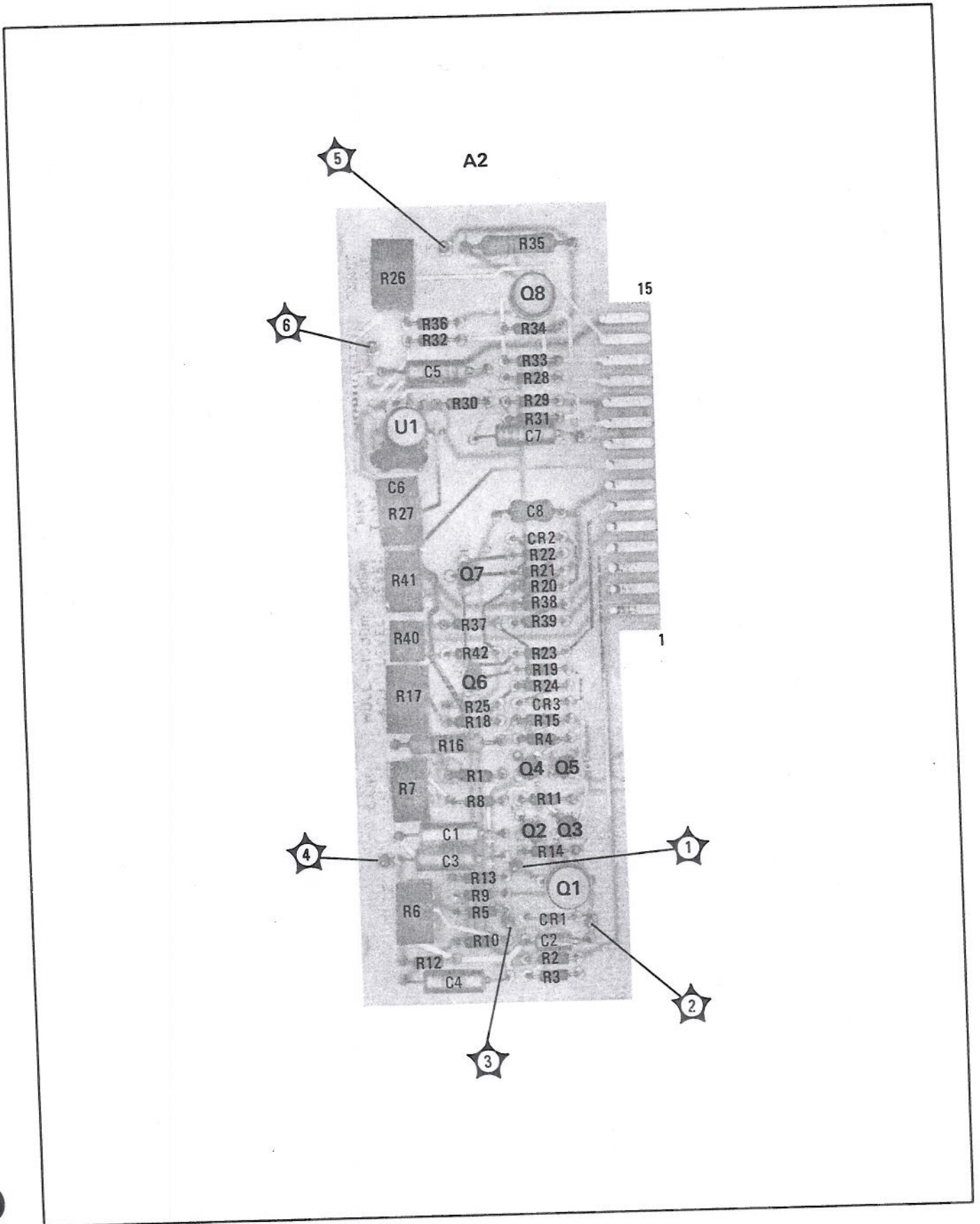
Figure 8-14. A2 Modulator/Oscillator Driver Assy, Component Location
