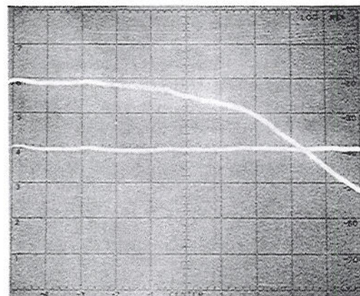
Figure 3-9. Amplifier Gain and Bandwidth CRT Display
