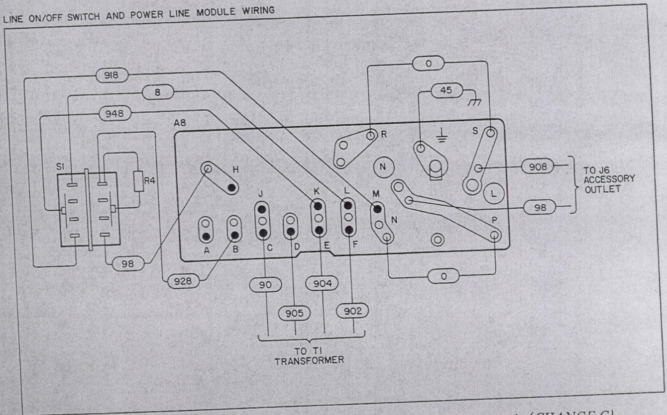
Figure 7-3. P/O Figure 8-17, Power Supply and Input Circuit, Schematic (CHANGE C)
