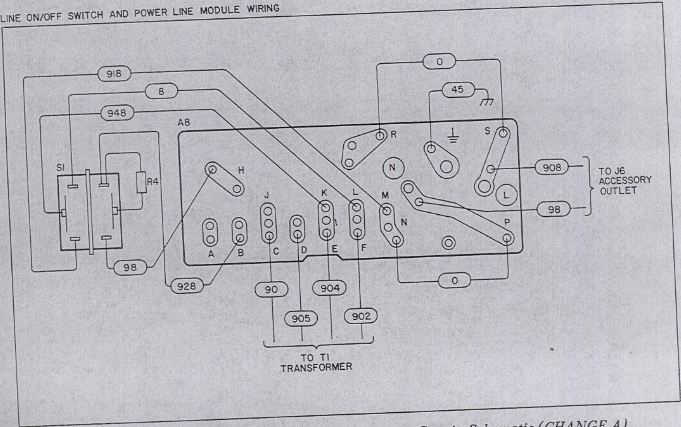
Figure 7-2. P/O Figure 8-17, Power Supply and Input Circuit, Schematic (CHANGE A)
