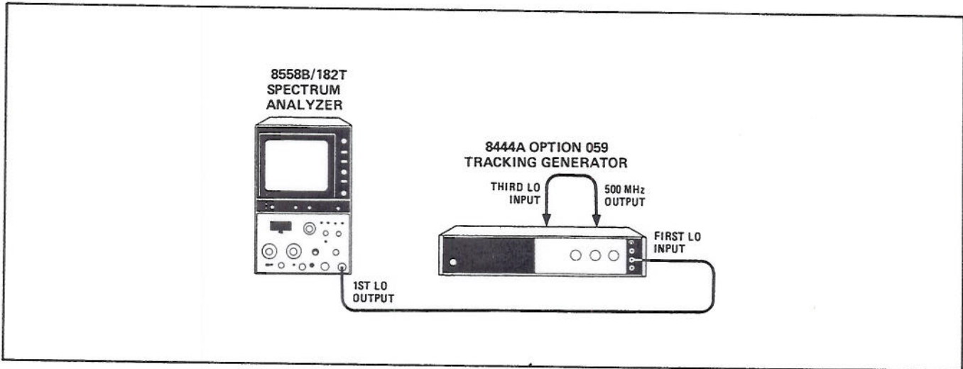
Figure E-4. Equipment Connections for 8444A Option 059/8558B
