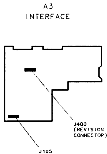
Figure 8-1. A3 Test Connectors
