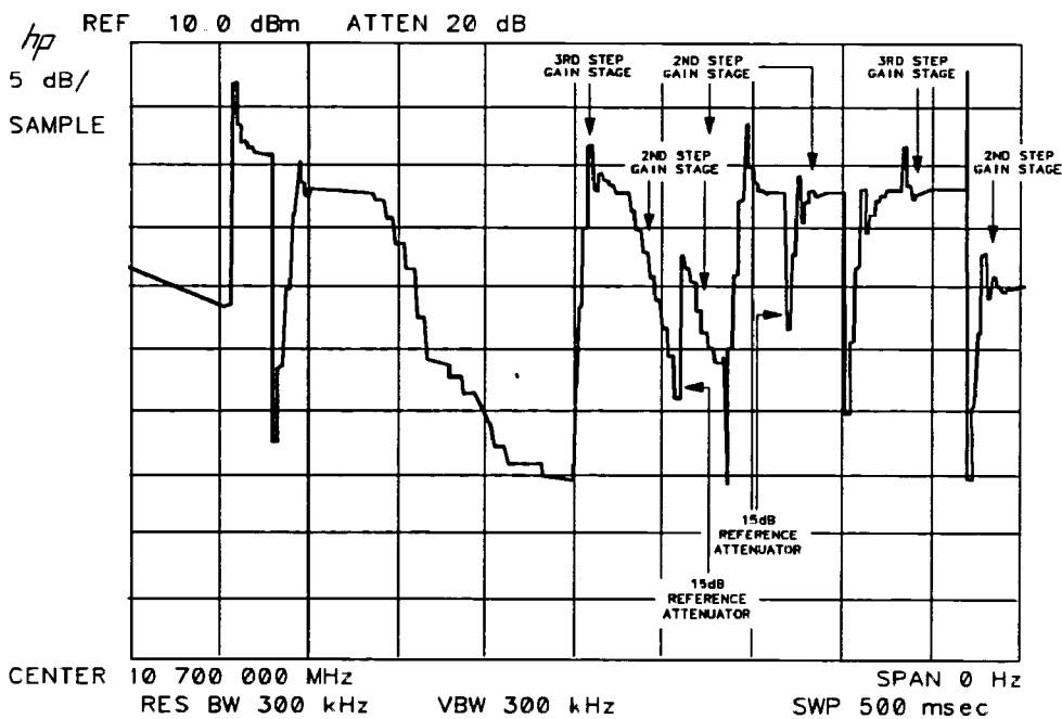
Figure 9-5. Detailed IF Adjust Signature (2)
