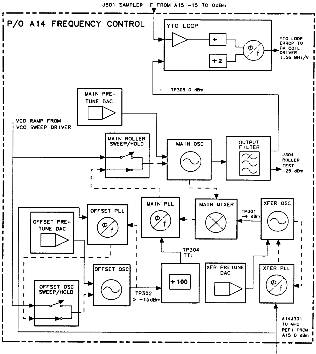
Figure 11-13. Simplified A14 Assembly Block Diagram
