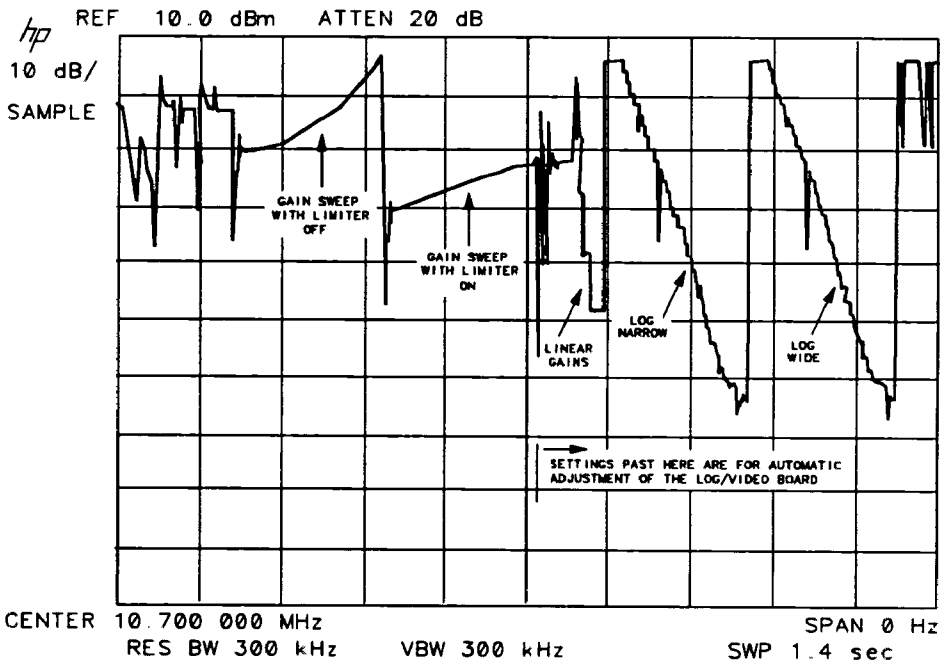
Figure 9-6. Detailed IF Adjust Signature (3)
