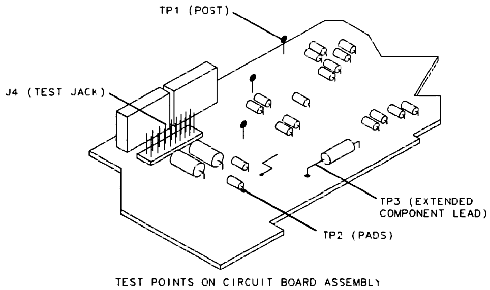
Figure 7-1. Assembly Test Points
