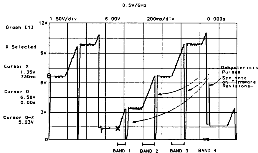
Figure 12-3. Rear-Panel SWP Output
