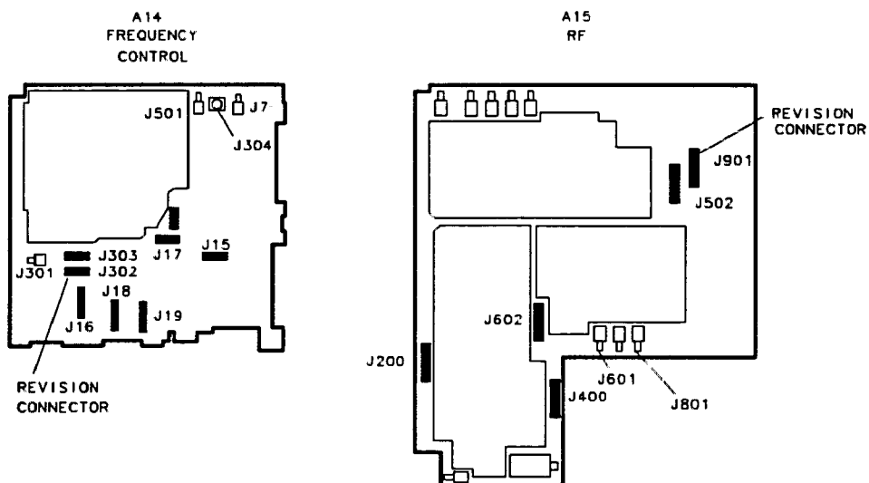
Figure 12-1. A14 and A15 Test Connectors
