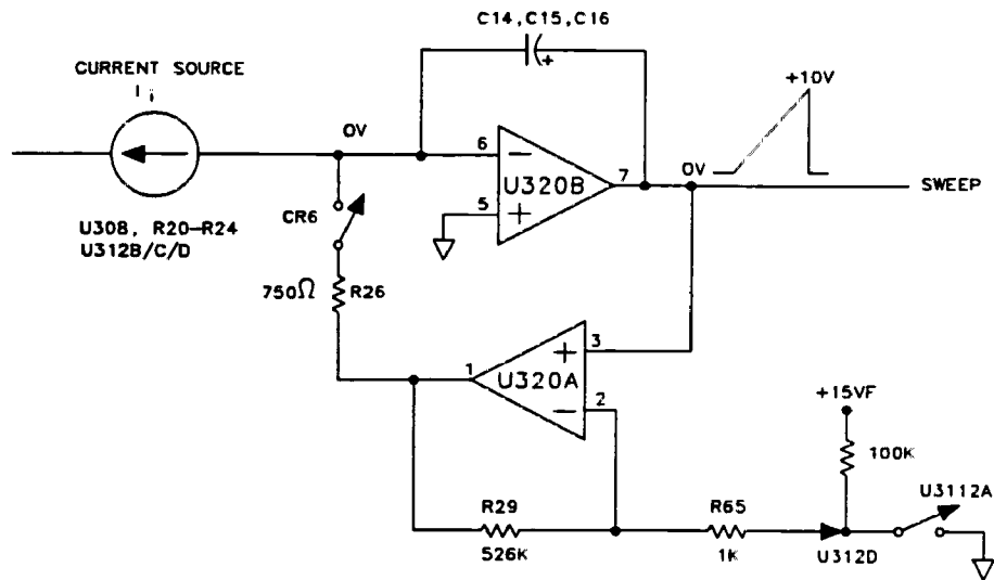
Figure 11-10. Simplified Sweep Generator
