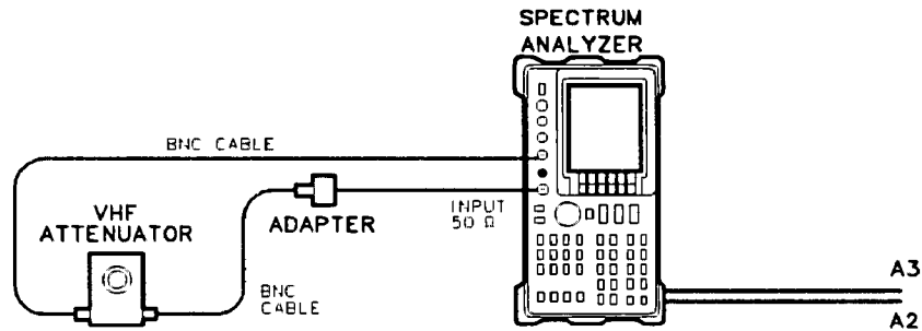
Figure 2-2. Display Adjustment Setup
