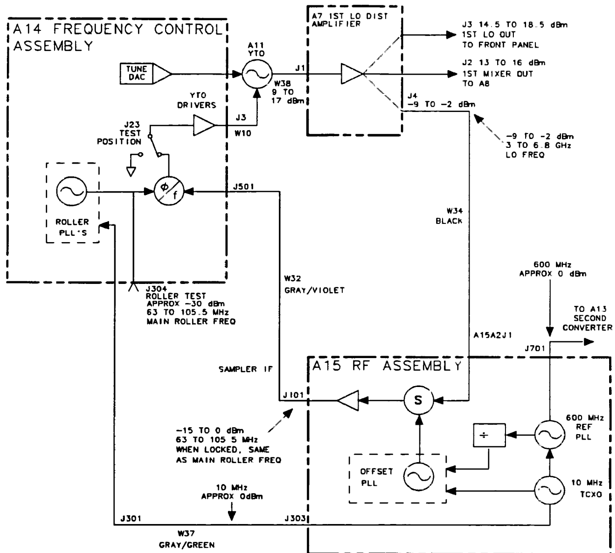
Figure 11-12. Simplified Synthesizer Section
