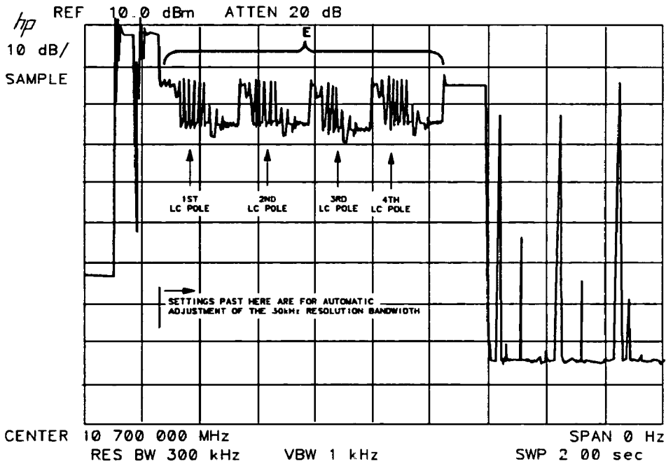
Figure 9-8. Detailed IF Adjust Signature (5)
