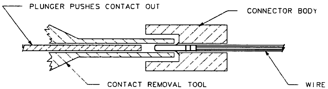
Figure 3-29. W3 Cable Connector
