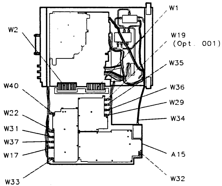
Figure 5-5. Bottom View (A15 Unfolded)
