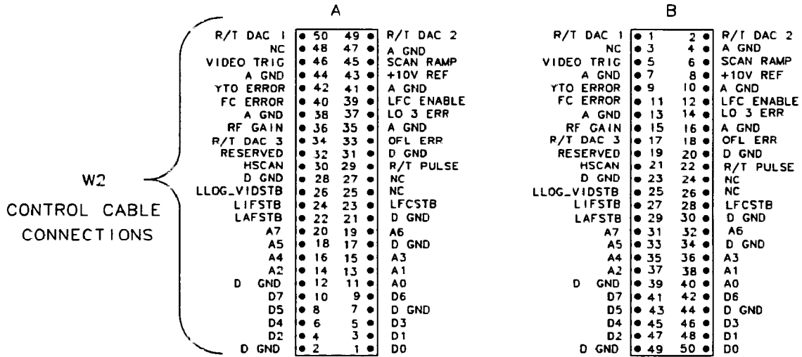
Figure 7-2. Ribbon Cable Connections (1 of 2)
