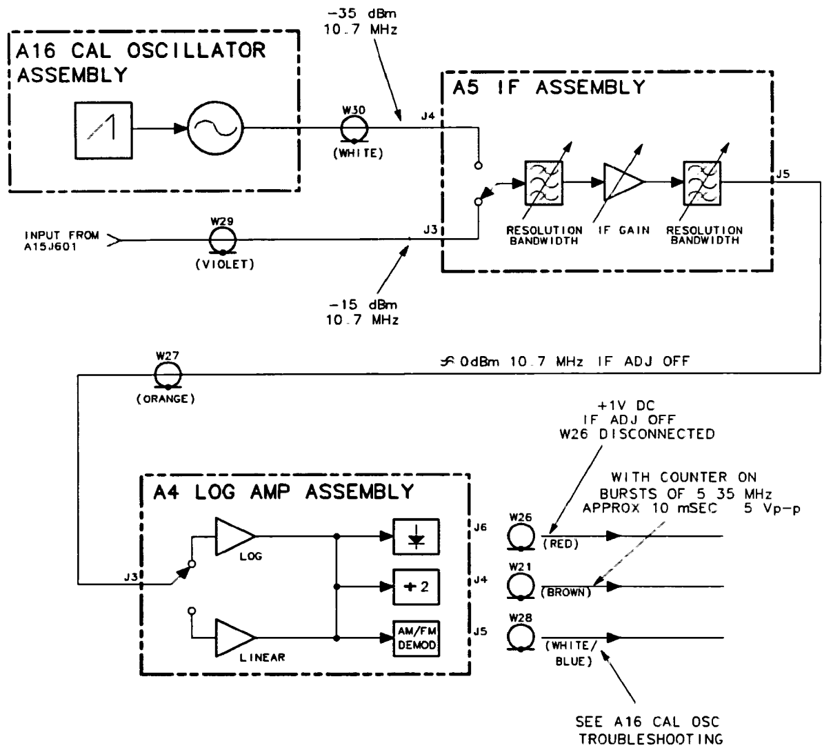
Figure 9-2. IF Section Troubleshooting with TAM
