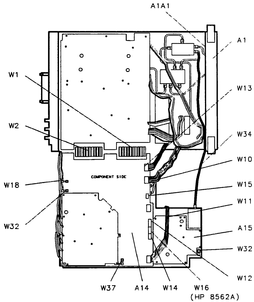
Figure 5-6. Bottom View (A15 and A14 Unfolded)
