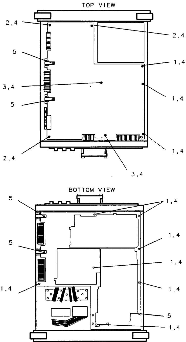
Figure 4-1. Parts Identification, Assembly Mounting (1 of 2)
