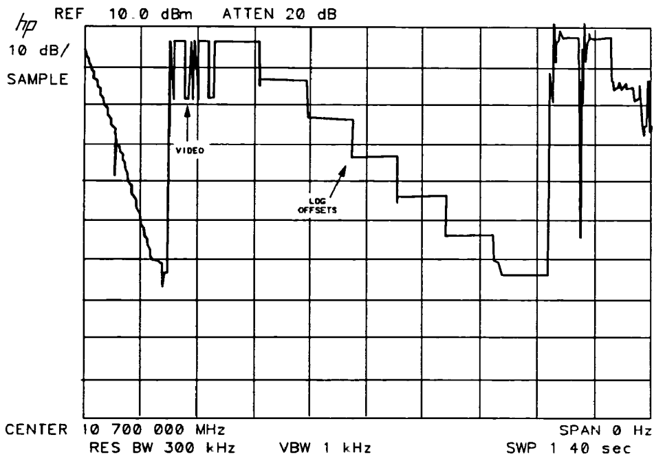
Figure 9-7. Detailed IF Adjust Signature (4)
