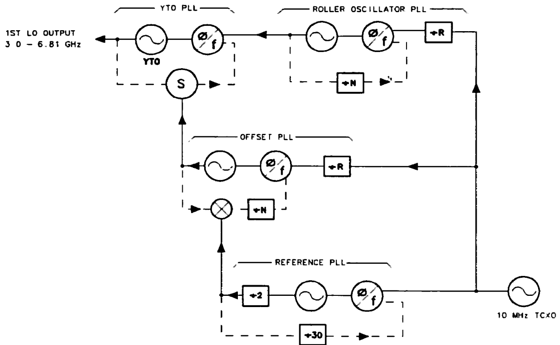
Figure 7-4. Phase Lock Loops
