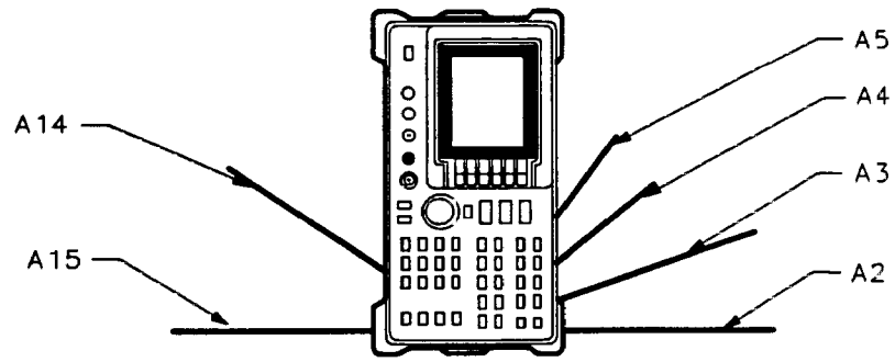
Figure 5-1. Hinged Assemblies
