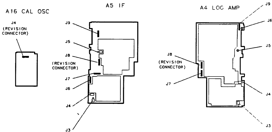
Figure 9-1. A4, A5, and A16 Test Connectors
