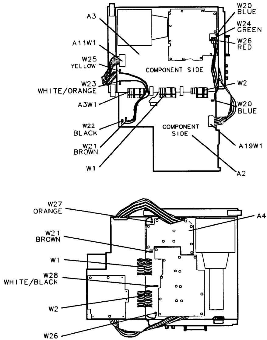
Figure 3-9. Assembly Cables (1 of 2)
