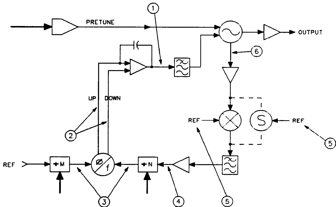
Figure 11-5. Unlocked PLL
