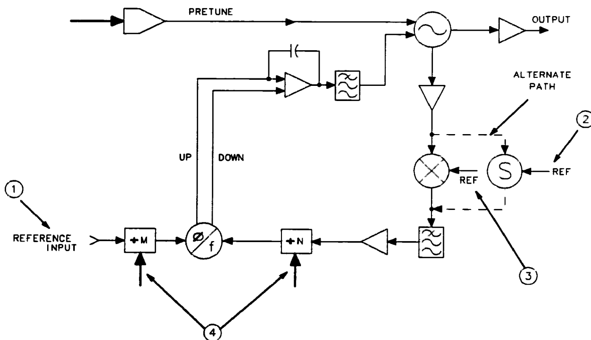
Figure 11-4. PLL Locked at Wrong Frequency
