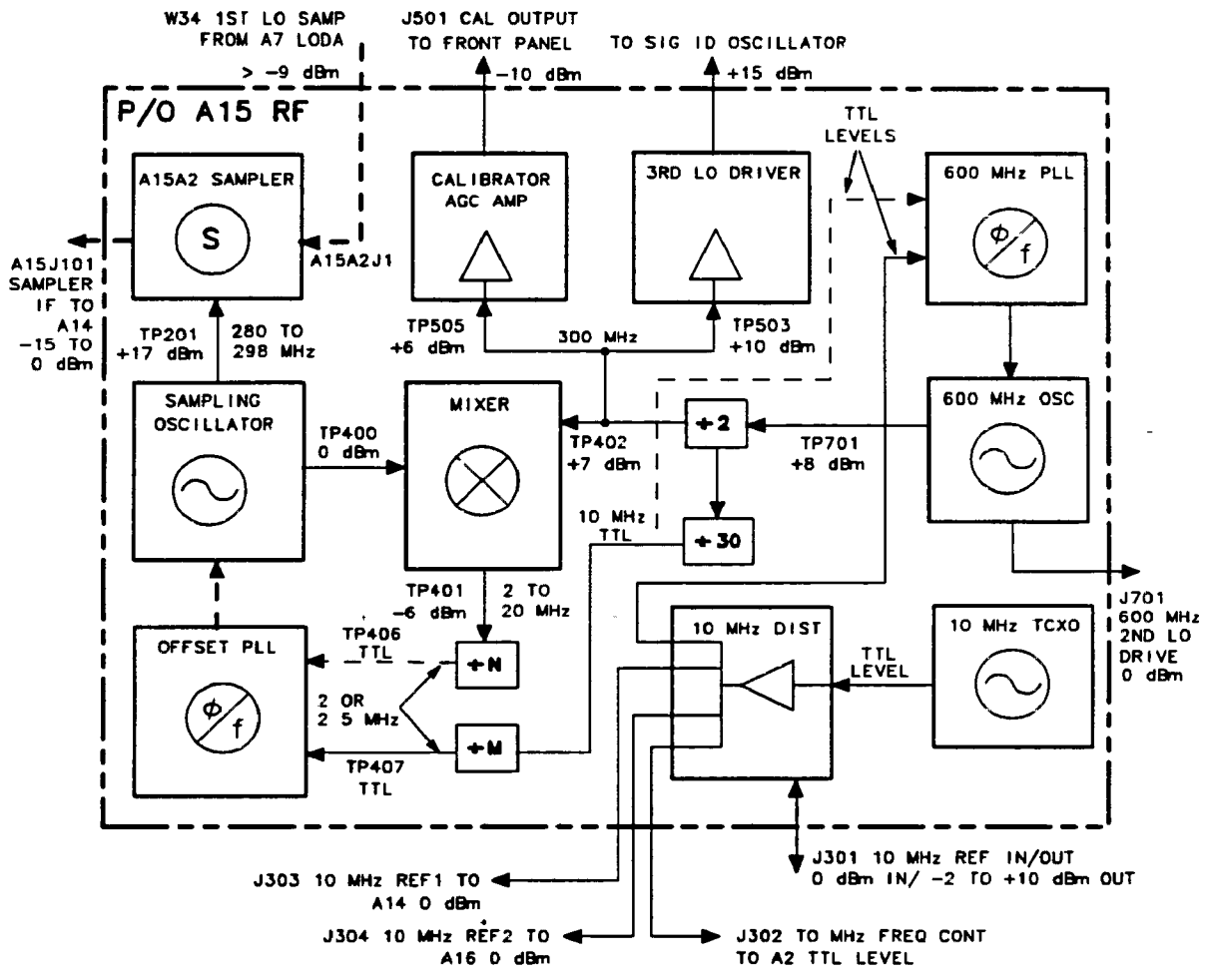
Figure 11-14. Simplified A15 Assembly Block Diagram
