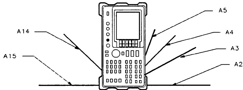
Figure 3-1. Hinged Assemblies
