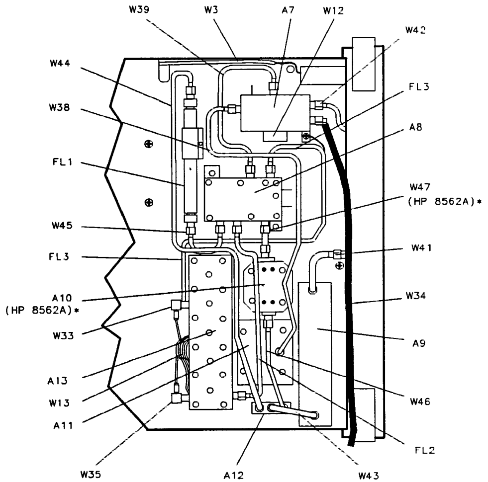
Figure 5-7. Front End
