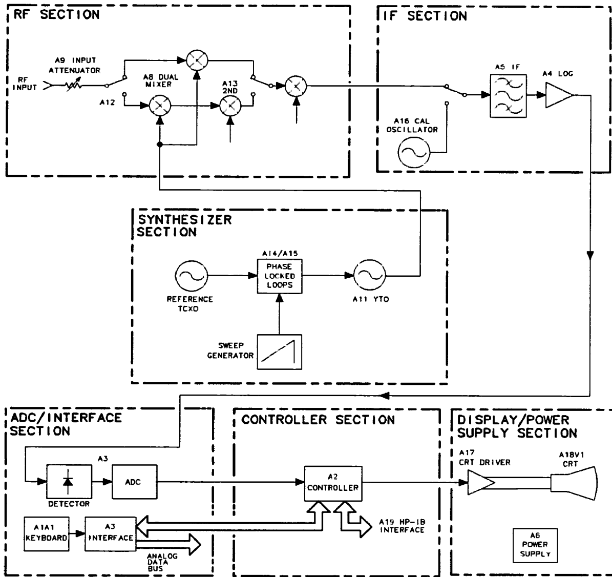
Figure 7-3. Functional Sections
