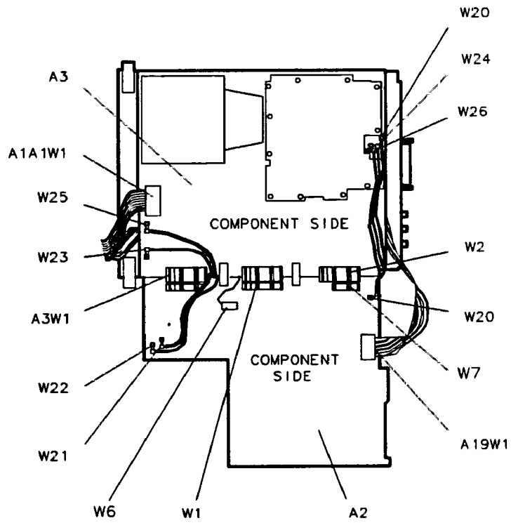
Figure 5-2. Top View (A2 Unfolded)
