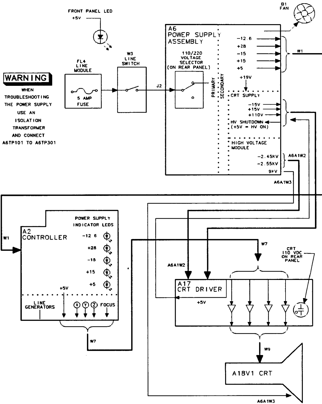
Figure 13-1. Simplified Section Block Diagram
