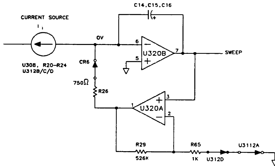
Figure 11-11. Simplified Sweep Generator During Retrace
