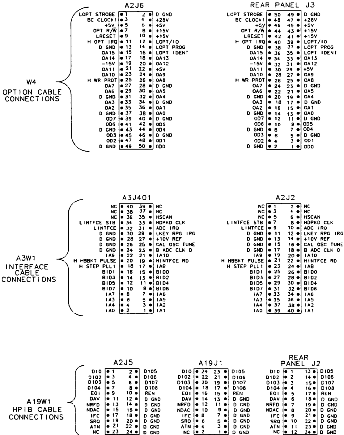
Figure 7-2. Ribbon Cable Connections (2 of 2)
