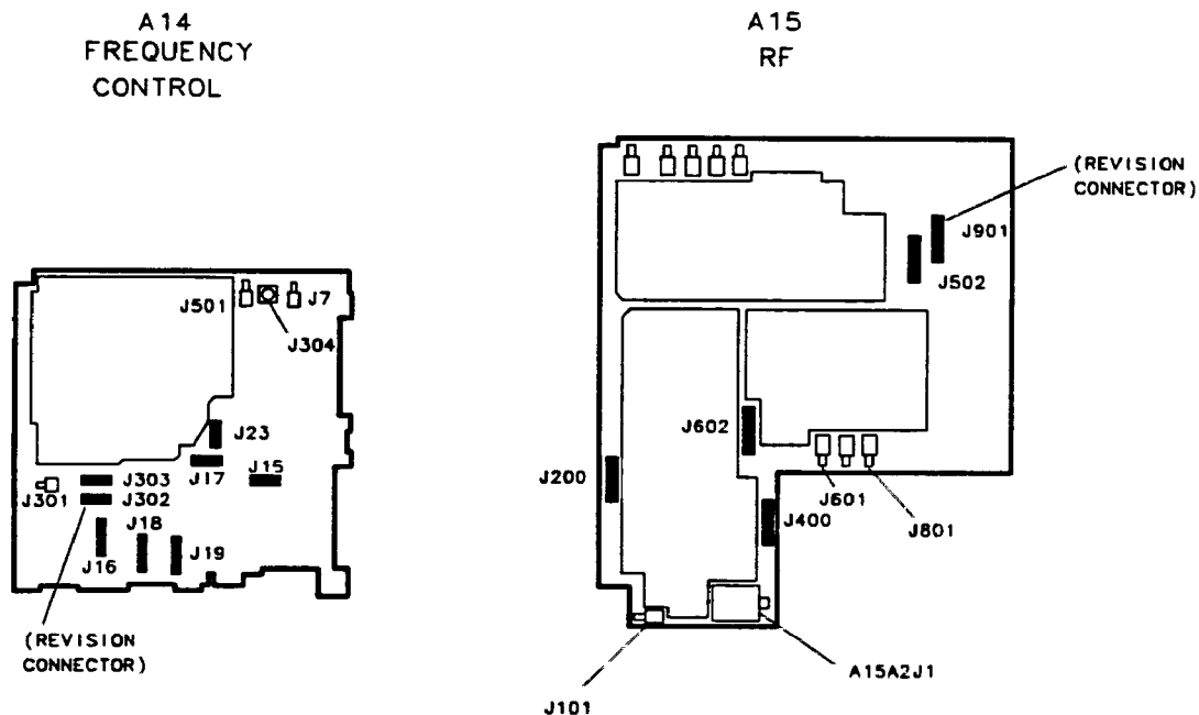
Figure 11-3. A14 and A15 Test Connectors
