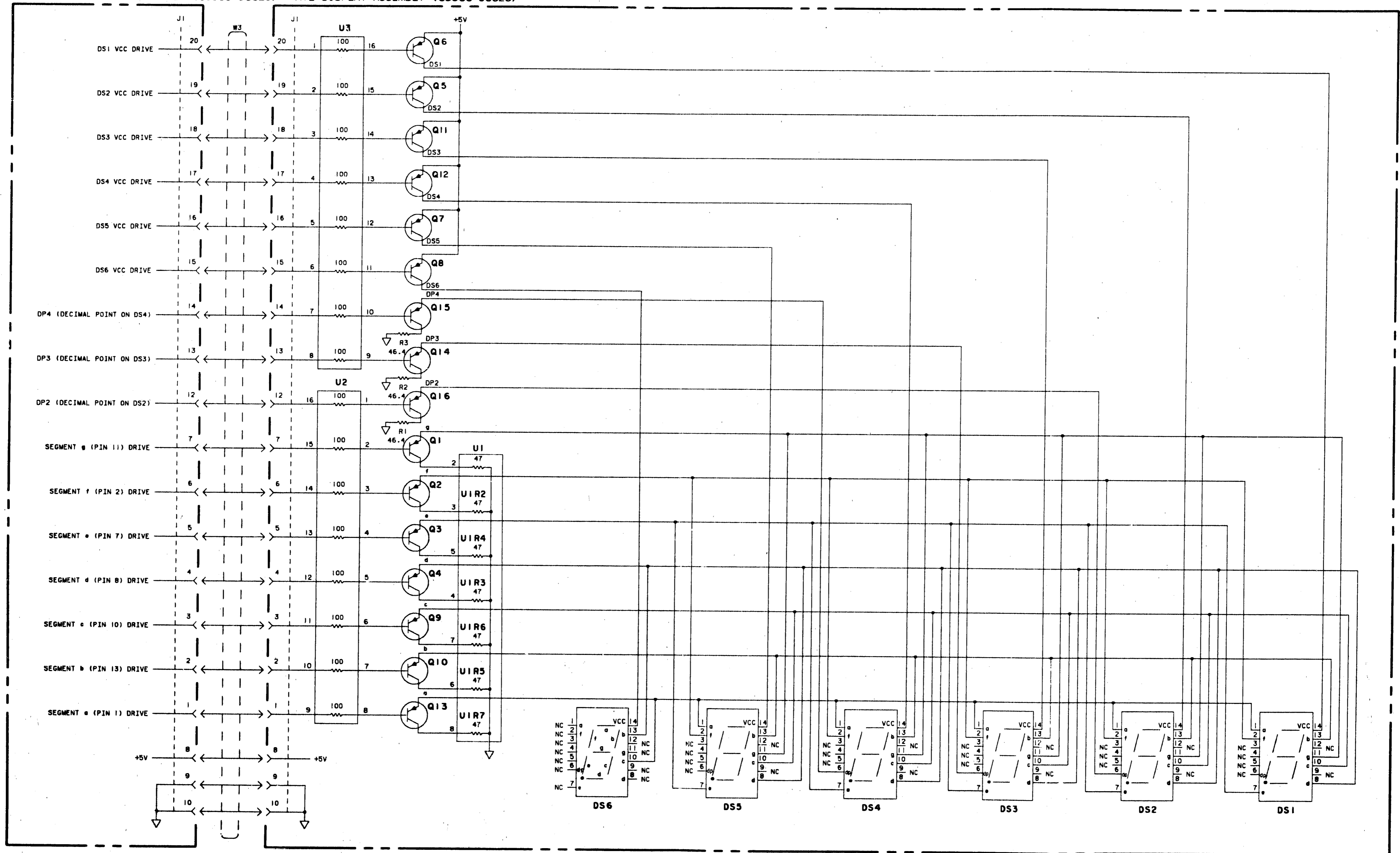
Figure 8-34B. A12 Display. Schematic (CHANGE 11)
