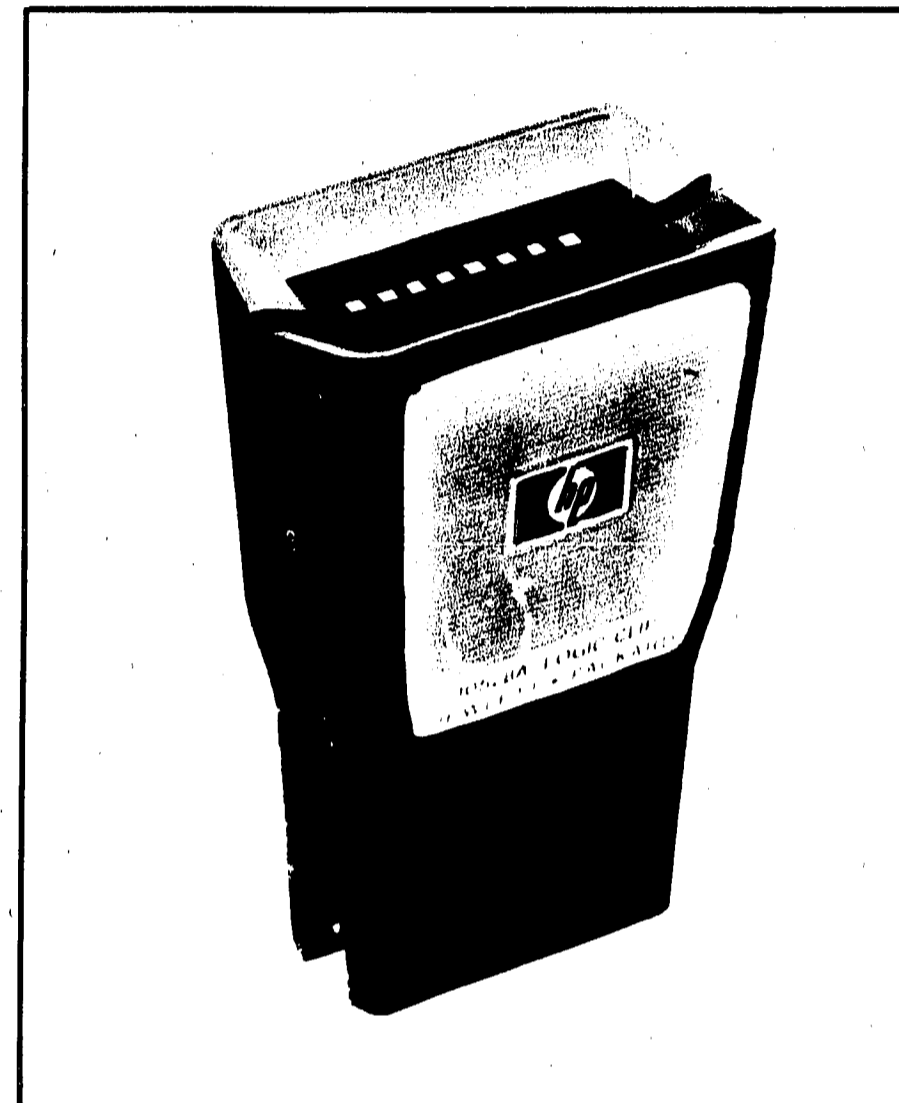
Figure 8-31. HP 10528A Logic Clip
