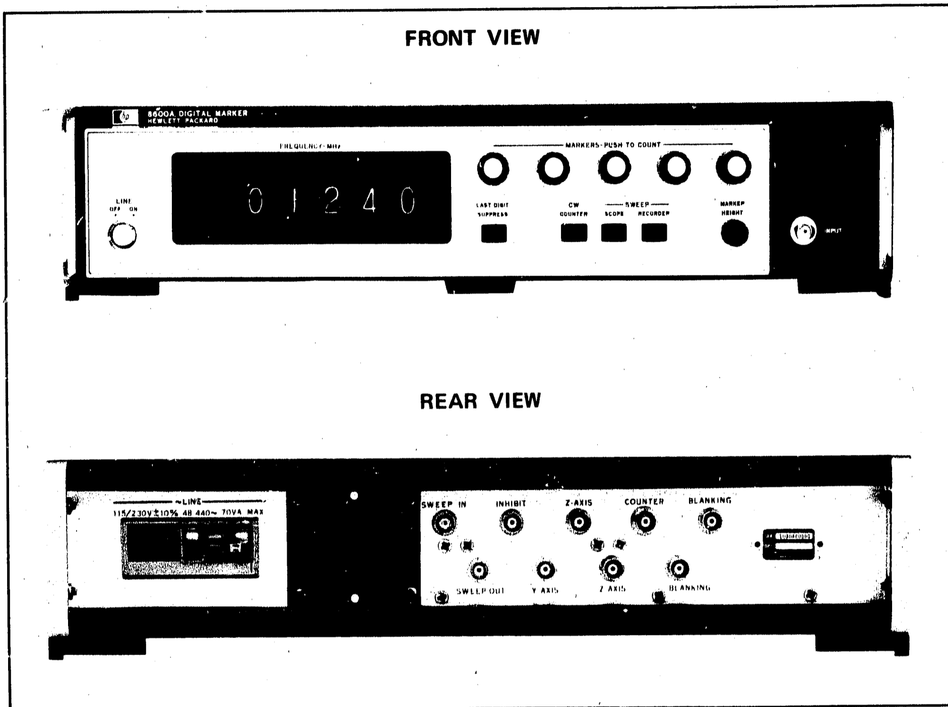
Figure 3-1. Digital Marker Controls, Connectors and Indicators
