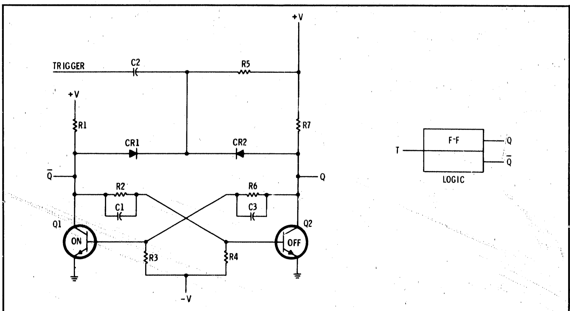
Figure 8-6. Triggered Flip-Flop
