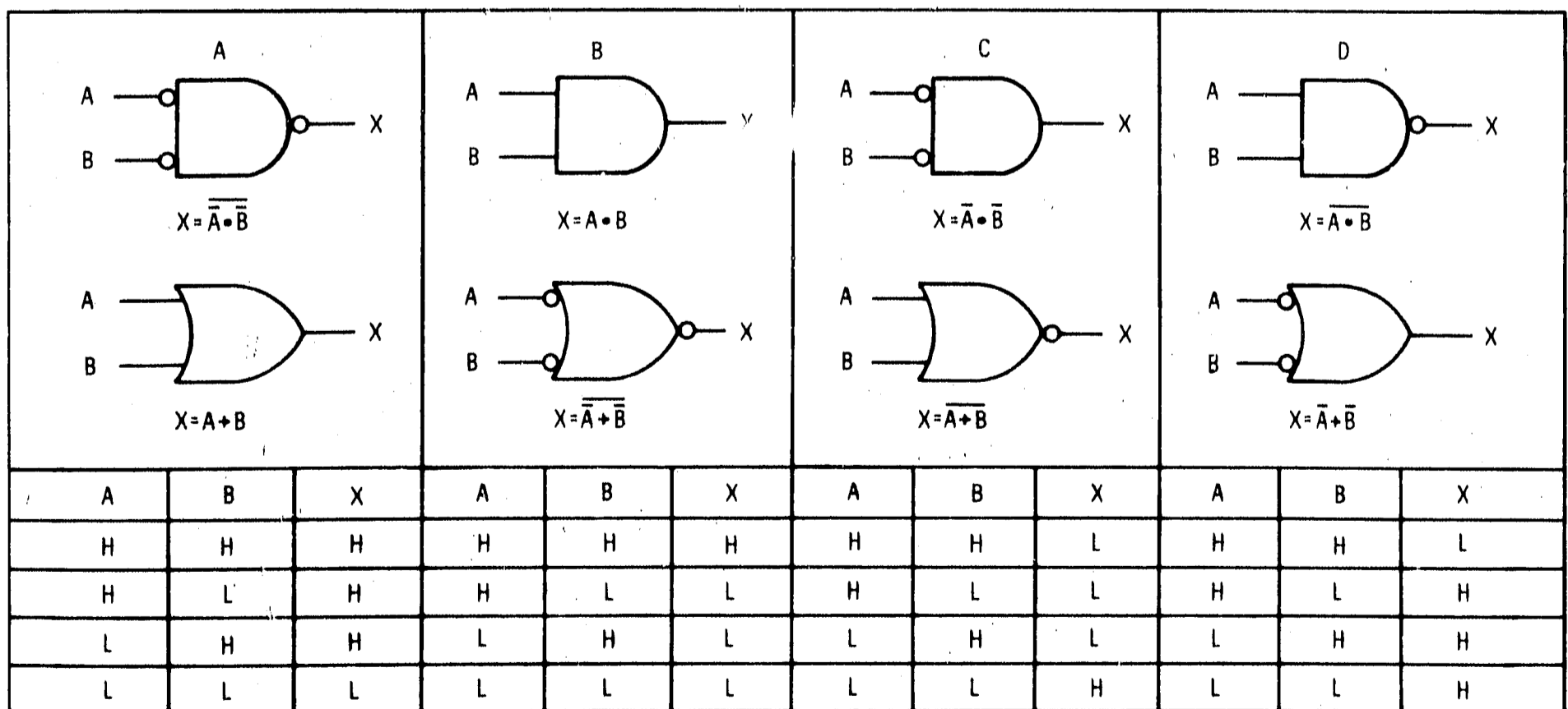
Figure 8-4. Logic Comparison Diagrams
