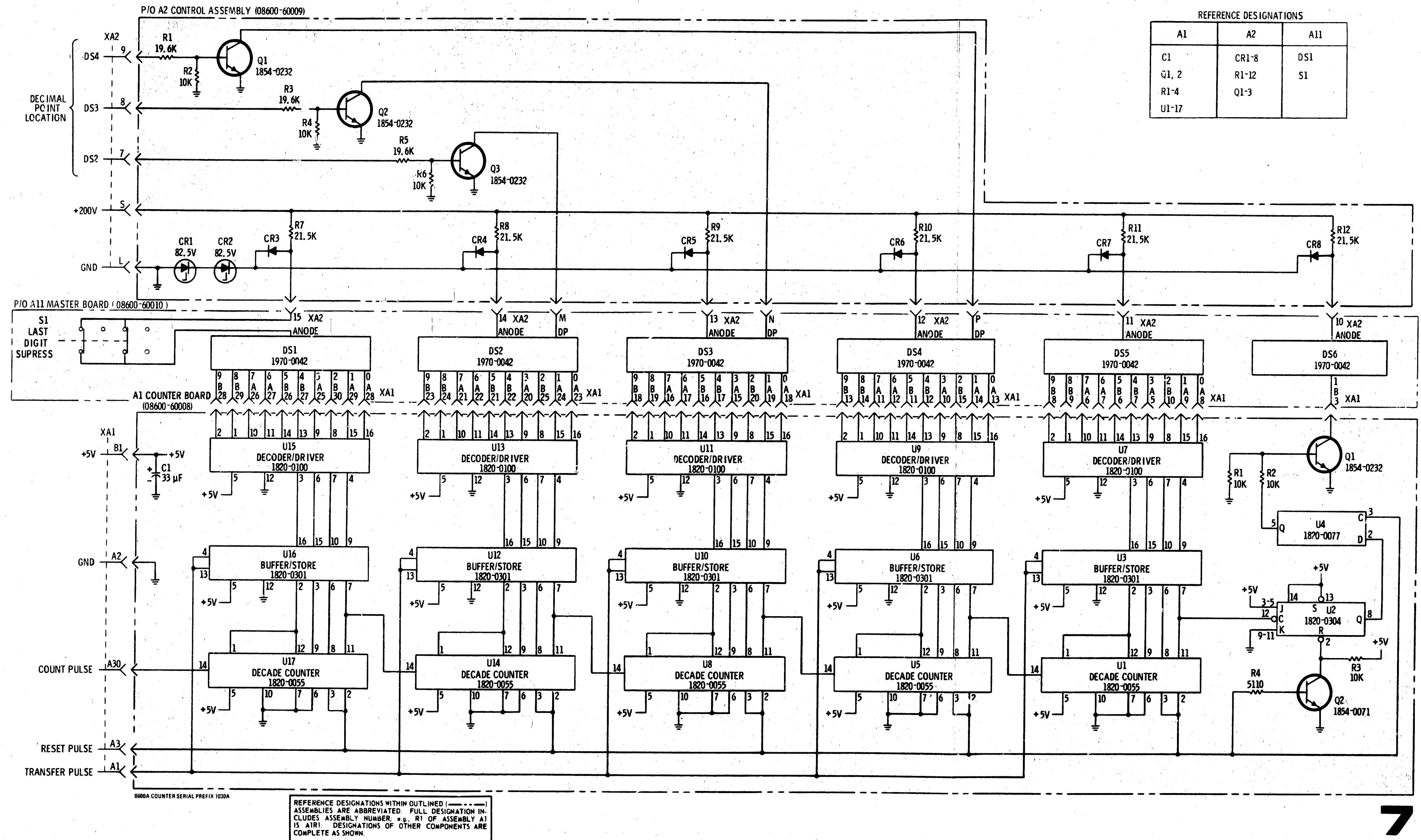
Figure 8-34. Counter and Decimal Control Schematic Diagram
