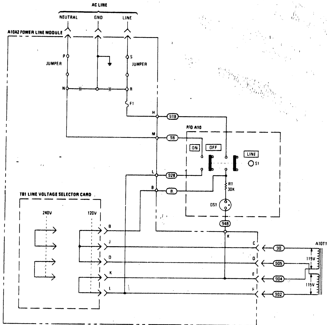
Figure 2. A10A2 Power Line Module (Change 7)
