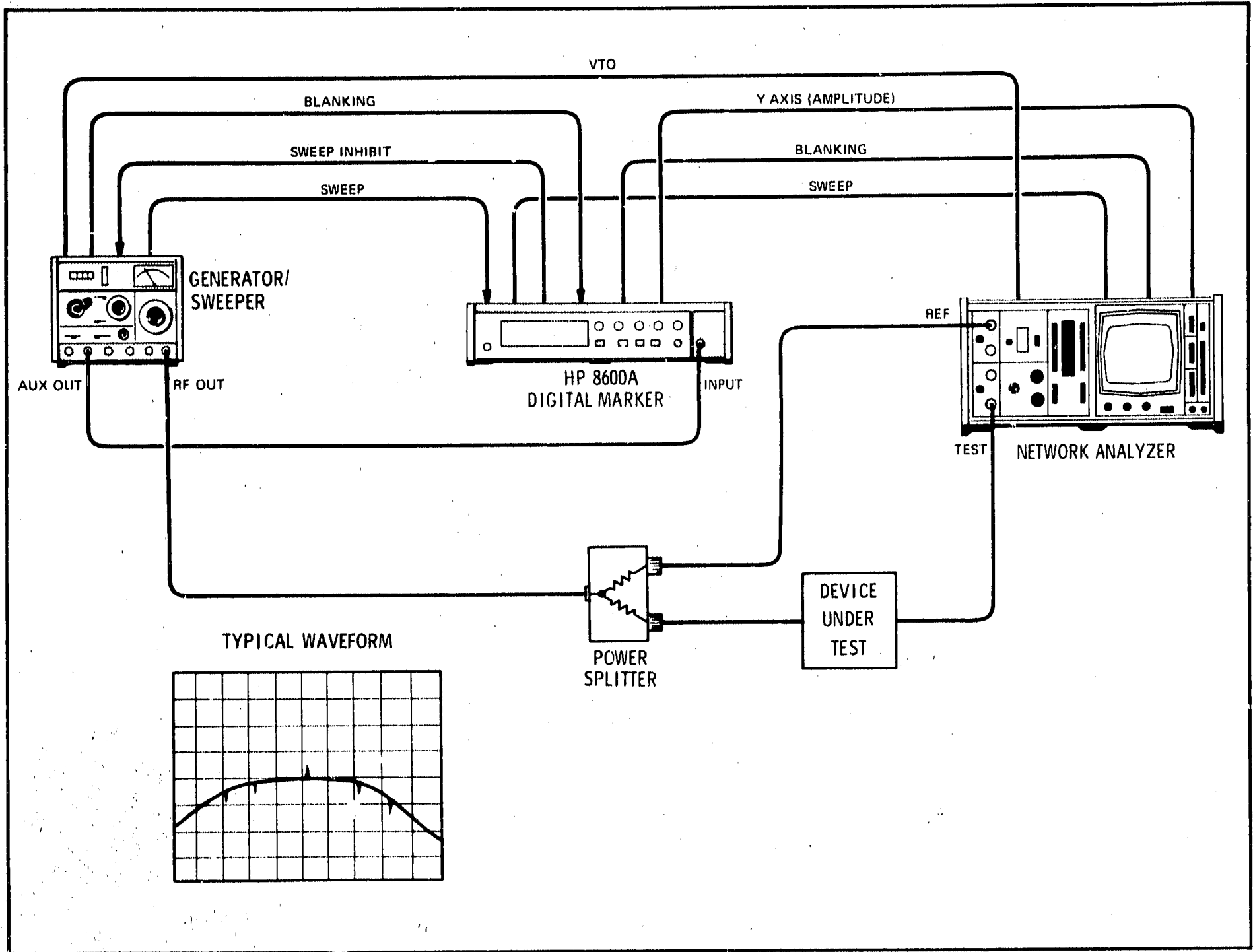
Figure 3-3. Network Analyzer Interconnections and Typical Waveform
