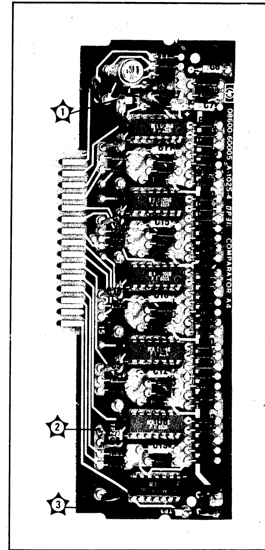
Figure 8-21. Comparator Assembly Component Locations
