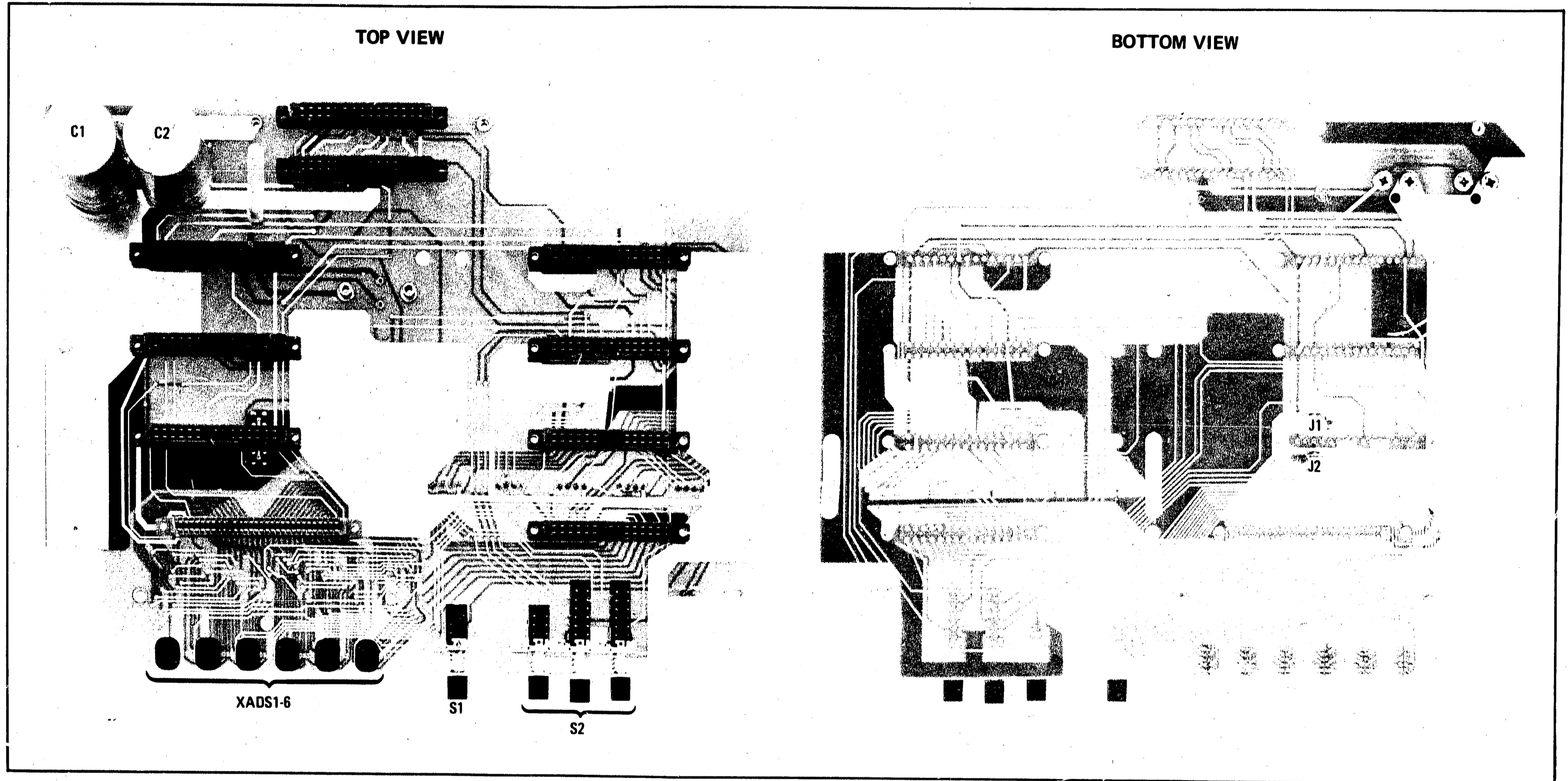
Figure 8-38. Mother Board
