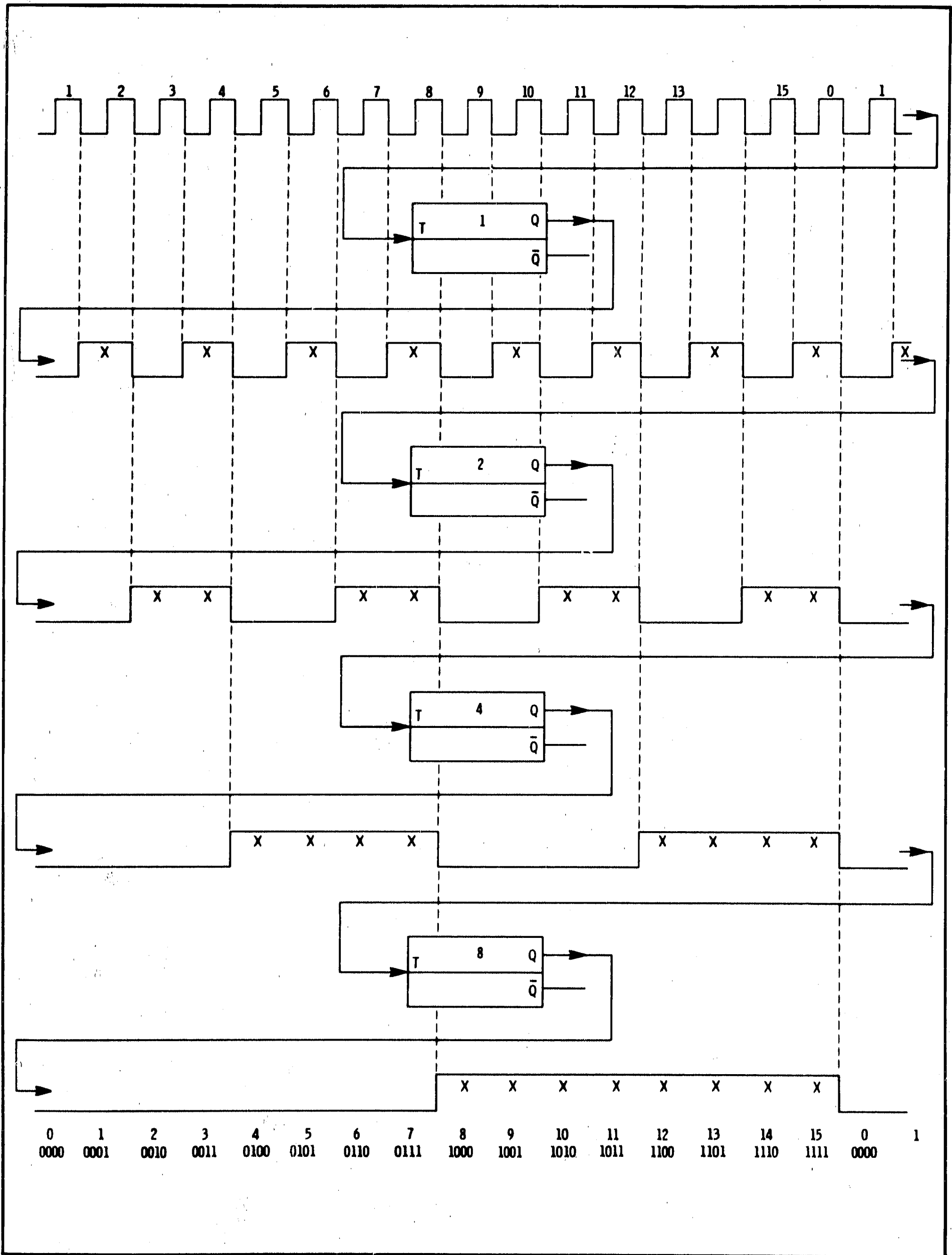
Figure 8-11. 16 Counter Binary Counter Chain
