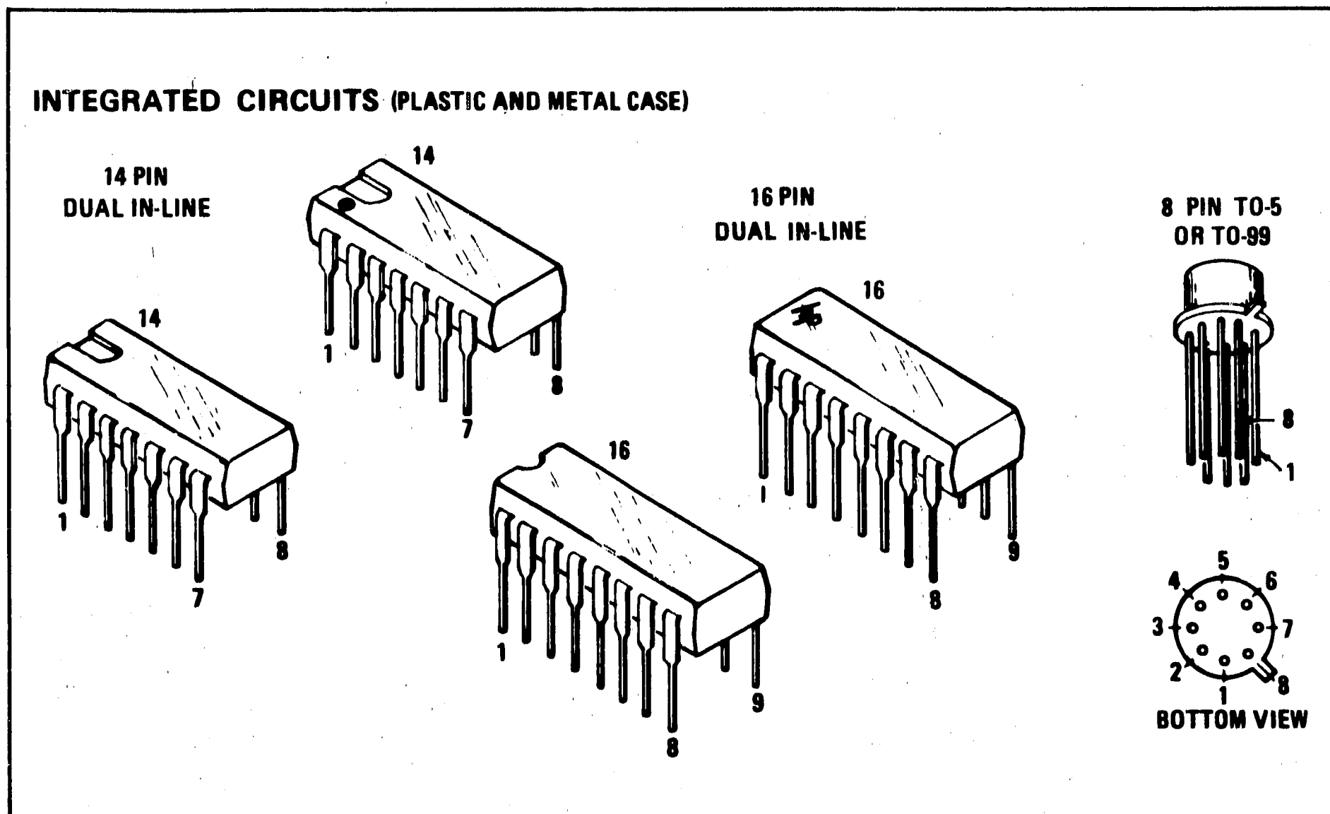
Figure 8-16. Integrated Circuit Packaging
