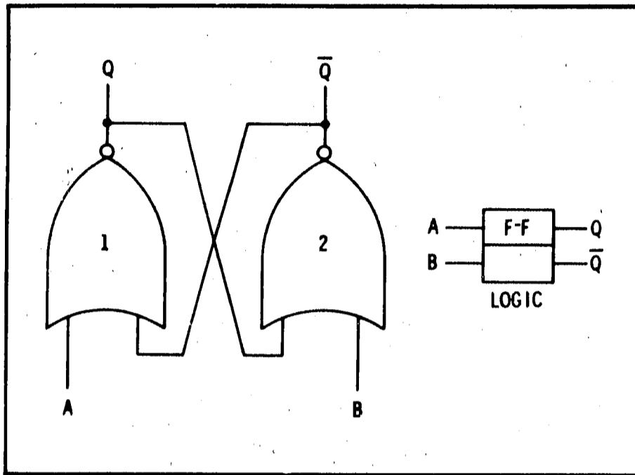
Figure 8-5. Basic NOR Gate Flip-Flop
