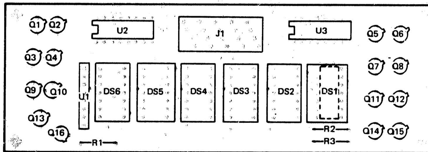
Figure 8-32A. A12 Display 08600-60028 Component Location (CHANGE 11)
