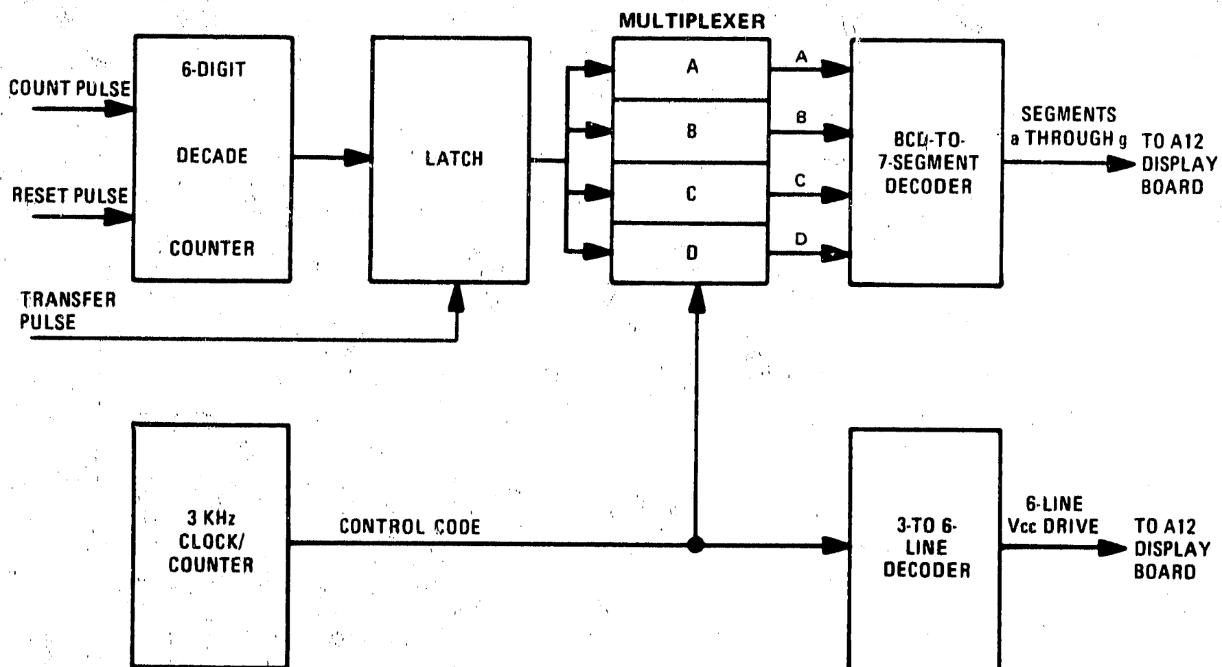
Figure 8-31A. A1 Counter/Driver 08600-60026, Simplified Block Diagram (CHANGE 11)
