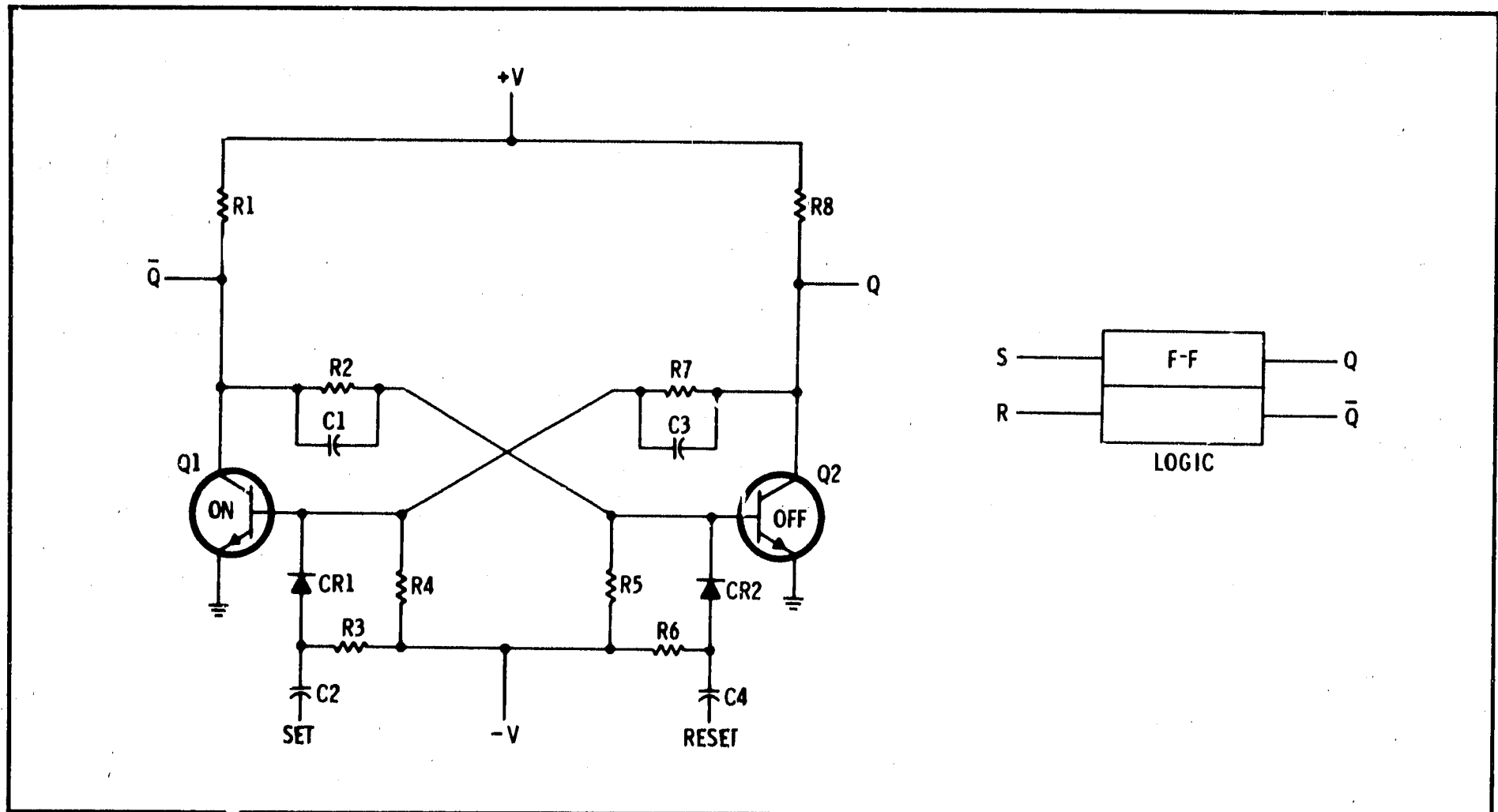
Figure 8-7. RS Flip-Flop
