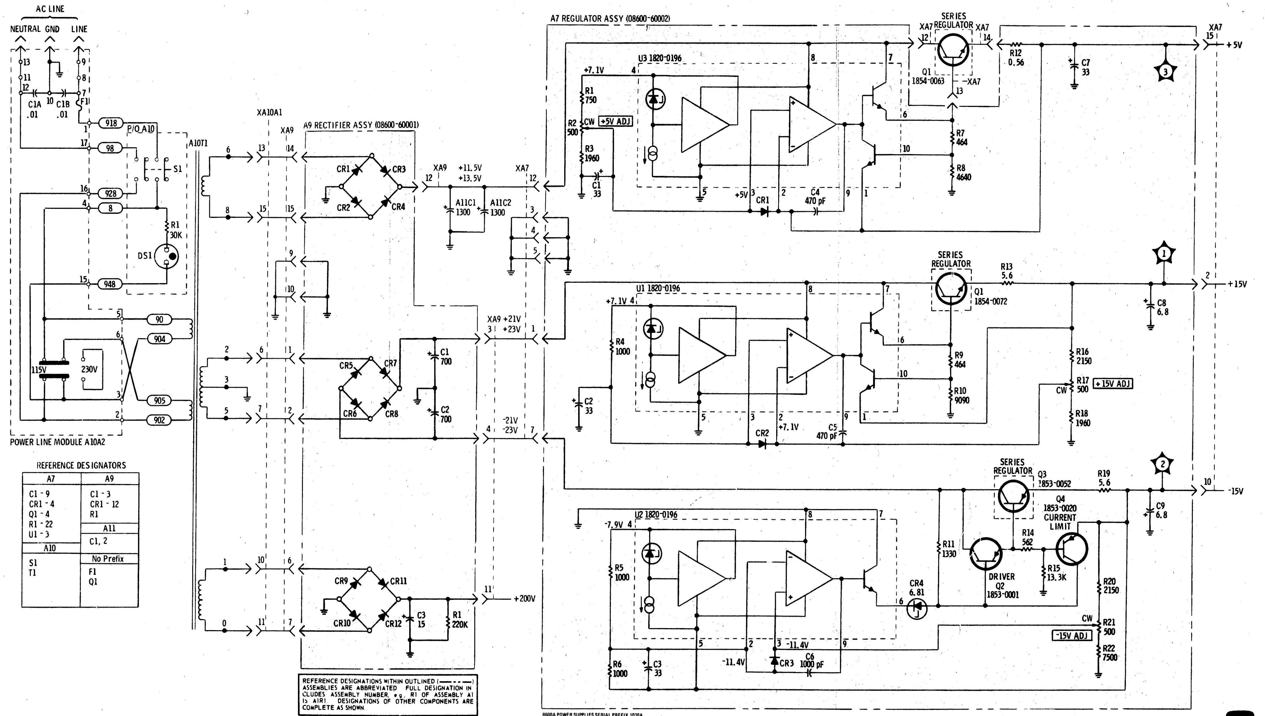
Figure 8-37. Rectifier and Regulator Schematic Diagram
