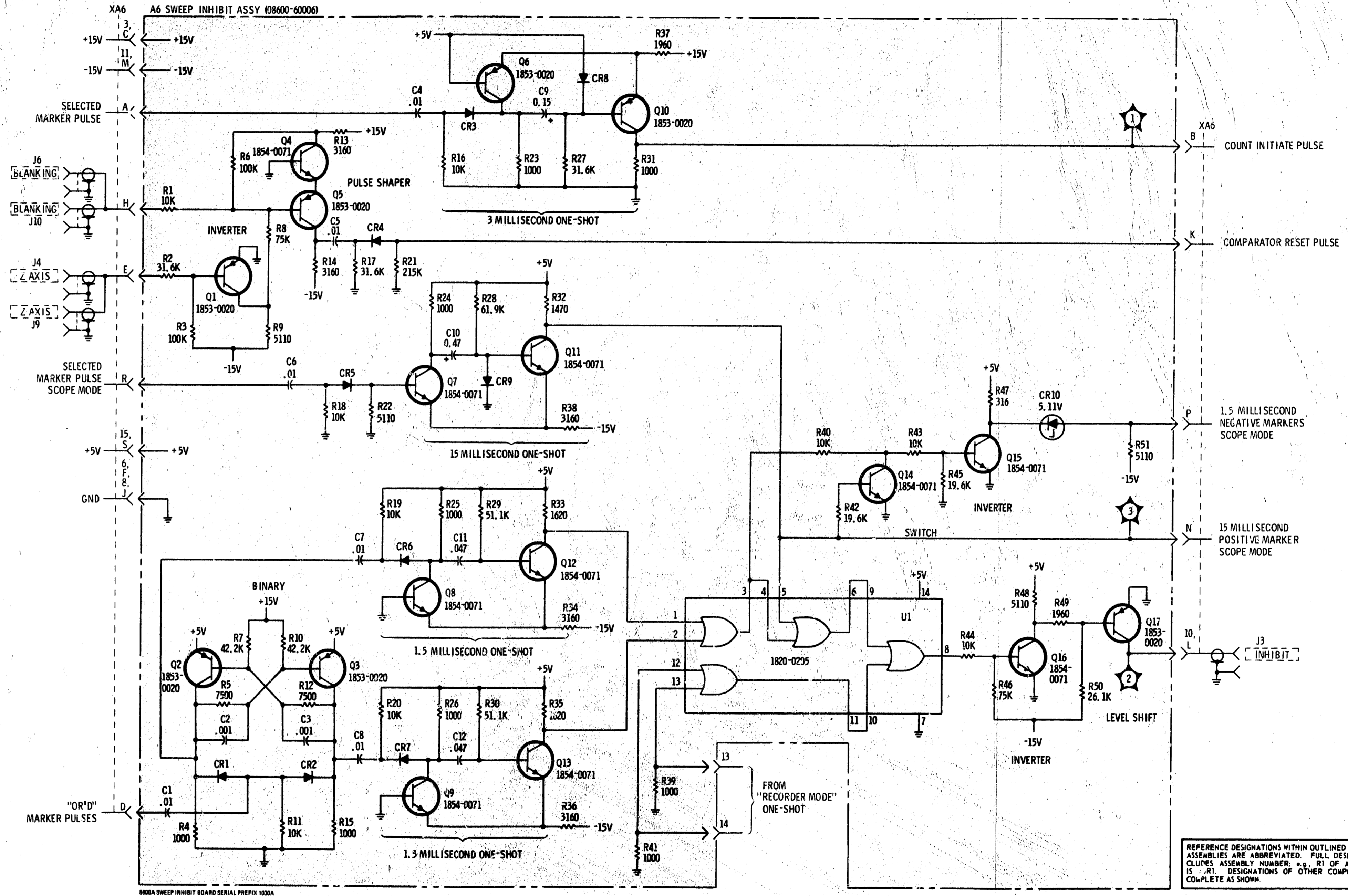
Figure 8-24. Sweep Inhibit Schematic Diagram
