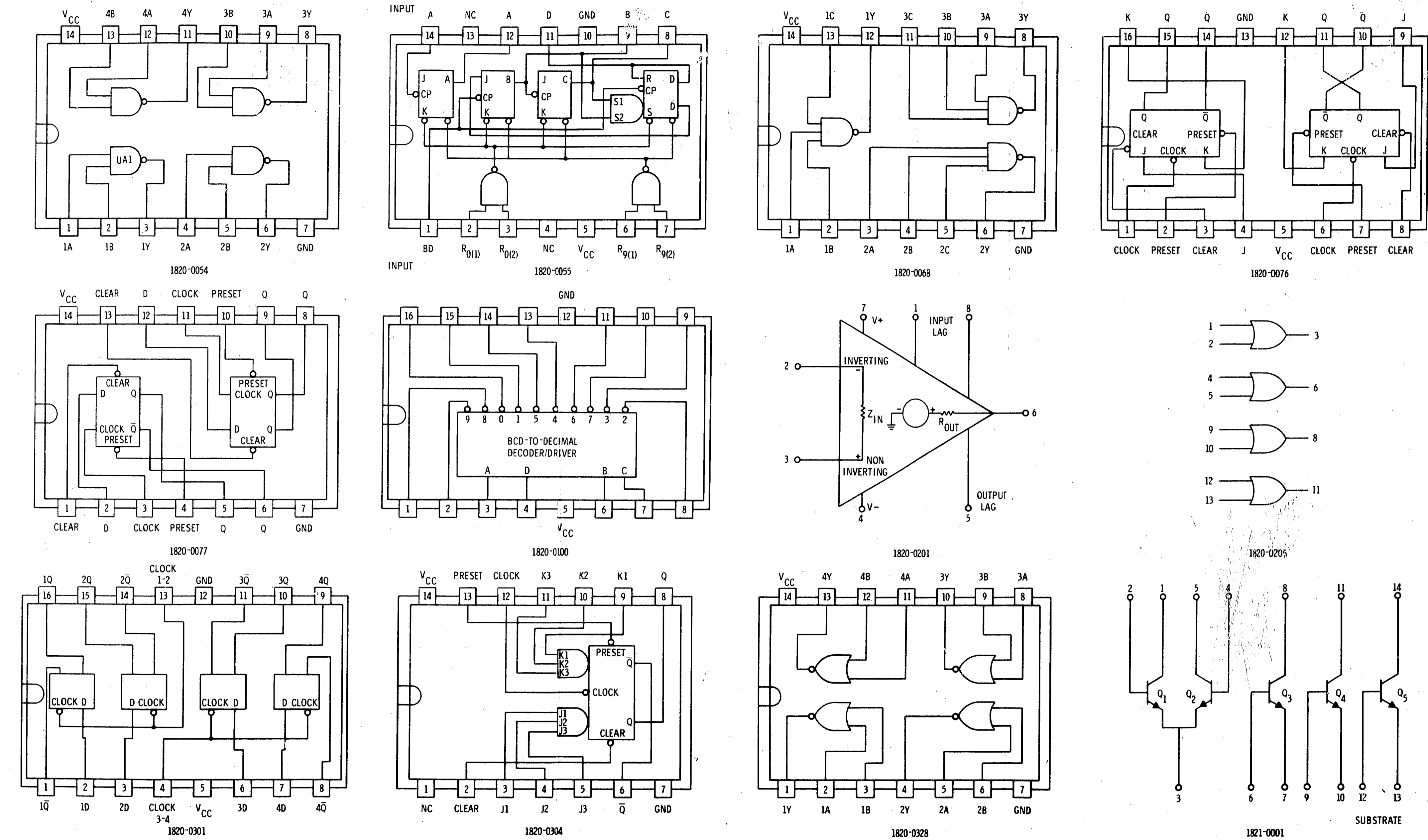
Figure 8-18. Integrated Circuits Used in the Model 8600A Internal Logic
