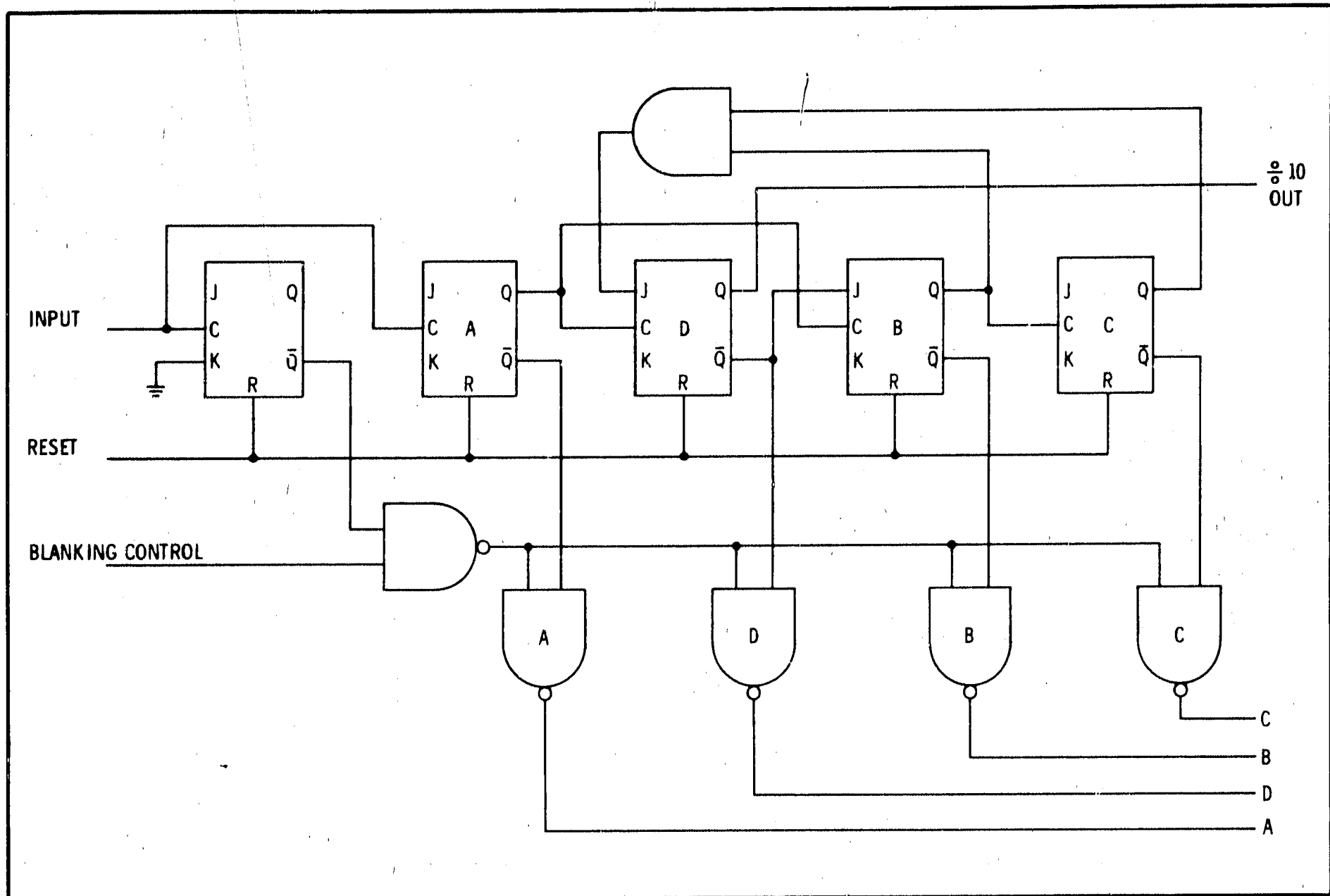
Figure 8-13. Blanking Decade Counter
