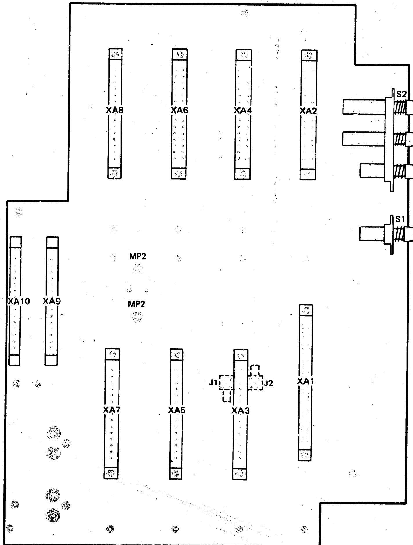
Figure 8-38. Mother Board 08600-60027 (Change 11)
