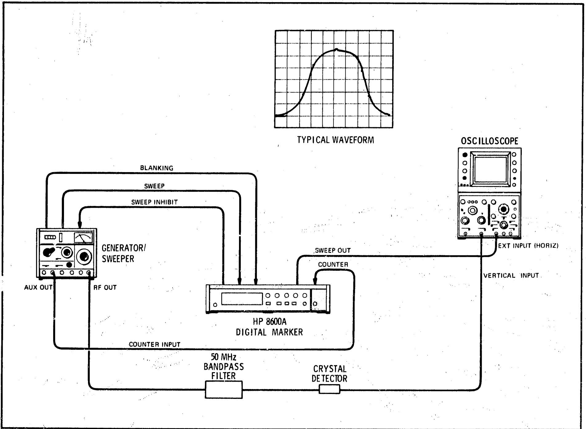
Figure 3-2. Oscilloscope Interconnections and Typical Waveform
