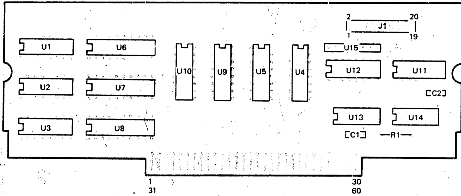
Figure 8-32. A1 Counter/Driver 08600-60026 Component Location (CHANGE 11)
