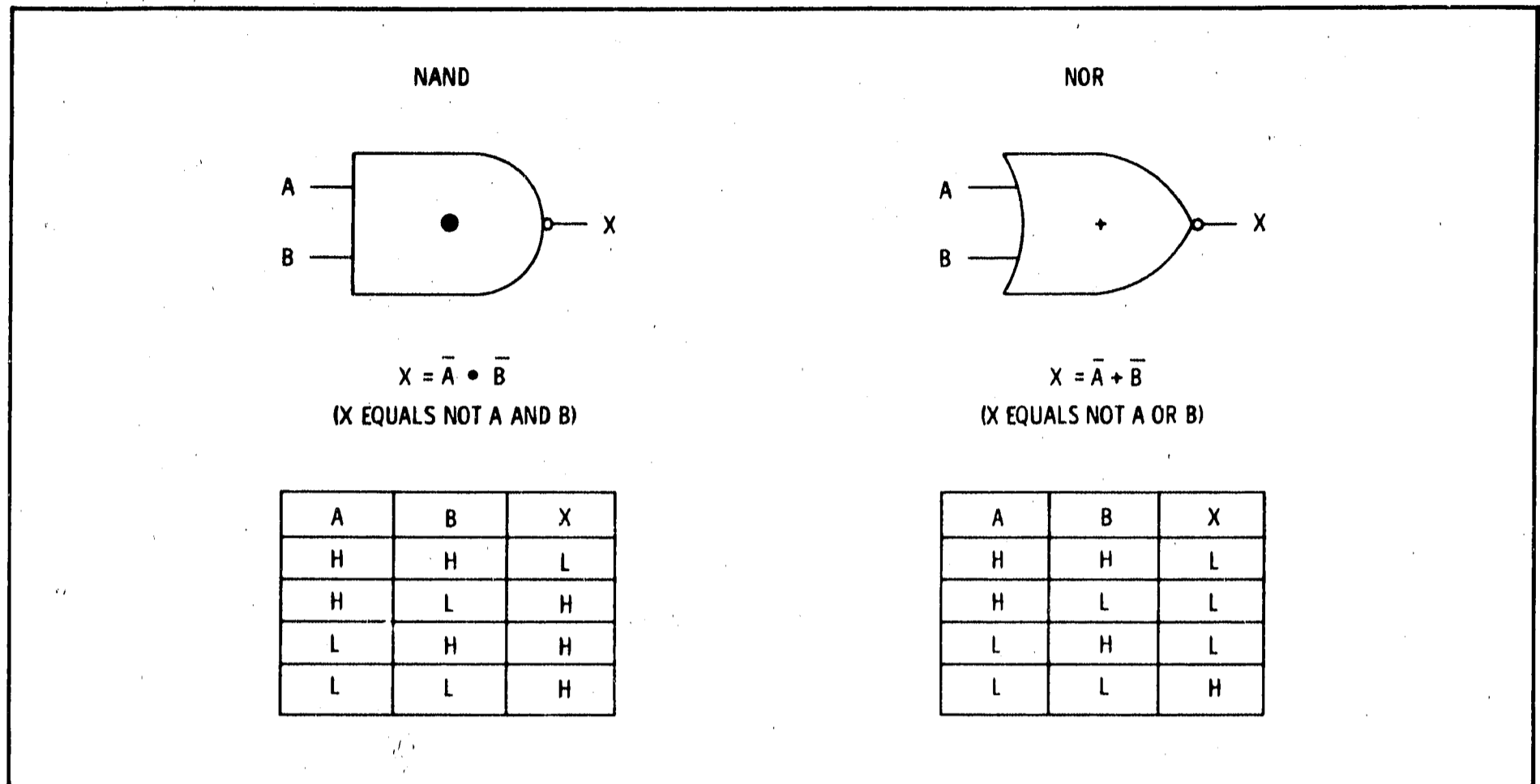
Figure 8-3. Basic NAND and NOR Gates
