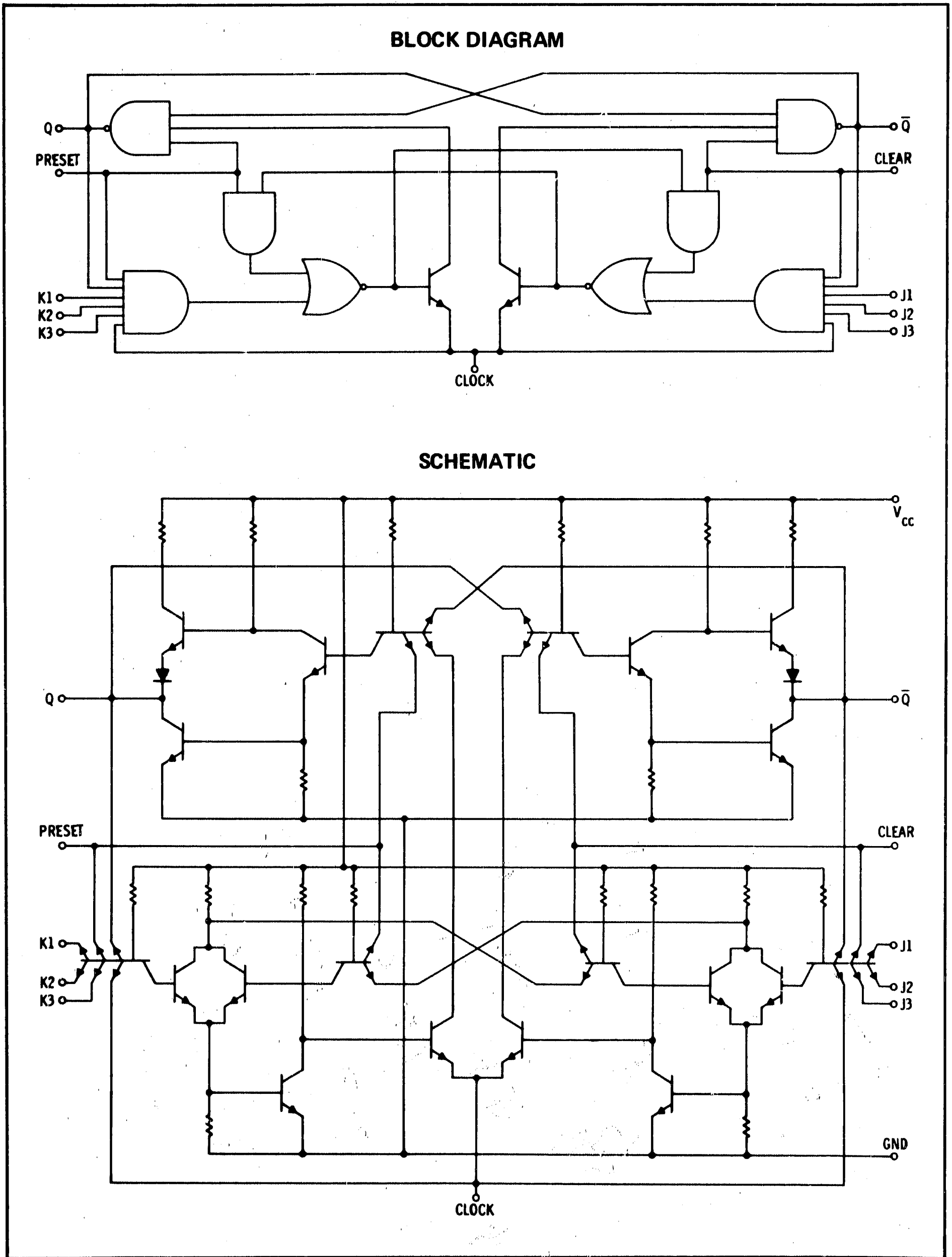
Figure 8-10. JK Master-Slave Flip-Flop
