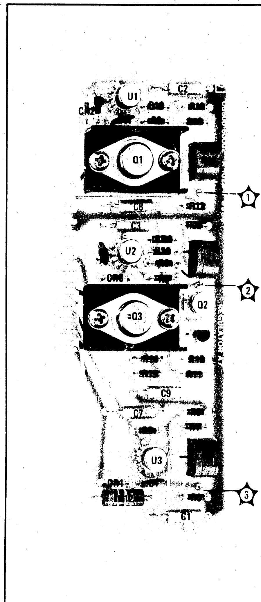
Figure 8-36. Regulator Assembly Component Locations
