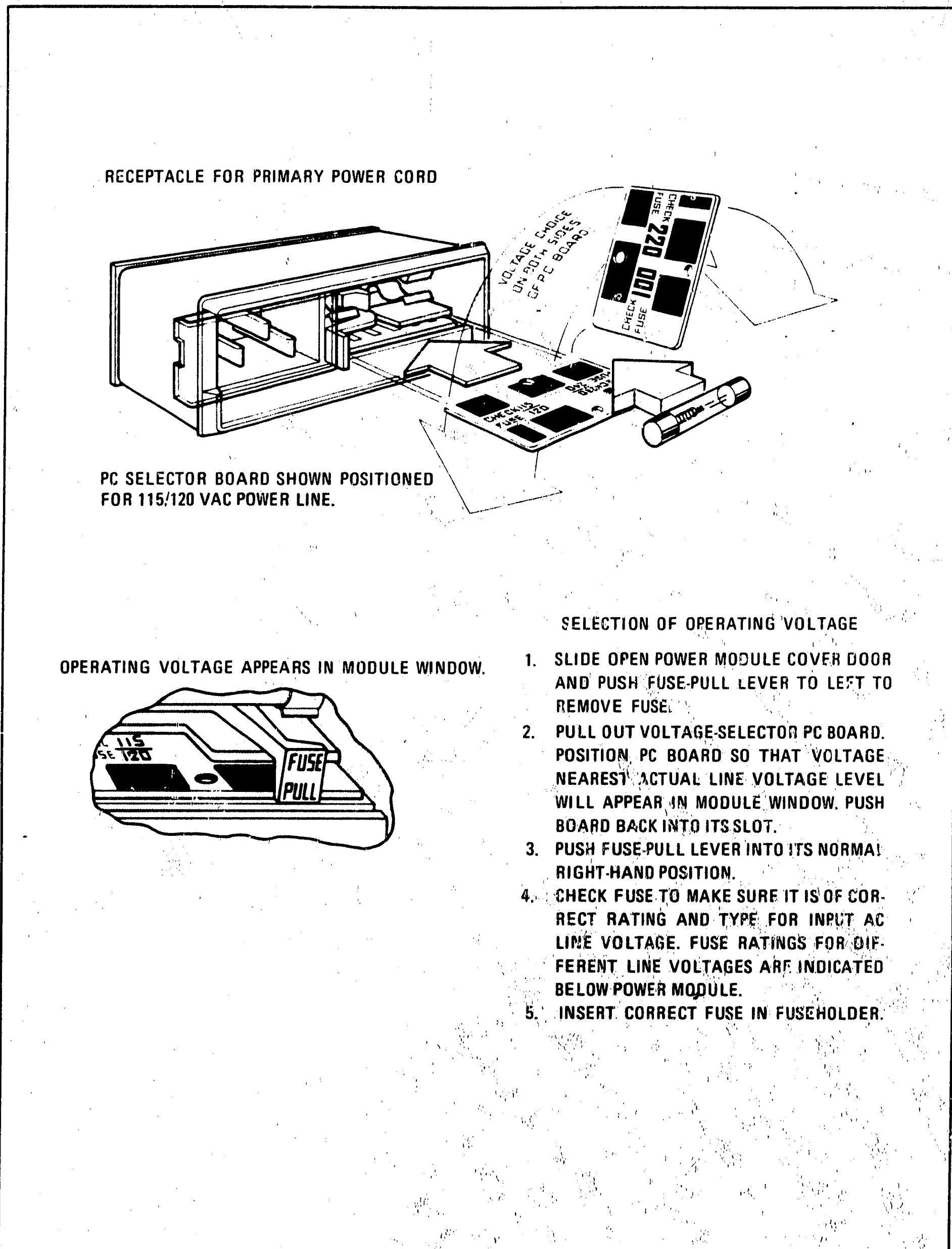
Figure 2-1. Line Voltage Selection with Power Module PC Board (CHANGE 7)
