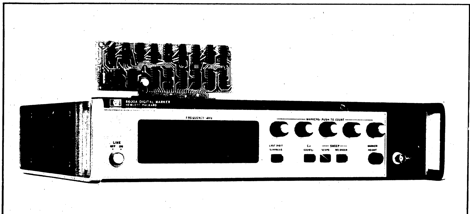
Figure 8-1. Model 8600A with Circuit Board Extended for Maintenance
