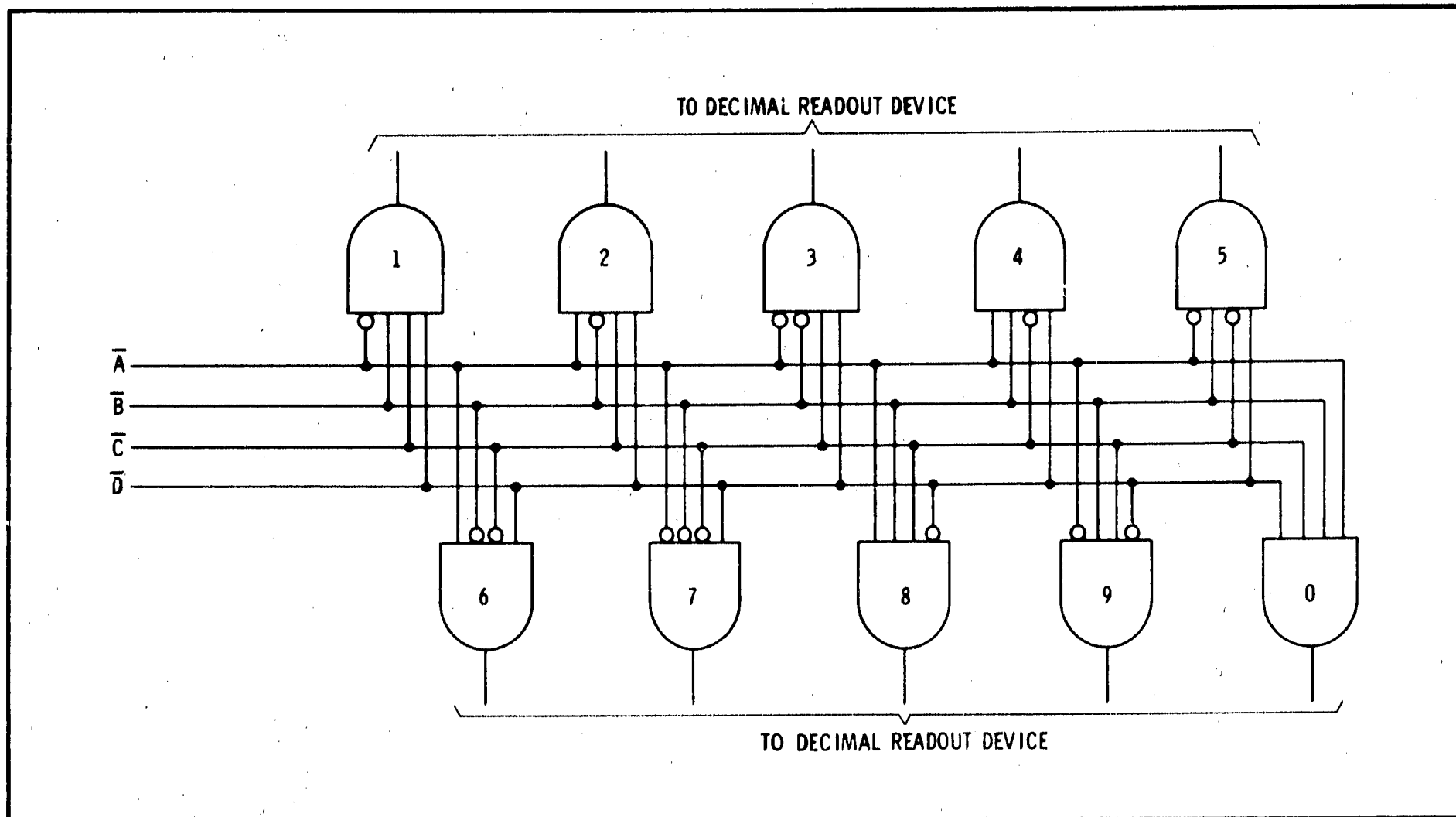
Figure 8-15. Decoder
