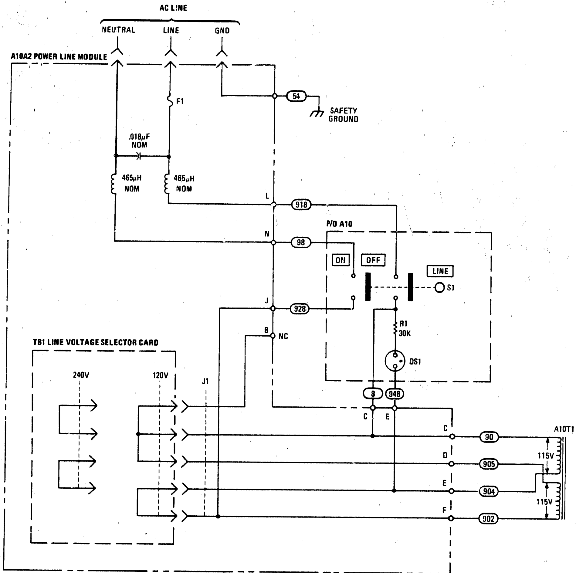
Figure 3. A10A2 Power Line Module (CHANGE 9)
