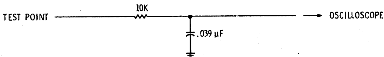
Figure 5-1. 400 Hz Low Pass Filter, Schematic
