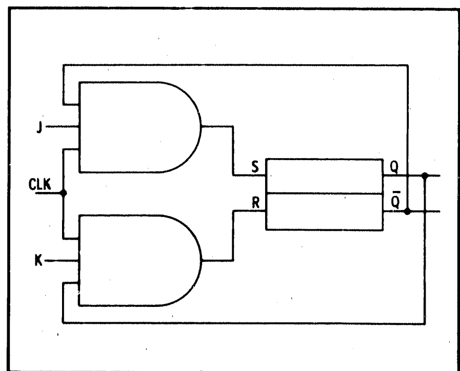
Figure 8-9. Clocked JK Flip-Flop
