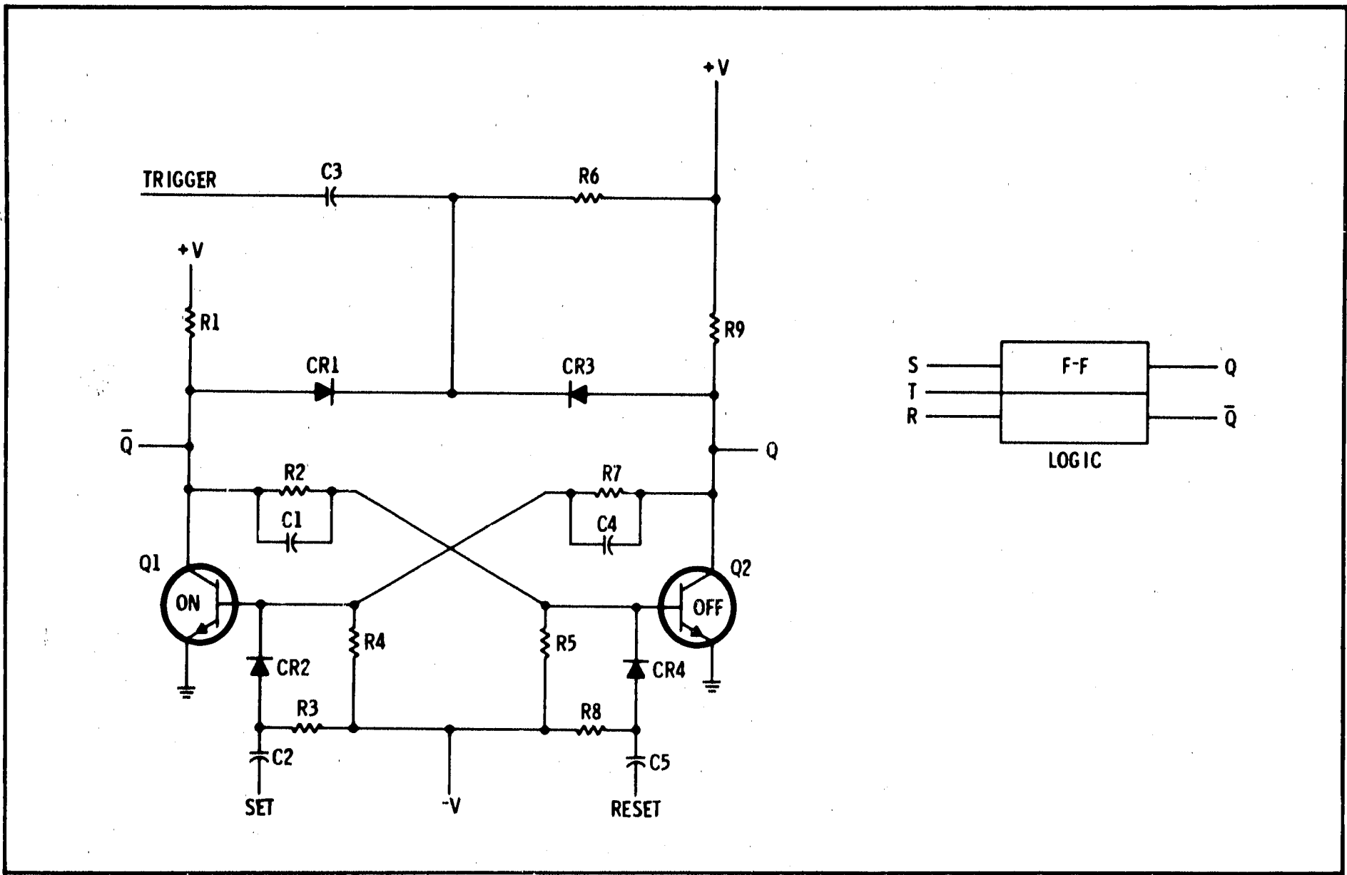
Figure 8-8. RST Flip-Flop
