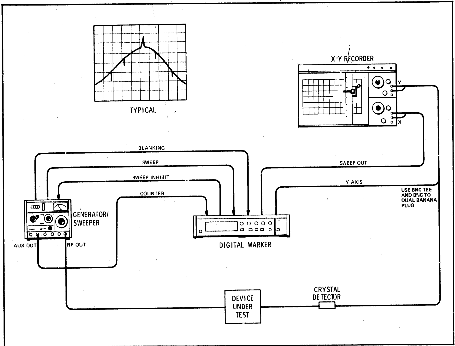
Figure 3-4. X-Y Recorder Interconnections and Typical Display
