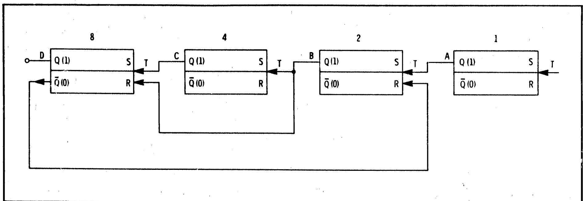
Figure 8-12. 8421 BCD Decade Counter
