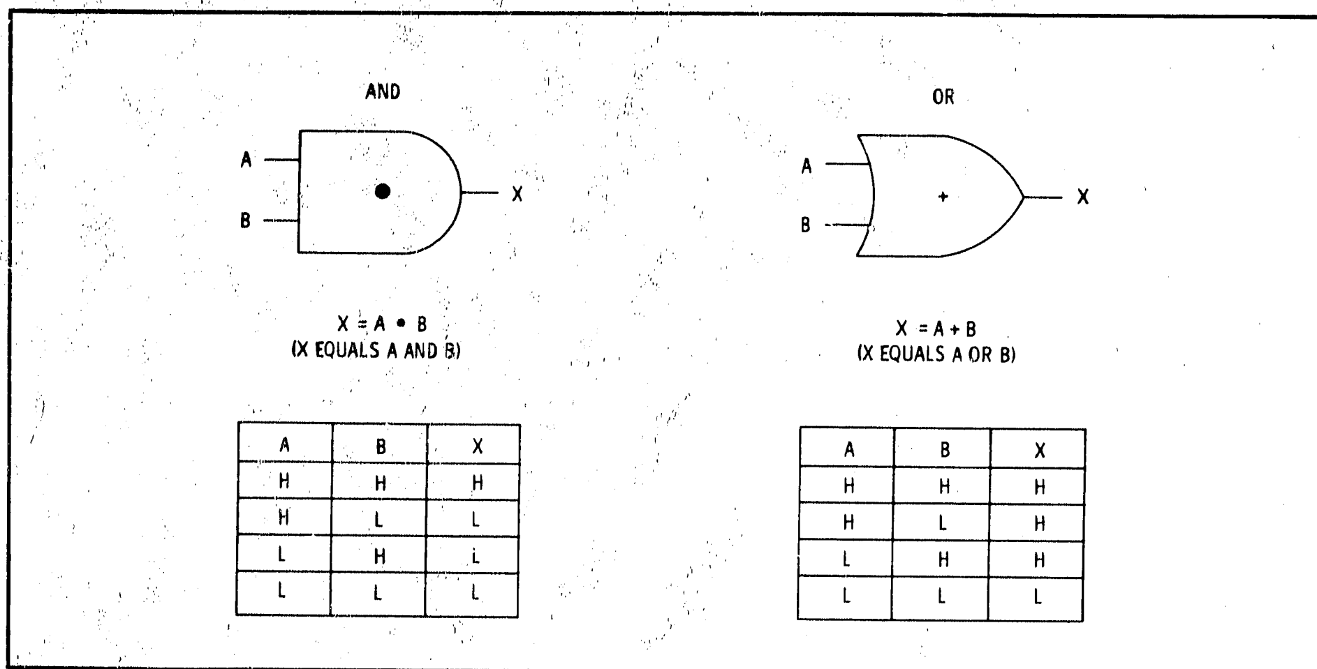
Figure 8-2. Basic AND and OR Gates
