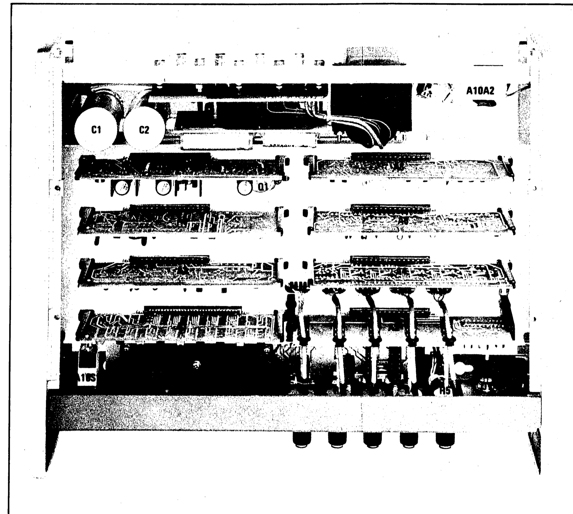
Figure 8-17. Chassis Mounted Parts and Assemblies Locations
