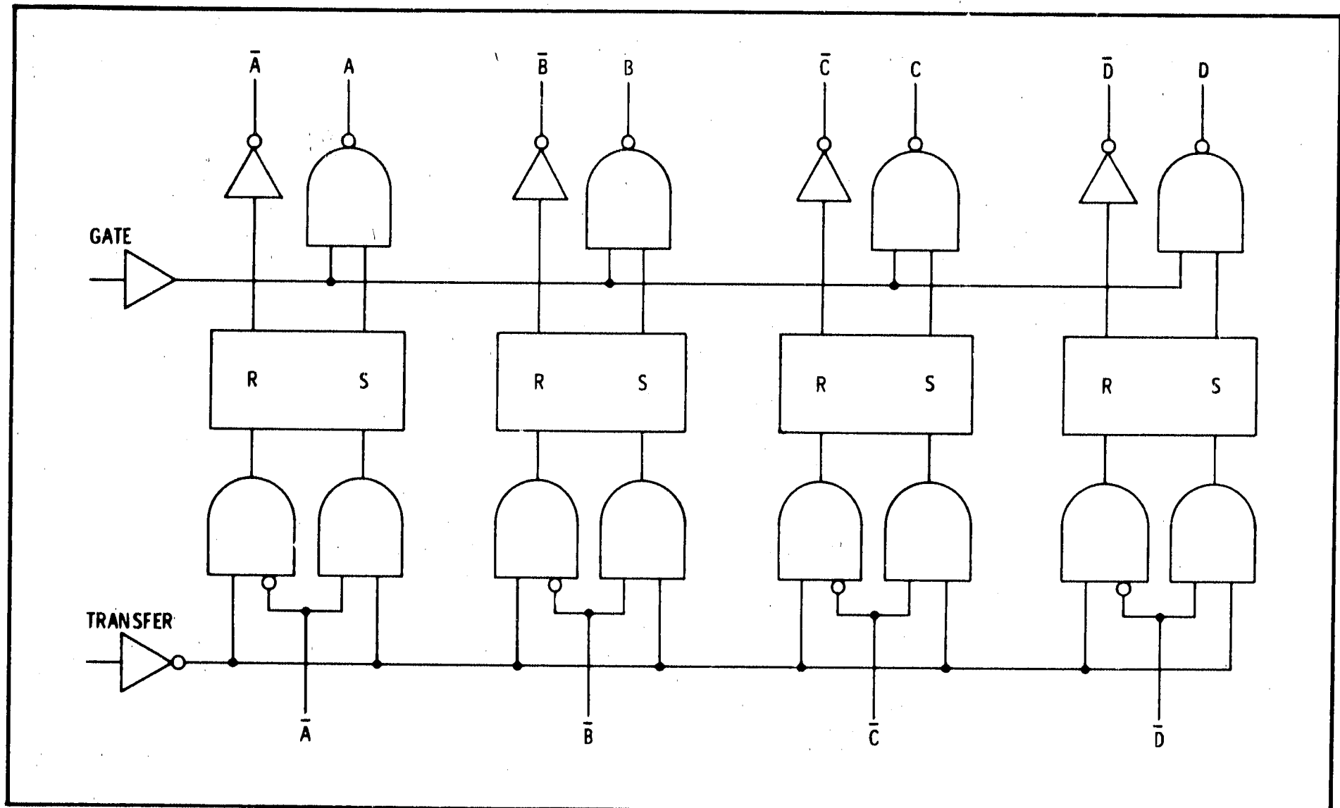
Figure 8-14. Buffer/Store
