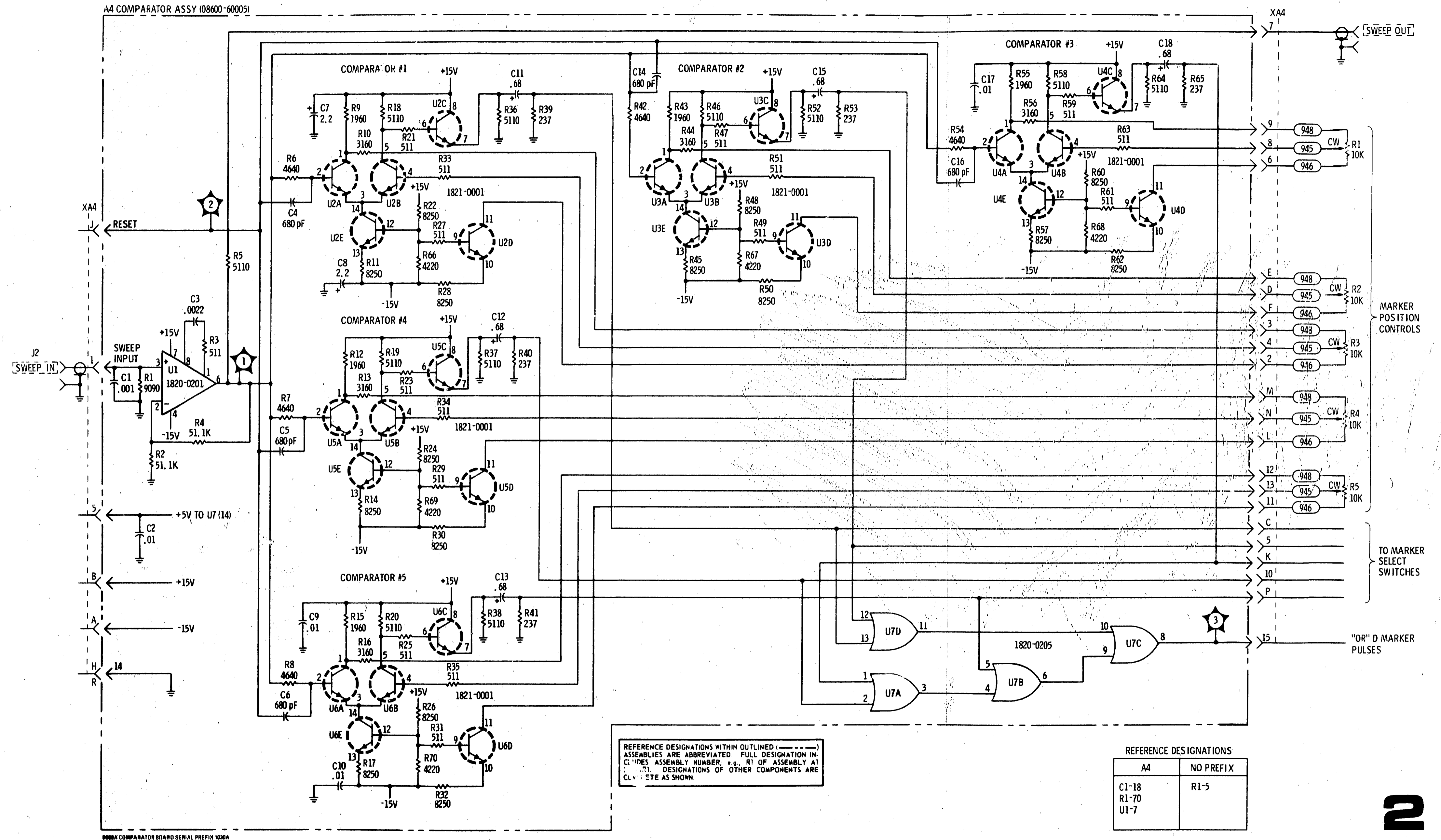
Figure 8-22. Comparator Schematic Diagram
