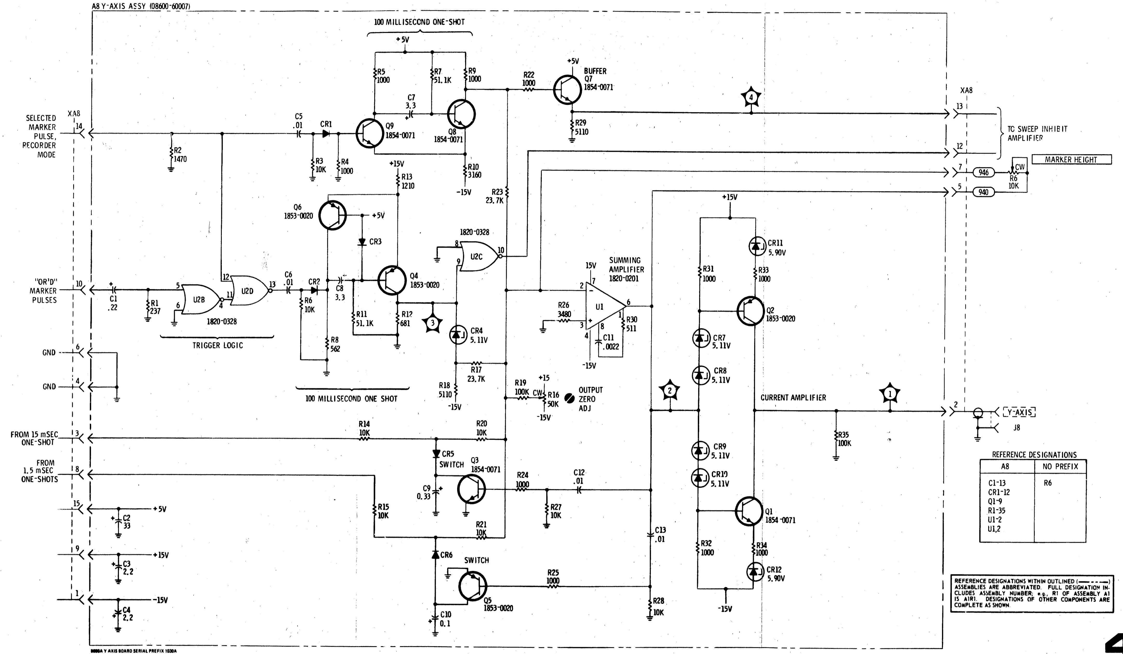
Figure 8-26. Y-Axis Schematic Diagram
