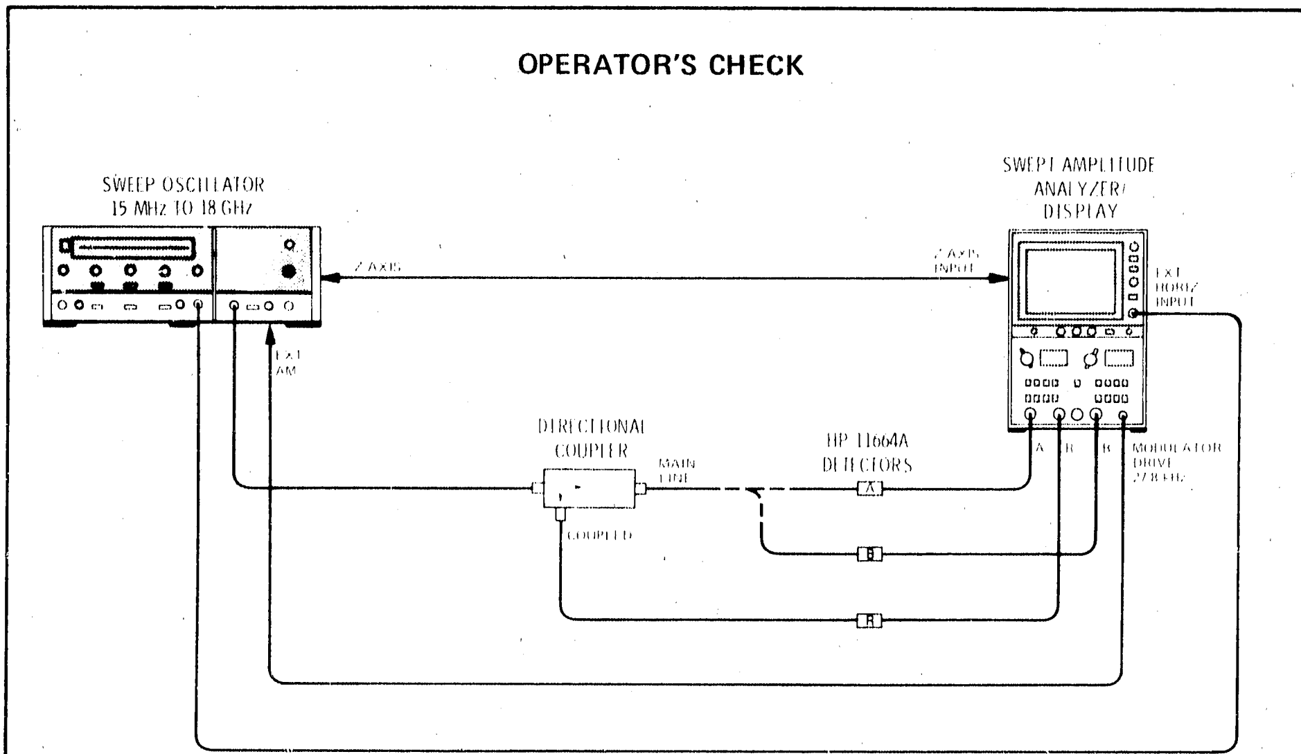
Operator's Check Test Setup
