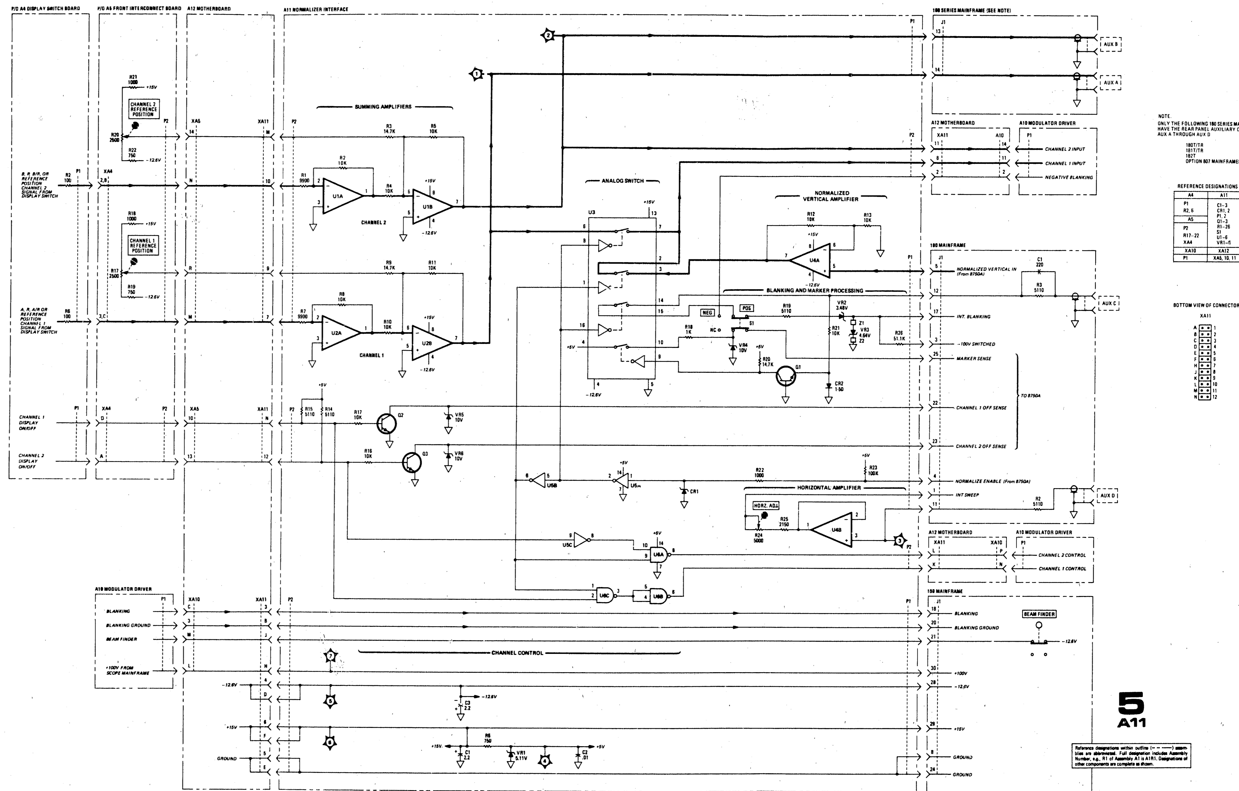
Figure 8-27. A11 Normalizer Interface, Schematic
