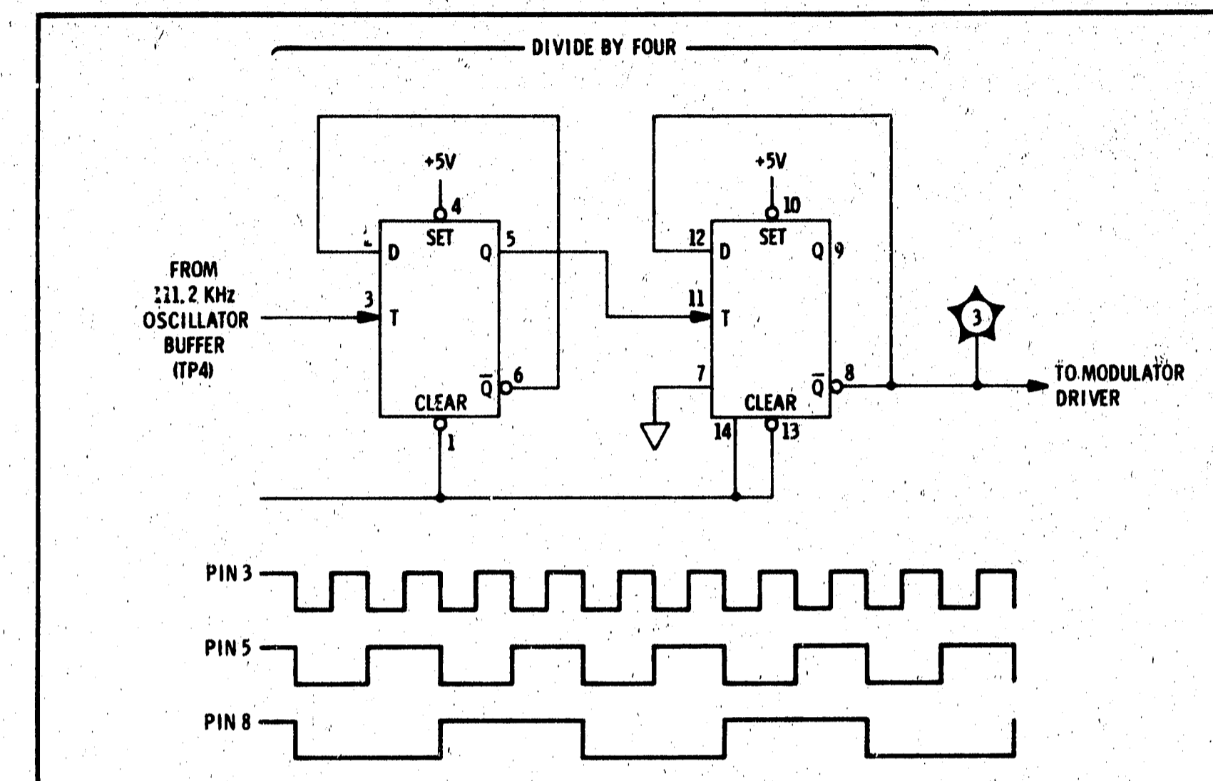
Figure 8-20. Dual "D" Flip-Flop
