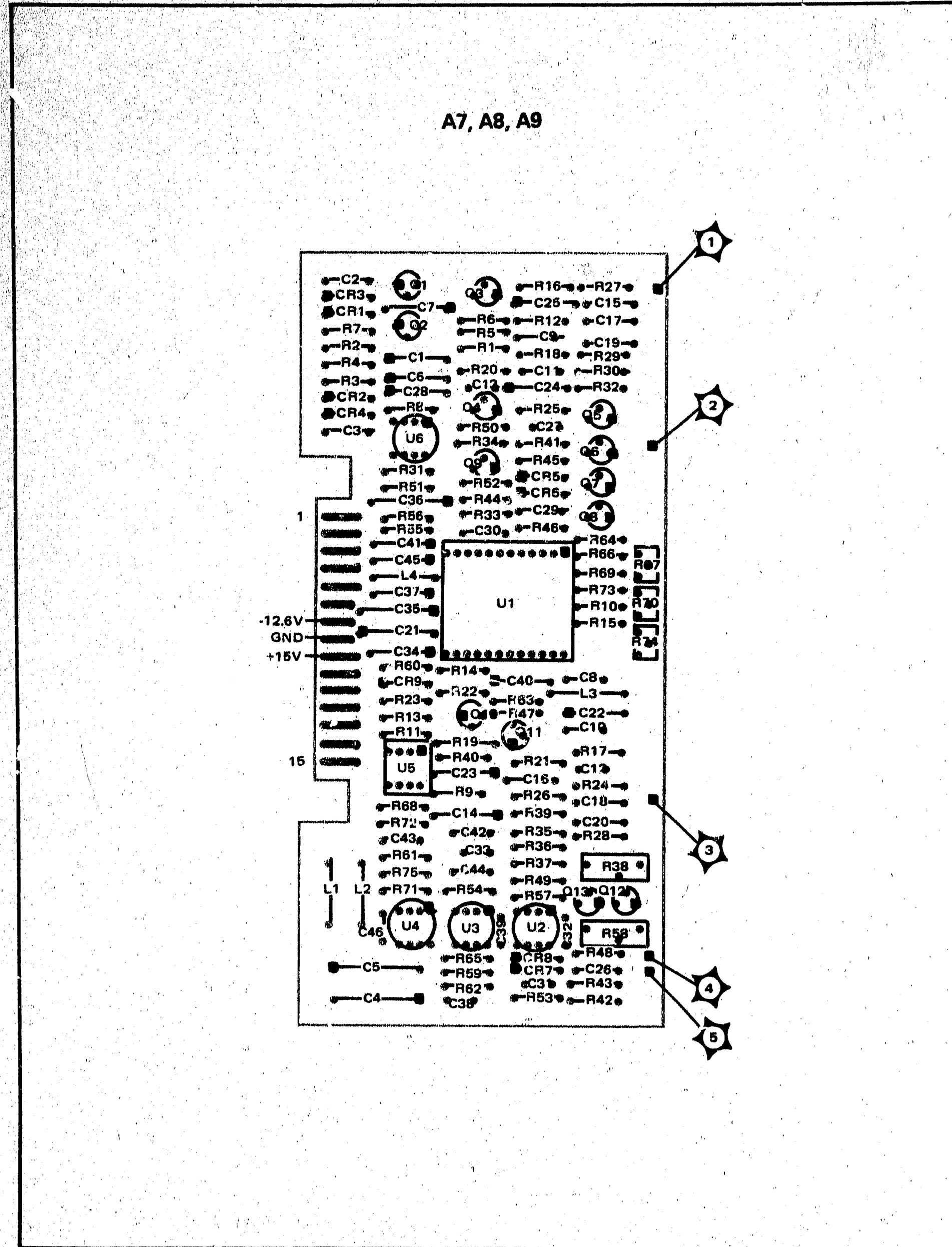
Figure 8-10. A7, A8, and A9 27.8 kHz Log Amplifier Parts Identification
