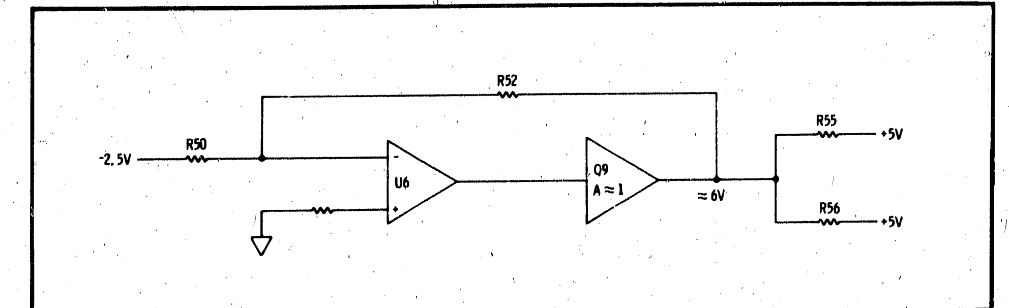
Figure 8-8 -2.5V Supply Simplified Diagram
