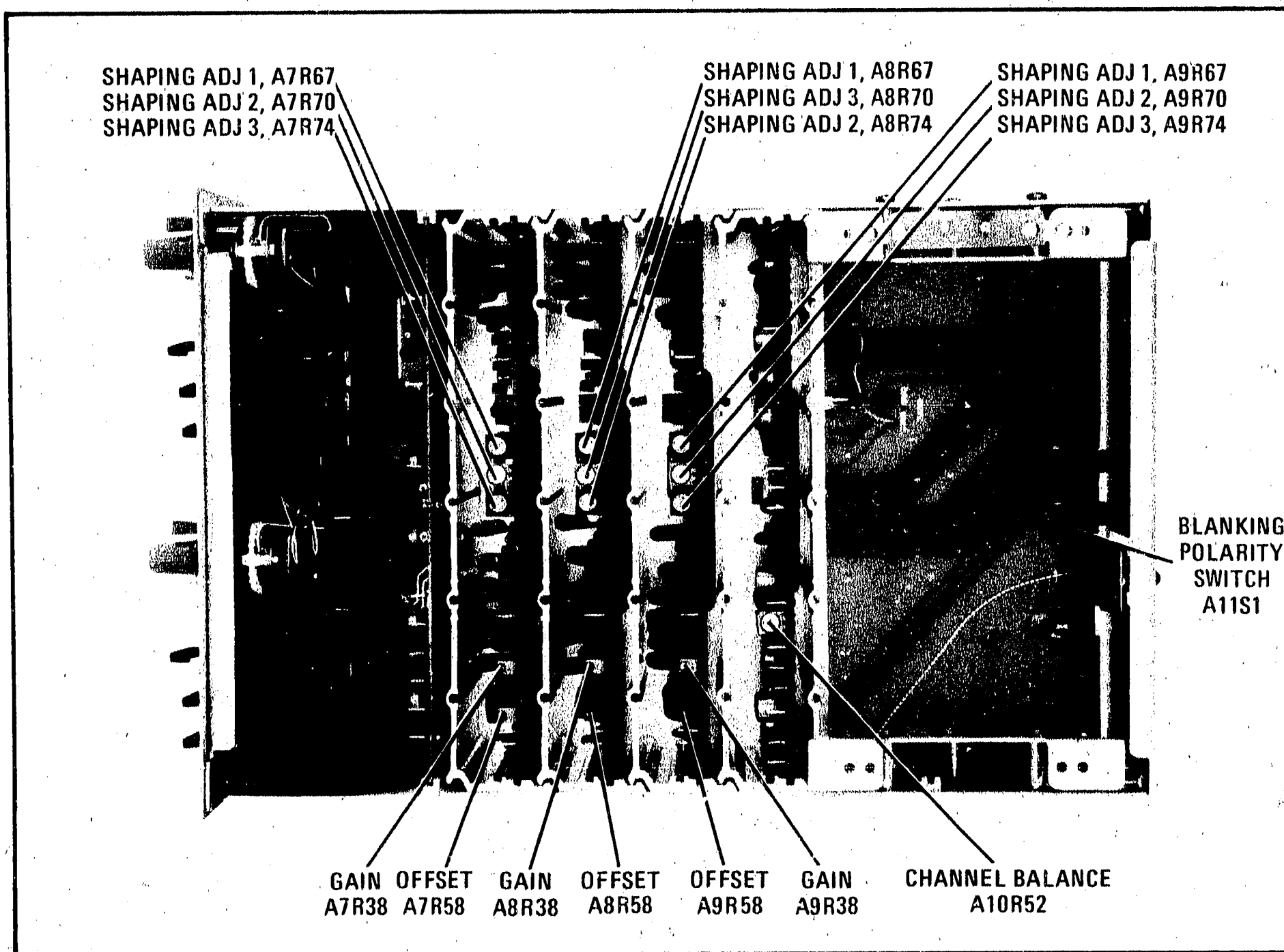
Figure 5-1. Adjustment Locations
