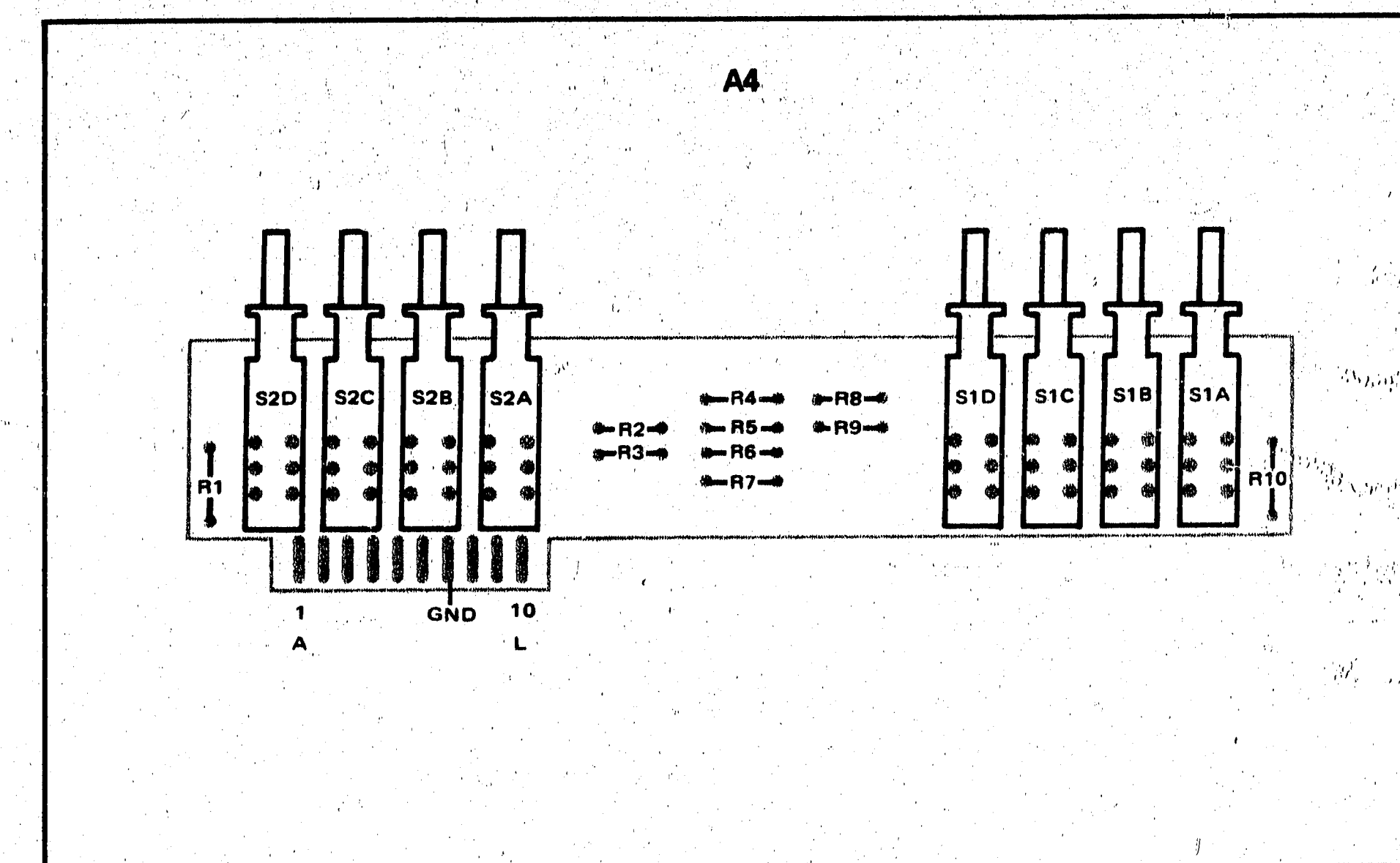
Figure 8-14. A4 Display Switch, Parts Location
