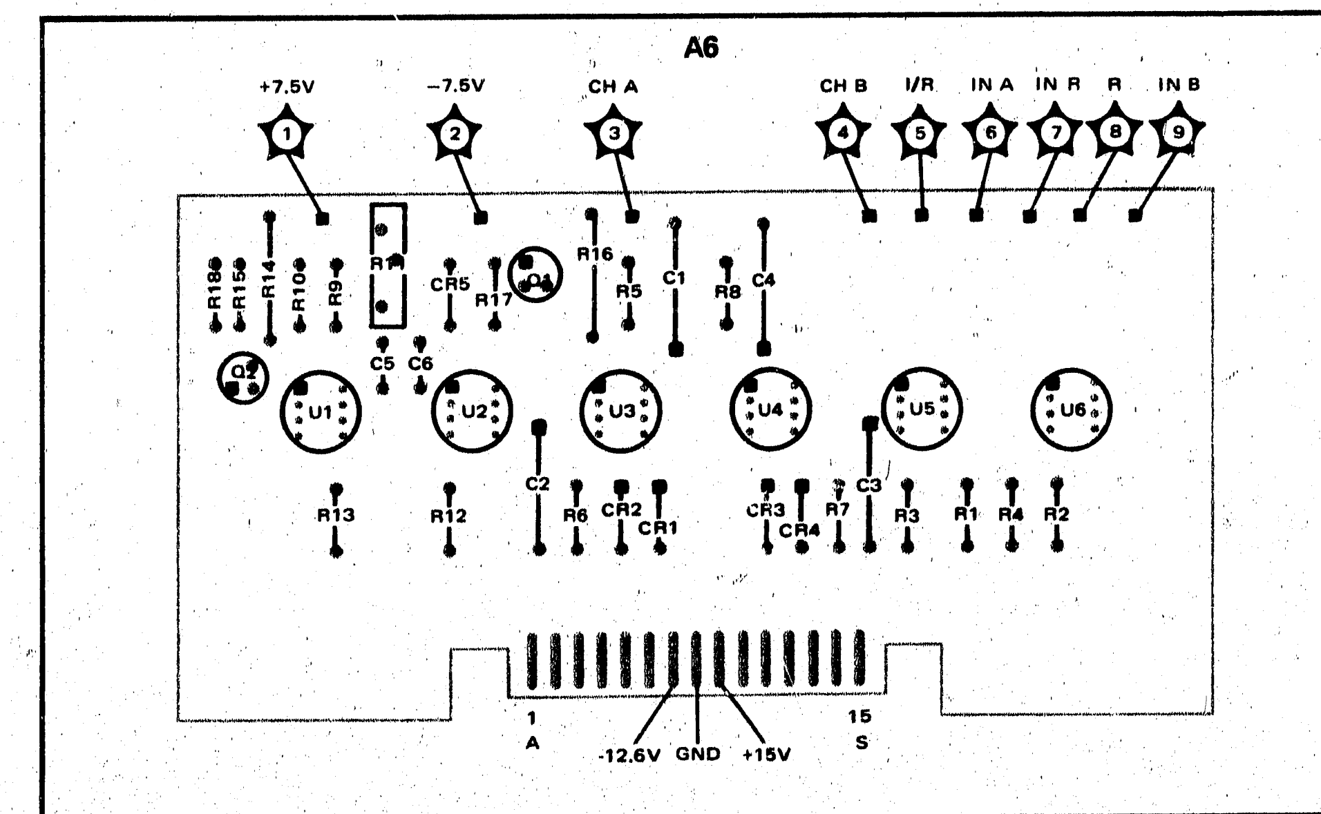
Figure 8-15. A6 Processor Assembly, Parts Location
