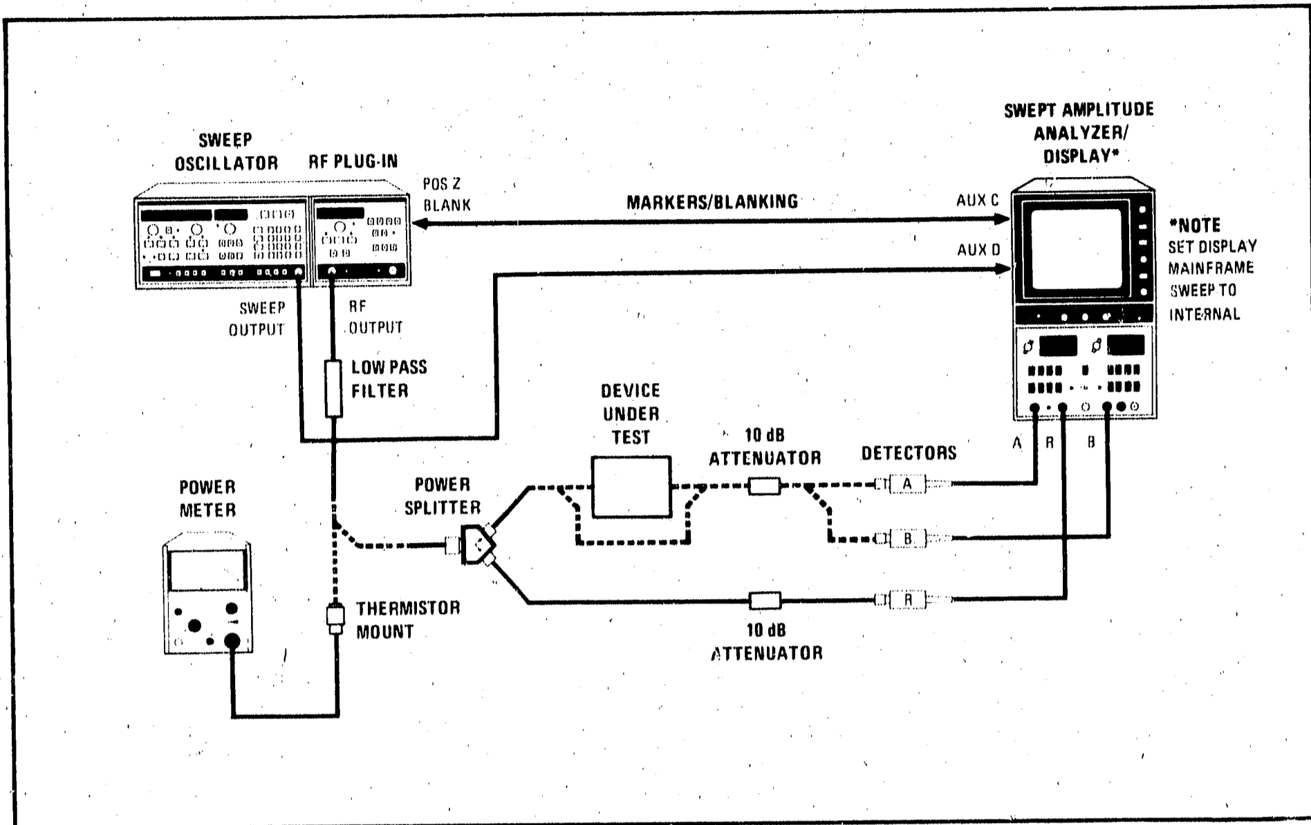
Figure 3-5. Model 11666A Reflectometer Bridge Typical Test Setup
