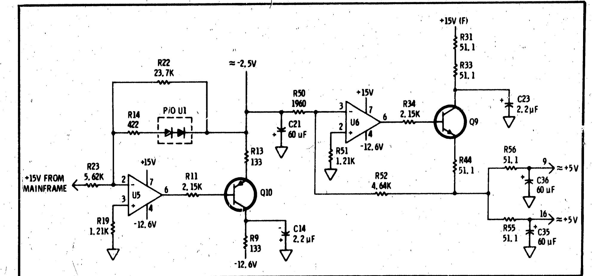
Figure 8-7 Positive and Negative Power Supplies
