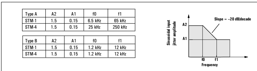
Figure 2 ITU-T G.958 SDH optical line systems jitter tolerance specifications
