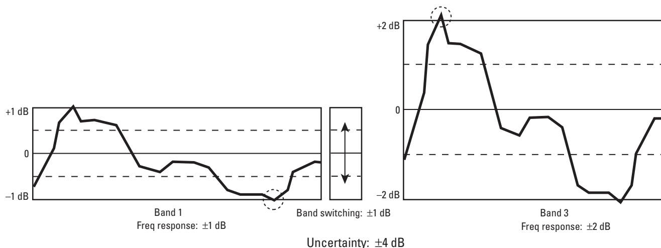
Figure 7. Frequency response uncertainty for a between-band measurement
