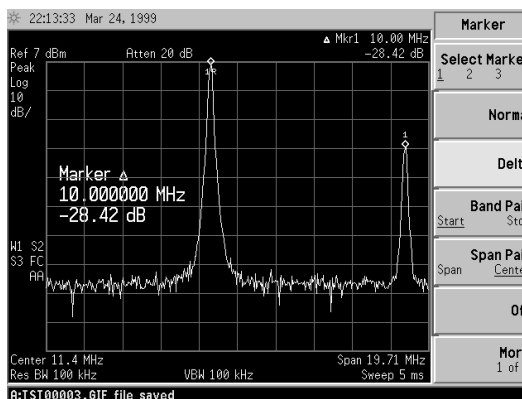
Figure 2. Relative measurement (difference between two signal levels measured with the delta marker)
