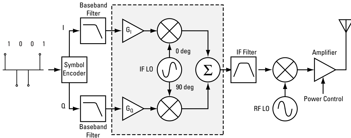
Figure 6. I/Q modulator
