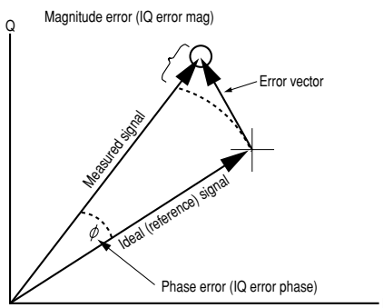
Figure 1. Error vector magnitude (EVM) and related quantities
