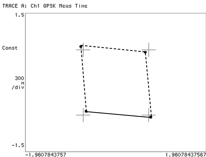
Figure 7. Quadrature error
