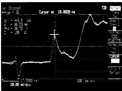
Figure 30. TDR Response to IC package path
