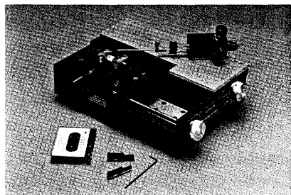
Figure 27. Coaxial to microstrip adaptor
