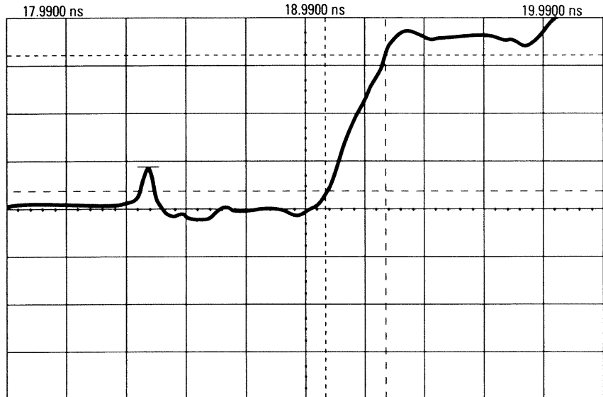
Figure 17. Launching through a semirigid cable onto trace with via hole
