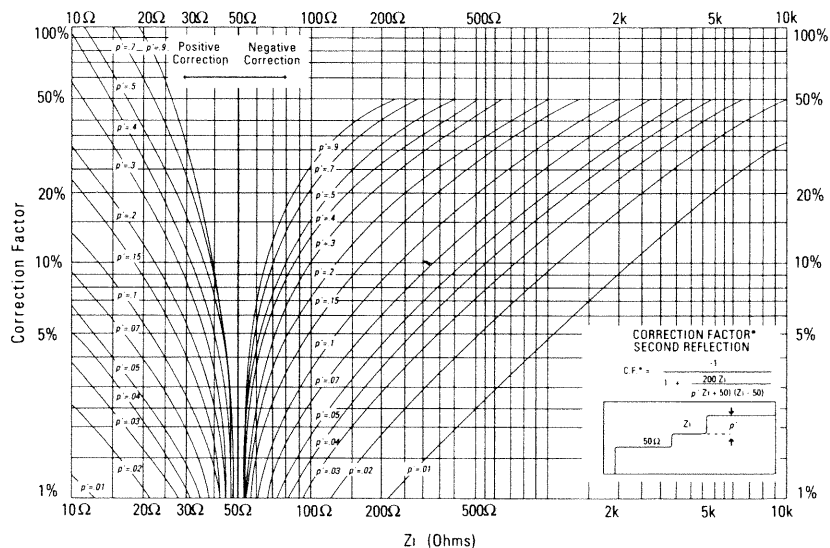
Figure 37. Second reflection correction factor
