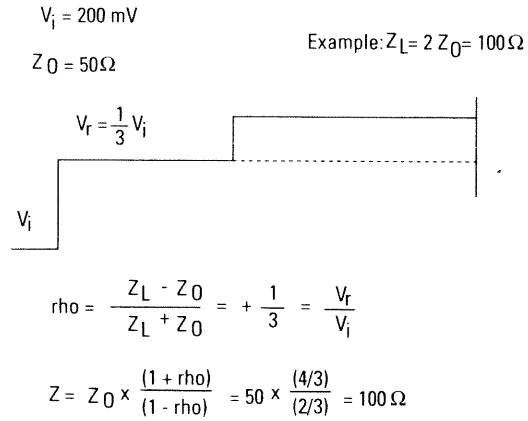
Figure 2. Resistive TDR equations
