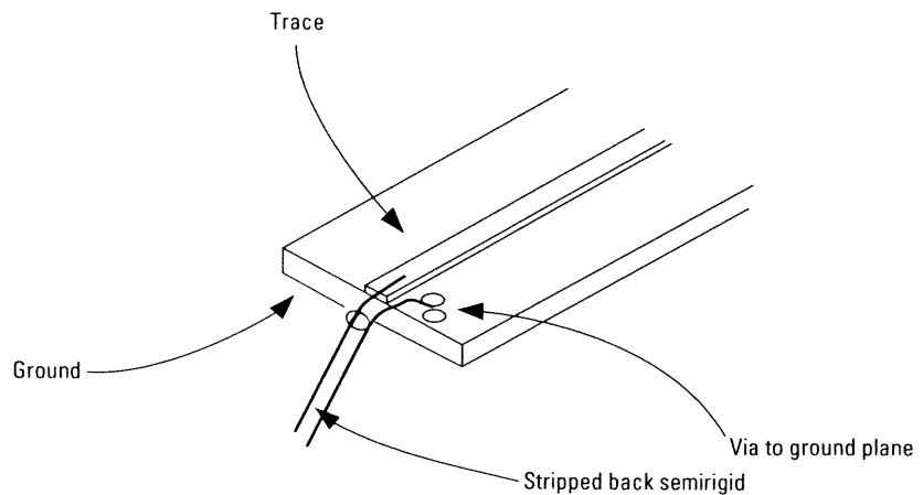
Figure 15. Semirigid cable launched onto trace and via hole
