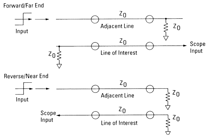
Figure 22. Near and far end crosstalk
