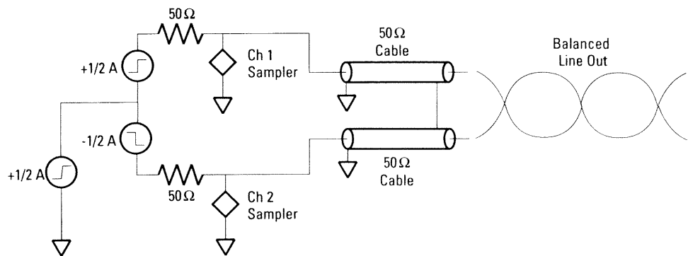
Figure 34. Differential TDR
