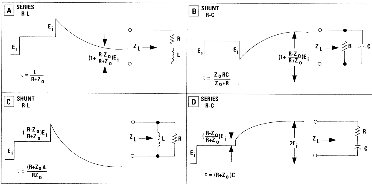
Figure 3. TDR responses to complex loads
