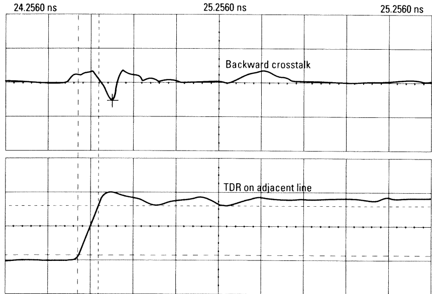
Figure 23. PC Board microstrip trace crosstalk
