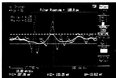
Figure 28. Hybrid measurement
