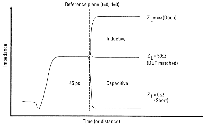
Figure 1. Time domain reflectometry (TDR)
