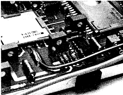
Figure 12. Testing the chip-to-chip interconnect
