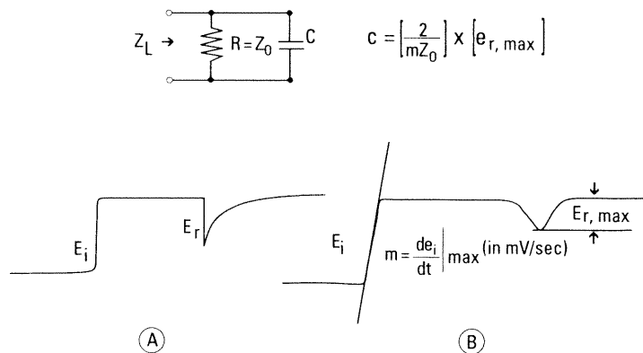
Figure 5. Ideal "A" versus actual "B" displays of reflection from a small capacitor in shunt with R = Z_0
