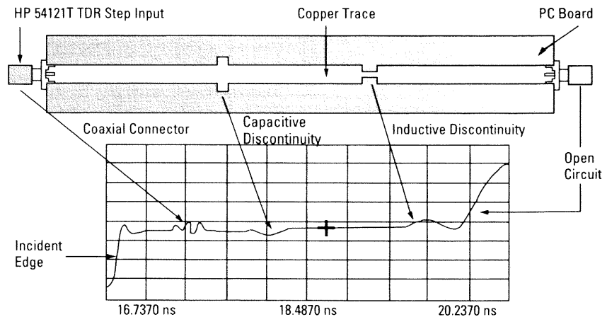
Figure 7. Typical performance characteristics
