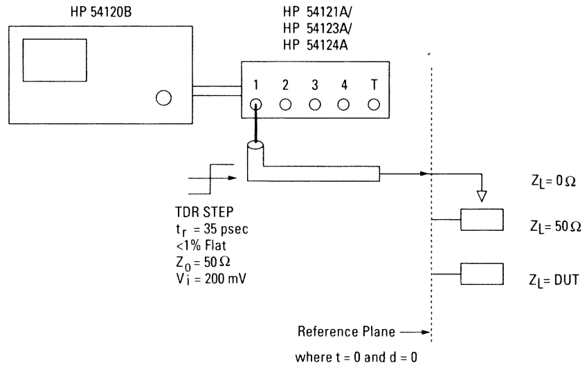
Figure 6. Time domain reflectometry
