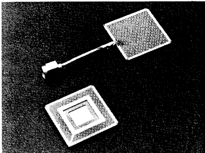
Figure 29. Short semirigid on IC package pad
