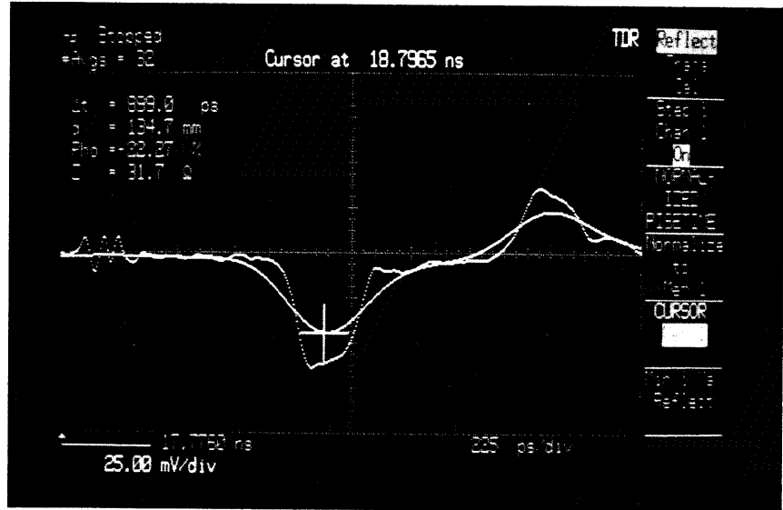
Figure 9. TDR normalized to 300 ps system speed
