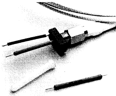
Figure 21. Transmission measurement using the HP 54006A 6 GHz probe
