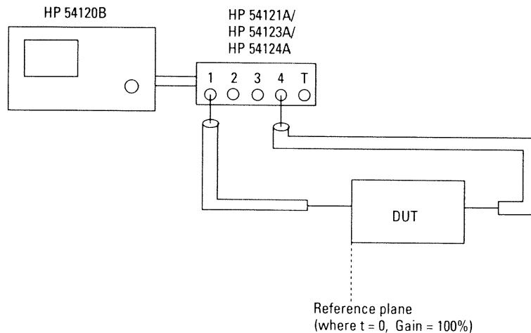
Figure 10. Time domain transmission
