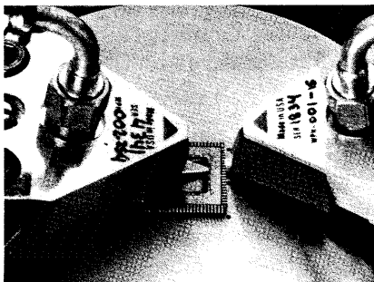
Figure 31. GHz probes to IC package
