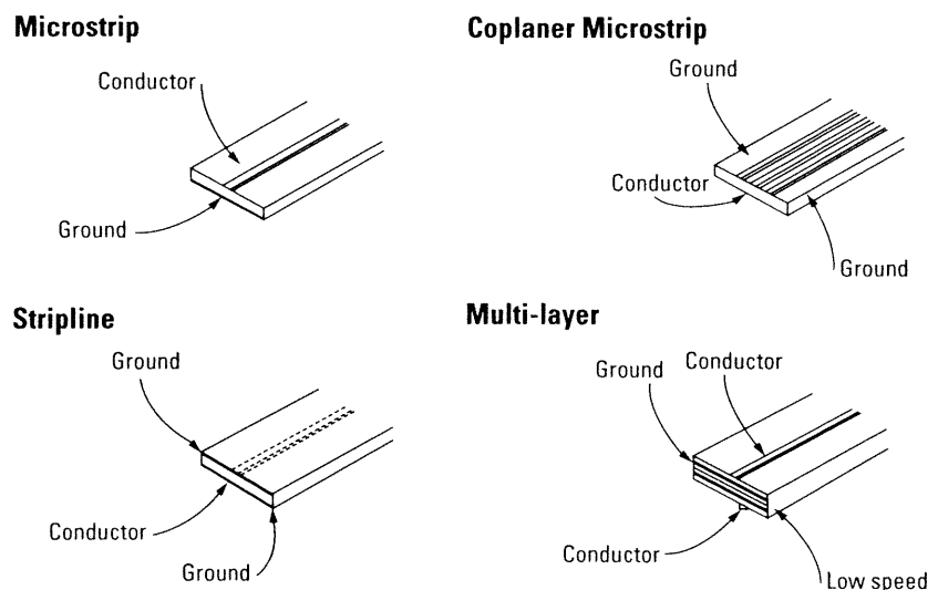
Figure 14. Controlled impedance lines
