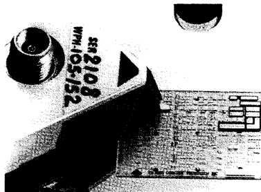
Figure 26. 50 \Omega probe tip to hybrid
