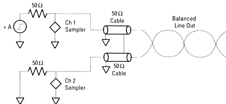
Figure 33. Differential TDR
