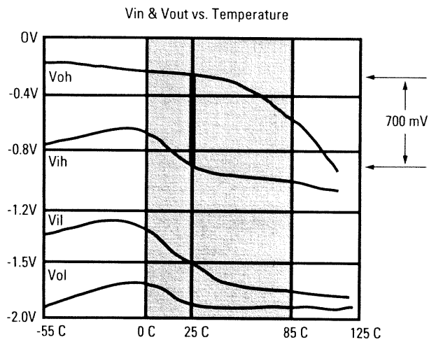
Figure 13. Typical GaAs performance characteristics
