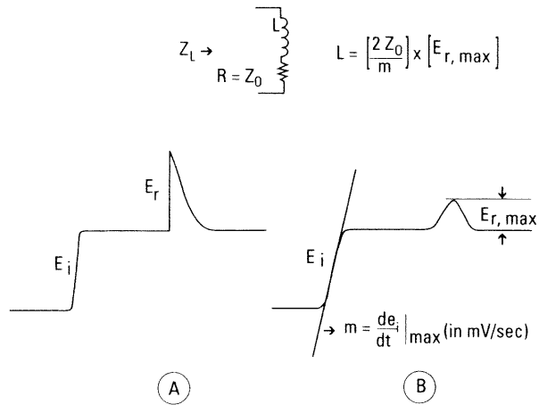
Figure 4. Ideal "A" versus actual "B" displays of reflection from a small inductor in series with R = Z_0
