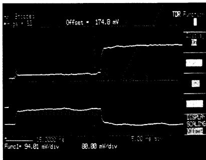
Figure 36. Twisted pair measurement
