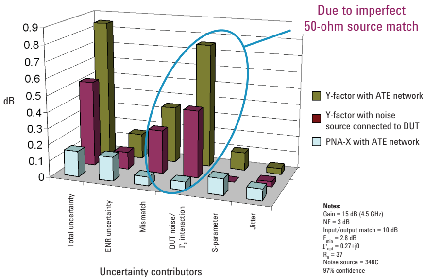
Figure 17. Breakdown of error contributions for noise figure uncertainty example of ATE environment
