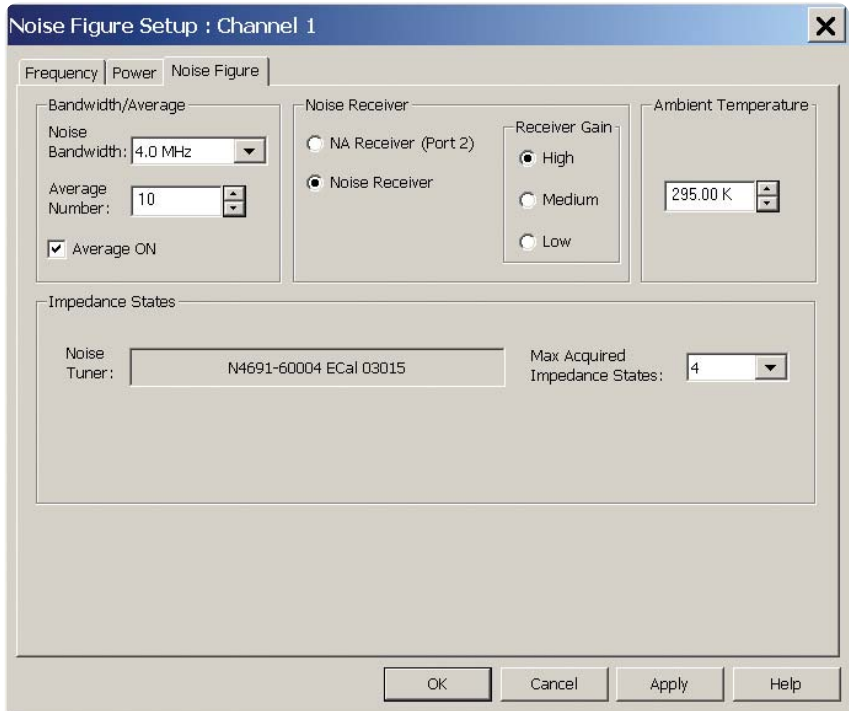
Figure 26. Option 029/H29 noise figure setup dialog, showing choice of noise receiver or standard NA receiver
