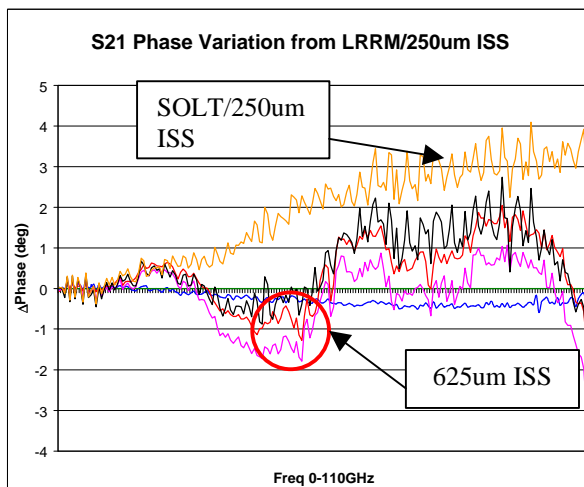
Fig. 10. S21 Phase variation of GaAs FET device with reference to LRRM calibration using 250um ISS.
