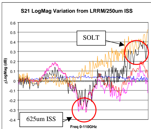
Fig. 9. S21 LogMag variation of GaAs FET device with reference to LRRM calibration using 250um ISS.
