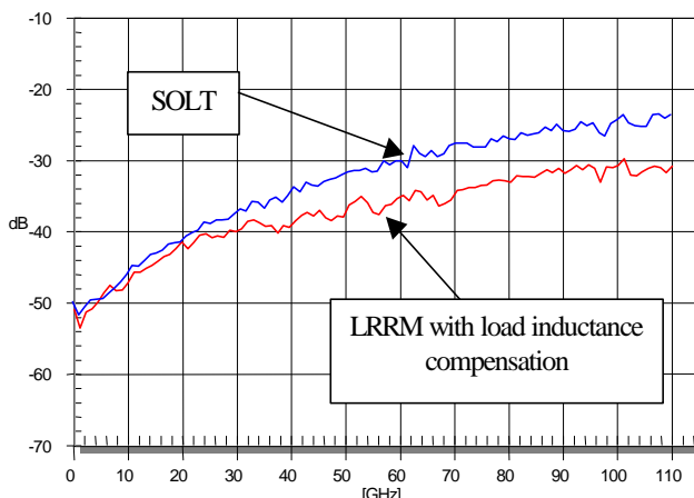
Fig. 12. The worst case errors for calibration repeatability, using two different sets of standards.
