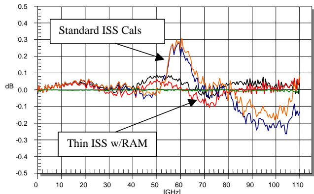
Fig. 2. Measurement of open standard after SOLT, LRM & LRRM calibrations.
