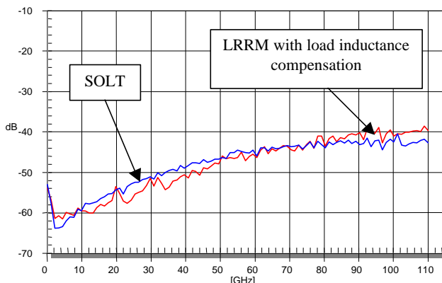
Fig. 11. The worst case errors for calibration repeatability using the same set of standards
