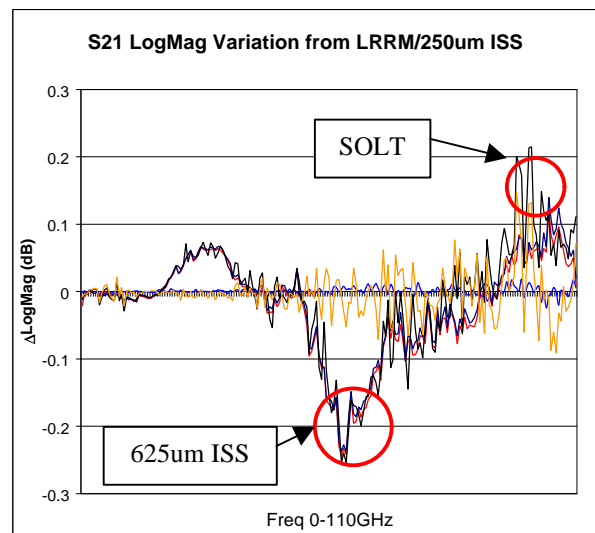
Fig 6. LogMag variations of line using LRRM/250um ISS as reference. (ISS calibrations only)
