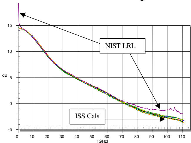
Fig. 8. Measurements of a GaAs FET device.
