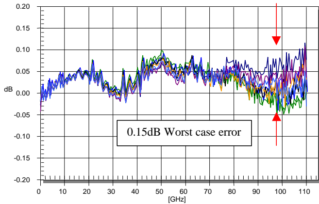
Fig. 13. Sii Open measurement of 8 LRRM calibrations
