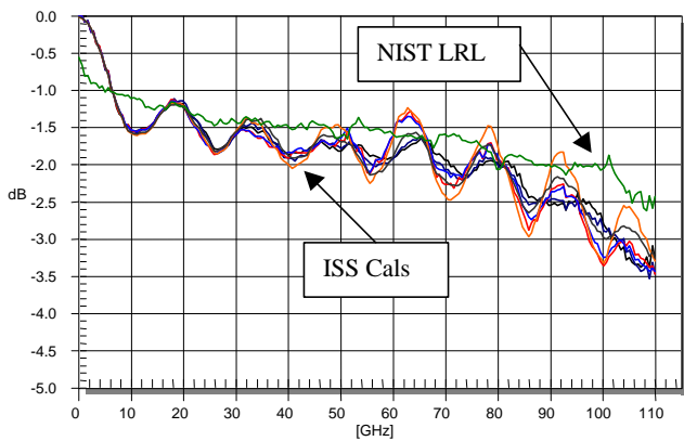
Fig. 3. S11 LogMag measurement of 3.2mm open stub.
