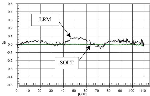
Fig. 1. Measurement of open standard after calibration falsely shows SOLT to be perfect, which is a result of the SOLT calibration forcing the reflections to be 0.0dB
