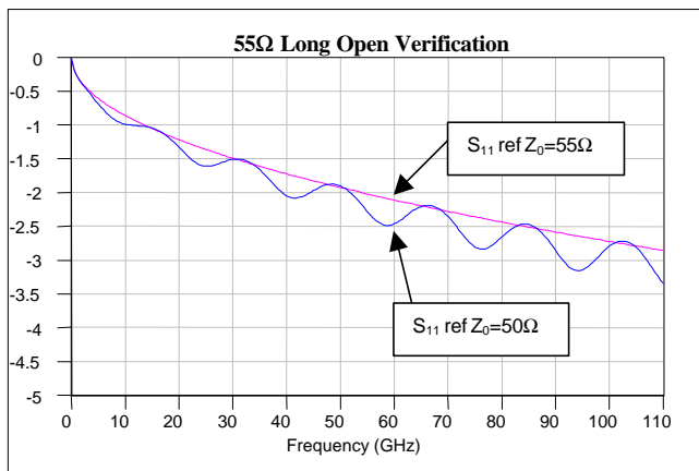
Fig. 4. Model of 3.2mm open verification standard, making the assumption that the GaAs line is not 50ohms
