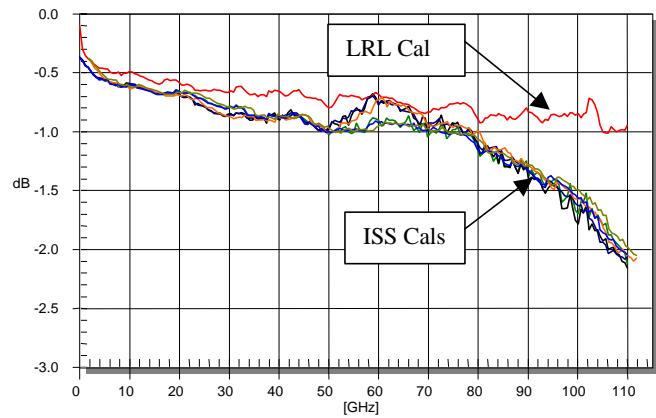
Fig. 5. S21 LogMag measurement of NIST 3.2mm line
