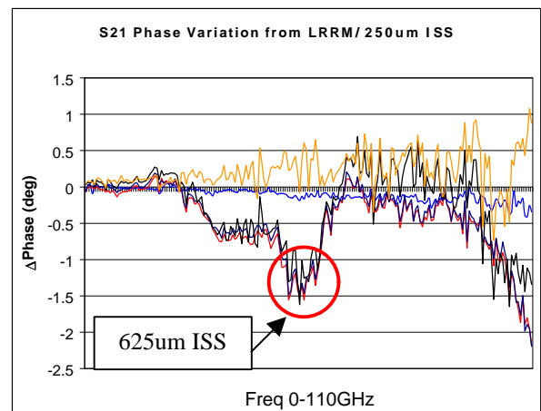
Fig. 7. Phase variation of line using LRRM/250um ISS as reference. (ISS calibrations only)
