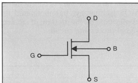
Figure 6a. Circuit symbol for the n -channel depletion-type MOSFET.
