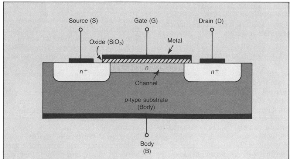
Figure 5. Basic structure of n -channel depletion-type MOSFET.
