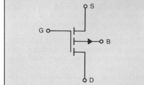
Figure 8b. Circuit symbol for the p -channel enhancement-type MOSFET.
