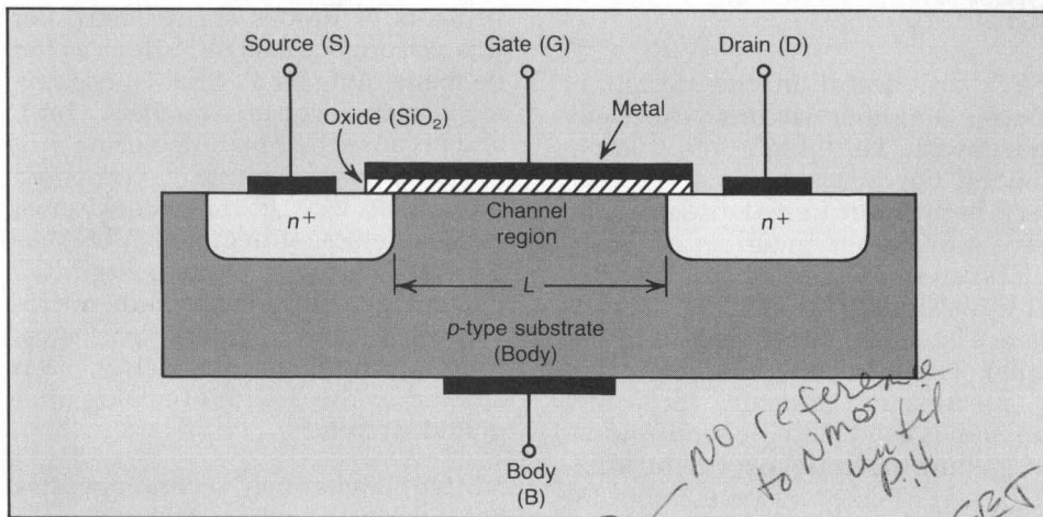
Figure 7. Basic structure of enhancement-type NMOS transistor.
