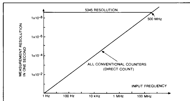
Figure 3. Measurement Resolution
