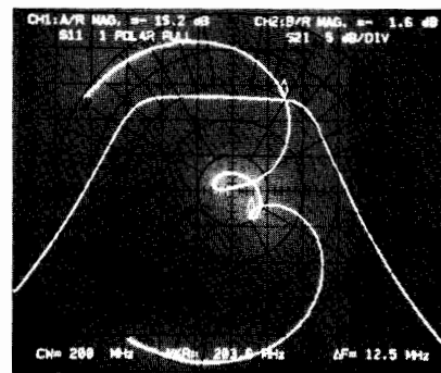
Both polar impedance and amplitude response of a filter are plotted on a network analyzer. Models 1332A, 1335A, 1340A, and 1345A can be used in many types of measurement instruments.
