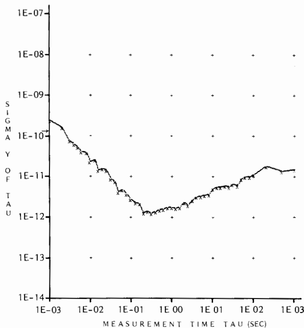
Sample \sigma_{\gamma}(\tau) vs \tau plot generated by 5390A.
