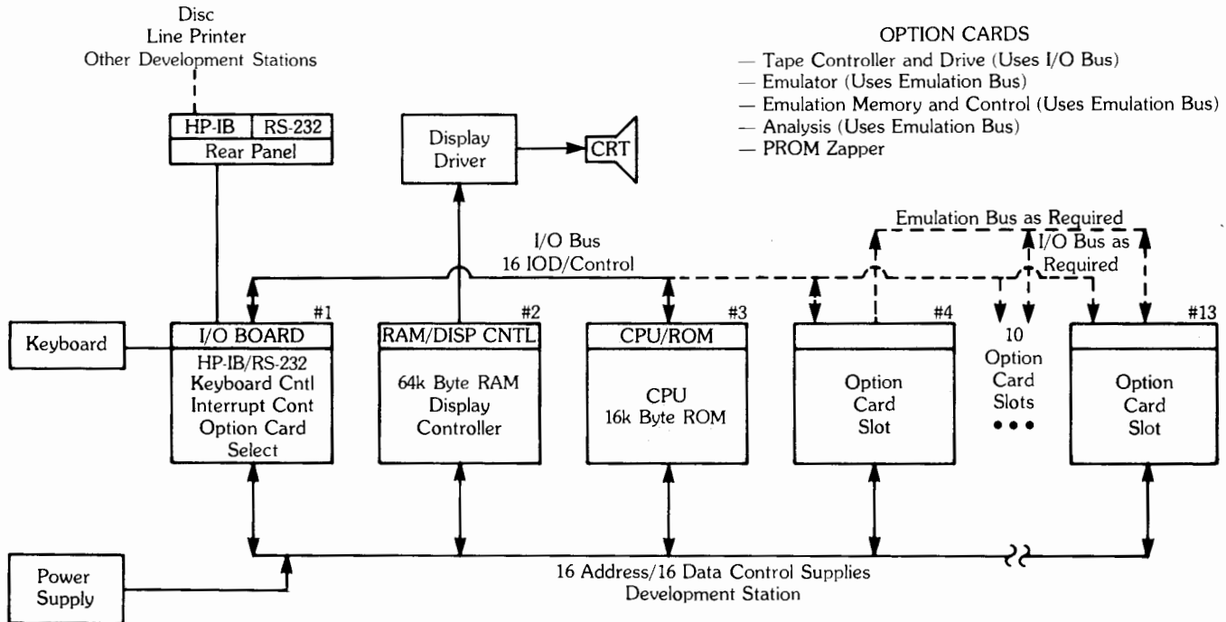
Figure 1. Model 64100A Development Station card cage reserves the first three slots for the host system, and the remaining ten slots are available for system options. If an emulation function is added, a separate, high-speed bus is used for the emulator.
