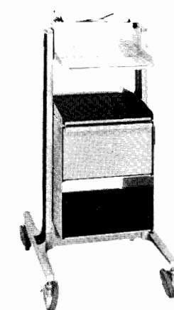
Opt 005: storage cabinet and drawer in upper position with shelf on top; load limit 18 kg (40 lb) ea on shelf and in cabinet, 11 kg (25 lb) in drawer.
