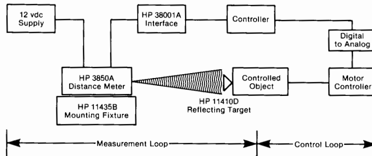
Typical HP 3850A Control System
