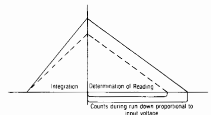
Figure 1. The classical dual-slope integration technique is limited in speed to how fast the zero crossing can be detected accurately. In addition, the final reading is not known until run-down has been completed. Note that the voltage remaining on the integrator's capacitor is proportional to input level.
