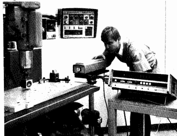
Machine tool calibration using 5526A
