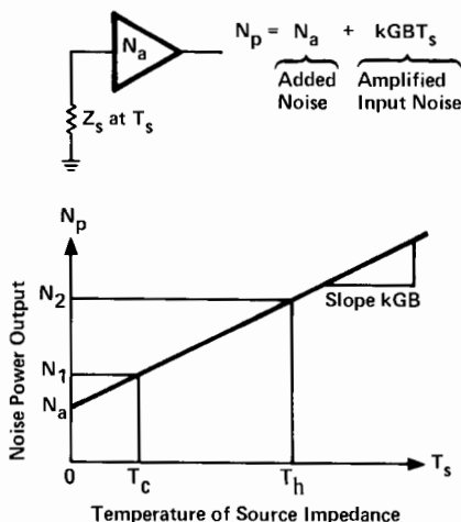
Figure 2. Available noise power.
