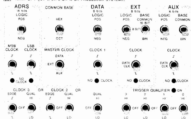
1611A OPT 001 (FOR 8 OR 16 BIT PROCESSOR SYSTEMS)
