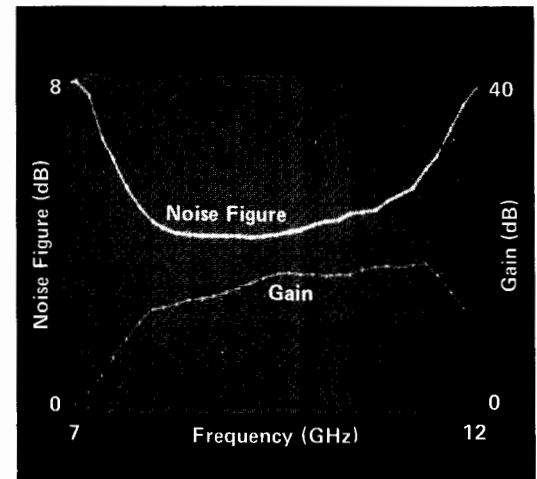
Typical oscilloscope display of amplifier.
