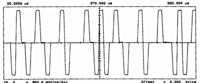
3- and 4-level signals produced by HP 8118A's internal channel addition feature a) HDB3 signal b) 2B1Q signal
