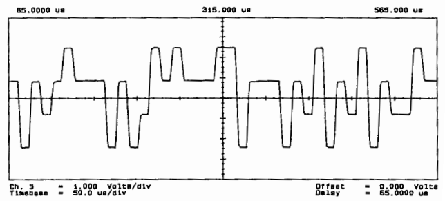
3- and 4-level signals produced by HP 8118A's internal channel addition feature a) HDB3 signal b) 2B1Q signal
