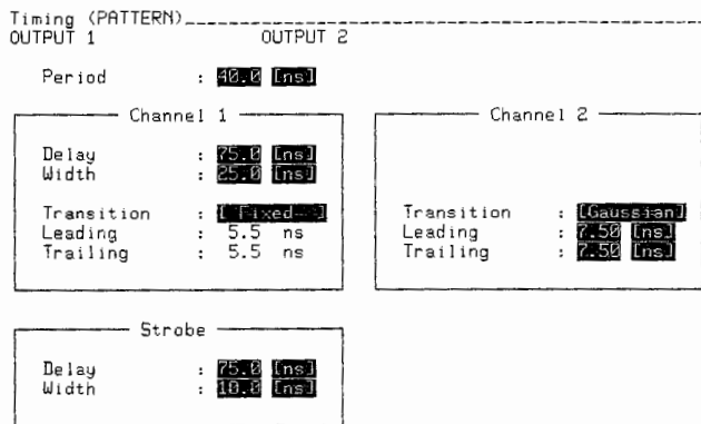
Timing parameter display of both channels and the additional strobe channel
