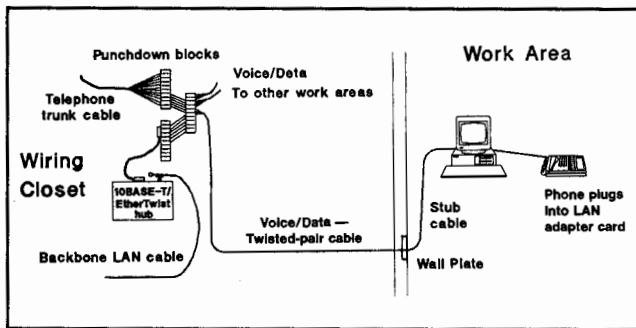
Twisted-pair cable installation
