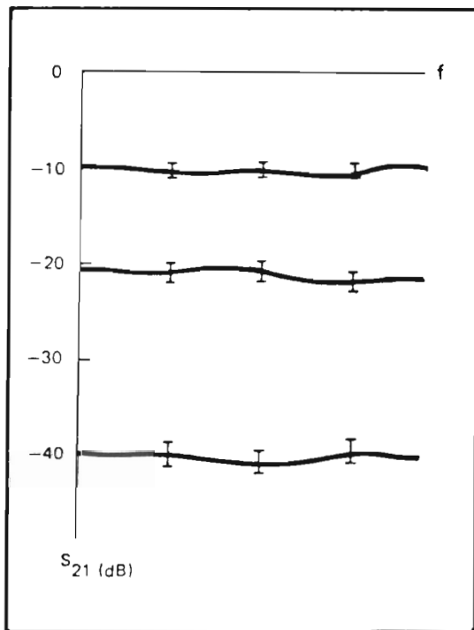
S 21 Magnitude of fixed attenuators used as cross-check devices
