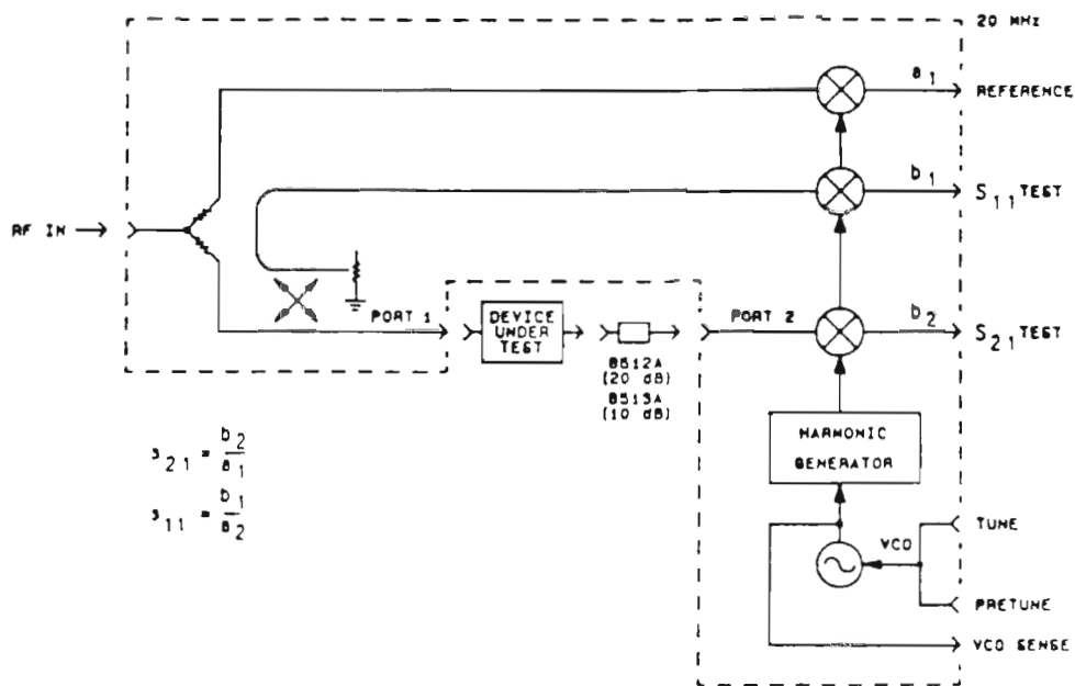
Reflection/Transmission Test Sets Signal Flow.
