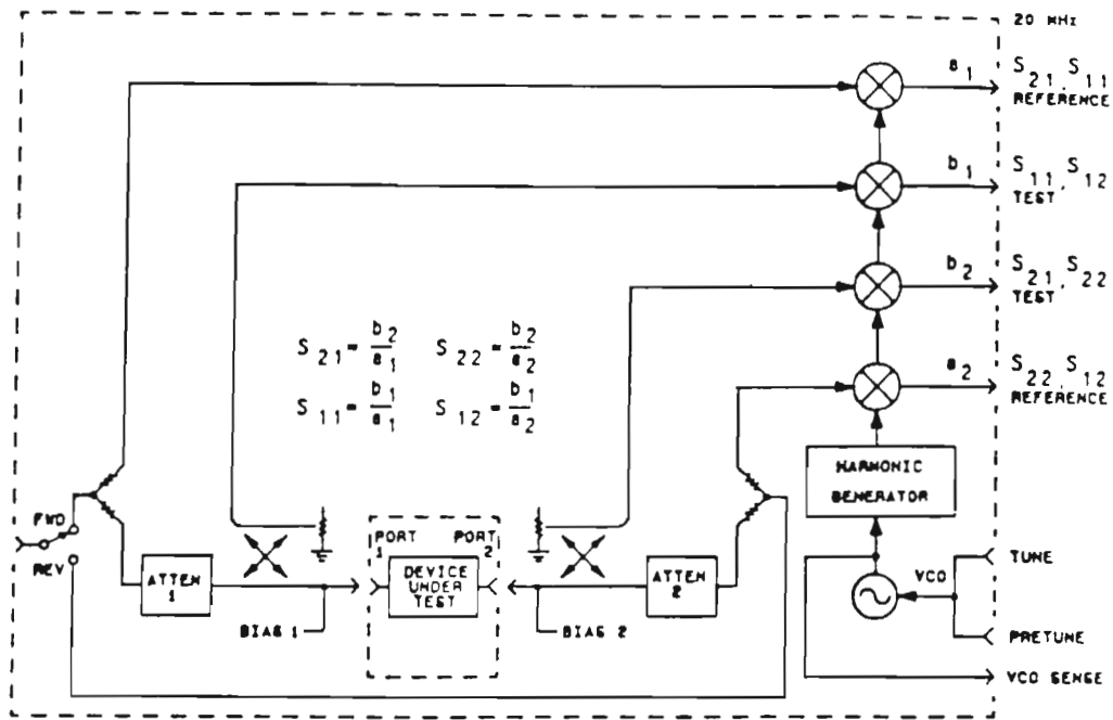
S-Parameter Test Sets Signal Flow.
