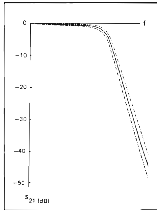
S 21 Magnitude of a low-pass filter
