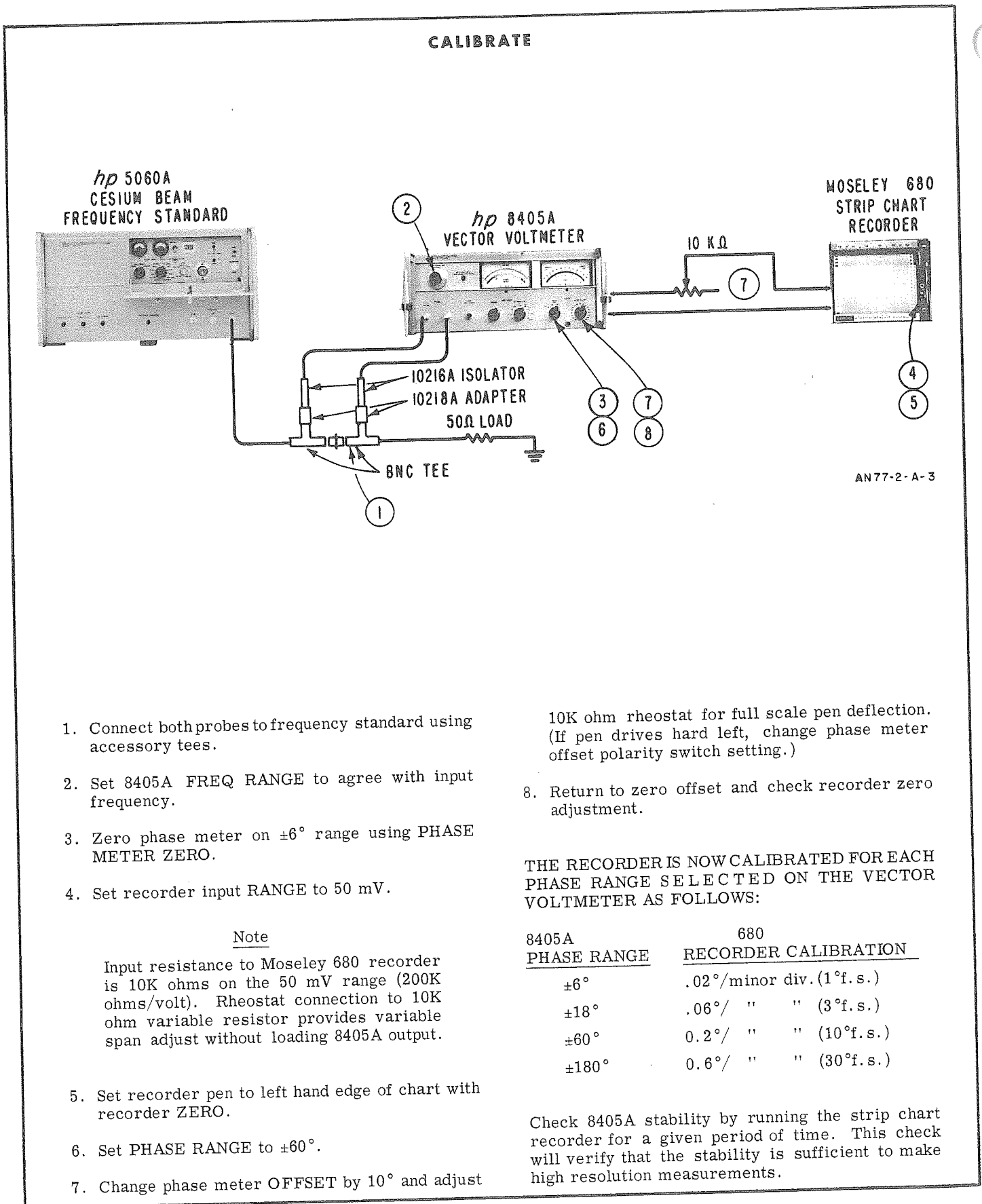
Figure 4. Measurement procedure for high resolution comparisons of frequency standards (sheet 1 of 2).
