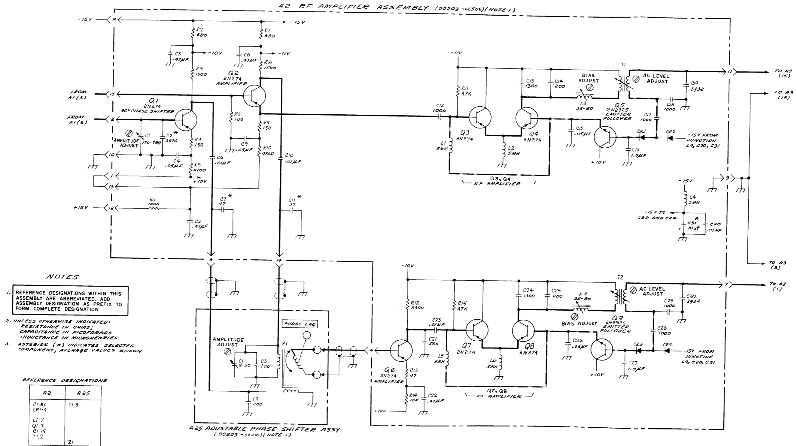
Figure 5-12. RF Amplifier Assy A2 and Adjustable Phase Shifter Assy A25--Schematic
