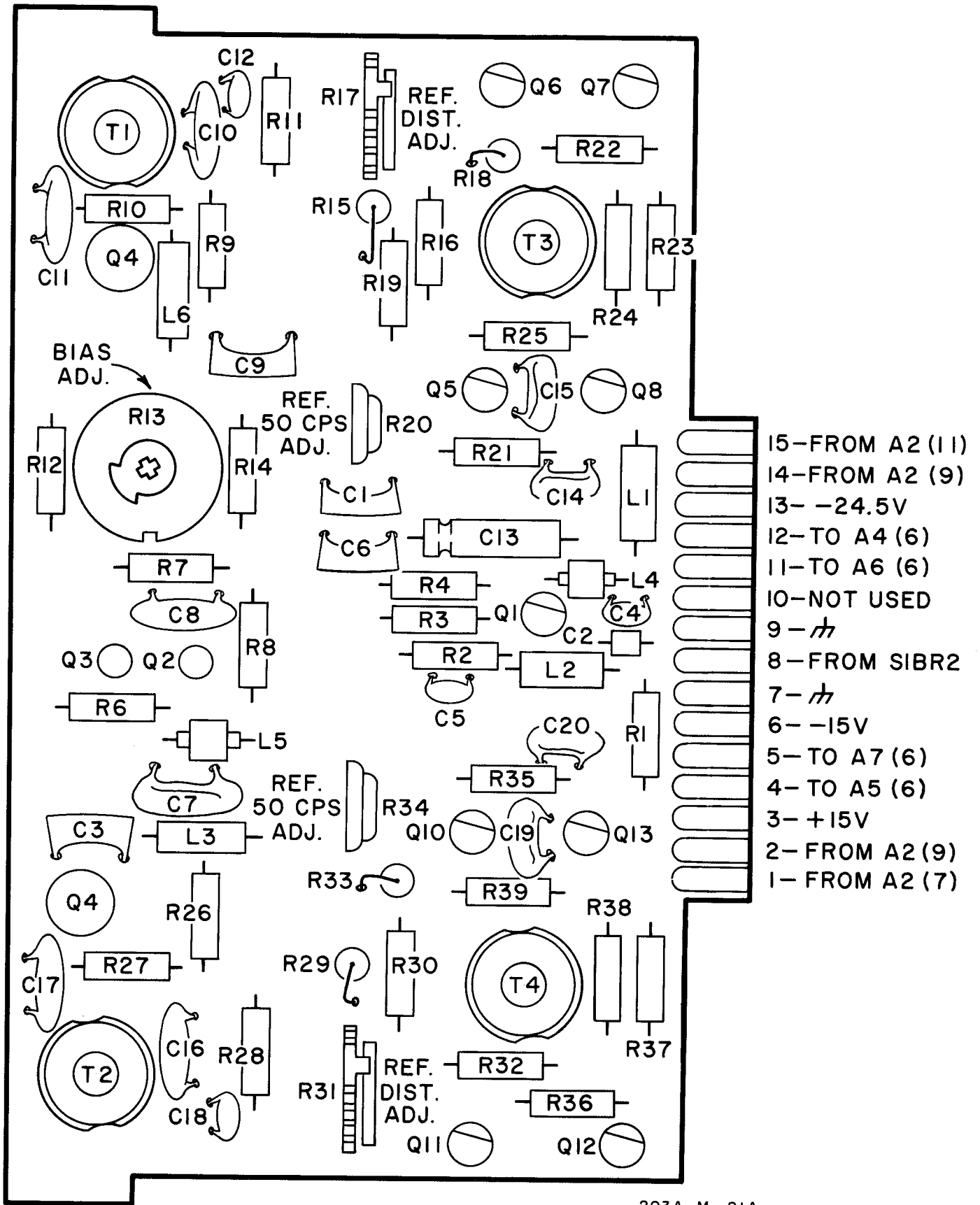
Figure 5-15. Modulator Assy A3--Component Location
