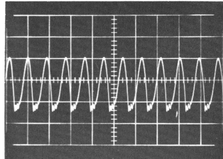
12- A11Q3 Emitter L2 nominal .5 V/CM; 2 \mu SEC/CM
