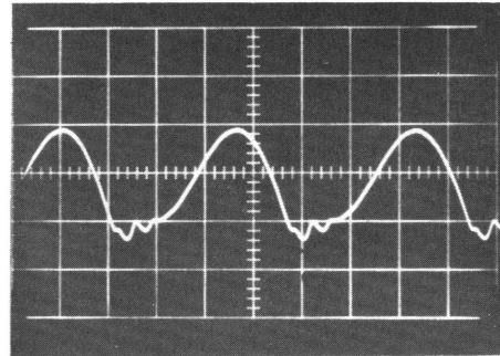
11- A11Q3 Emitter L2 maximum for synchronization .5 V/CM; .5 \mu SEC/CM
