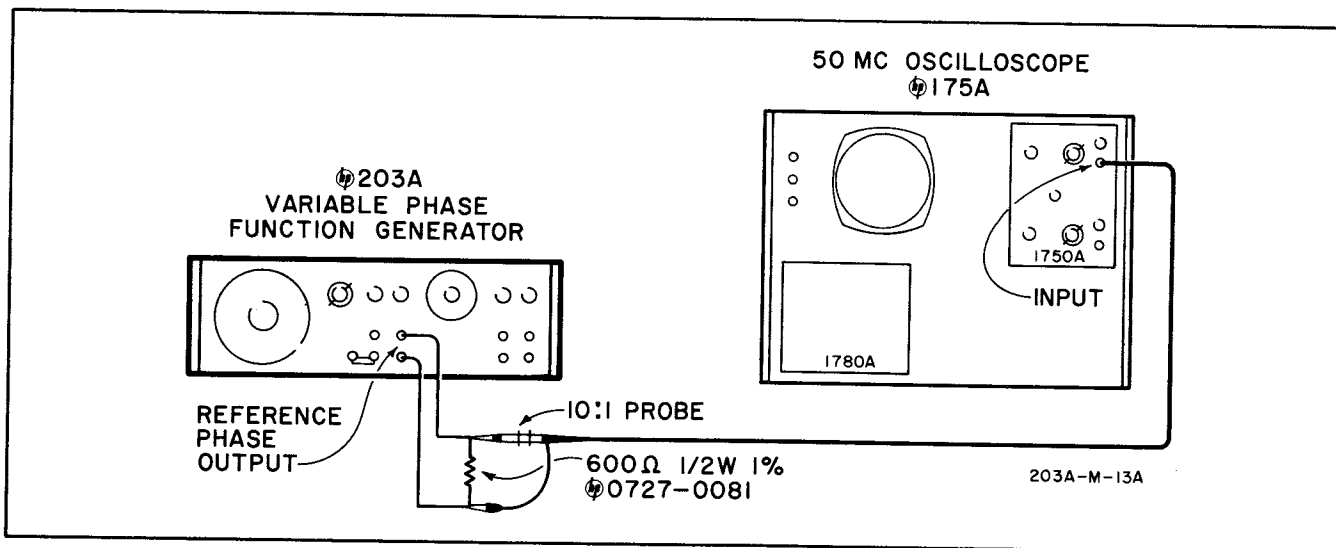
Figure 5-4. Square Wave Check
