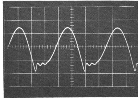
10- A11Q3 Emitter L2 minimum for synchronization .5 V/CM; .5 \mu SEC/CM
