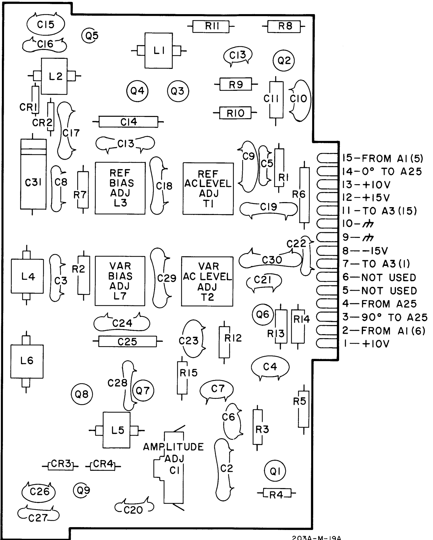
Figure 5-11. RF Amplifier Assy A2--Component Location
