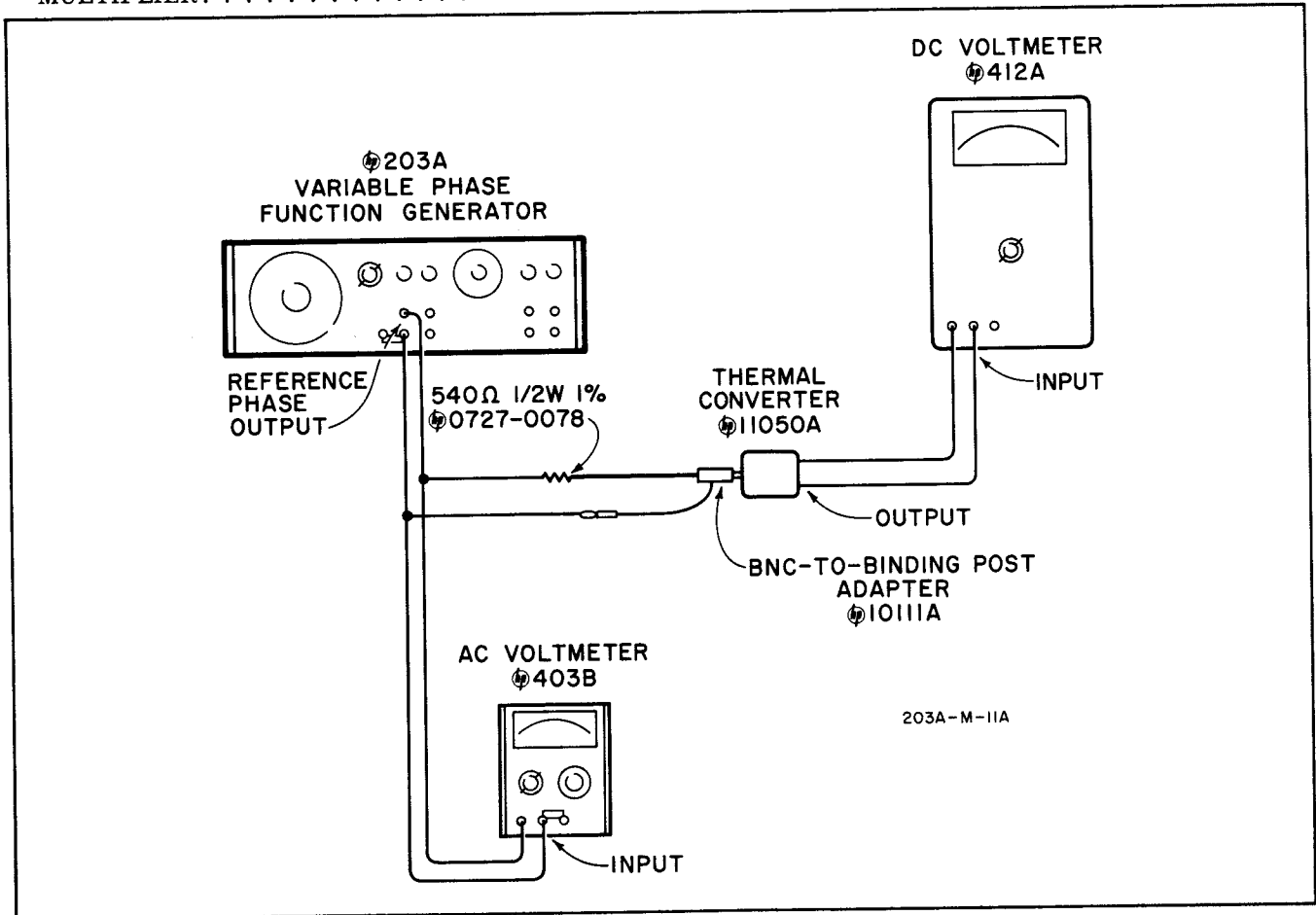
Figure 5-2. Frequency Response
