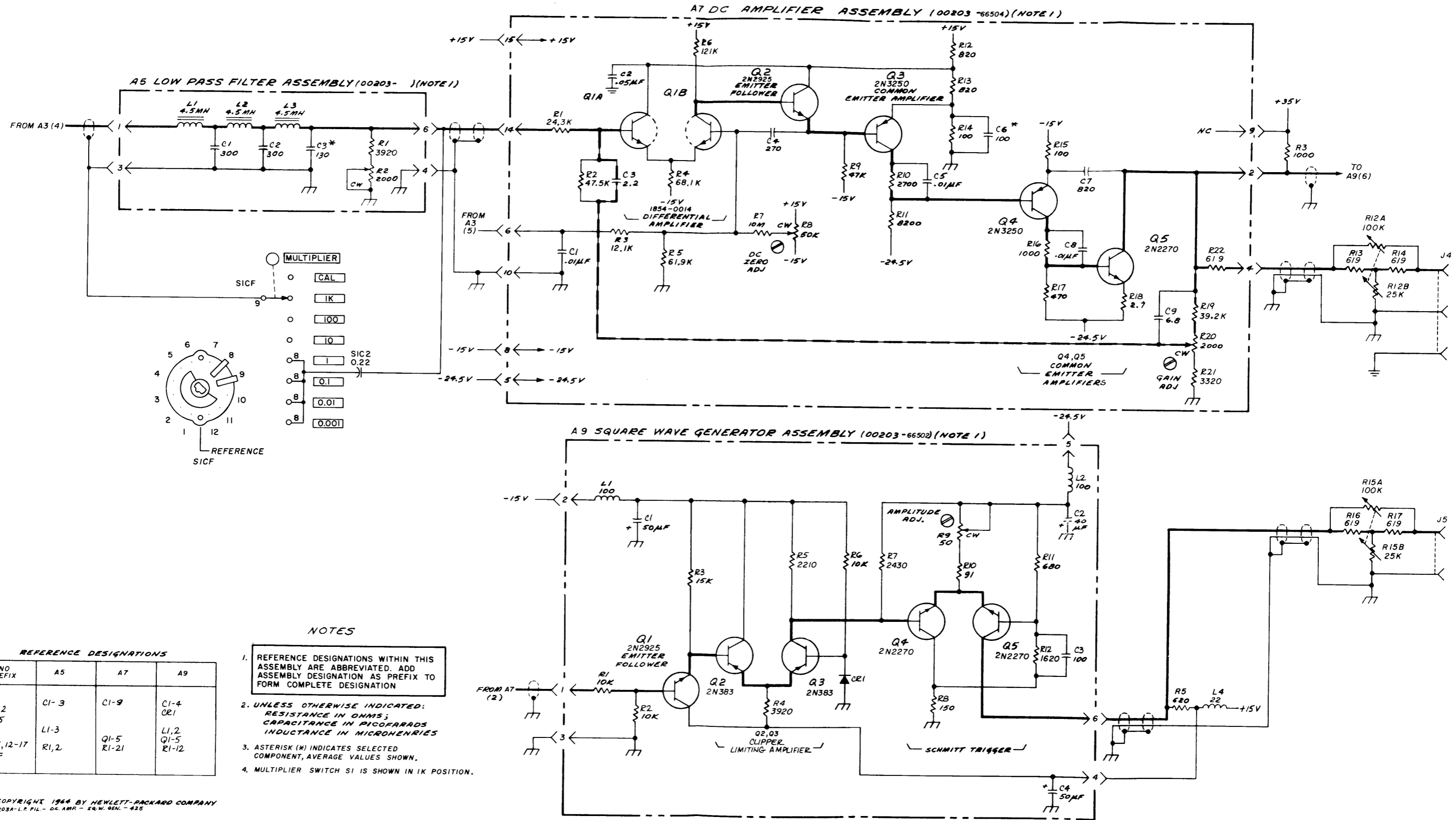
Figure 5-20. Low Pass Filter Assy A5, DC Amp Assy A7, and Square Wave Gen Assy A9--Schematic
