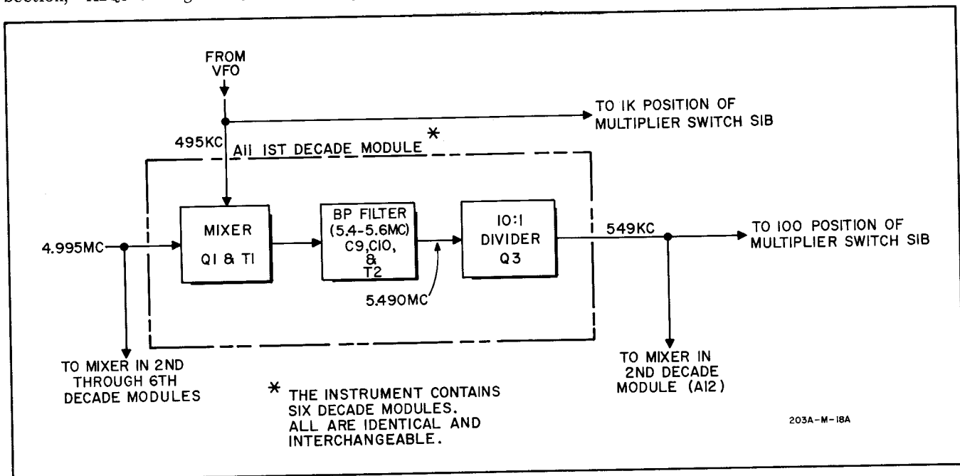
Figure 4-2. Circuit Details
