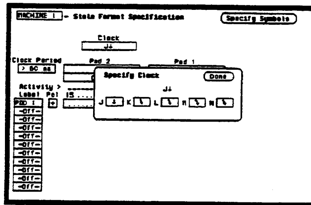
Figure 3-3. State Clock Pop-Up Menu
