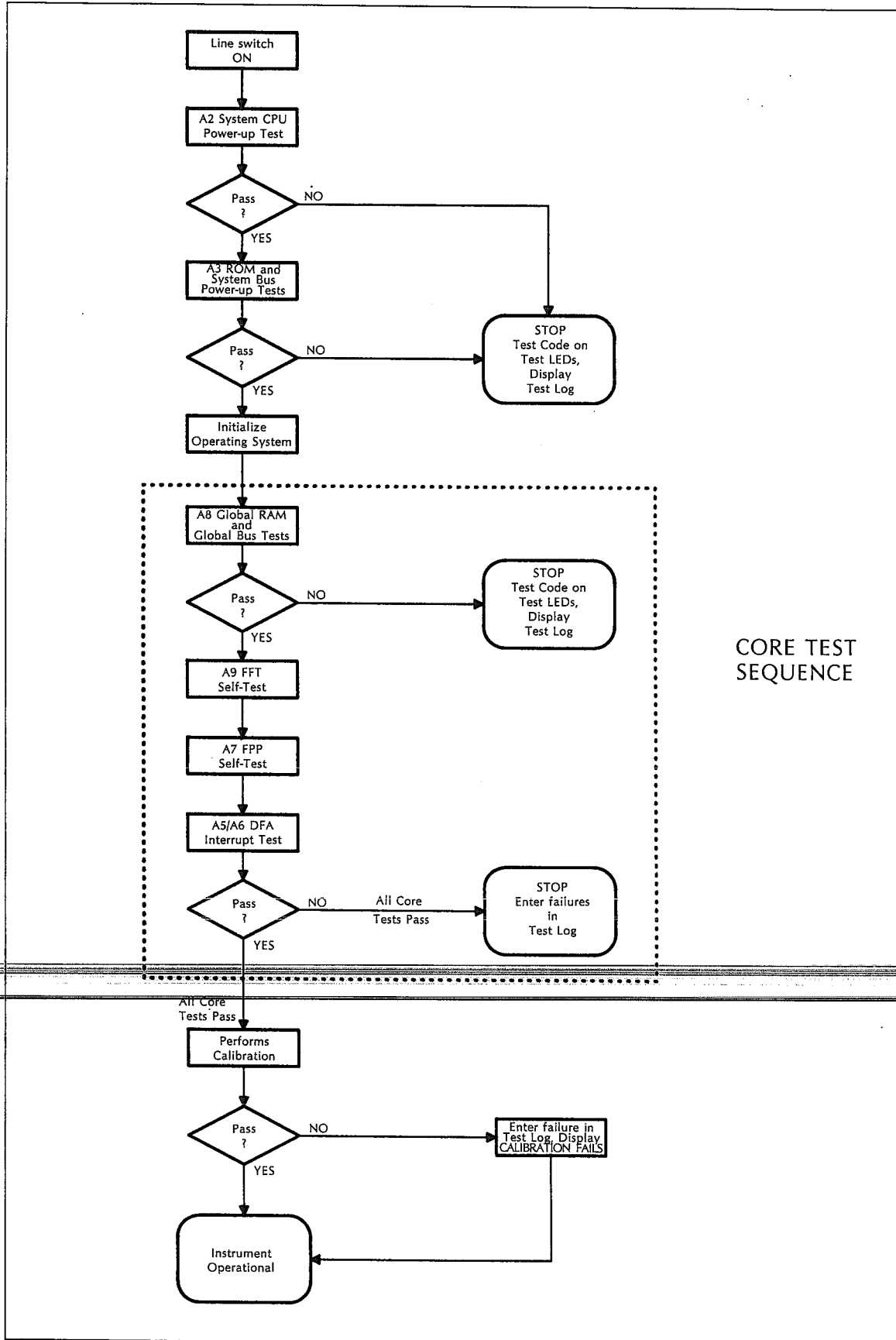
Figure 7-12 Power-up Sequence
