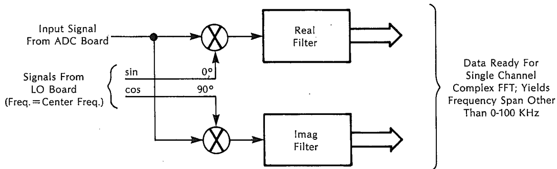
Figure 6-A5b Zoom Implementation
