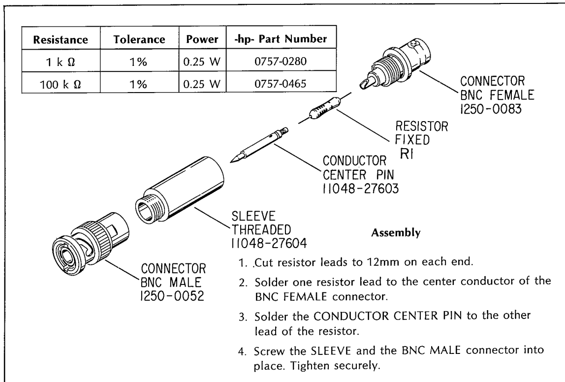
Figure 1-4 Constructing a Feedthrough
