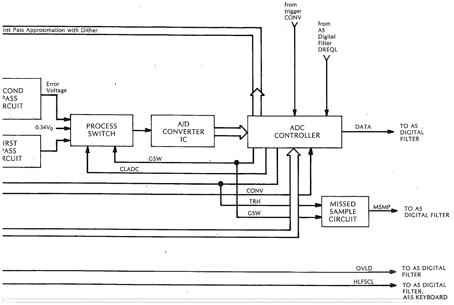
Analog Digital Converter Block Diagram
