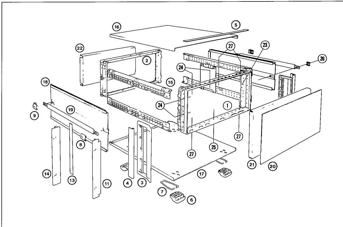
Figure 4-2 Cabinet Parts, Exploded View
