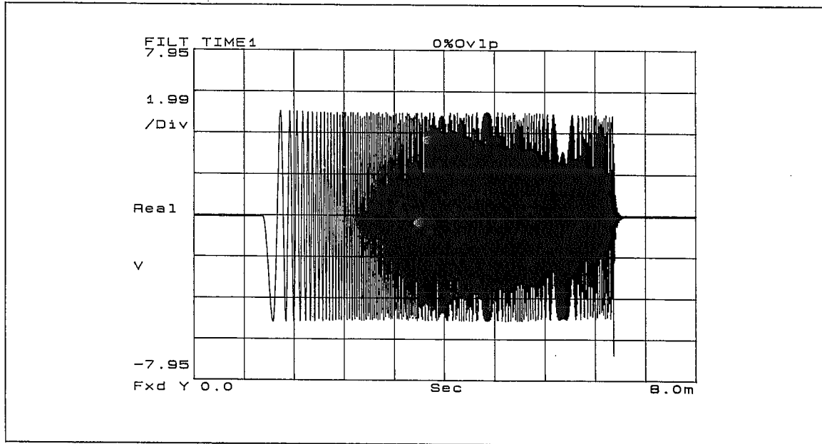
Figure 7-8 Burst Chirp
