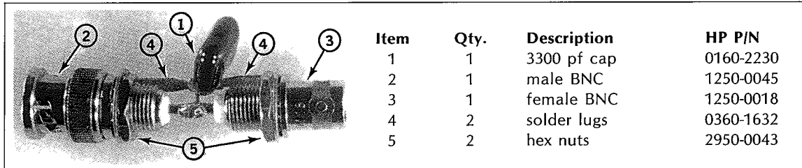
Figure 3-3 Capacitive load
