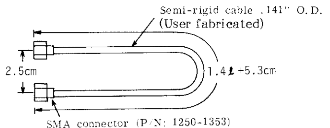
Semi-rigid cable E-L compensator.
