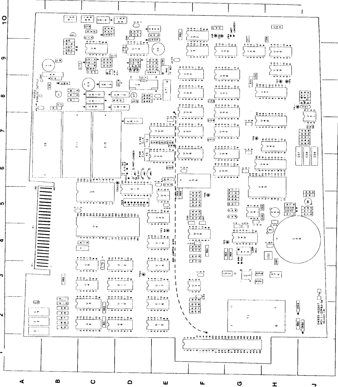
A14 Transmitter Board Component Locator
