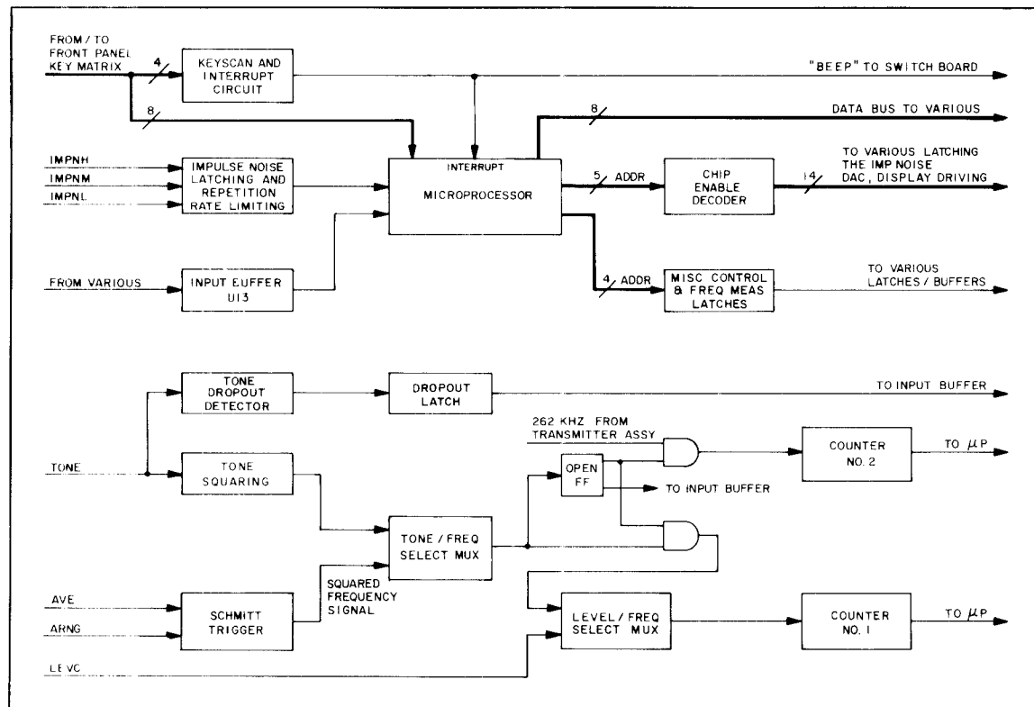
Figure 8-5. Control Circuitry Block Diagram
