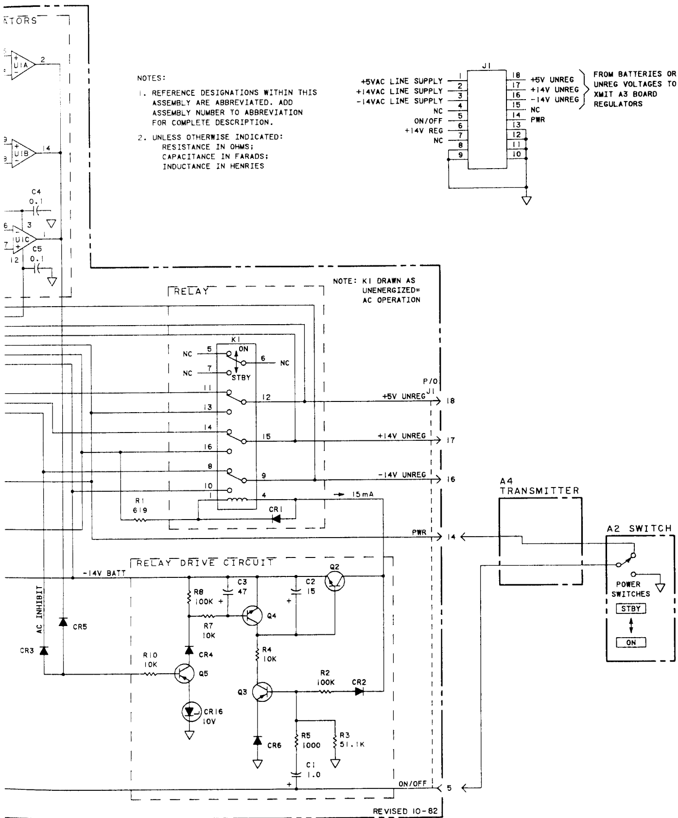
Figure 7-32. A5 Charger Board Schematic Diagram 7-43 / (7-44 blank)
