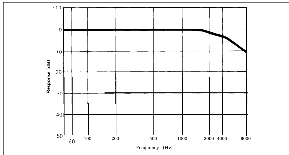
Figure 3-7. 3 kHz Flat Weighting Characteristic
