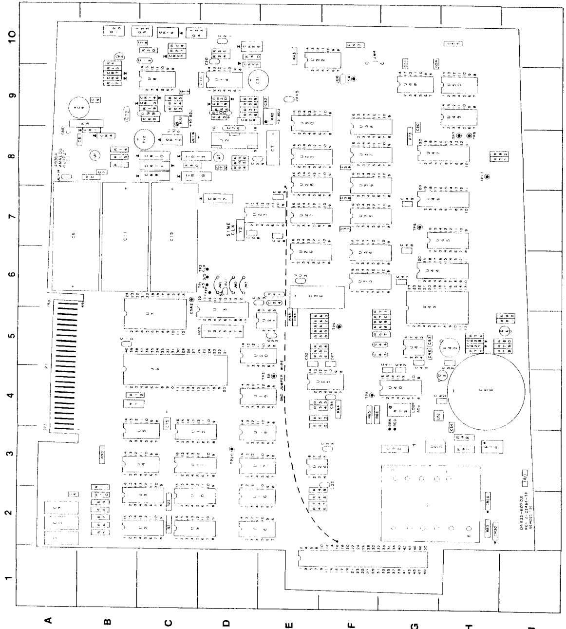
Figure 7-27. A4 Transmitter Board Component Locator
