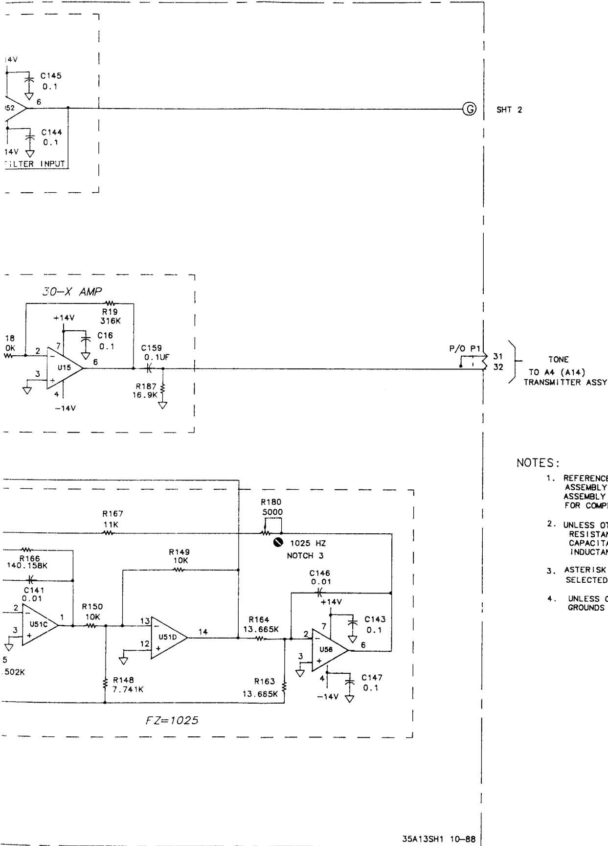
Figure 8-30 A3 Receiver Board Schematic Diagram (Sheet 1 of 4) 8-75
