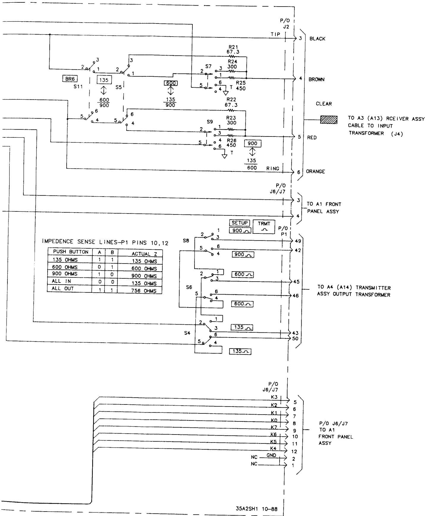
Figure 8-26. A2 Switchboard Schematic Diagram (Sheet 1 of 2) 8-71
